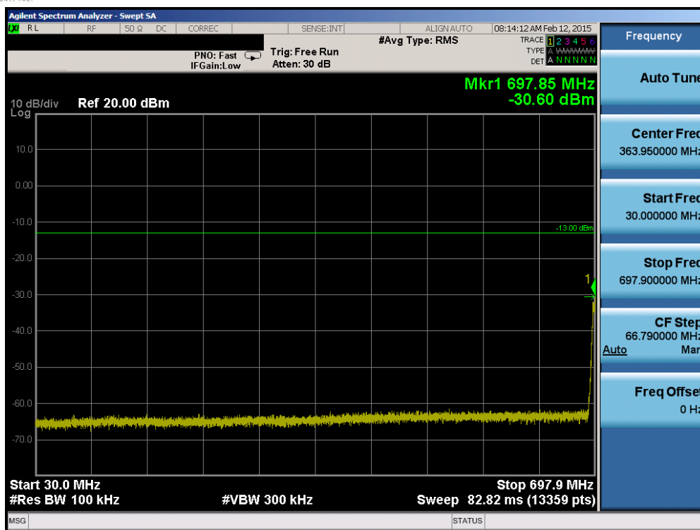
Plot 6-43. Conducted Spurious Plot (Band 12 – 5.0MHz QPSK – RB Size 1, RB Offset 0 – Low Channel)
