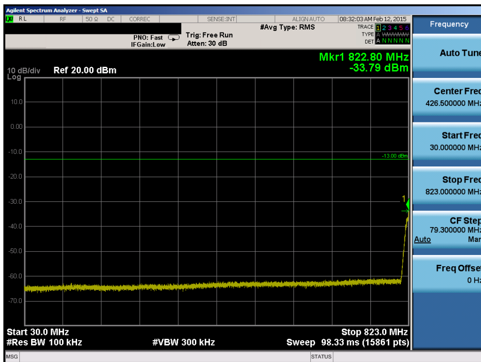
Plot 6-52. Conducted Spurious Plot (Band 26 – 10.0MHz QPSK – RB Size 1, RB Offset 0– Low Channel)
