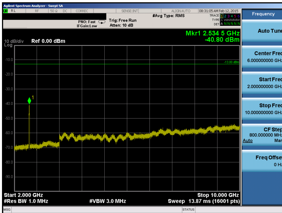
Plot 6-60. Conducted Spurious Plot (Band 26 – 10.0MHz QPSK – RB Size 1, RB Offset 0 – High Channel)
