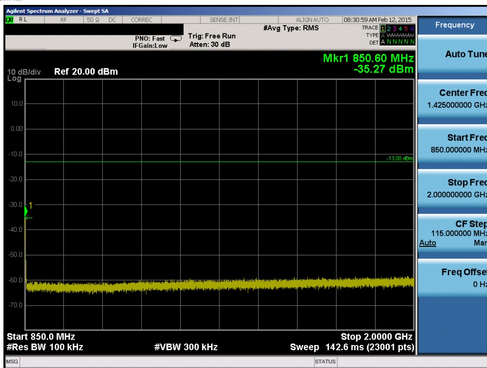
Plot 6-59. Conducted Spurious Plot (Band 26 – 10.0MHz QPSK – RB Size 1, RB Offset 0 – High Channel)
