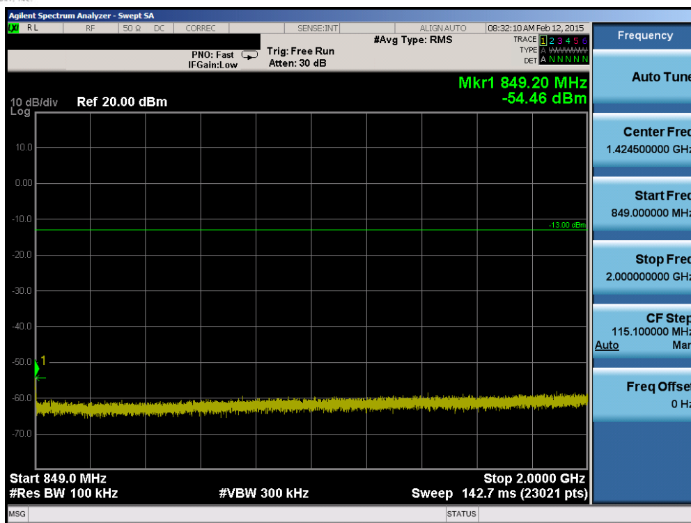
Plot 6-53. Conducted Spurious Plot (Band 26 – 10.0MHz QPSK – RB Size 1, RB Offset 0 – Low Channel)
