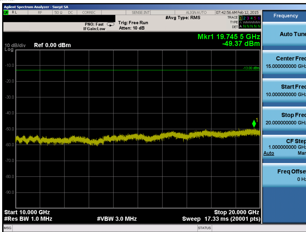
Plot 6-63. Conducted Spurious Plot (Band 4 – 3.0MHz QPSK – RB Size 1, RB Offset 0 – Low Channel)
