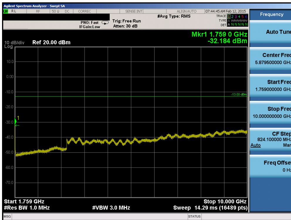
Plot 6-68. Conducted Spurious Plot (Band 4 – 3.0MHz QPSK – RB Size 1, RB Offset 0 – High Channel)
