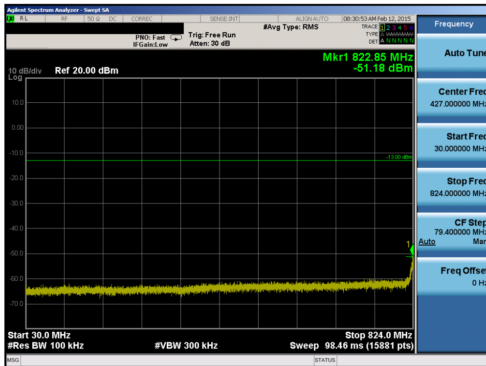
Plot 6-58. Conducted Spurious Plot (Band 26 – 10.0MHz QPSK – RB Size 1, RB Offset 0 – High Channel)
