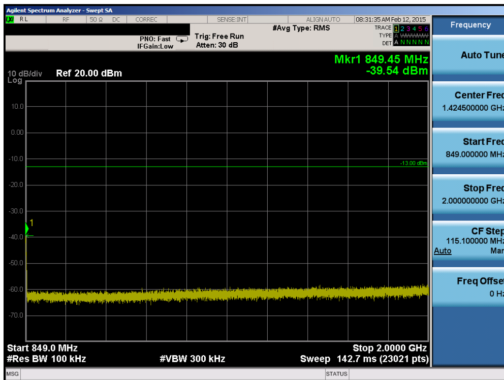
Plot 6-56. Conducted Spurious Plot (Band 26 – 10.0MHz QPSK – RB Size 1, RB Offset 0 – Mid Channel)
