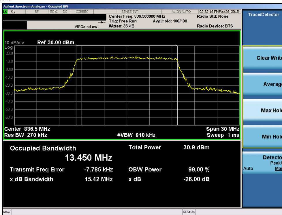
Plot 6-17. Occupied Bandwidth Plot (Band 26 – 15.0MHz QPSK – RB Size 75)
