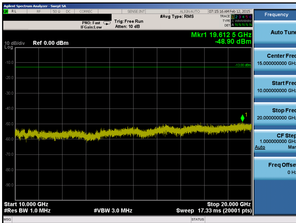
Plot 6-72. Conducted Spurious Plot (Band 2 – 20.0MHz QPSK – RB Size 1, RB Offset 0 – Low Channel)
