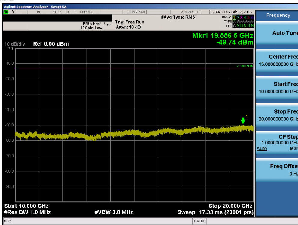
Plot 6-69. Conducted Spurious Plot (Band 4 – 3.0MHz QPSK – RB Size 1, RB Offset 0 – High Channel)
