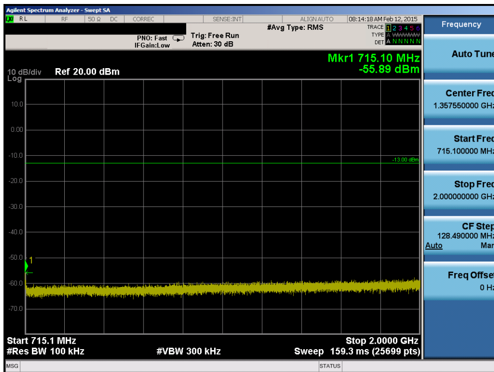
Plot 6-44. Conducted Spurious Plot (Band 12 – 5.0MHz QPSK – RB Size 1, RB Offset 0 – Low Channel)
