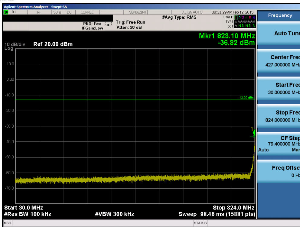
Plot 6-55. Conducted Spurious Plot (Band 26 – 10.0MHz QPSK – RB Size 1, RB Offset 0 – Mid Channel)
