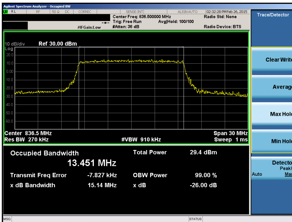
Plot 6-18. Occupied Bandwidth Plot (Band 26 – 15.0MHz 16-QAM – RB Size 75)
