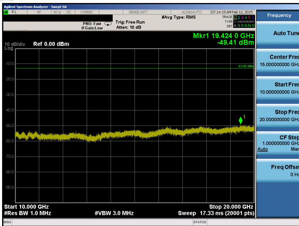
Plot 6-75. Conducted Spurious Plot (Band 2 – 20.0MHz QPSK – RB Size 1, RB Offset 0 – Mid Channel)
