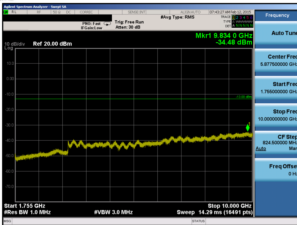
Plot 6-65. Conducted Spurious Plot (Band 4 – 3.0MHz QPSK – RB Size 1, RB Offset 0 – Mid Channel)
