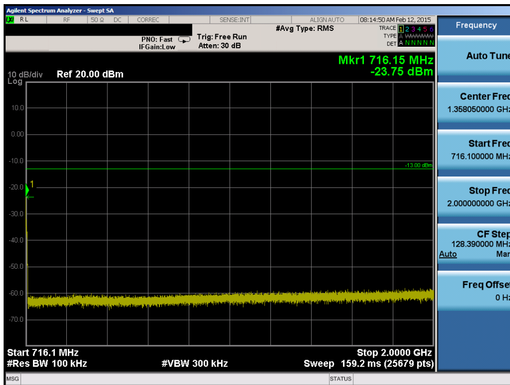
Plot 6-50. Conducted Spurious Plot (Band 12 – 5.0MHz QPSK – RB Size 1, RB Offset 0 – High Channel)
