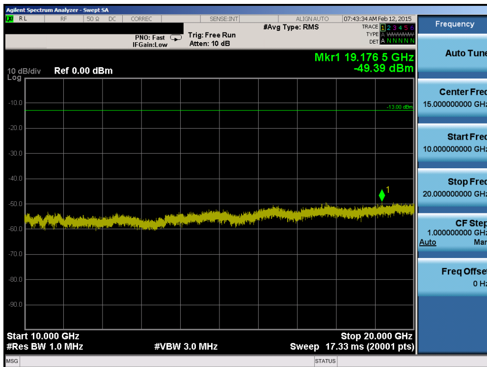
Plot 6-66. Conducted Spurious Plot (Band 4 – 3.0MHz QPSK – RB Size 1, RB Offset 0 – Mid Channel)
