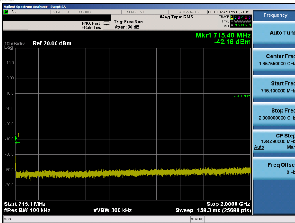
Plot 6-47. Conducted Spurious Plot (Band 12 – 5.0MHz QPSK – RB Size 1, RB Offset 0 – Mid Channel)
