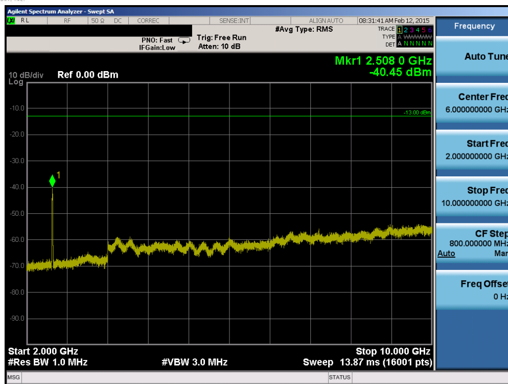
Plot 6-57. Conducted Spurious Plot (Band 26 – 10.0MHz QPSK – RB Size 1, RB Offset 0 – Mid Channel)
