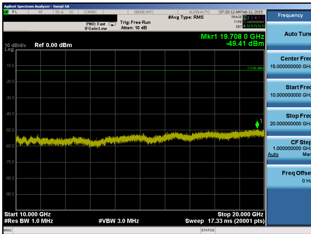
Plot 6-78. Conducted Spurious Plot (Band 2 – 20.0MHz QPSK – RB Size 1, RB Offset 0 – High Channel)
