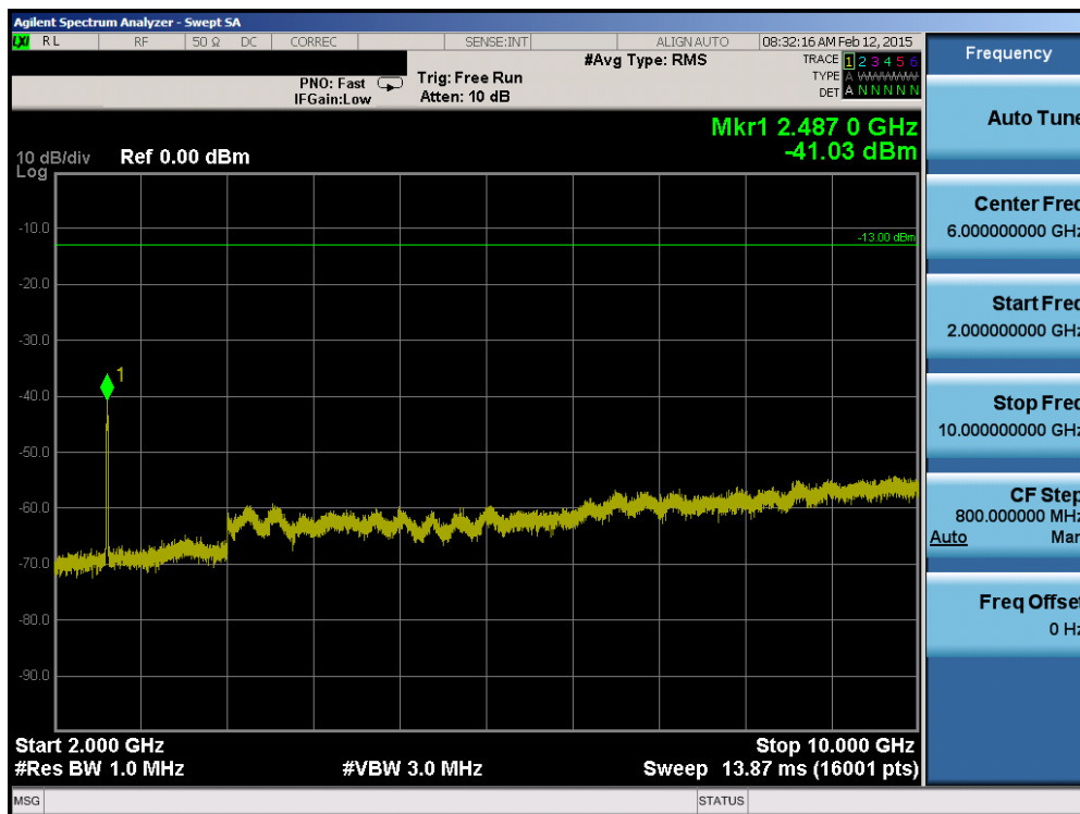
Plot 6-54. Conducted Spurious Plot (Band 26 – 10.0MHz QPSK – RB Size 1, RB Offset 0 – Low Channel)
