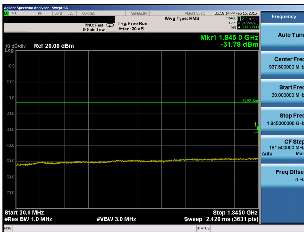
Plot 6-34. Conducted Spurious Plot (PCS WCDMA Mode – Ch. 9262)
