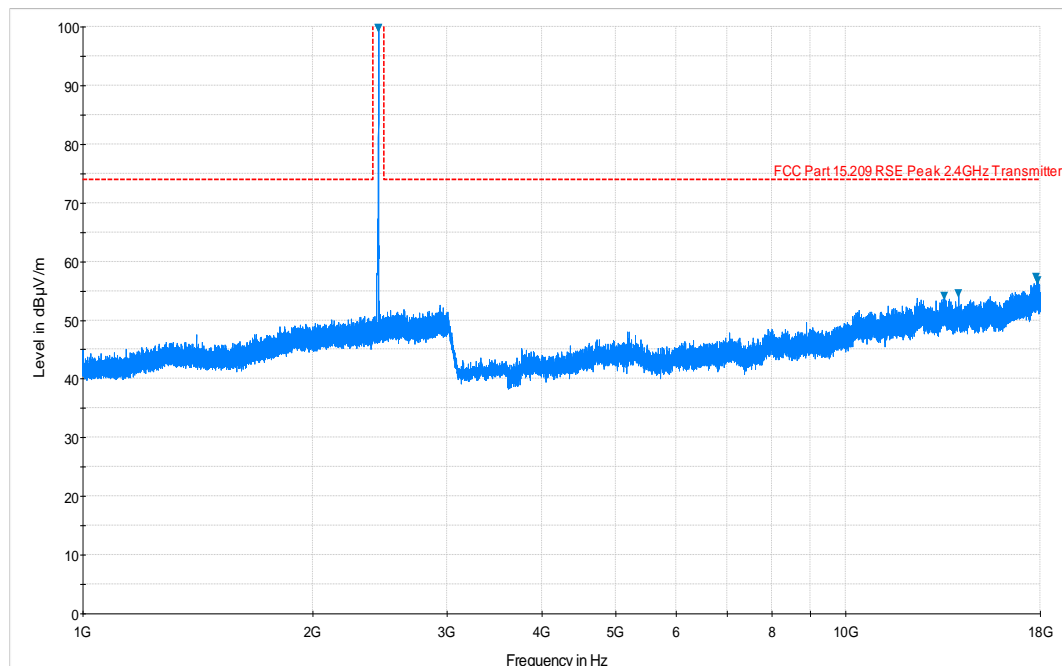
Plot 6-20. Radiated Spurious Plot above 1GHz (BTLE – Ch. 19, Ant. Pol. H)
