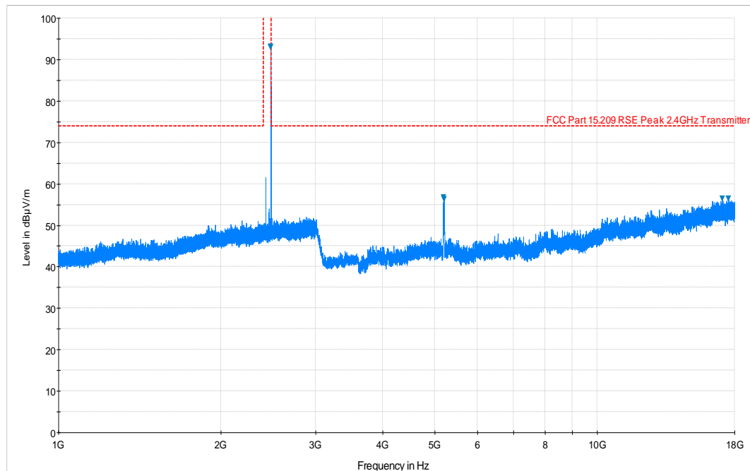
Plot 6-23. Radiated Spurious Plot above 1GHz (BTLE – Ch. 39, Ant. Pol. V)
