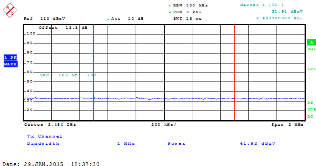
Plot 6-26. Radiated Restricted Upper Band Edge Measurement (Average)
