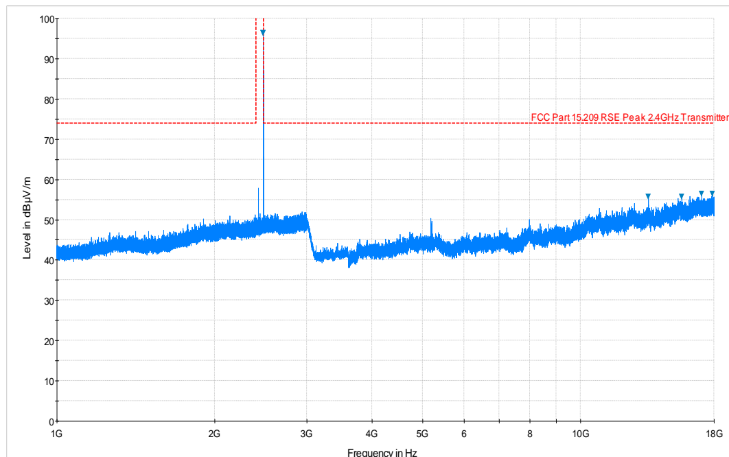
Plot 6-22. Radiated Spurious Plot above 1GHz (BTLE – Ch. 39, Ant. Pol. H)
