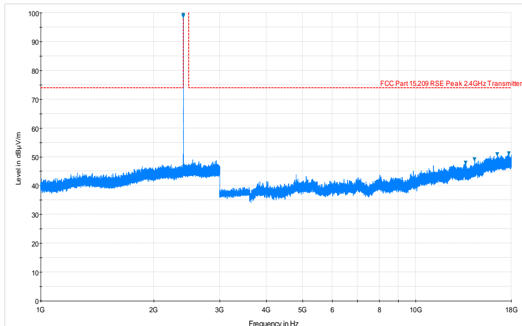
Plot 6-18. Radiated Spurious Plot above 1GHz (BTLE – Ch. 0, Ant. Pol. H)
