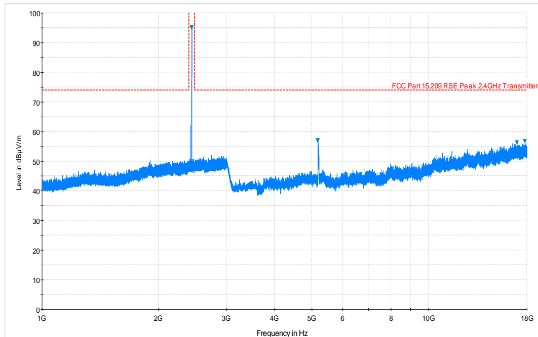
Plot 6-21. Radiated Spurious Plot above 1GHz (BTLE – Ch. 19, Ant. Pol. V)
