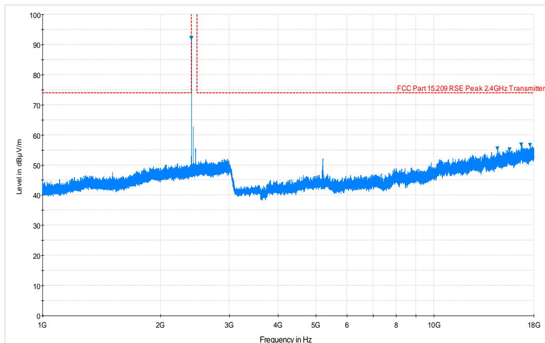
Plot 6-19. Radiated Spurious Plot above 1GHz (BTLE – Ch. 0, Ant. Pol. V)
