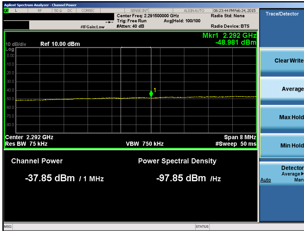
Plot 6-174. Lower Extended Band Edge Plot (Band 30 – 10MHz QPSK – RB Size 50)
