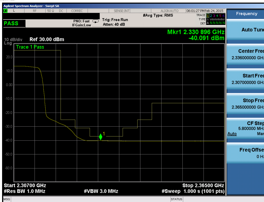
Plot 6-176. Upper Extended Band Edge Plot (Band 30 – 10MHz QPSK – RB Size 50)
