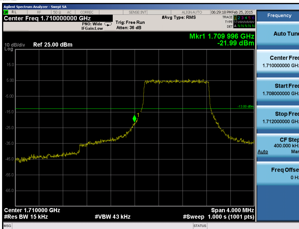
Plot 6-118. Lower Band Edge Plot (Band 4 – 1.4MHz QPSK – RB Size 6)
