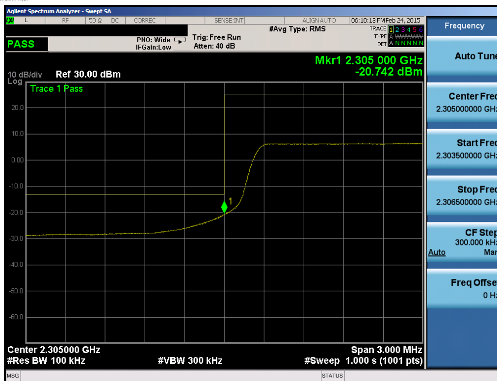
Plot 6-166. Lower Band Edge Plot (Band 30 – 5MHz QPSK – RB Size 25)
