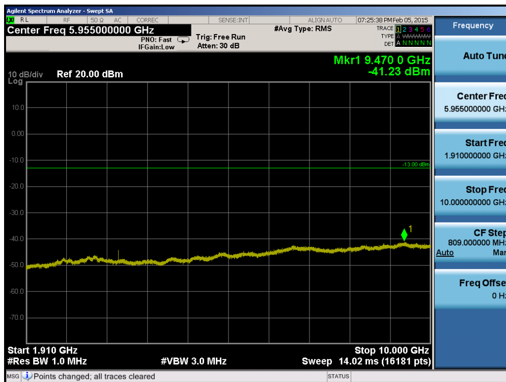
Plot 6-76. Conducted Spurious Plot (Band 2 – 5.0MHz QPSK – RB Size 1, RB Offset 0 – Mid Channel)
