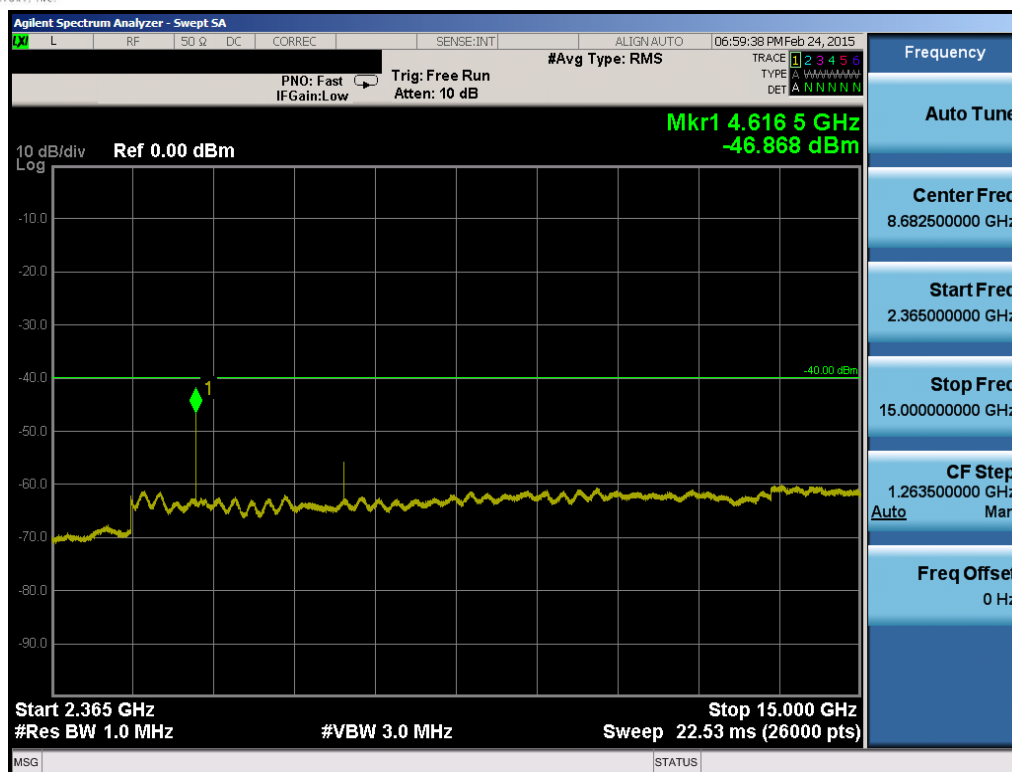
Plot 6-85. Conducted Spurious Plot (Band 30 – 5.0MHz QPSK – RB Size 1, RB Offset 0 – Mid Channel)
