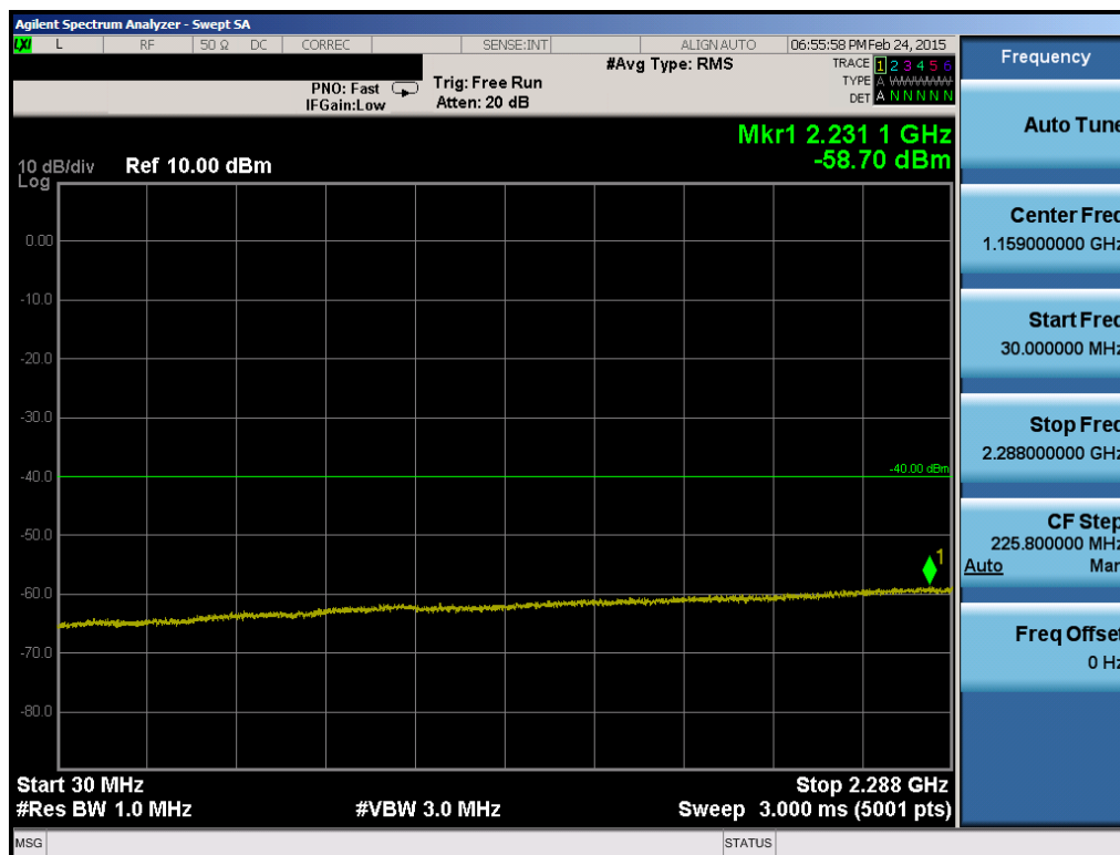
Plot 6-84. Conducted Spurious Plot (Band 30 – 5.0MHz QPSK – RB Size 1, RB Offset 0 – Mid Channel)
