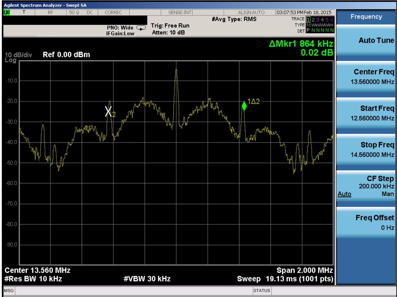
Figure 7-3. 20dB Bandwidth Plot with WCC
