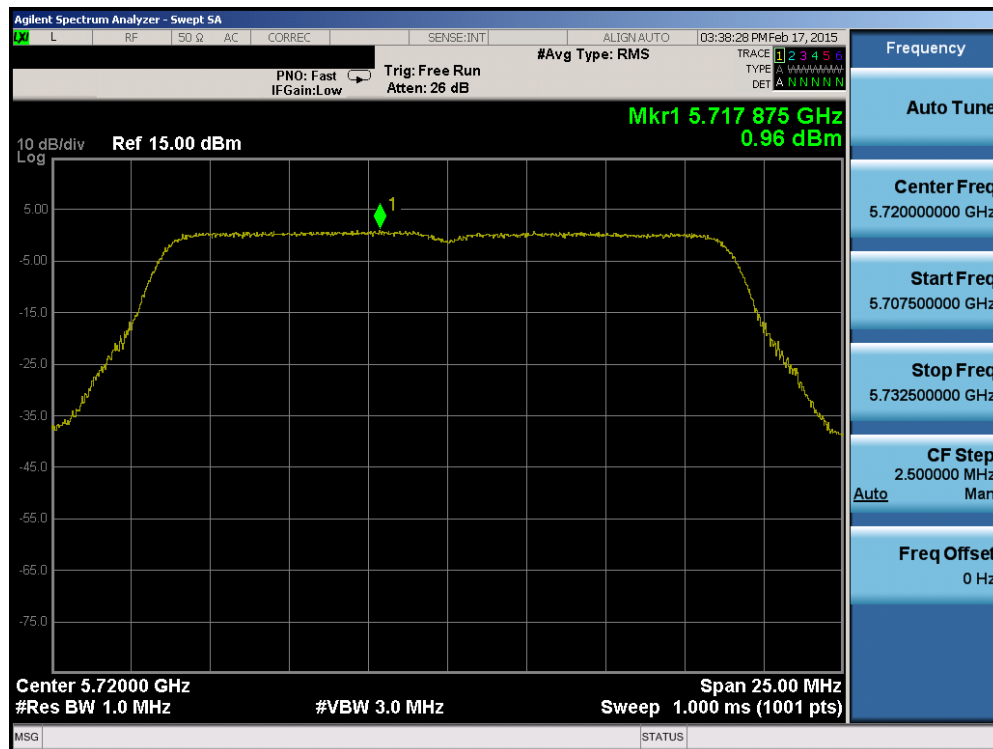
Plot 6-138. Power Spectral Density Plot (20MHz 802.11n (UNII Band 2C) – Ch. 144)
