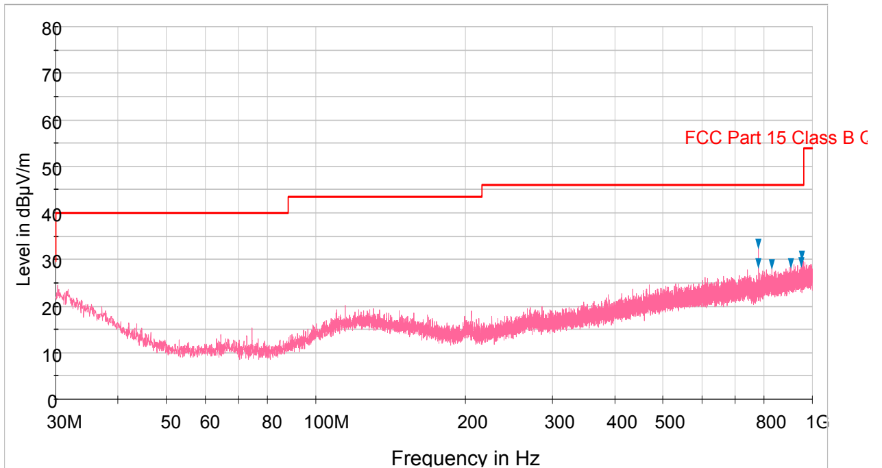
Plot 6-239. Radiated Spurious Plot below 1GHz (802.11a – U3 Ch. 157, Ant. Pol. V)
