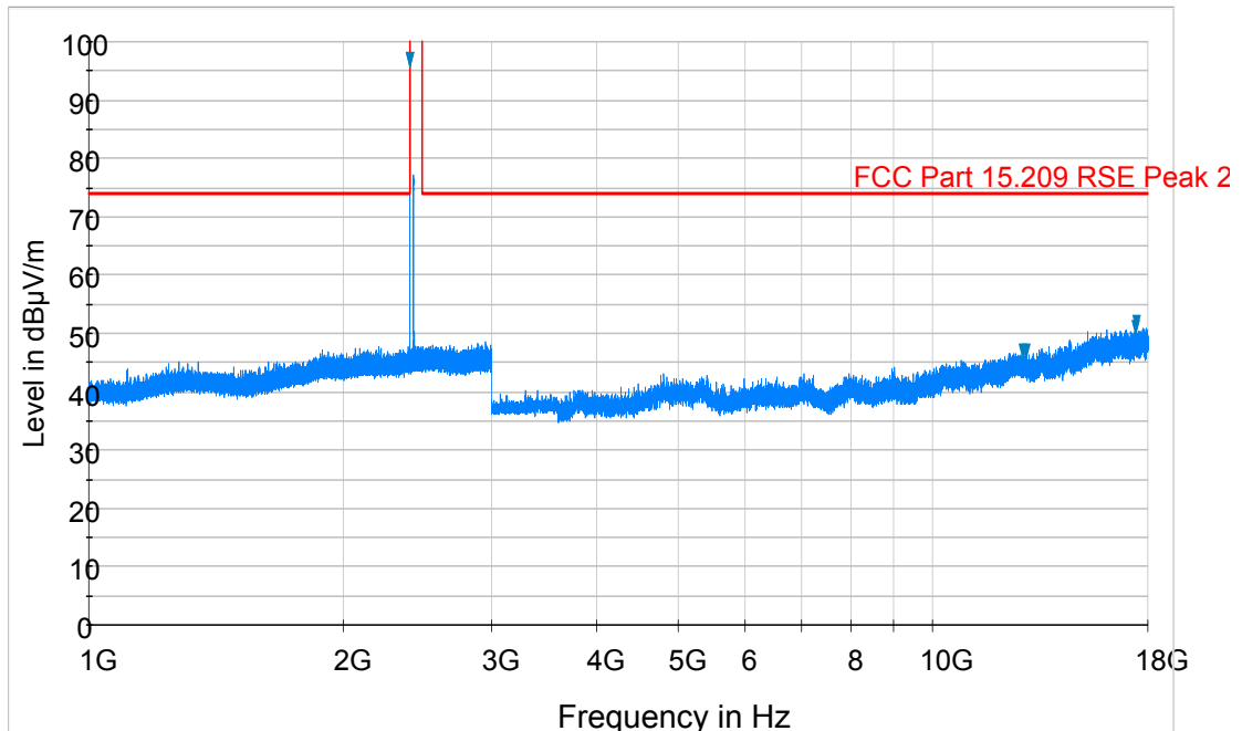
Plot 6-19. Radiated Spurious Plot above 1GHz (BTLE – Ch. 0, Ant. Pol. V)
