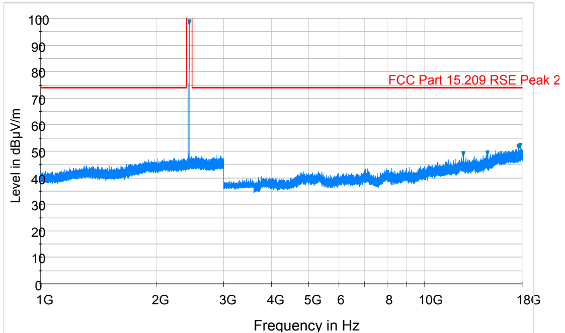
Plot 6-20. Radiated Spurious Plot above 1GHz (BTLE – Ch. 19, Ant. Pol. H)
