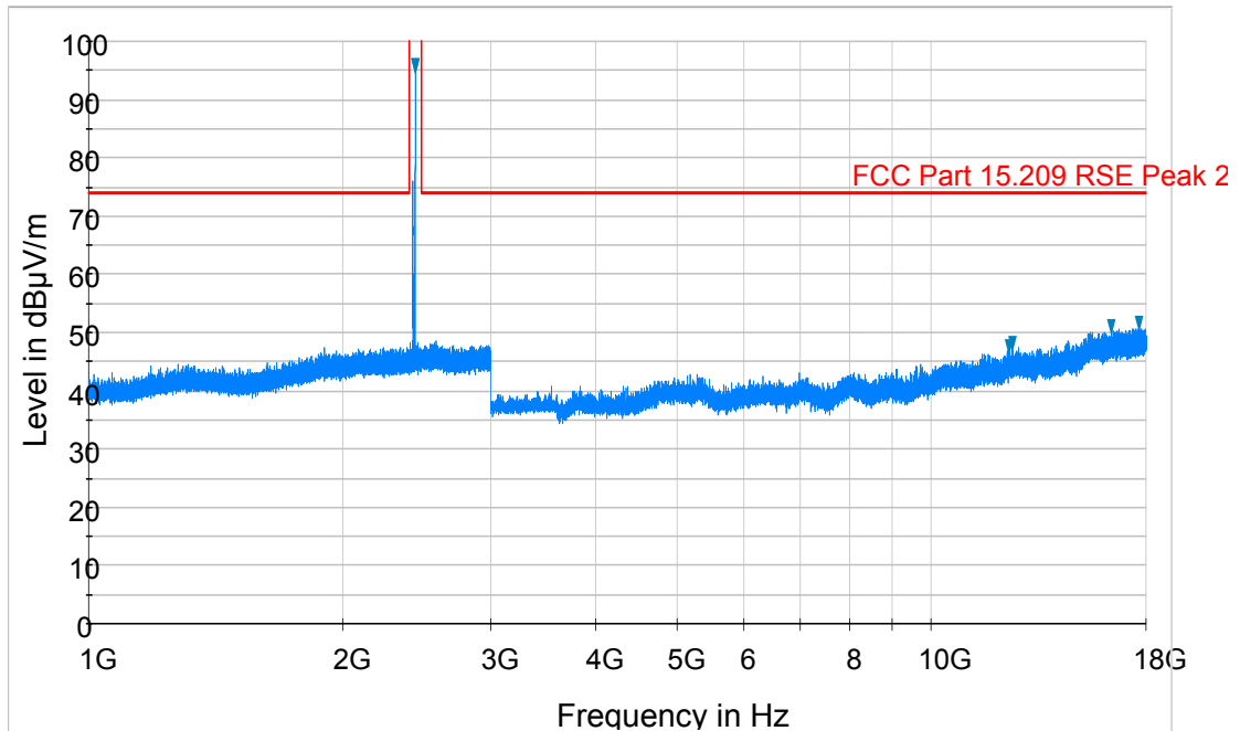
Plot 6-21. Radiated Spurious Plot above 1GHz (BTLE – Ch. 19, Ant. Pol. V)
