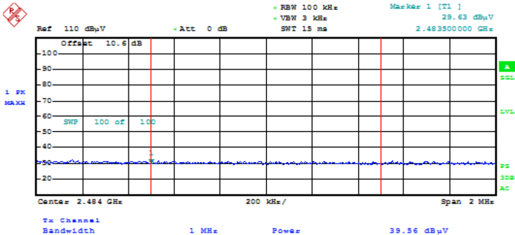
Plot 6-26. Radiated Restricted Upper Band Edge Measurement (Average)
