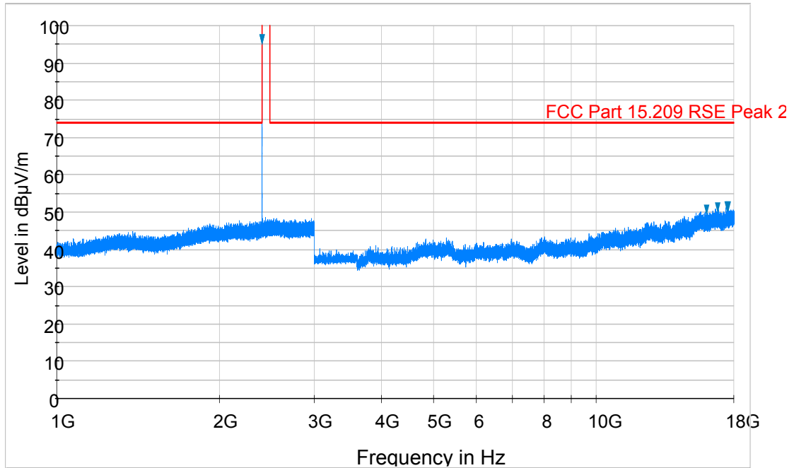
Plot 6-18. Radiated Spurious Plot above 1GHz (BTLE – Ch. 0, Ant. Pol. H)
