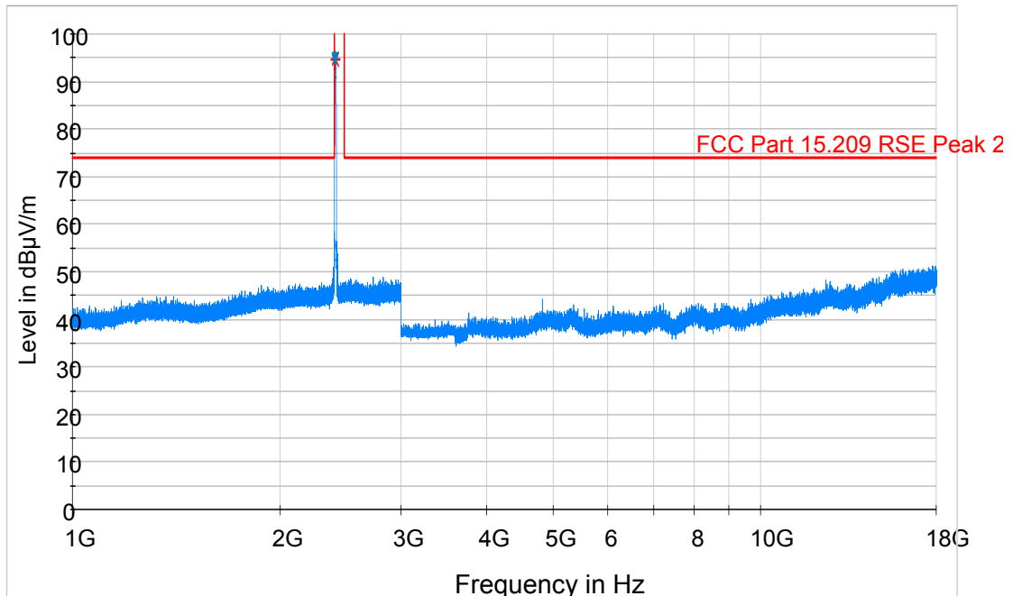
Plot 6-70. Radiated Spurious Plot above 1GHz (802.11b – Ch. 1, Ant. Pol. V)
