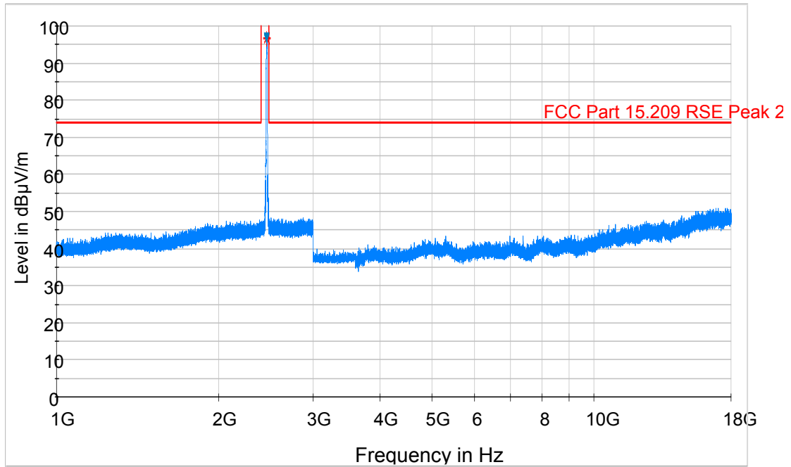
Plot 6-73. Radiated Spurious Plot above 1GHz (802.11b – Ch. 11, Ant. Pol. H)
