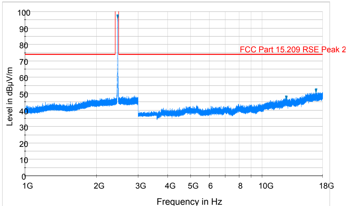
Plot 6-74. Radiated Spurious Plot above 1GHz (802.11b – Ch. 11, Ant. Pol. V)
