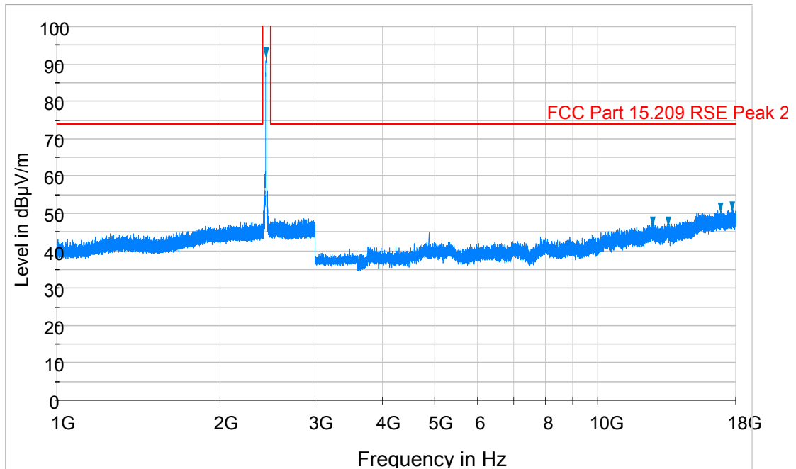
Plot 6-72. Radiated Spurious Plot above 1GHz (802.11b – Ch. 6, Ant. Pol. V)
