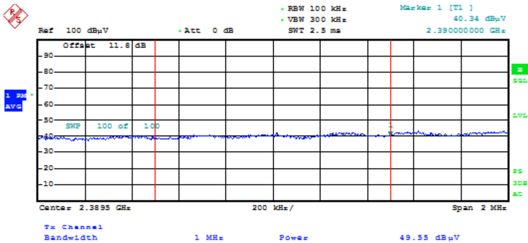
Plot 6-77. Radiated Restricted Lower Band Edge Measurement (Average)
