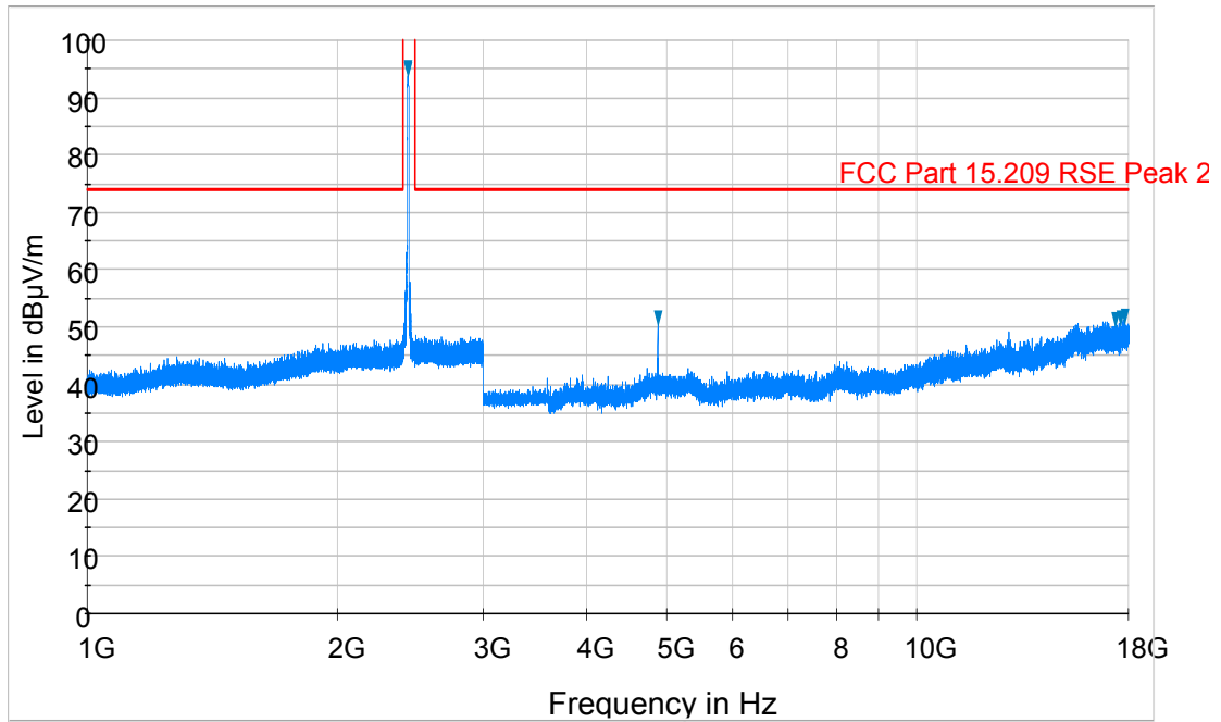
Plot 6-71. Radiated Spurious Plot above 1GHz (802.11b – Ch. 6, Ant. Pol. H)
