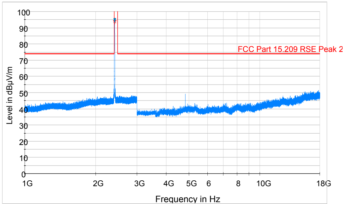
Plot 6-62. Radiated Spurious Plot above 1GHz (802.11b – Ch. 1, Ant. Pol. V)
