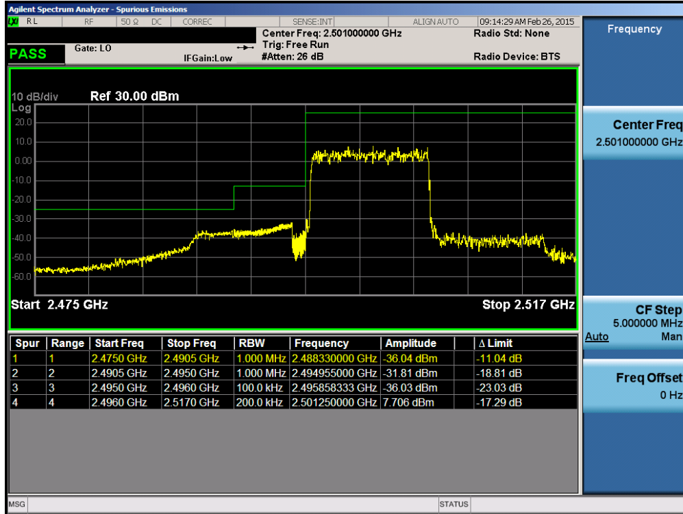
Plot 6-65. Lower Channel Edge Plot (Band 41 – 10.0MHz QPSK – RB Size 50)
