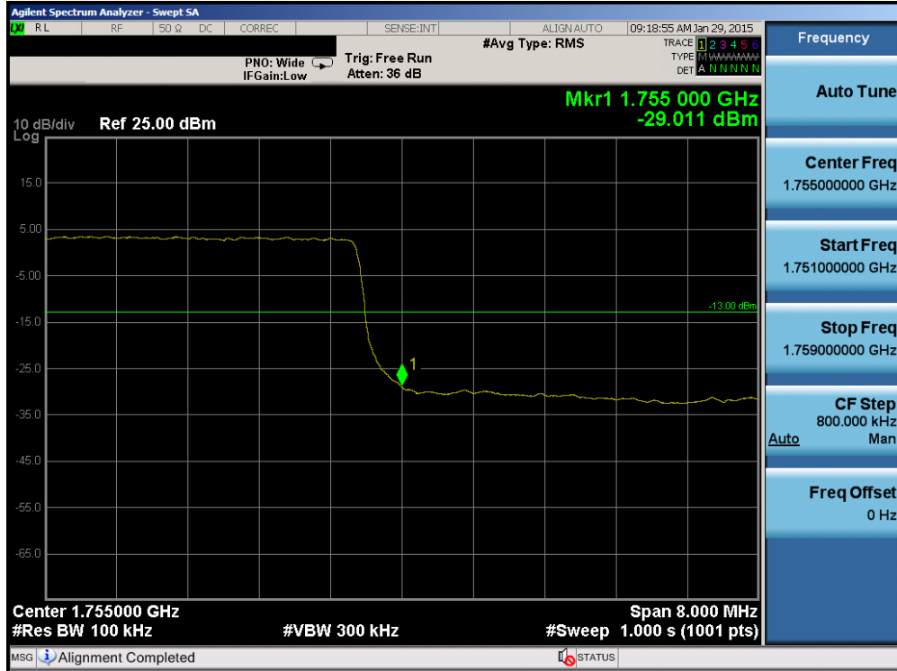
Plot 6-53. Upper Band Edge Plot (Band 4 – 10.0MHz QPSK – RB Size 50)
