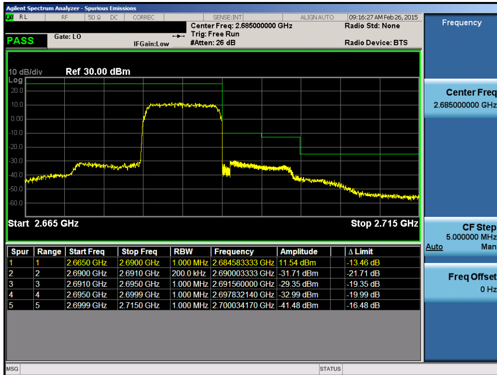
Plot 6-66. Upper Channel Edge Plot (Band 41 – 10.0MHz QPSK – RB Size 50)
