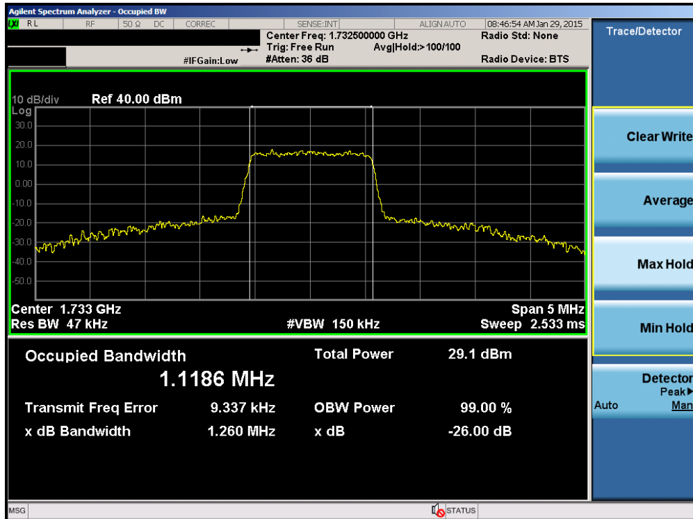
Plot 6-2. Occupied Bandwidth Plot (Band 4 – 1.4MHz 16-QAM – RB Size 6)
