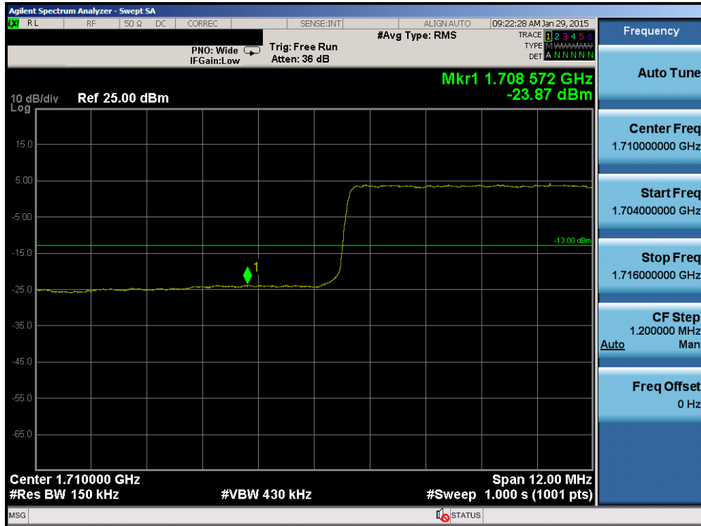
Plot 6-55. Lower Band Edge Plot (Band 4 – 15.0MHz QPSK – RB Size 75)
