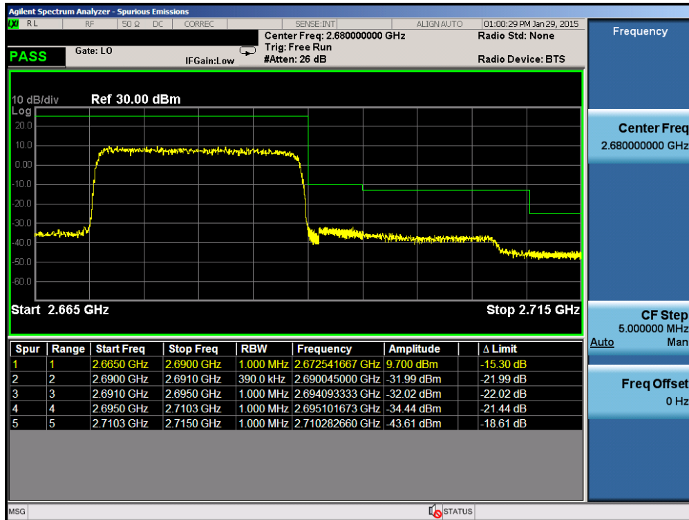
Plot 6-70. Upper Channel Edge Plot (Band 41 – 20.0MHz QPSK – RB Size 100)
