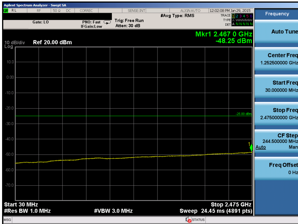
Plot 6-30. Conducted Spurious Plot (Band 41 – 10.0MHz QPSK – RB Size 1, RB Offset 0– Low Channel)
