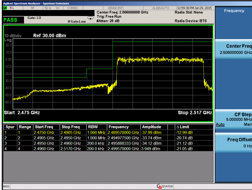
Plot 6-69. Lower Channel Edge Plot (Band 41 – 20.0MHz QPSK – RB Size 100)
