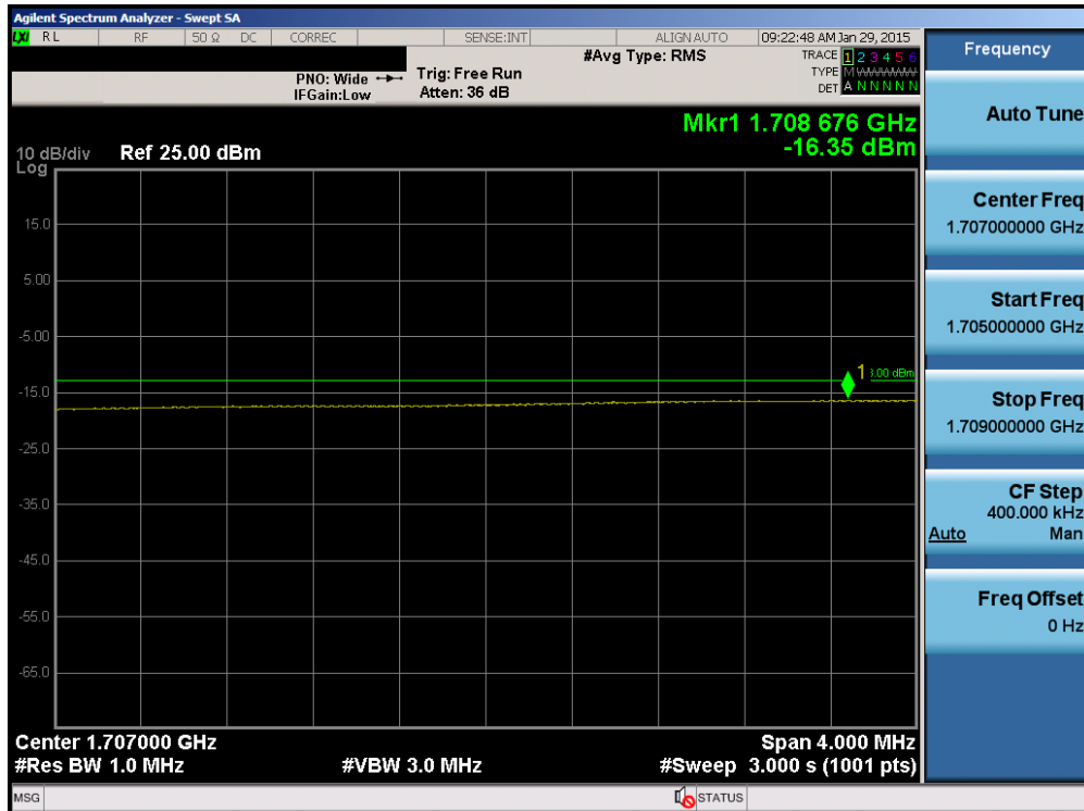
Plot 6-56. Lower Extended Band Edge Plot (Band 4 – 15.0MHz QPSK – RB Size 75)
