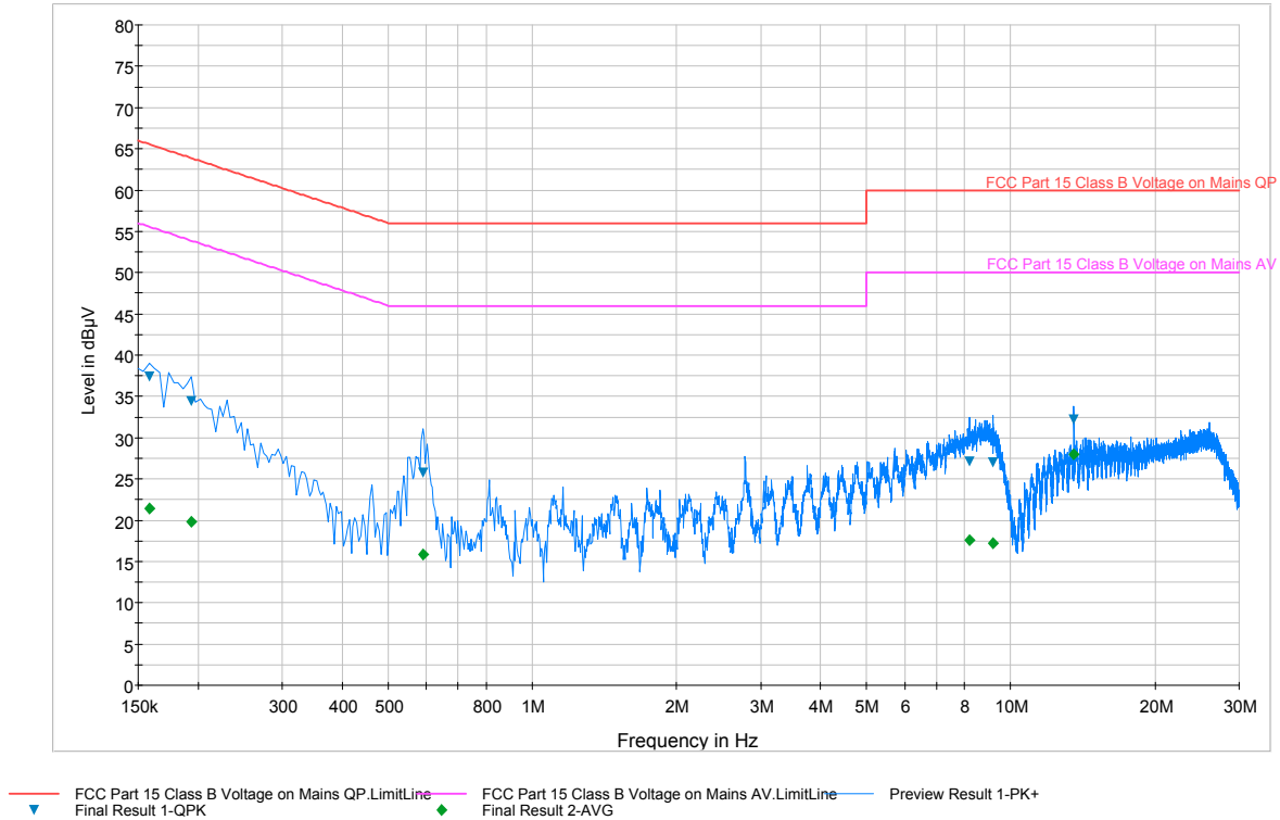
Plot 8-2. Line-Conducted Test Plot (N)
