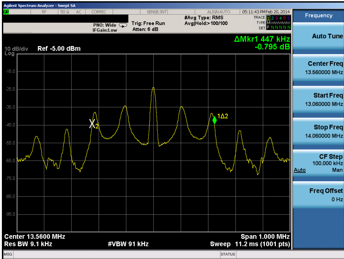
Figure 8-3. 20dB Bandwidth Plot with WCC
