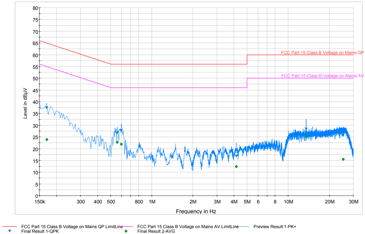
Plot 8-1. Line-Conducted Test Plot (L1)
