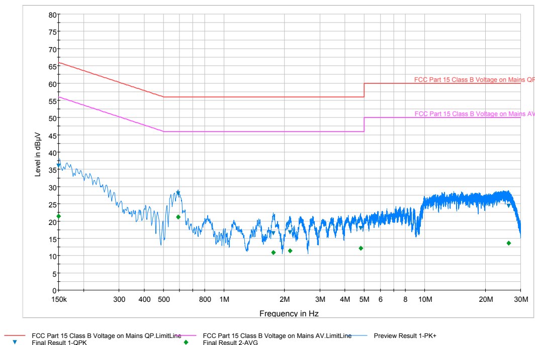
Plot 6-22. Line Conducted Plot with Bluetooth LE (L1)
