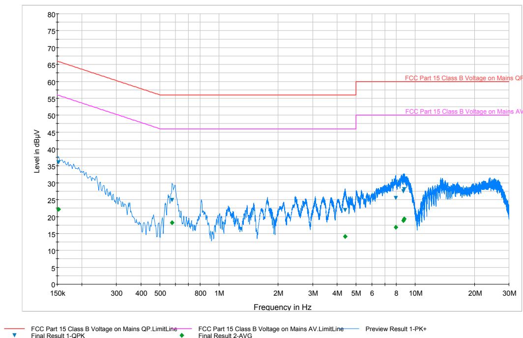
Plot 6-23. Line Conducted Plot with Bluetooth LE (N)
