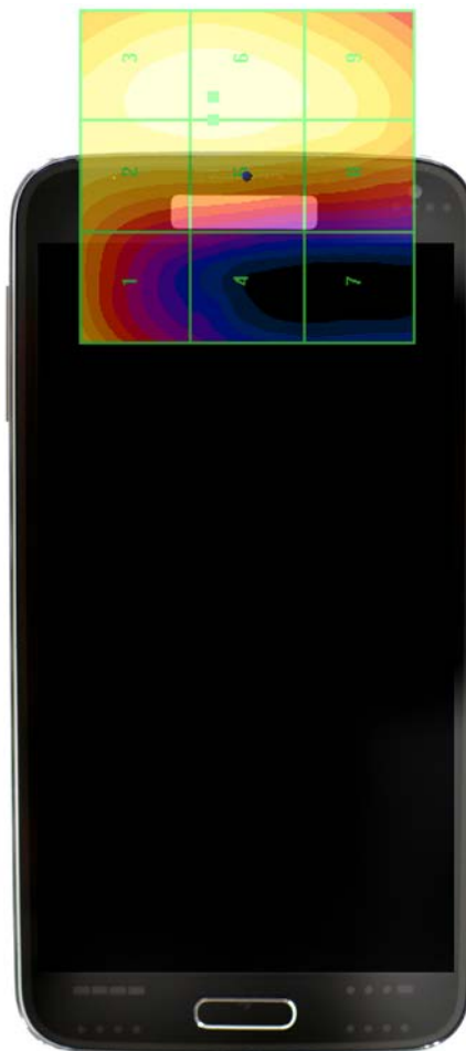
Figure 18-4 E-Field WD Scan overlay
