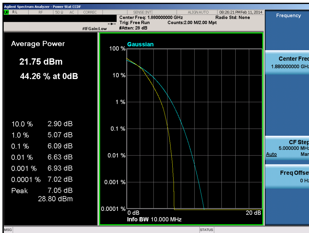
Plot 6-140. PAR Plot (Band 2 – 10.0MHz 16-QAM – RB Size 50)
