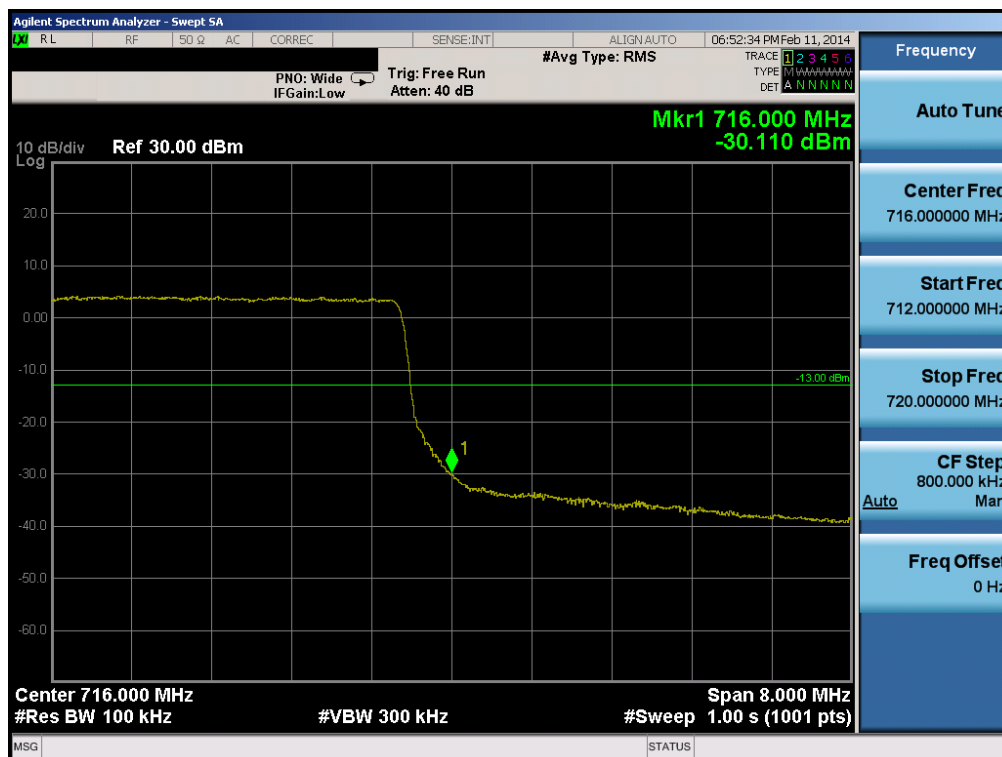
Plot 6-64. Upper Band Edge Plot (Band 17 – 10.0MHz QPSK – RB Size 50)
