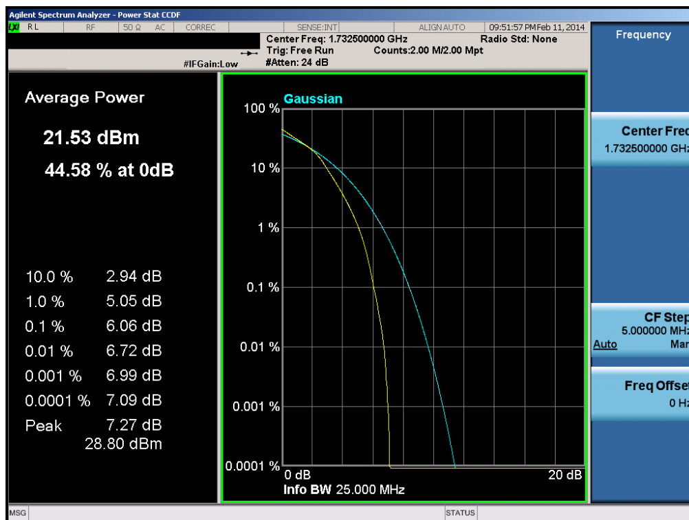
Plot 6-132. PAR Plot (Band 4 – 20.0MHz 16-QAM – RB Size 100)
