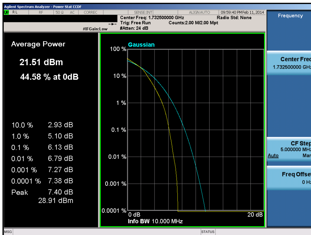
Plot 6-128. PAR Plot (Band 4 – 10.0MHz 16-QAM – RB Size 50)
