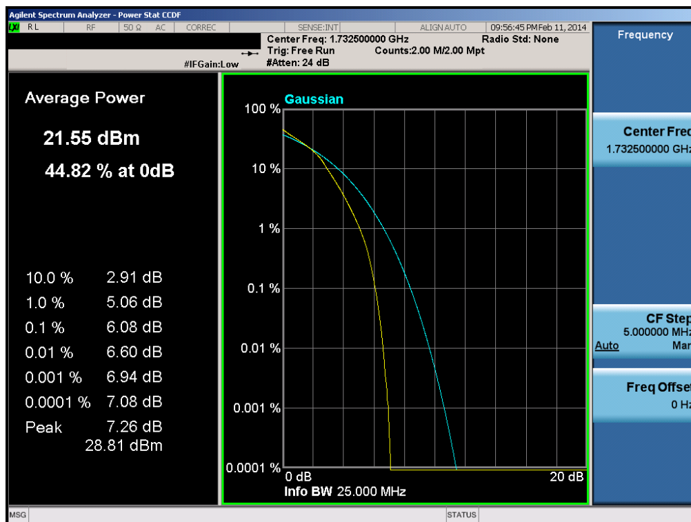
Plot 6-130. PAR Plot (Band 4 – 15.0MHz 16-QAM – RB Size 75)
