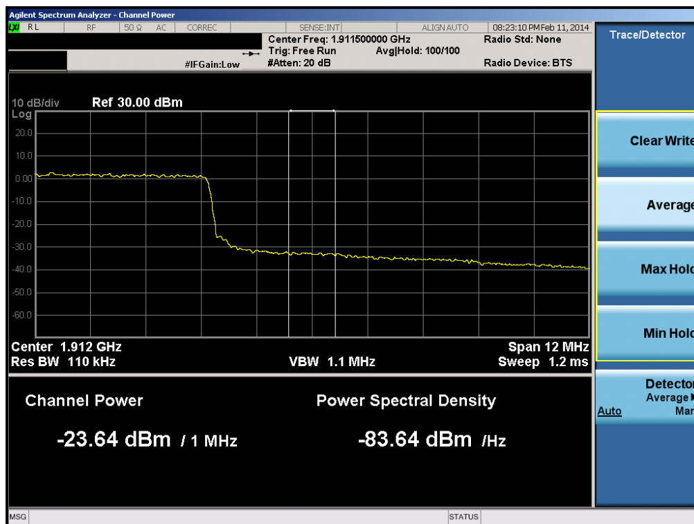
Plot 6-116. Upper Extended Band Edge Plot (Band 2 – 15.0MHz QPSK – RB Size 75)
