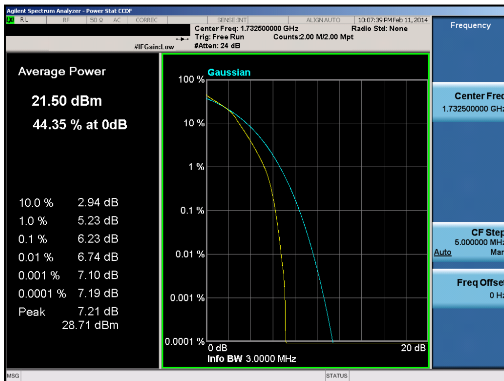
Plot 6-124. PAR Plot (Band 4 – 3.0MHz 16-QAM – RB Size 15)
