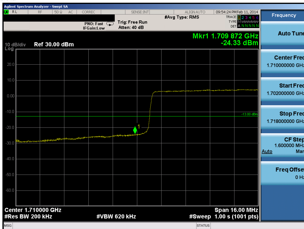
Plot 6-93. Lower Band Edge Plot (Band 4 – 20.0MHz QPSK – RB Size 100)
