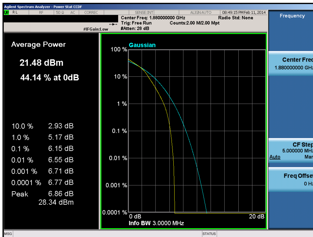
Plot 6-136. PAR Plot (Band 2 – 3.0MHz 16-QAM – RB Size 15)
