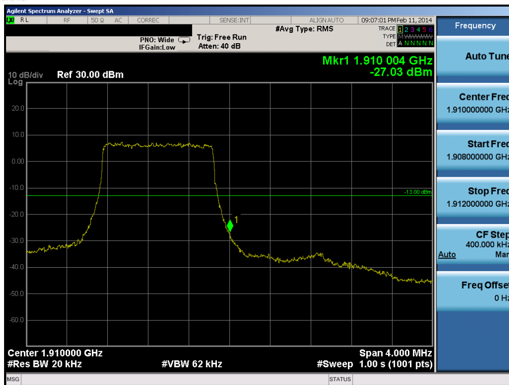
Plot 6-99. Upper Band Edge Plot (Band 2 – 1.4MHz QPSK – RB Size 6)
