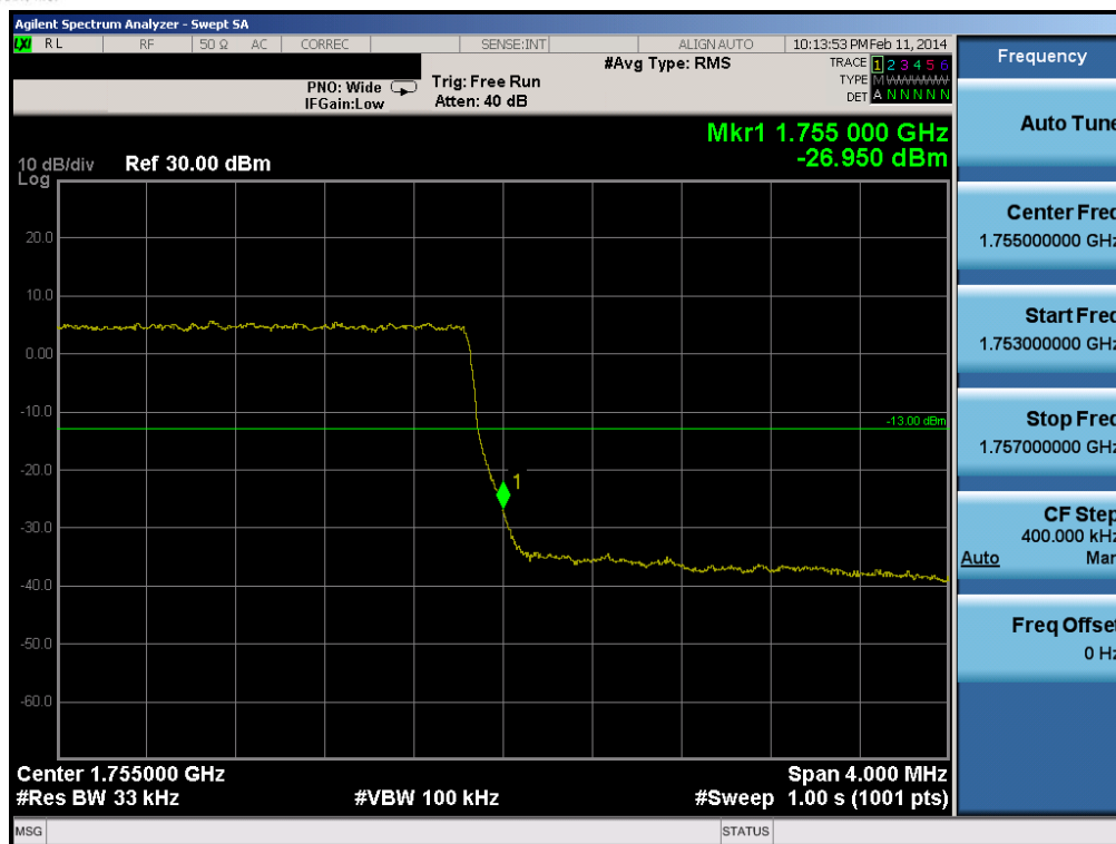
Plot 6-79. Upper Band Edge Plot (Band 4 – 3.0MHz QPSK – RB Size 15)
