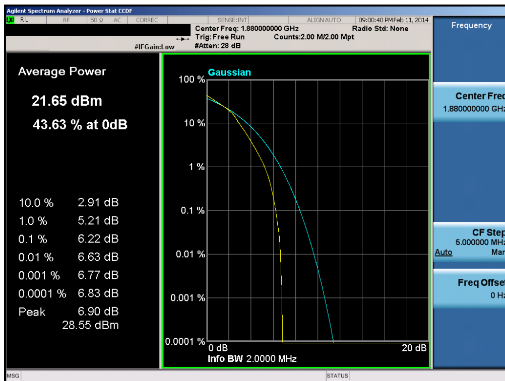
Plot 6-134. PAR Plot (Band 2 – 1.4MHz 16-QAM – RB Size 6)
