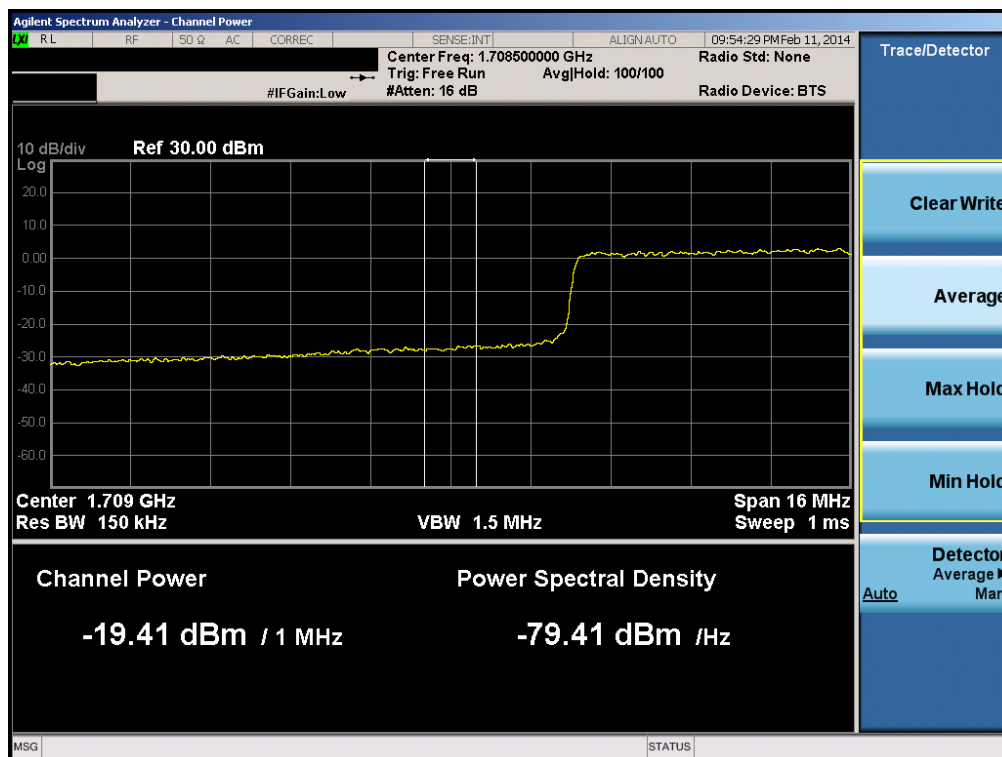
Plot 6-94. Lower Extended Band Edge Plot (Band 4 – 20.0MHz QPSK – RB Size 100)
