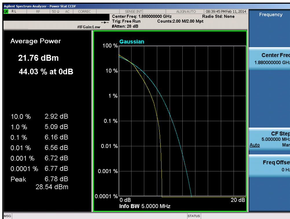
Plot 6-138. PAR Plot (Band 2 – 5.0MHz 16-QAM – RB Size 25)
