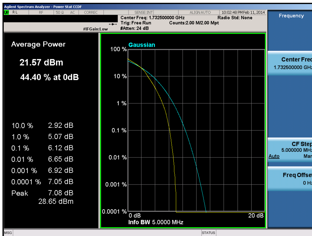
Plot 6-126. PAR Plot (Band 4 – 5.0MHz 16-QAM – RB Size 25)
