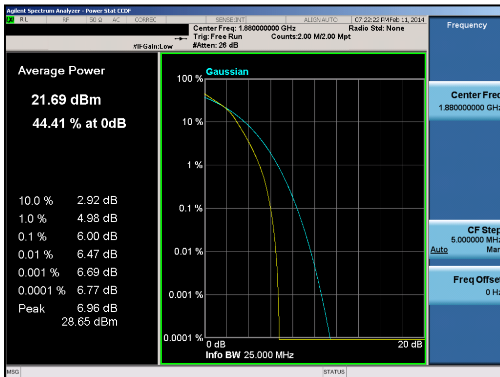
Plot 6-144. PAR Plot (Band 2 – 20.0MHz 16-QAM – RB Size 100)
