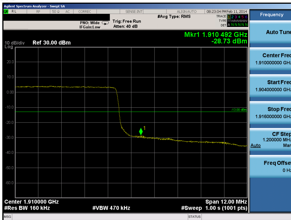
Plot 6-115. Upper Band Edge Plot (Band 2 – 15.0MHz QPSK – RB Size 75)
