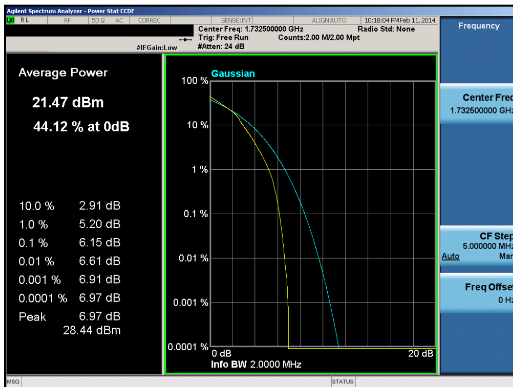
Plot 6-122. PAR Plot (Band 4 – 1.4MHz 16-QAM – RB Size 6)
