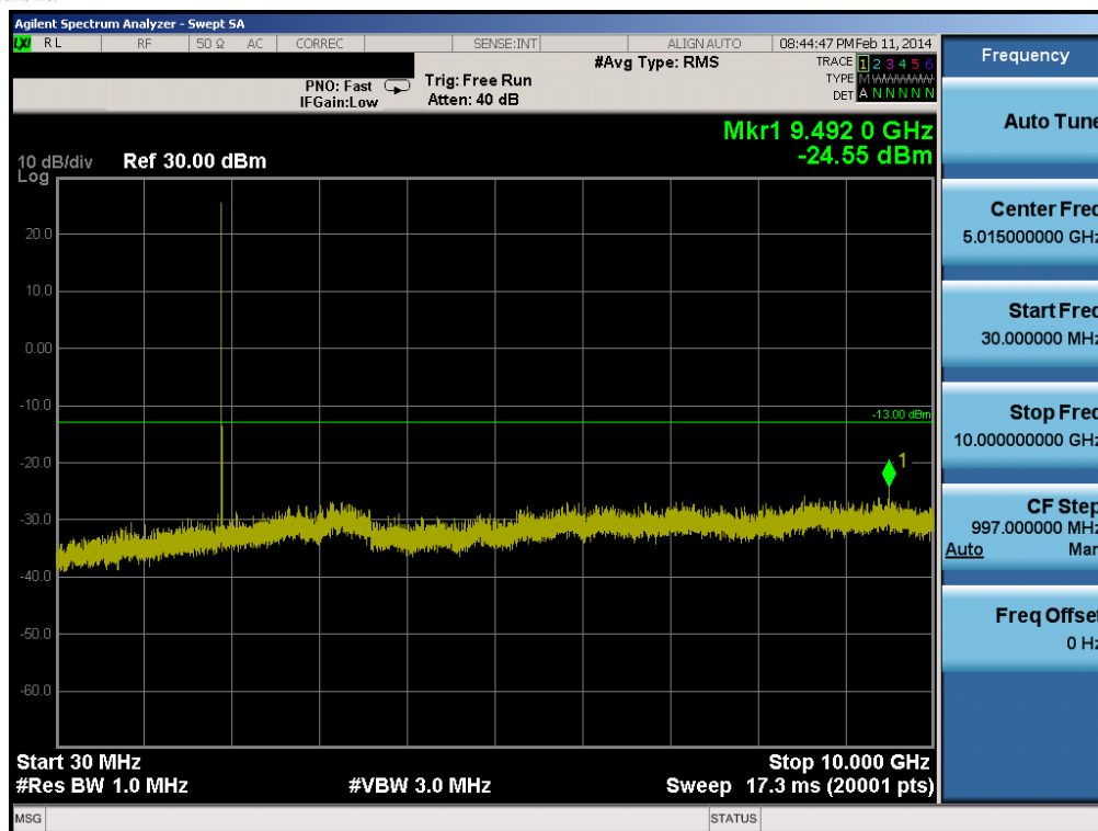
Plot 6-59. Conducted Spurious Plot (Band 2 – 5.0MHz QPSK – RB Size 1, RB Offset 0 – High Channel)
