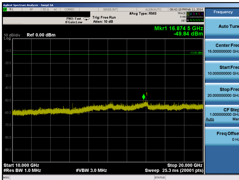
Plot 6-58. Conducted Spurious Plot (Band 2 – 5.0MHz QPSK – RB Size 1, RB Offset 0 – Mid Channel)
