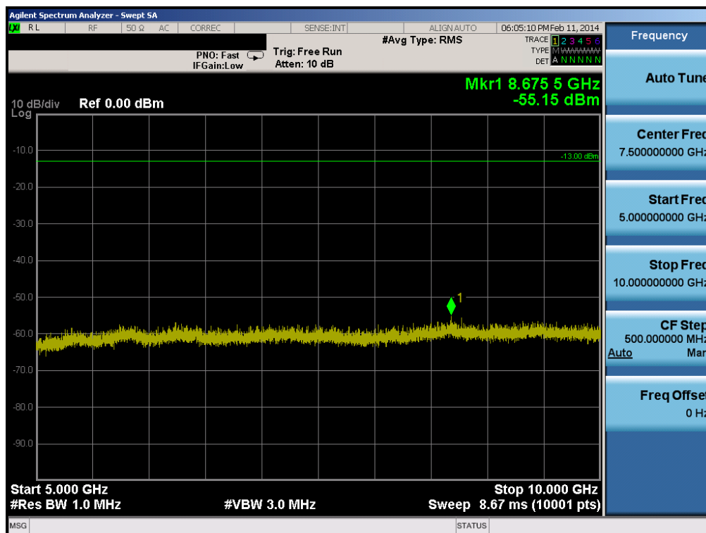
Plot 6-48. Conducted Spurious Plot (Band 5 – 3.0MHz QPSK – RB Size 1, RB Offset 0 – High Channel)
