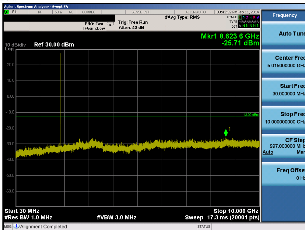
Plot 6-55. Conducted Spurious Plot (Band 2 – 5.0MHz QPSK – RB Size 1, RB Offset 0 – Low Channel)
