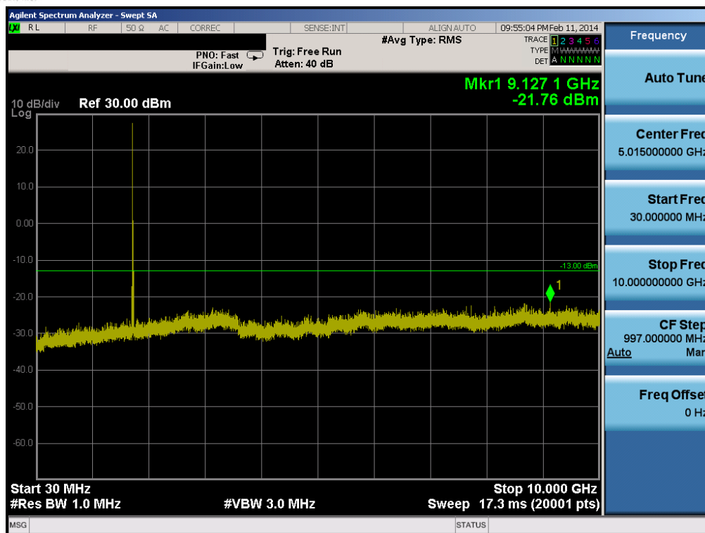
Plot 6-53. Conducted Spurious Plot (Band 4 – 5.0MHz QPSK – RB Size 1, RB Offset 0 – High Channel)
