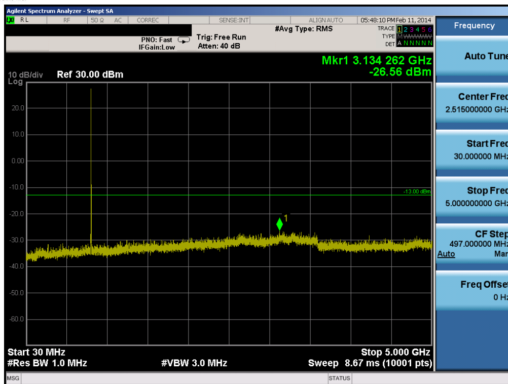
Plot 6-43. Conducted Spurious Plot (Band 5 – 3.0MHz QPSK – RB Size 1, RB Offset 0 – Low Channel)
