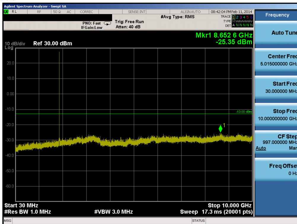
Plot 6-57. Conducted Spurious Plot (Band 2 – 5.0MHz QPSK – RB Size 1, RB Offset 0 – Mid Channel)
