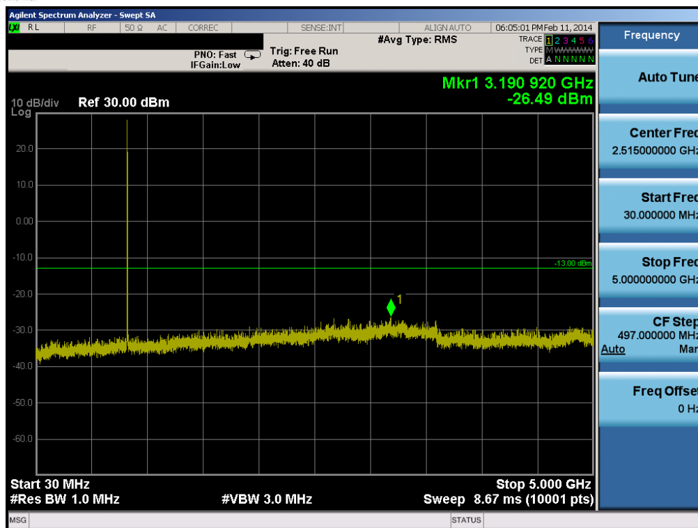
Plot 6-47. Conducted Spurious Plot (Band 5 – 3.0MHz QPSK – RB Size 1, RB Offset 0 – High Channel)
