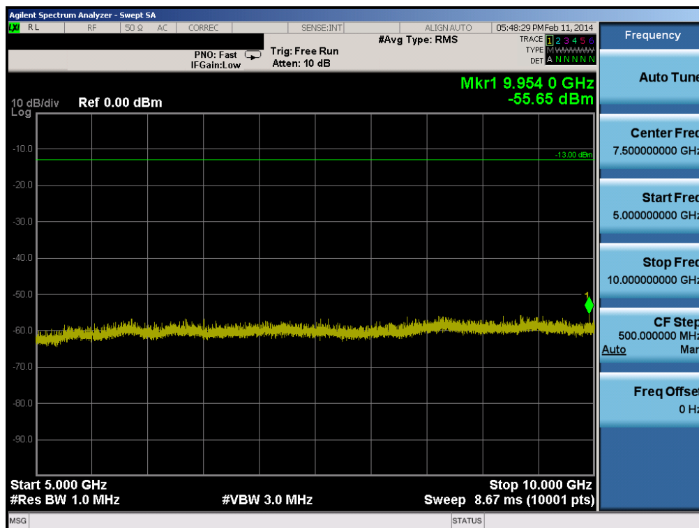
Plot 6-44. Conducted Spurious Plot (Band 5 – 3.0MHz QPSK – RB Size 1, RB Offset 0 – Low Channel)
