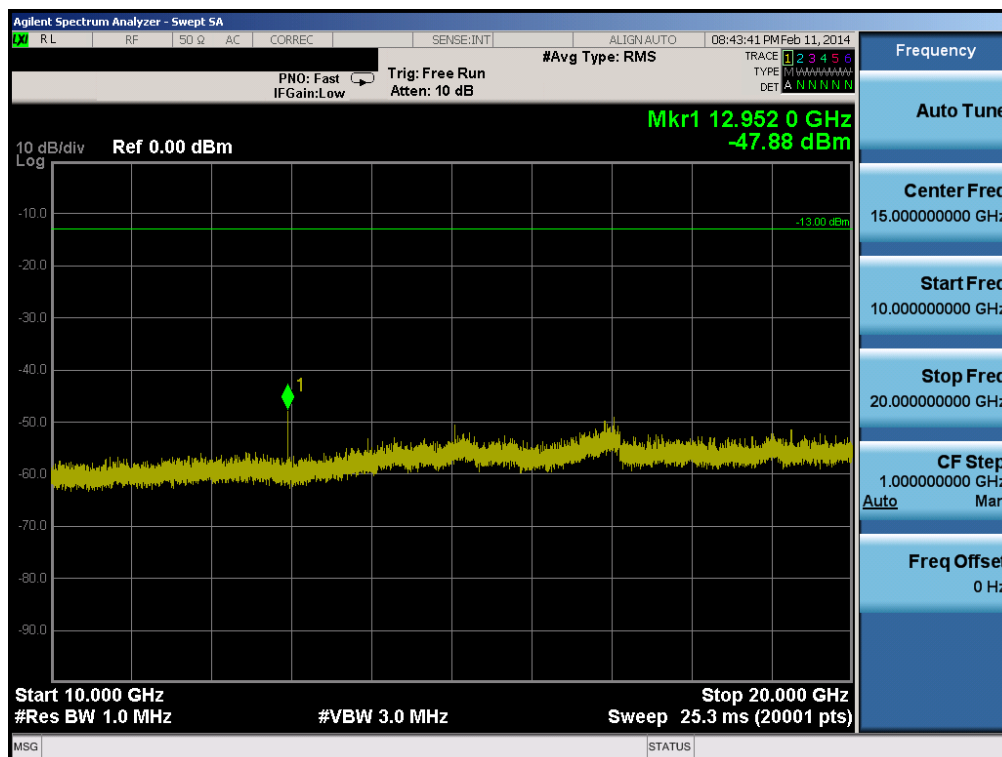
Plot 6-56. Conducted Spurious Plot (Band 2 – 5.0MHz QPSK – RB Size 1, RB Offset 0 – Low Channel)
