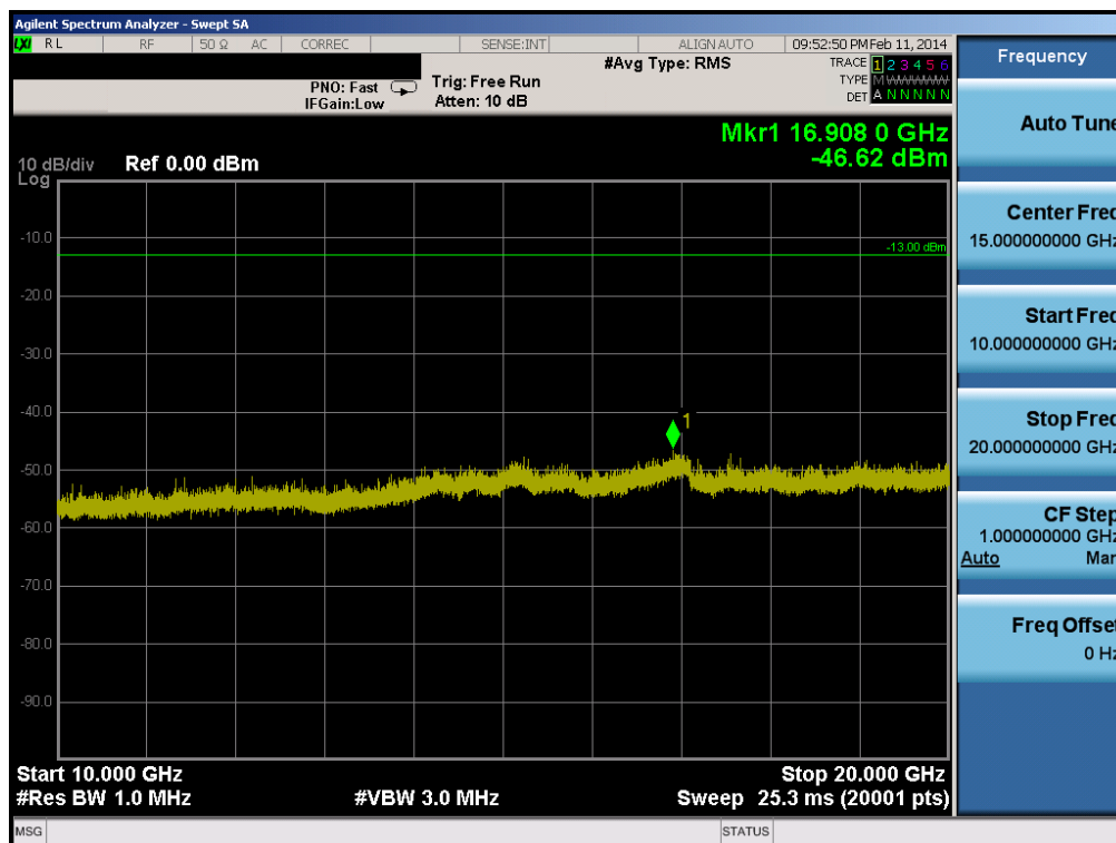
Plot 6-52. Conducted Spurious Plot (Band 4 – 5.0MHz QPSK – RB Size 1, RB Offset 0 – Mid Channel)
