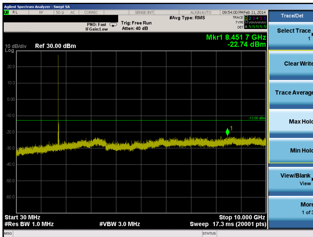
Plot 6-49. Conducted Spurious Plot (Band 4 – 5.0MHz QPSK – RB Size 1, RB Offset 0 – Low Channel)
