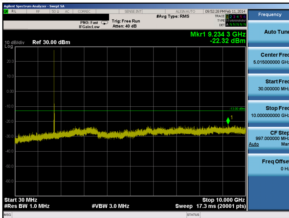
Plot 6-51. Conducted Spurious Plot (Band 4 – 5.0MHz QPSK – RB Size 1, RB Offset 0 – Mid Channel)
