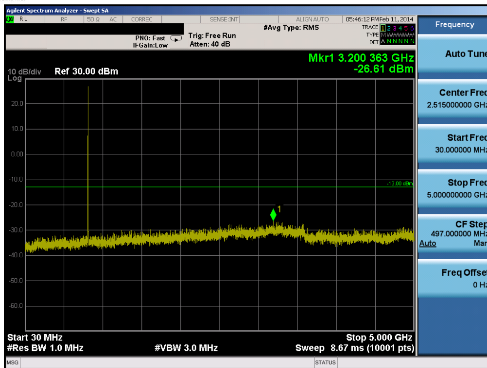
Plot 6-45. Conducted Spurious Plot (Band 5 – 3.0MHz QPSK – RB Size 1, RB Offset 0 – Mid Channel)
