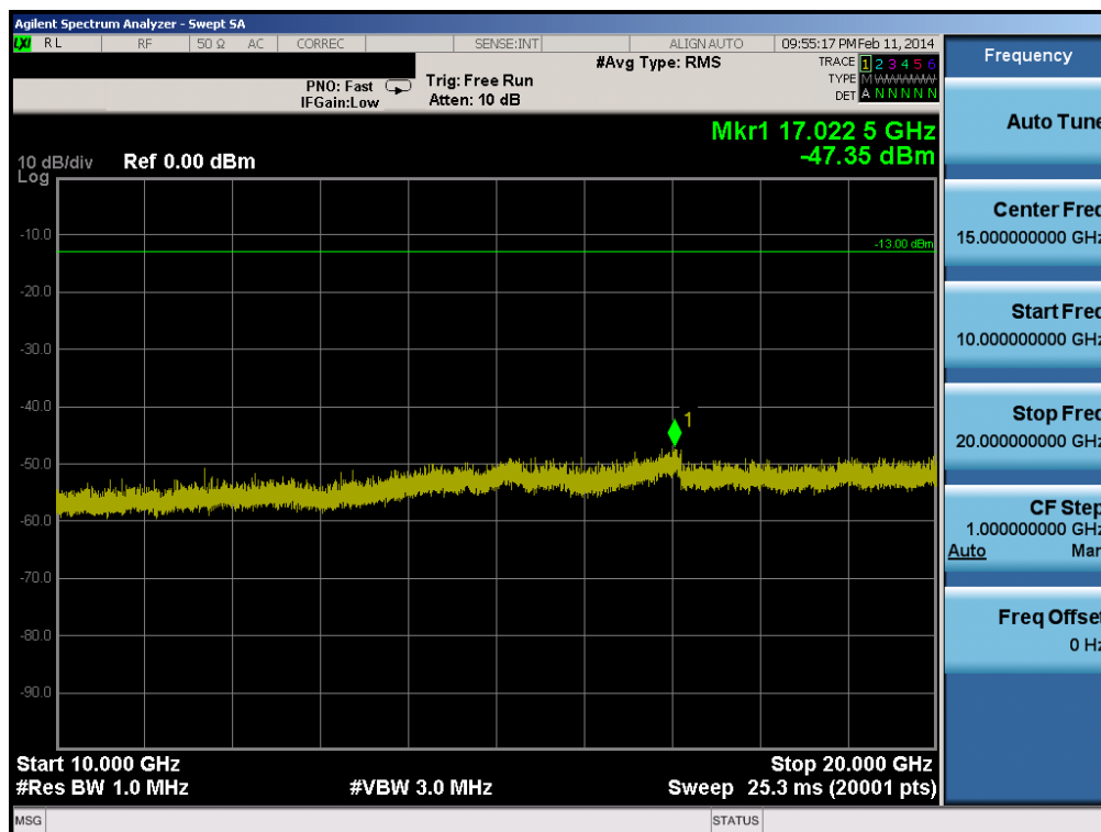
Plot 6-54. Conducted Spurious Plot (Band 4 – 5.0MHz QPSK – RB Size 1, RB Offset 0 – High Channel)
