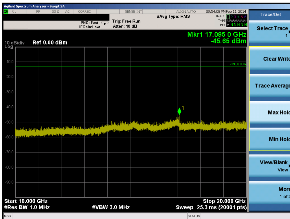
Plot 6-50. Conducted Spurious Plot (Band 4 – 5.0MHz QPSK – RB Size 1, RB Offset 0 – Low Channel)
