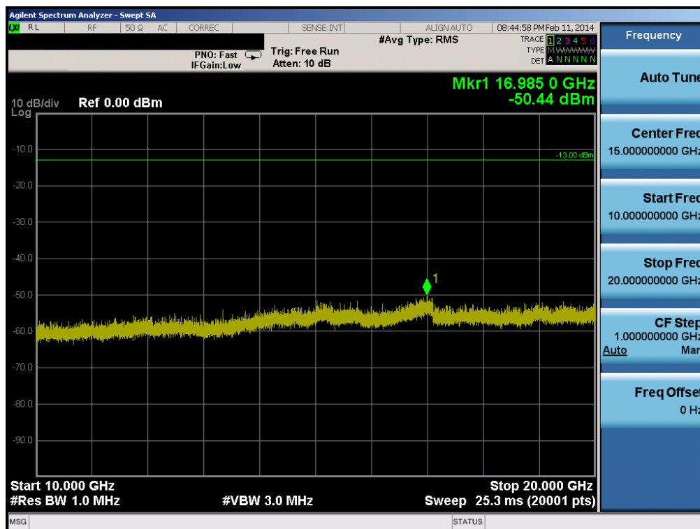
Plot 6-60. Conducted Spurious Plot (Band 2 – 5.0MHz QPSK – RB Size 1, RB Offset 0 – High Channel)
