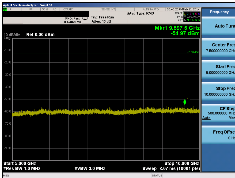
Plot 6-46. Conducted Spurious Plot (Band 5 – 3.0MHz QPSK – RB Size 1, RB Offset 0 – Mid Channel)
