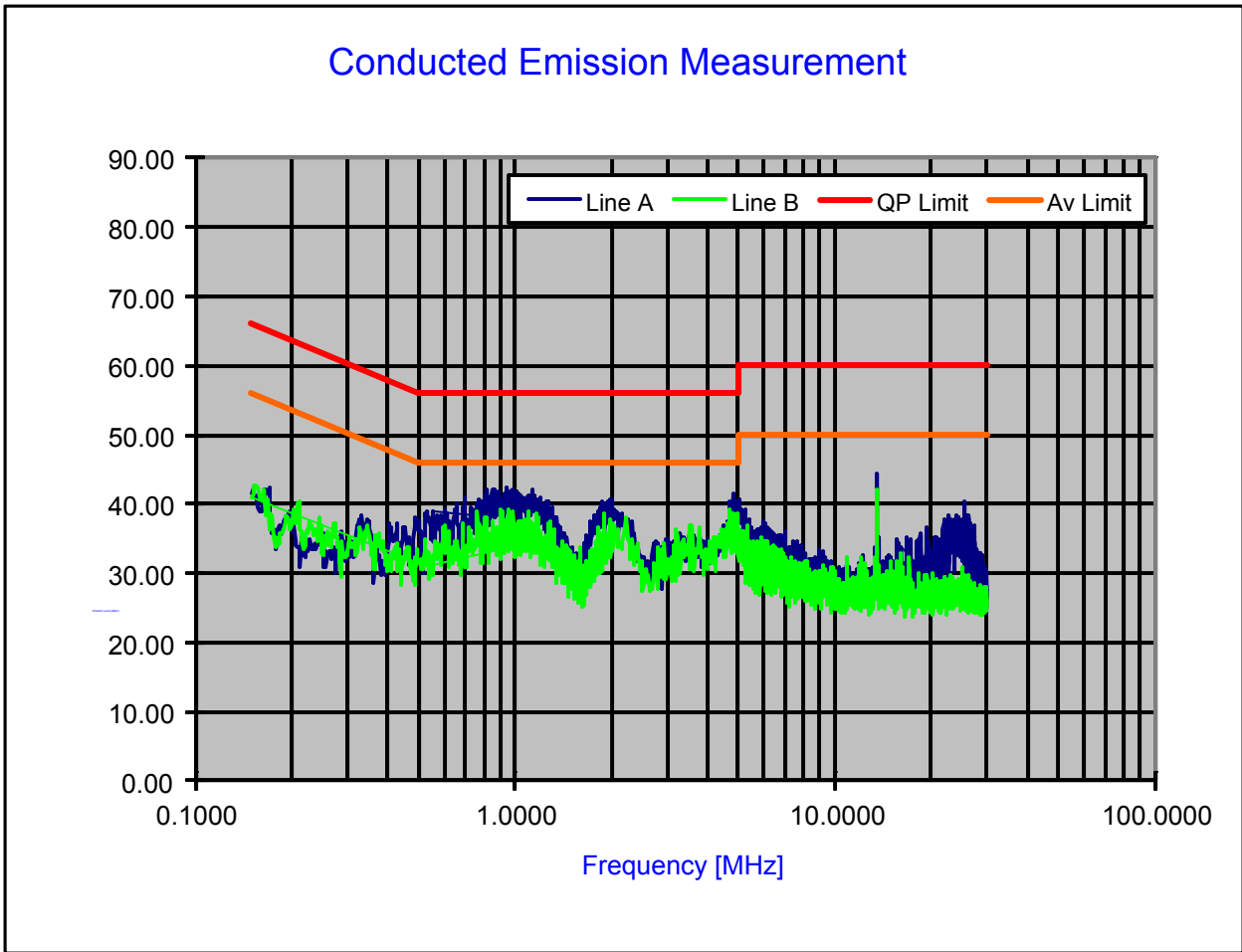
Plot 8-1. Line Conducted Plot with NFC
