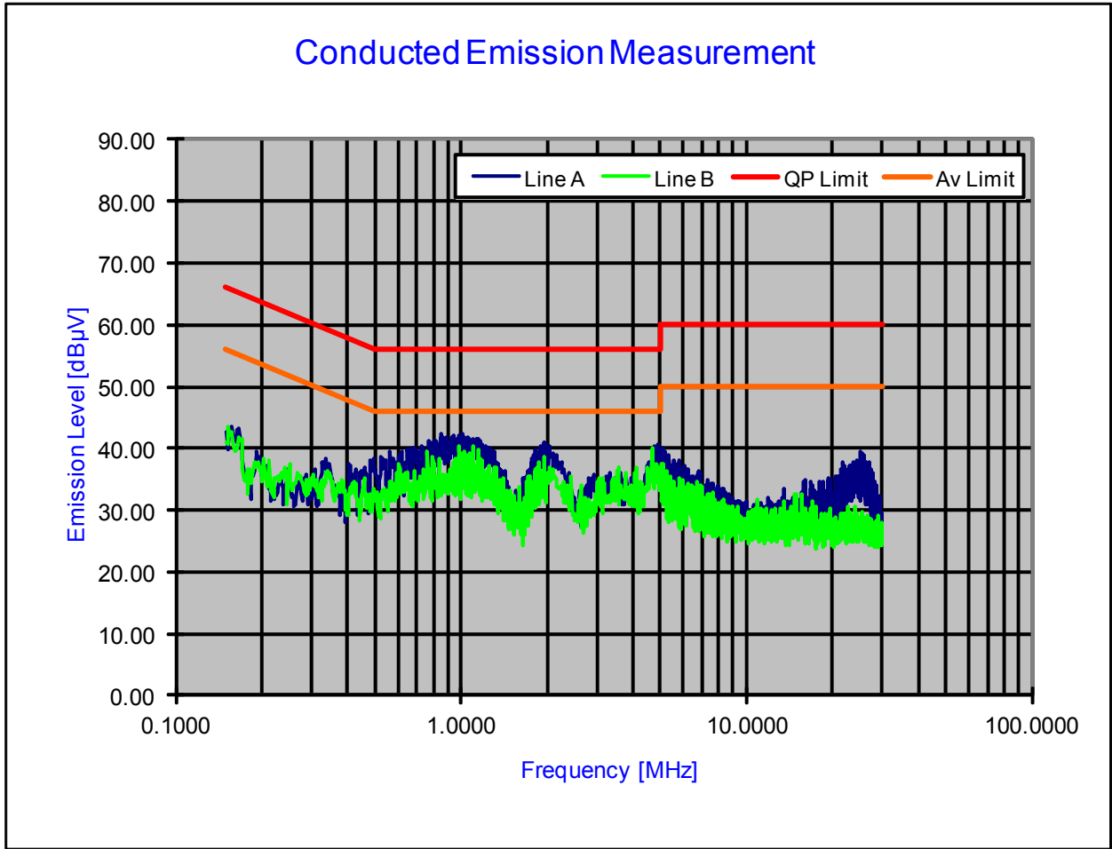
Plot 6-20. Line Conducted Plot with Bluetooth (LE)
