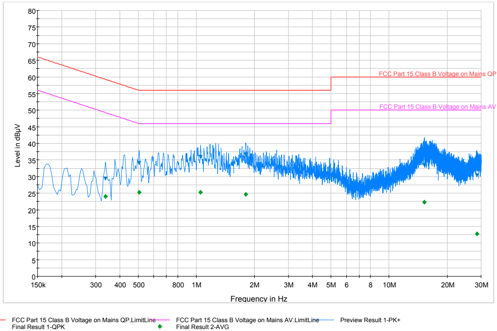
Plot 6-137. Line Conducted Plot with 802.11b (L1)
