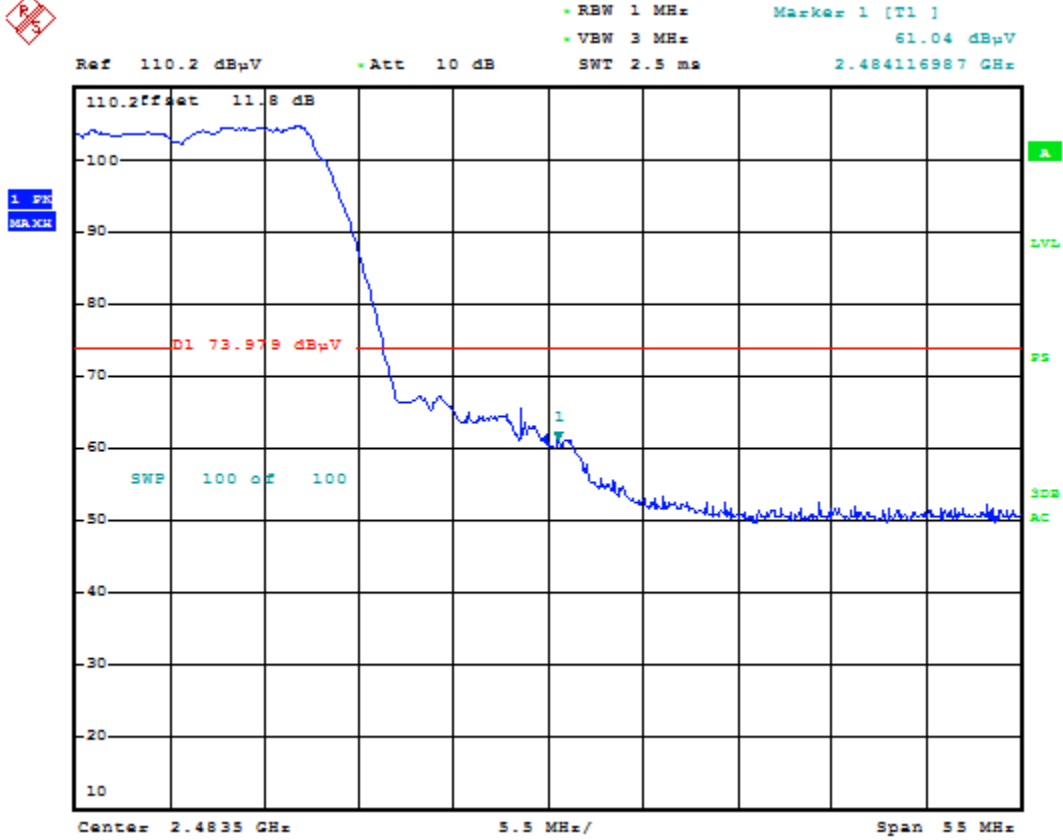
Plot 6-128. Radiated Restricted Upper Band Edge Measurement (Peak)
