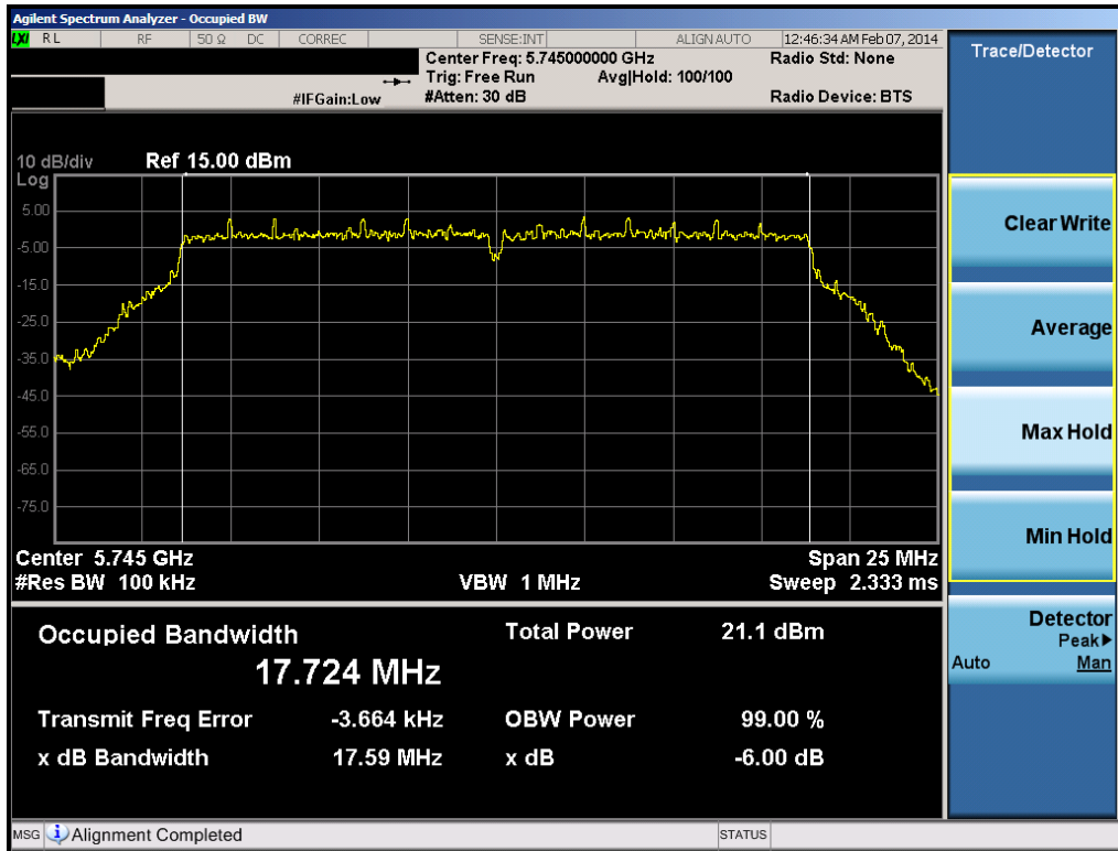
Plot 6-31. 6dB Bandwidth Plot (20MHz BW 802.11n (5.8GHz) – Ch. 149)
