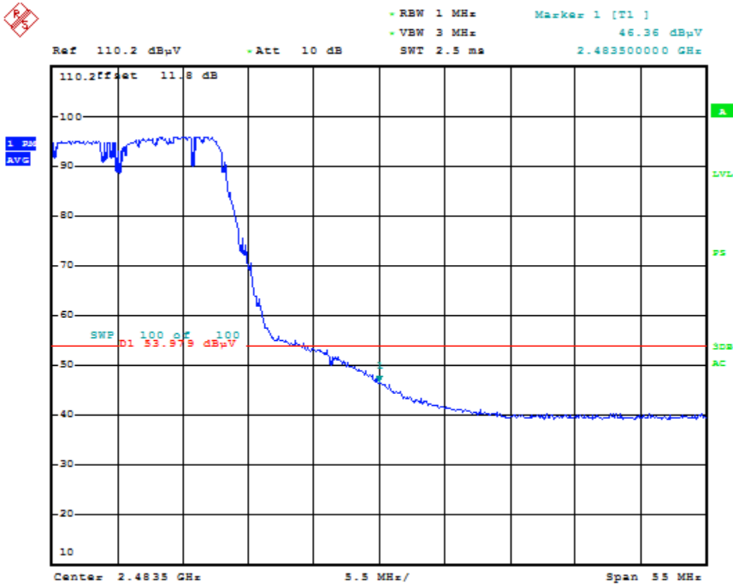
Plot 6-127. Radiated Restricted Upper Band Edge Measurement (Average)
