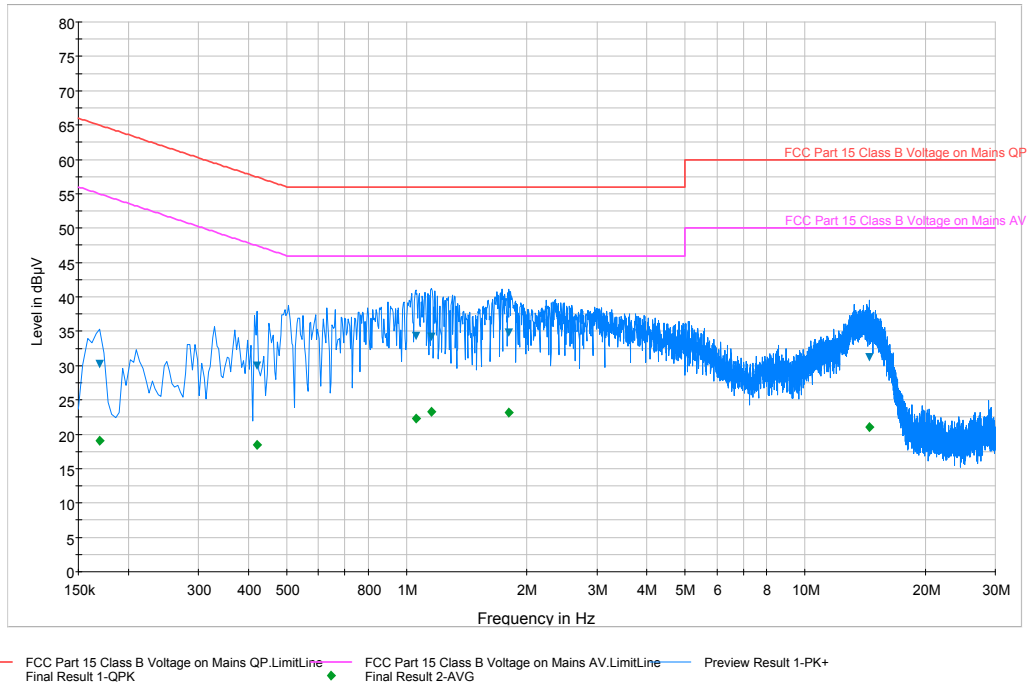
Plot 6-140. Line Conducted Plot with 802.11a (N)
