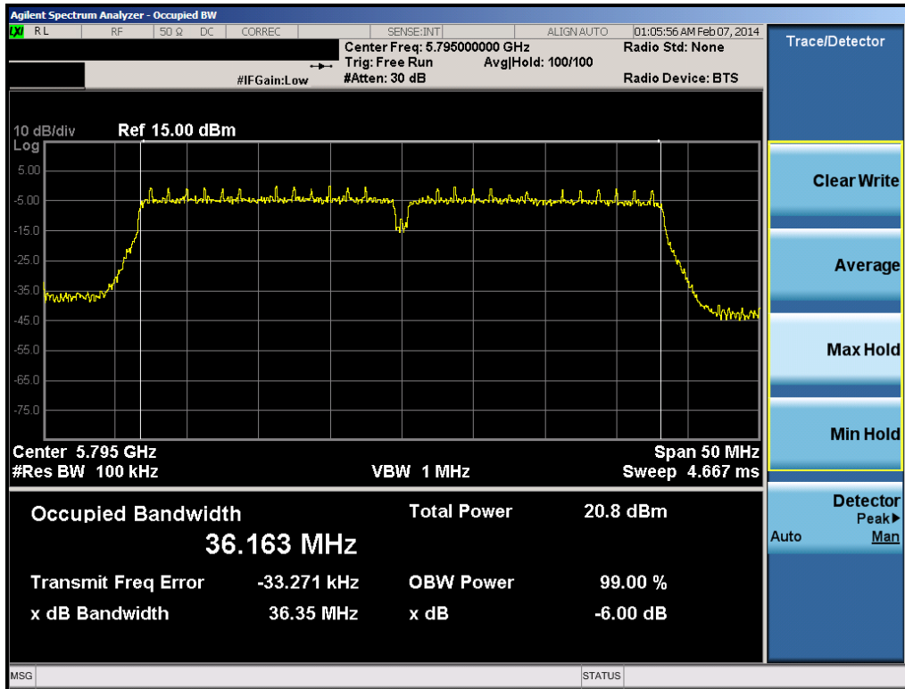
Plot 6-35. 6dB Bandwidth Plot (40MHz BW 802.11n (5.8GHz) – Ch. 159)
