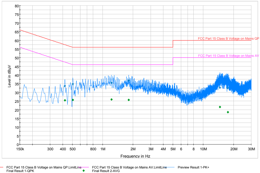
Plot 6-139. Line Conducted Plot with 802.11a (L1)
