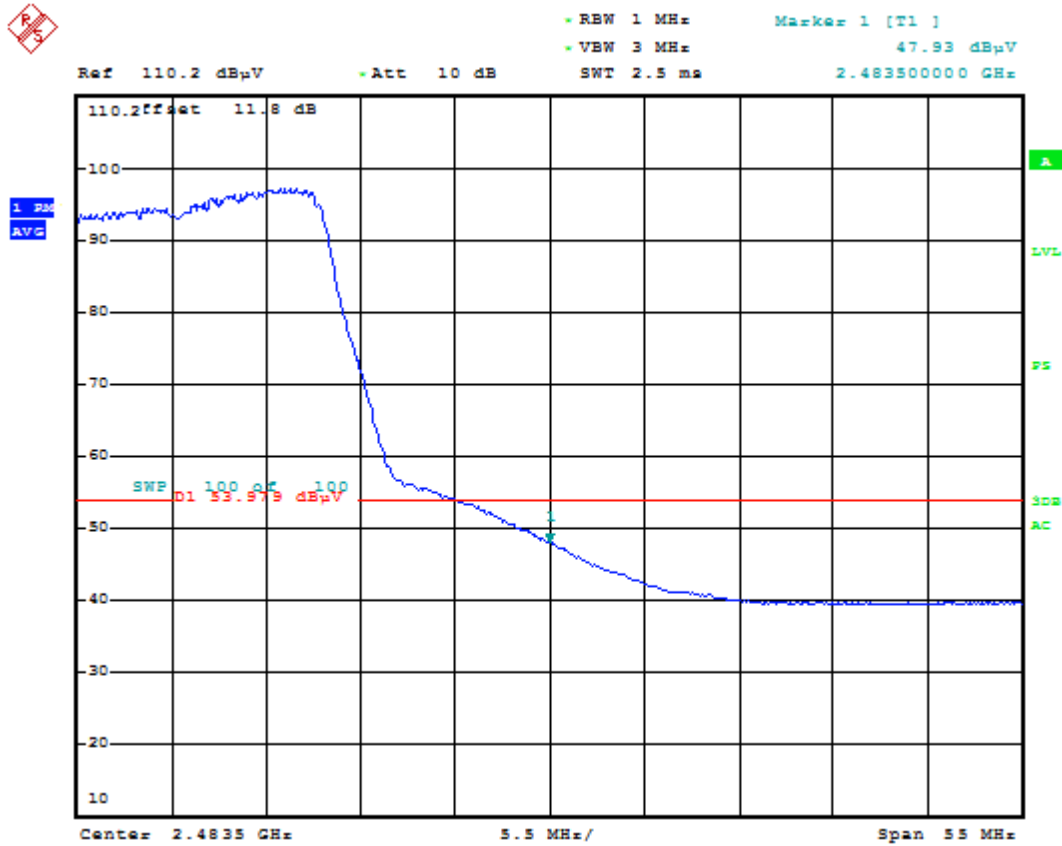
Plot 6-131. Radiated Restricted Upper Band Edge Measurement (Average)
