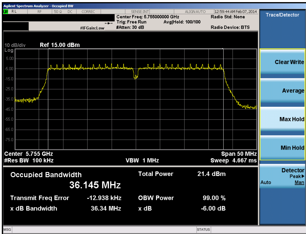
Plot 6-34. 6dB Bandwidth Plot (40MHz BW 802.11n (5.8GHz) – Ch. 151)
