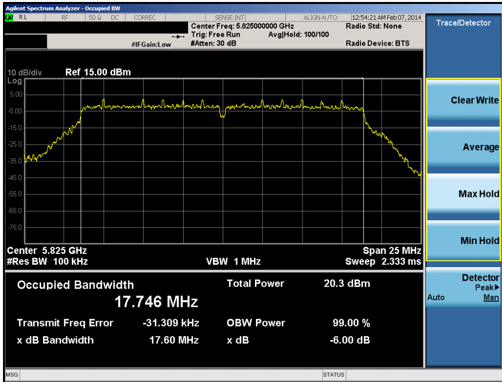
Plot 6-33. 6dB Bandwidth Plot (20MHz BW 802.11n (5.8GHz) – Ch. 165)
