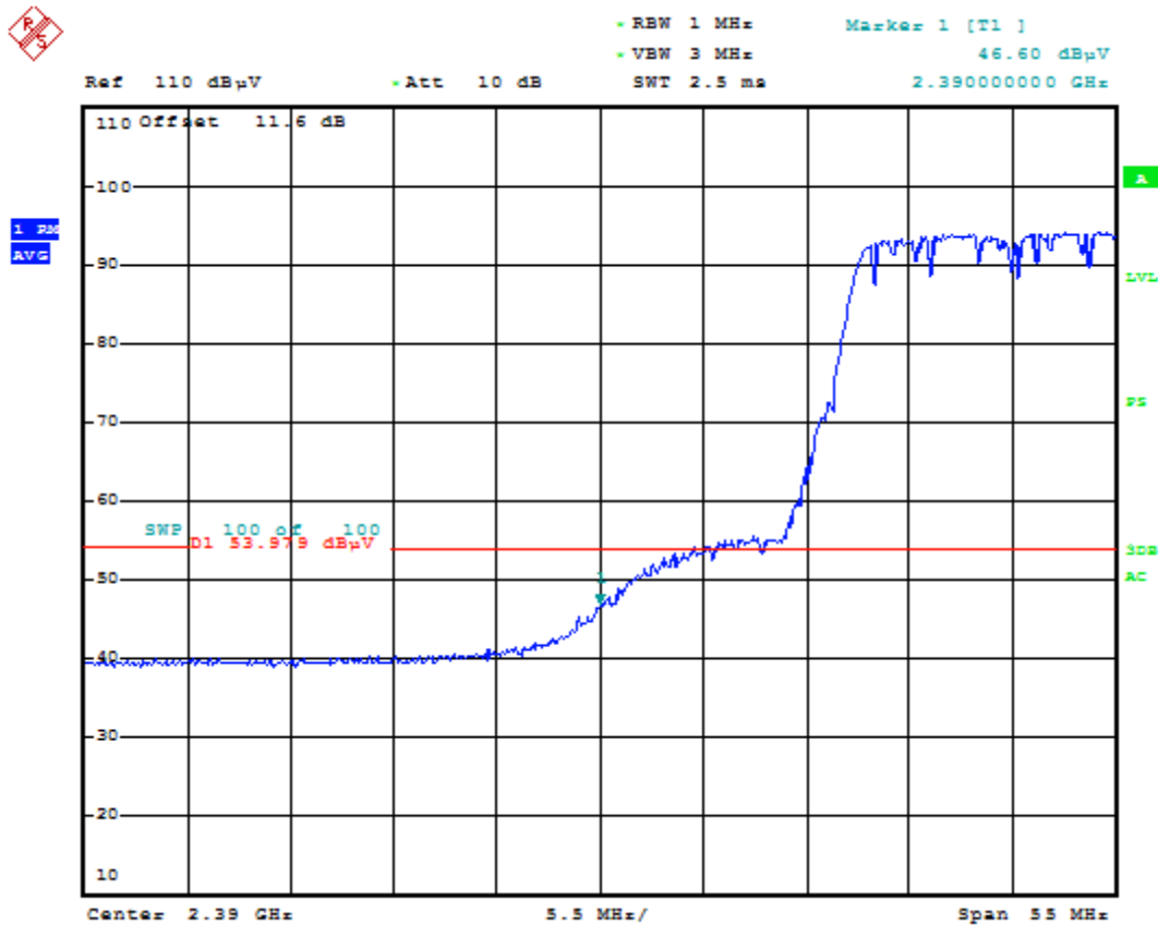
Plot 6-125. Radiated Restricted Lower Band Edge Measurement (Average)
