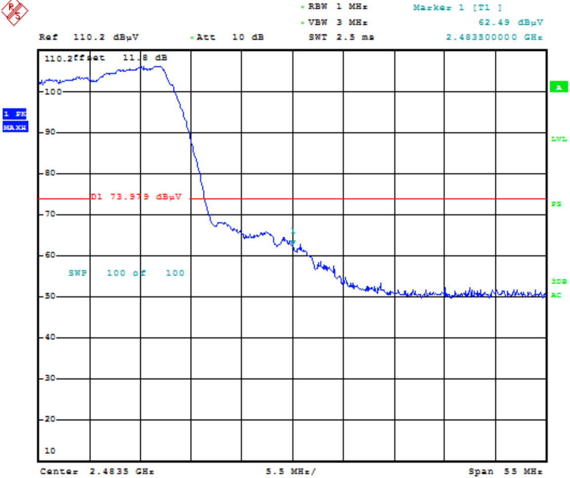
Plot 6-132. Radiated Restricted Upper Band Edge Measurement (Peak)
