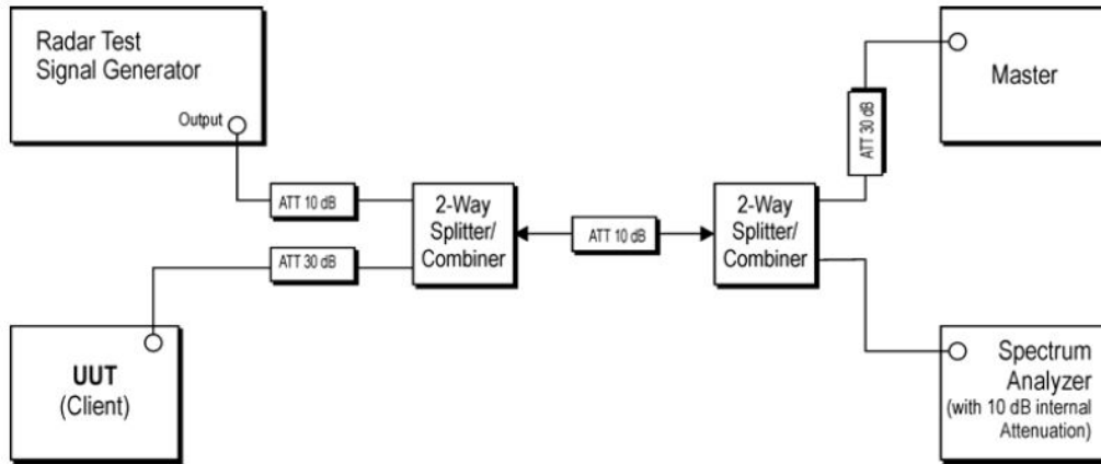
Figure 3-1. Conducted Test Setup for DFS
