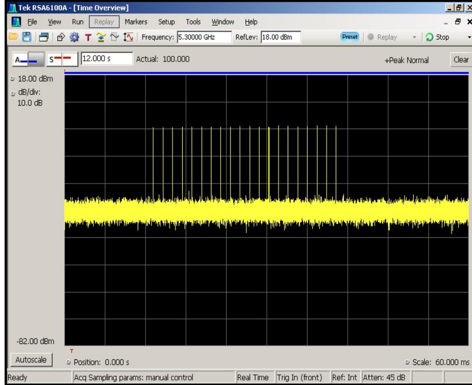
Figure 5-1. Type 1 Radar Pulse
