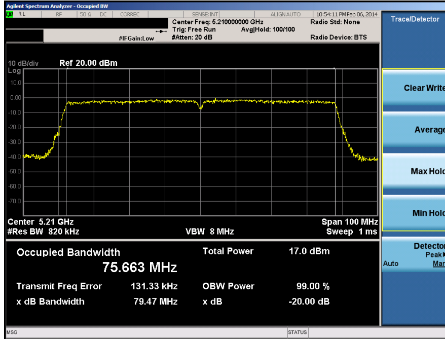
Plot 6-31. 20dB Bandwidth Plot (80MHz BW 802.11ac (UNII Band 1) – Ch. 42)
