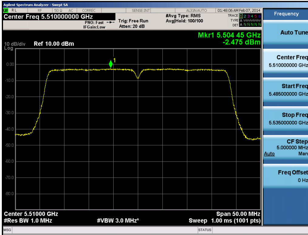
Plot 6-122. Peak Power Spectral Density Plot (40MHz BW 802.11n (UNII Band 2C) – Ch. 102)
