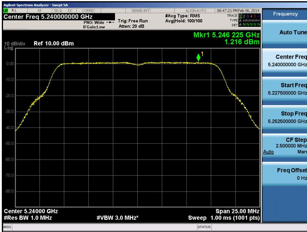
Plot 6-72. Peak Power Spectral Density Plot (802.11a (UNII Band 1) – Ch. 48)
