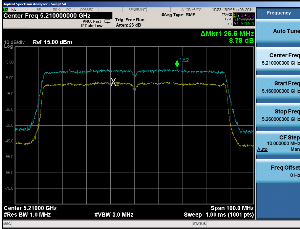
Plot 6-129. Peak Excursion Ratio Plot (80MHz BW 802.11ac)
