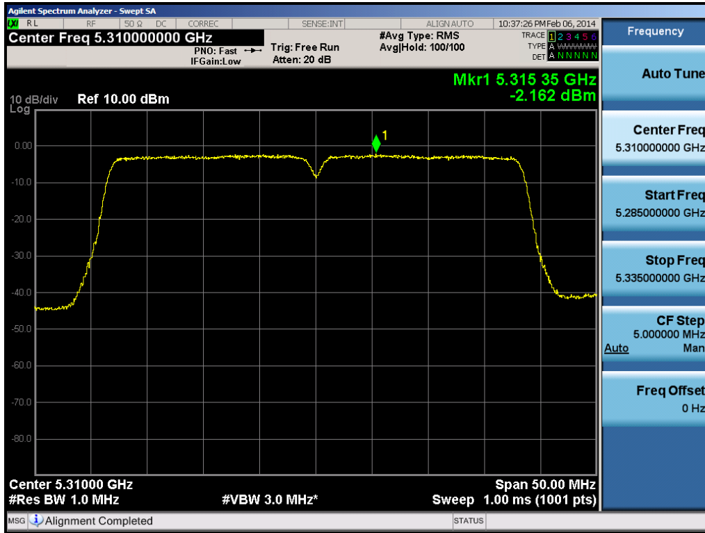
Plot 6-86. Peak Power Spectral Density Plot (40MHz BW 802.11n (UNII Band 2A) – Ch. 62)
