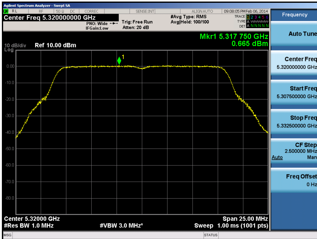
Plot 6-81. Peak Power Spectral Density Plot (802.11a (UNII Band 2A) – Ch. 64)
