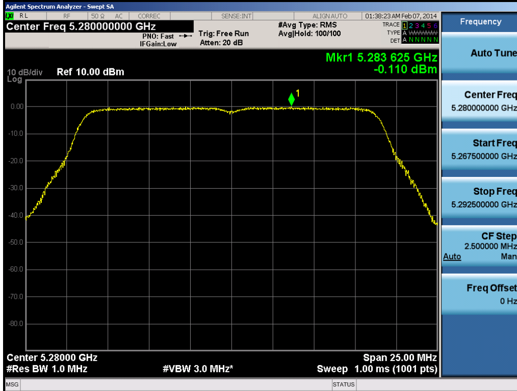
Plot 6-111. Peak Power Spectral Density Plot (20MHz BW 802.11n (UNII Band 2A) – Ch. 56)
