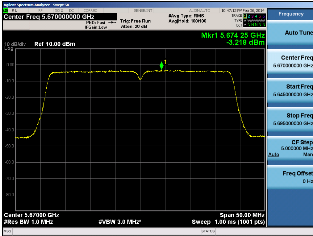
Plot 6-96. Peak Power Spectral Density Plot (40MHz BW 802.11n (UNII Band 2C) – Ch. 134)
