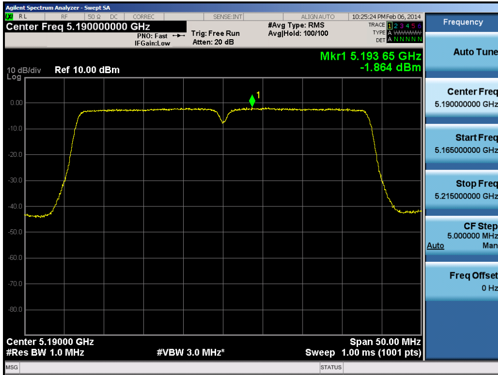
Plot 6-76. Peak Power Spectral Density Plot (40MHz BW 802.11n (UNII Band 1) – Ch. 38)
