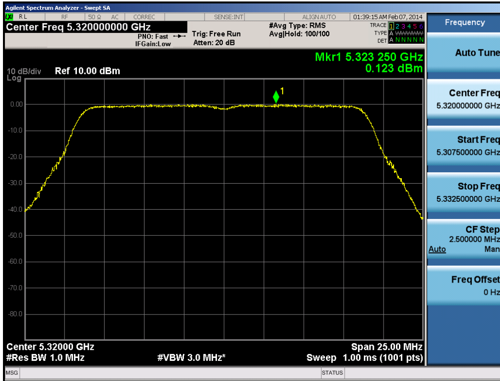
Plot 6-112. Peak Power Spectral Density Plot (20MHz BW 802.11n (UNII Band 2A) – Ch. 64)
