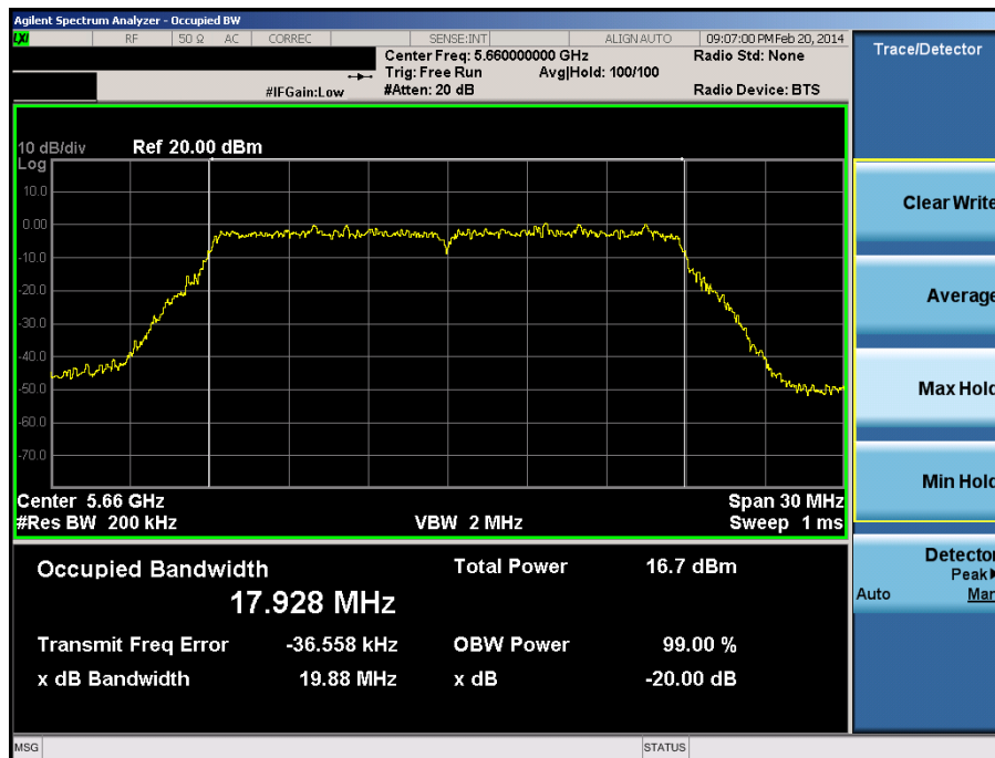
Plot 6-68. 20dB Bandwidth Plot (20MHz BW 802.11n (UNII Band 2C) – Ch. 132)
