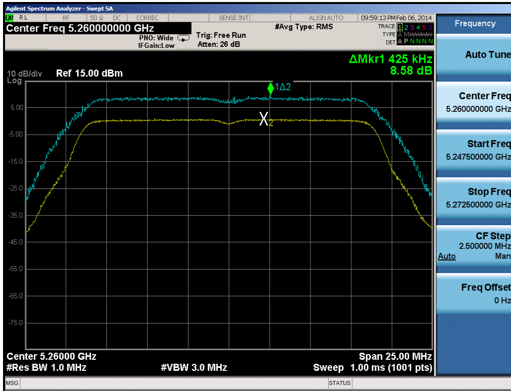
Plot 6-127. Peak Excursion Ratio Plot (20MHz BW 802.11n)
