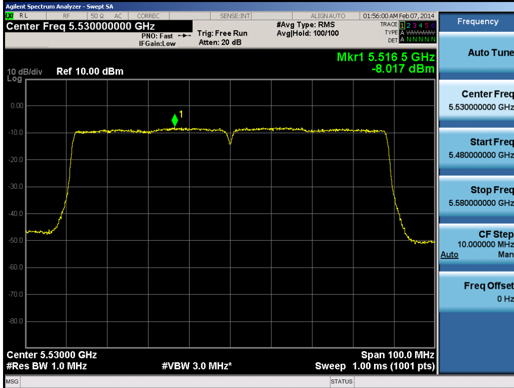
Plot 6-125. Peak Power Spectral Density Plot (80MHz BW 802.11ac (UNII Band 2C) – Ch. 106)
