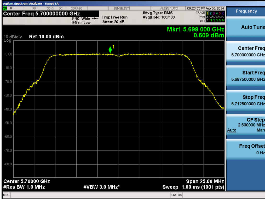
Plot 6-90. Peak Power Spectral Density Plot (802.11a (UNII Band 2C) – Ch. 140)
