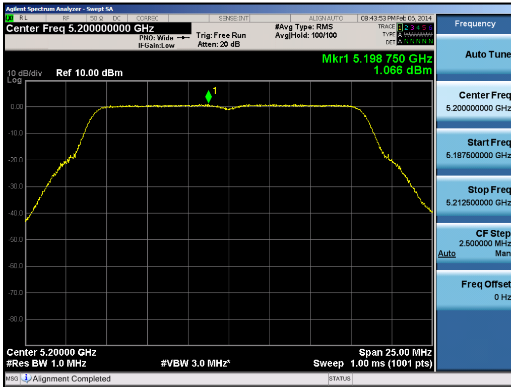
Plot 6-71. Peak Power Spectral Density Plot (802.11a (UNII Band 1) – Ch. 40)
