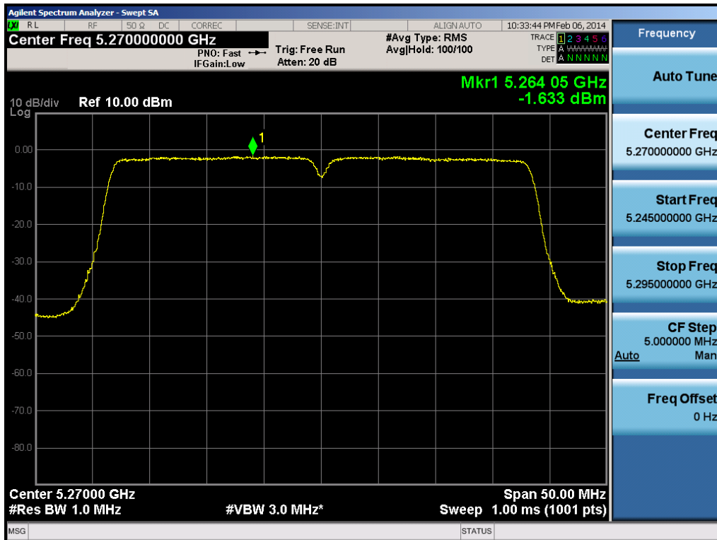
Plot 6-85. Peak Power Spectral Density Plot (40MHz BW 802.11n (UNII Band 2A) – Ch. 54)
