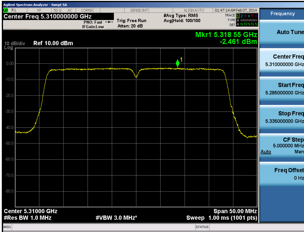
Plot 6-114. Peak Power Spectral Density Plot (40MHz BW 802.11n (UNII Band 2A) – Ch. 62)
