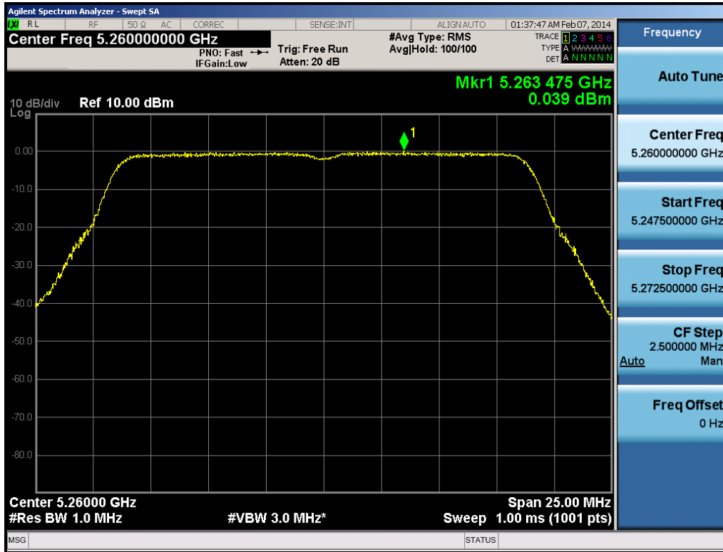
Plot 6-110. Peak Power Spectral Density Plot (20MHz BW 802.11n (UNII Band 2A) – Ch. 52)
