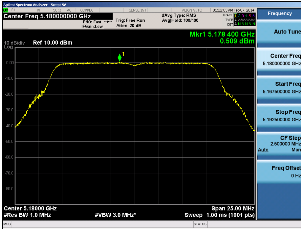
Plot 6-98. Peak Power Spectral Density Plot (802.11a (UNII Band 1) – Ch. 36)
