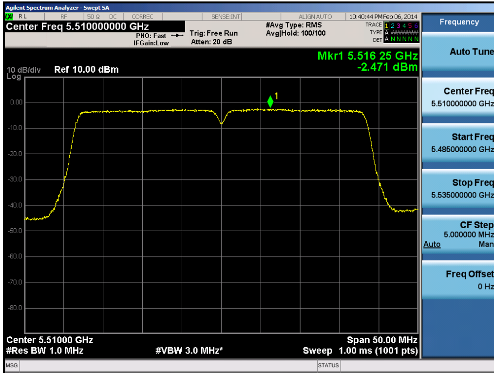
Plot 6-94. Peak Power Spectral Density Plot (40MHz BW 802.11n (UNII Band 2C) – Ch. 102)
