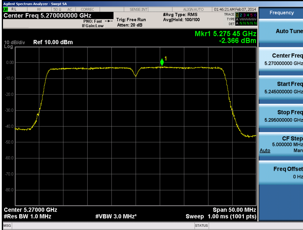
Plot 6-113. Peak Power Spectral Density Plot (40MHz BW 802.11n (UNII Band 2A) – Ch. 54)
