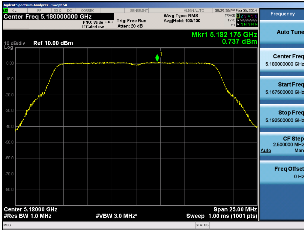
Plot 6-70. Peak Power Spectral Density Plot (802.11a (UNII Band 1) – Ch. 36)
