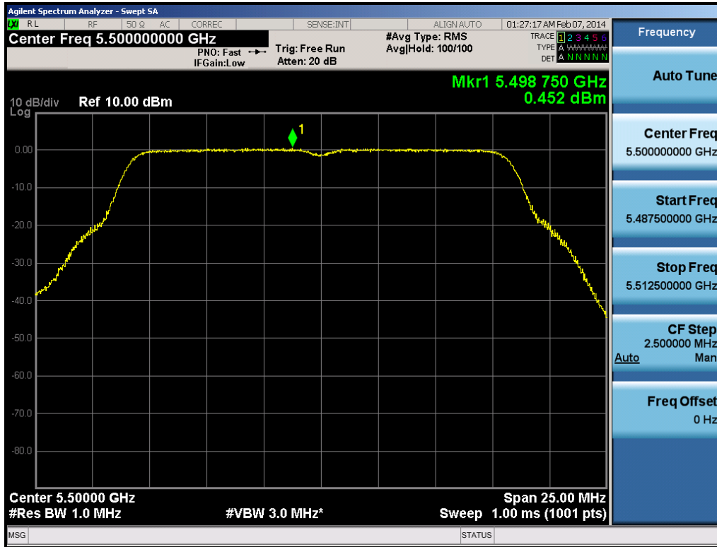
Plot 6-116. Peak Power Spectral Density Plot (802.11a (UNII Band 2C) – Ch. 100)
