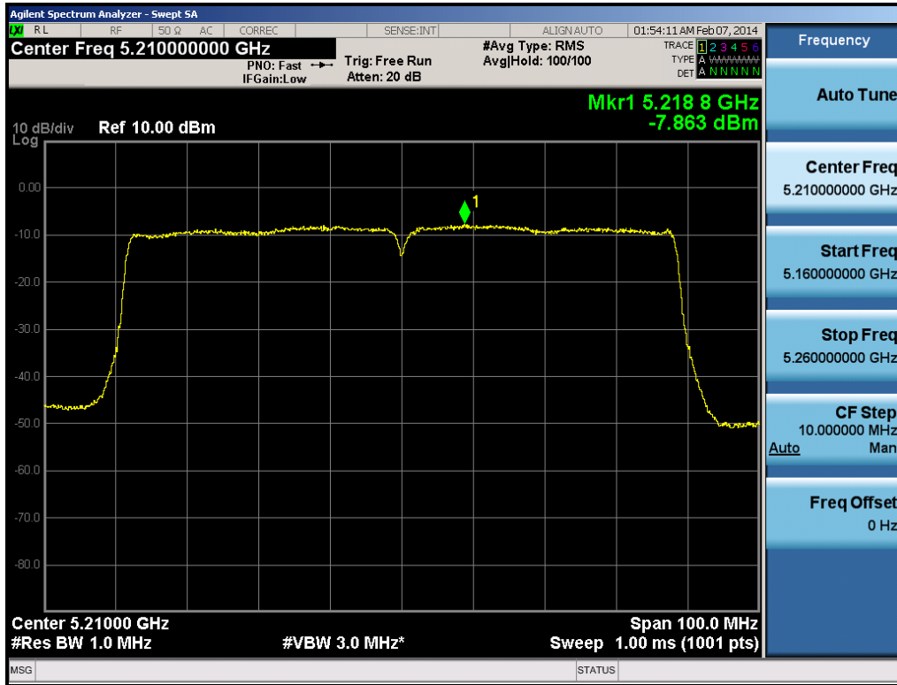
Plot 6-106. Peak Power Spectral Density Plot (80MHz BW 802.11ac (UNII Band 1) – Ch. 42)
