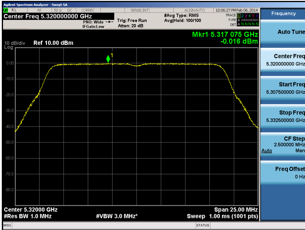
Plot 6-84. Peak Power Spectral Density Plot (20MHz BW 802.11n (UNII Band 2A) – Ch. 64)
