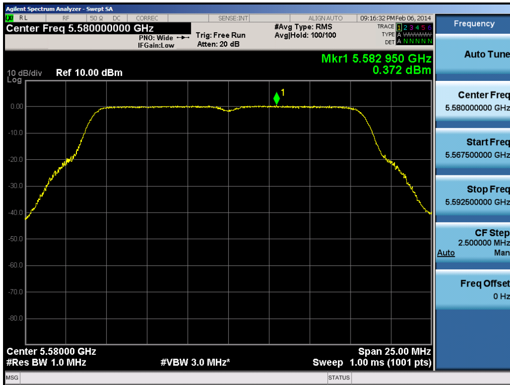
Plot 6-89. Peak Power Spectral Density Plot (802.11a (UNII Band 2C) – Ch. 116)
