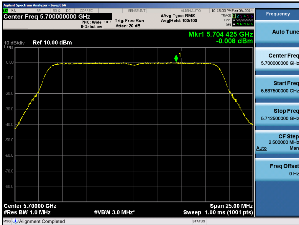
Plot 6-93. Peak Power Spectral Density Plot (20MHz BW 802.11n (UNII Band 2C) – Ch. 140)
