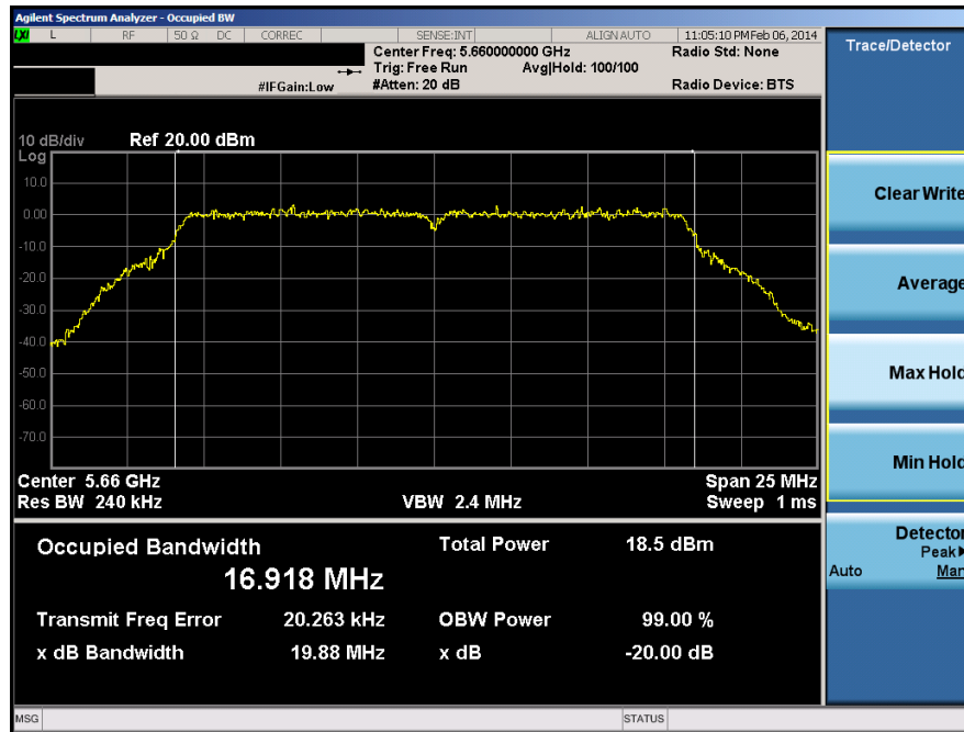
Plot 6-32. 20dB Bandwidth Plot (20MHz BW 802.11a (UNII Band 2C) – Ch. 132)
