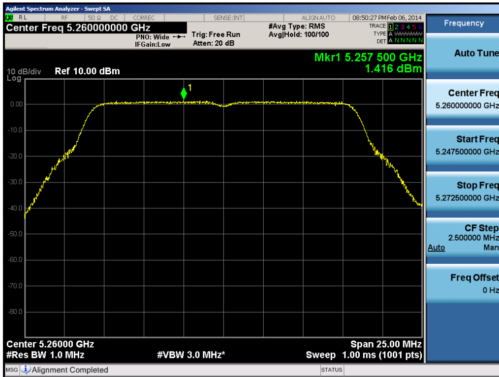
Plot 6-79. Peak Power Spectral Density Plot (802.11a (UNII Band 2A) – Ch. 52)
