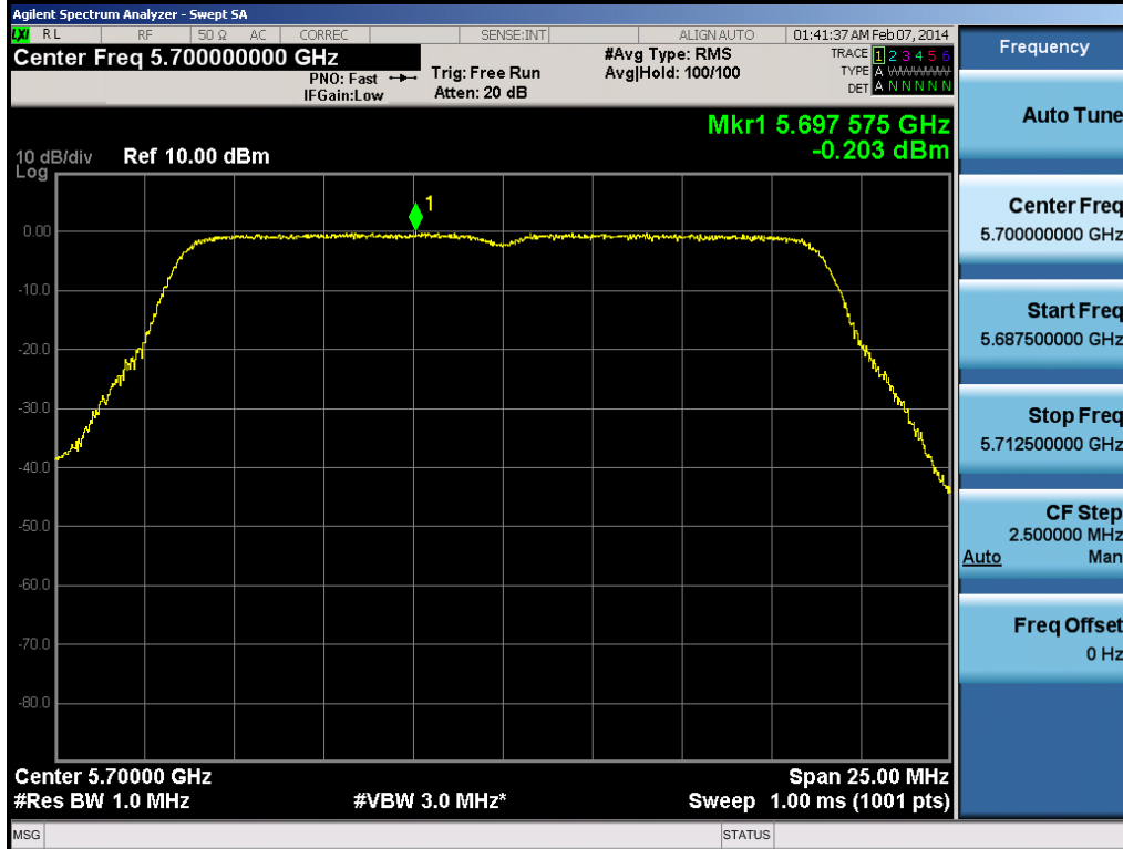
Plot 6-121. Peak Power Spectral Density Plot (20MHz BW 802.11n (UNII Band 2C) – Ch. 140)
