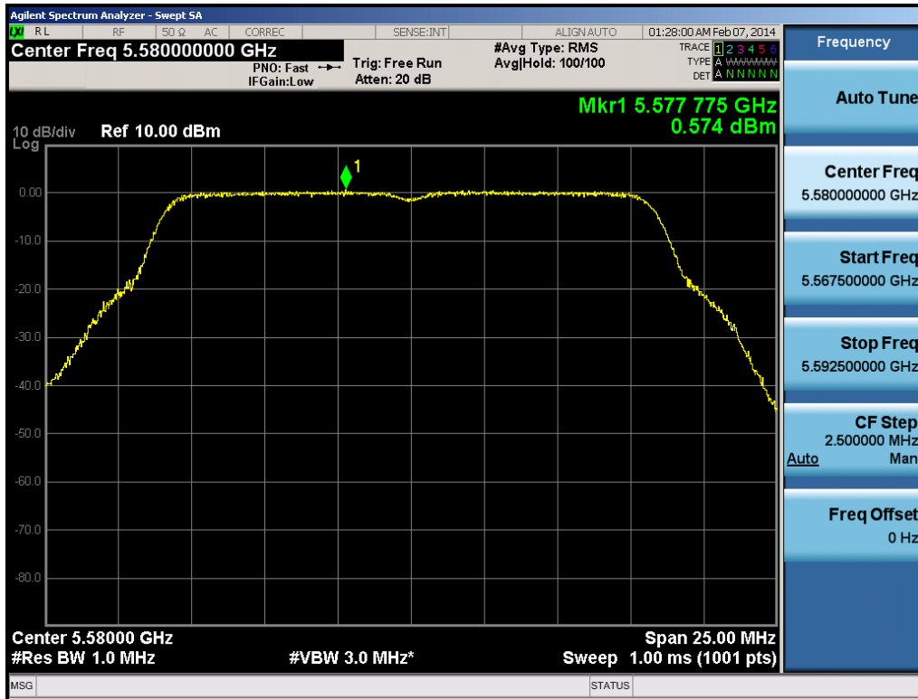
Plot 6-117. Peak Power Spectral Density Plot (802.11a (UNII Band 2C) – Ch. 116)
