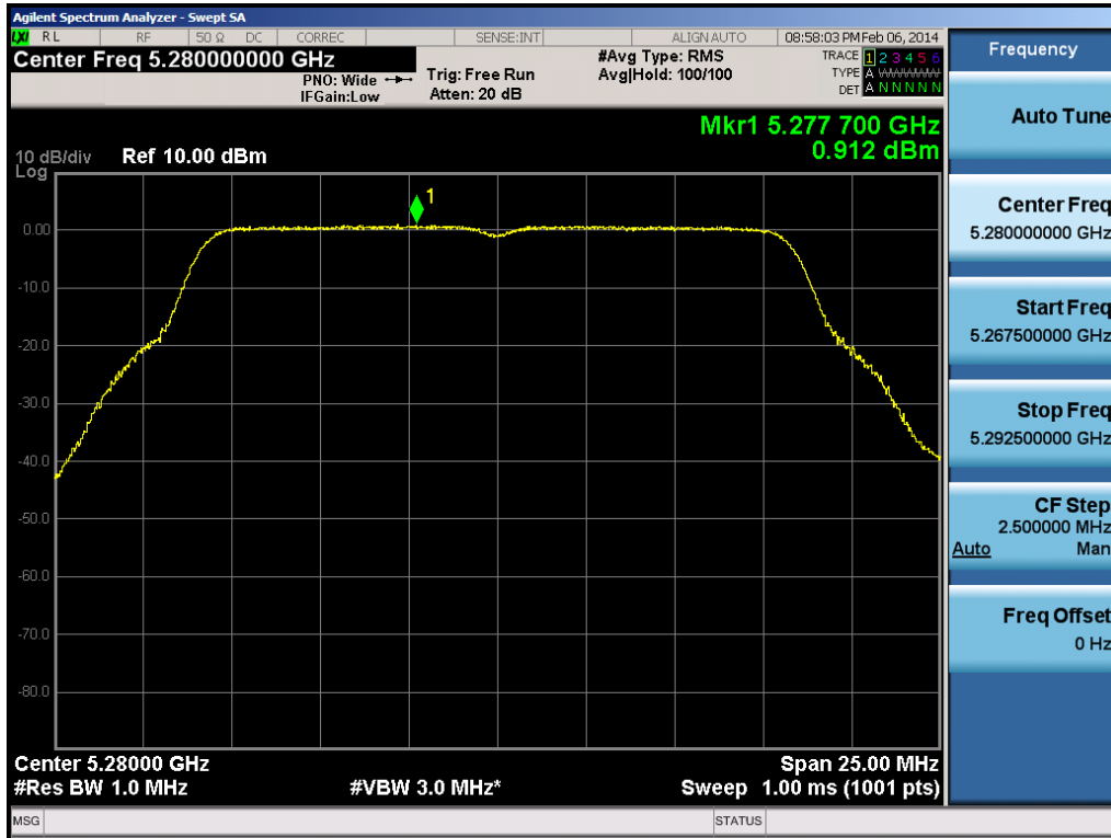
Plot 6-80. Peak Power Spectral Density Plot (802.11a (UNII Band 2A) – Ch. 56)
