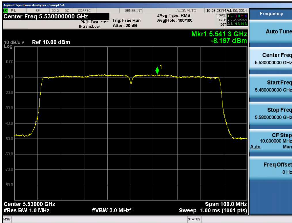
Plot 6-97. Peak Power Spectral Density Plot (80MHz BW 802.11ac (UNII Band 2C) – Ch. 106)
