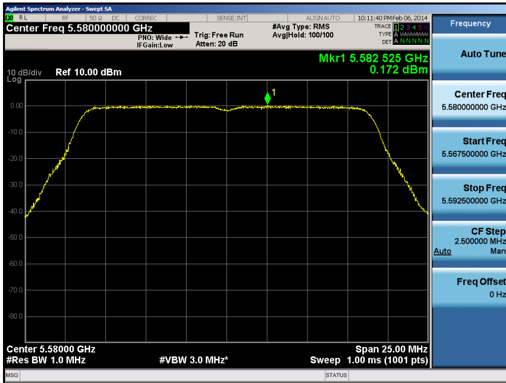
Plot 6-92. Peak Power Spectral Density Plot (20MHz BW 802.11n (UNII Band 2C) – Ch. 116)
