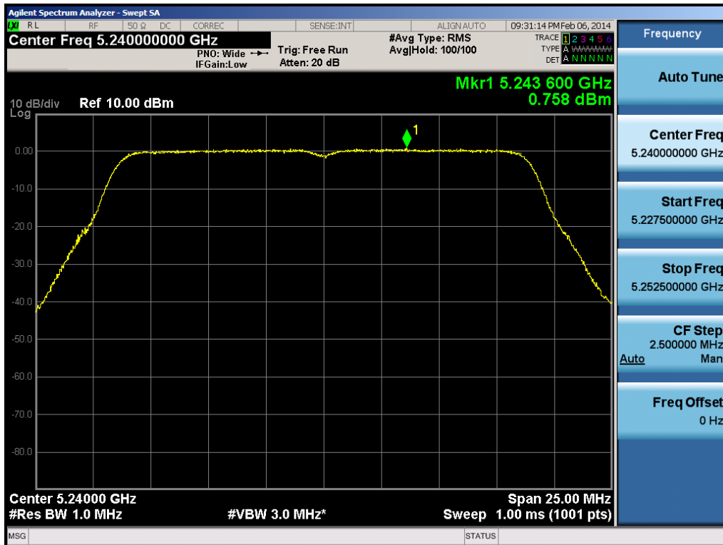
Plot 6-75. Peak Power Spectral Density Plot (20MHz BW 802.11n (UNII Band 1) – Ch. 48)
