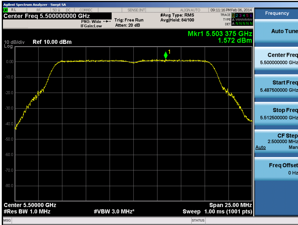
Plot 6-88. Peak Power Spectral Density Plot (802.11a (UNII Band 2C) – Ch. 100)
