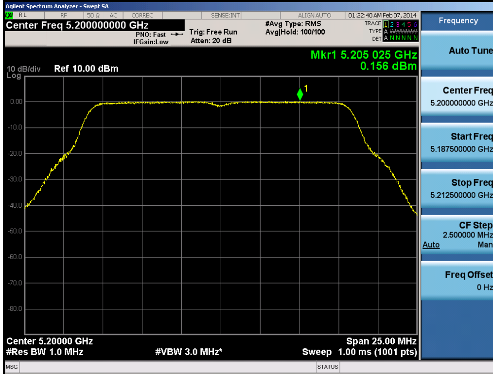
Plot 6-99. Peak Power Spectral Density Plot (802.11a (UNII Band 1) – Ch. 40)
