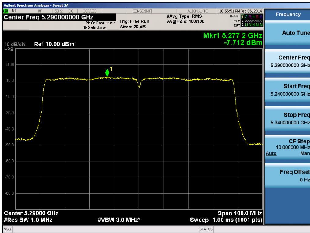
Plot 6-87. Peak Power Spectral Density Plot (80MHz BW 802.11ac (UNII Band 2A) – Ch. 58)
