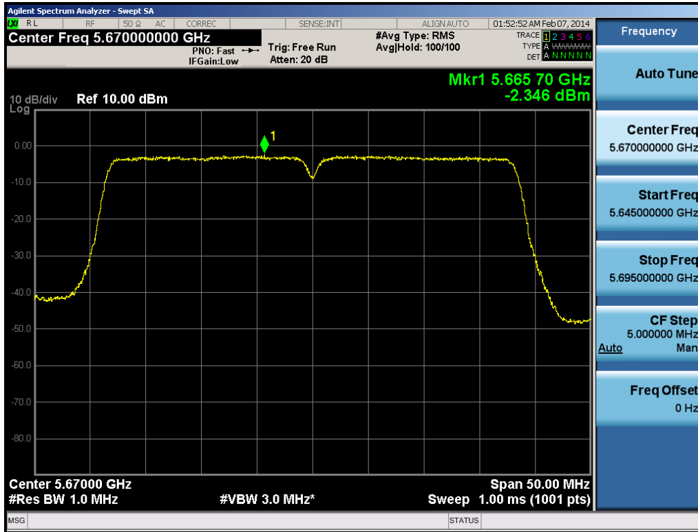
Plot 6-124. Peak Power Spectral Density Plot (40MHz BW 802.11n (UNII Band 2C) – Ch. 134)
