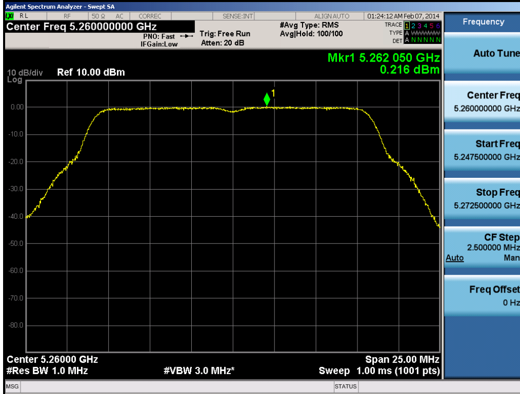
Plot 6-107. Peak Power Spectral Density Plot (802.11a (UNII Band 2A) – Ch. 52)
