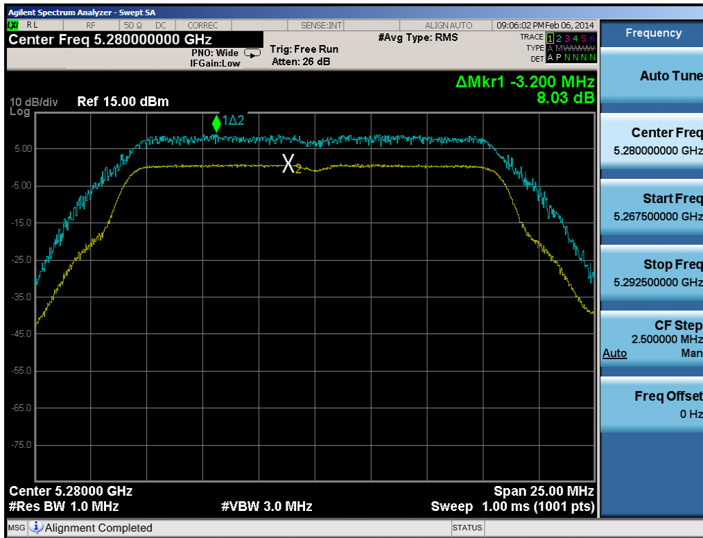
Plot 6-126. Peak Excursion Ratio Plot (802.11a)
