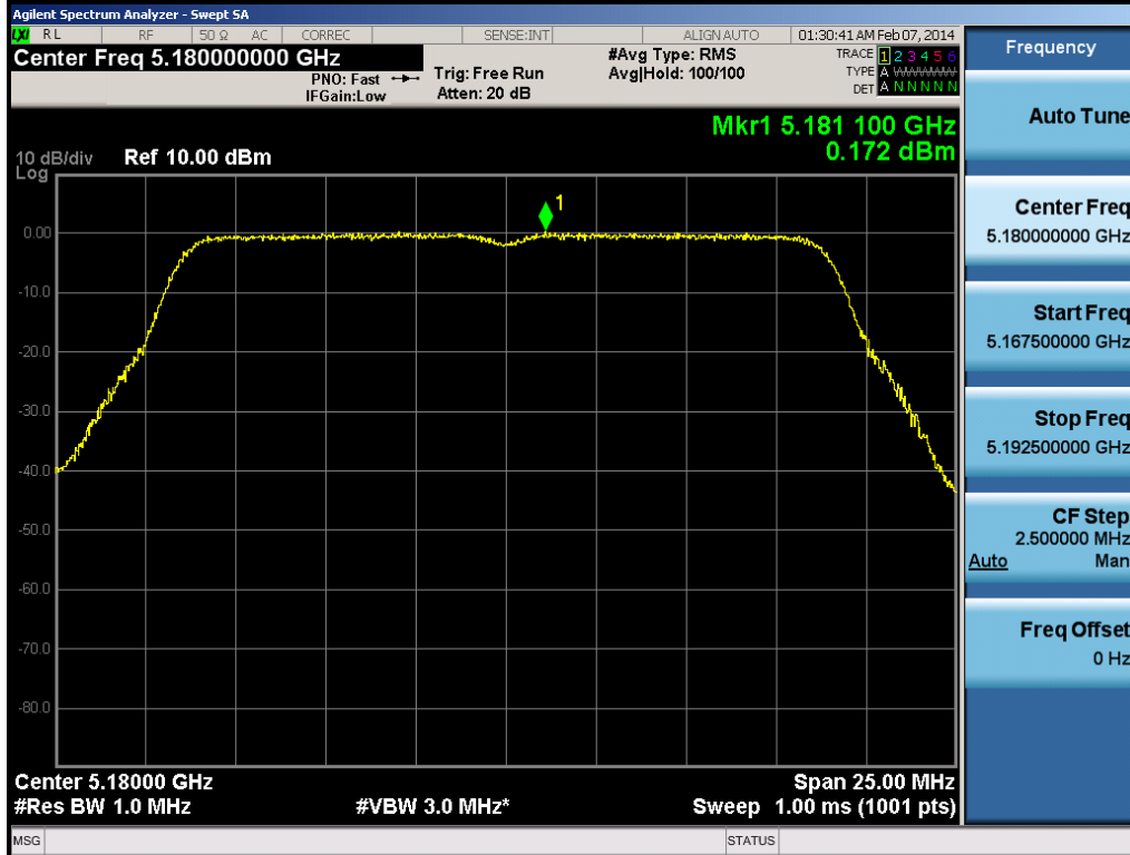
Plot 6-101. Peak Power Spectral Density Plot (20MHz BW 802.11n (UNII Band 1) – Ch. 36)
