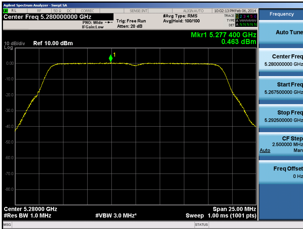
Plot 6-83. Peak Power Spectral Density Plot (20MHz BW 802.11n (UNII Band 2A) – Ch. 56)
