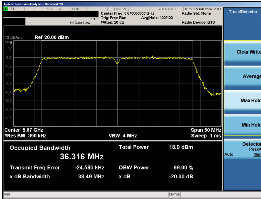
Plot 6-69. 20dB Bandwidth Plot (40MHz BW 802.11n (UNII Band 2C) – Ch. 134)
