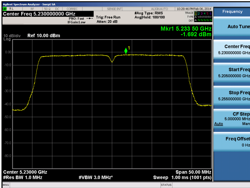
Plot 6-77. Peak Power Spectral Density Plot (40MHz BW 802.11n (UNII Band 1) – Ch. 46)
