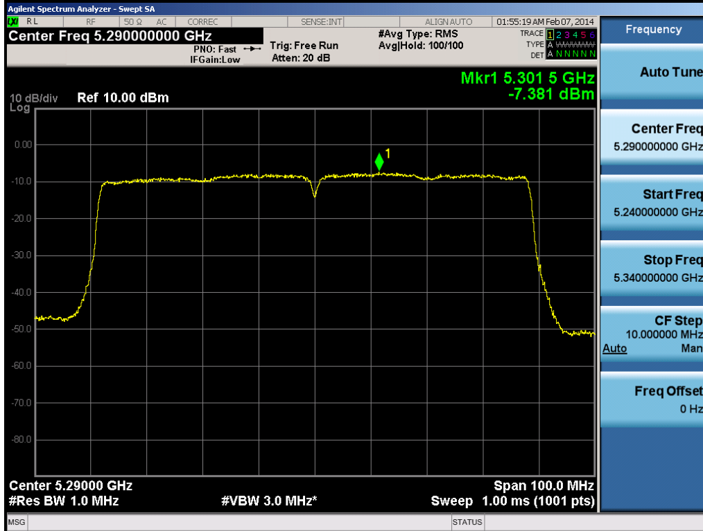
Plot 6-115. Peak Power Spectral Density Plot (80MHz BW 802.11ac (UNII Band 2A) – Ch. 58)
