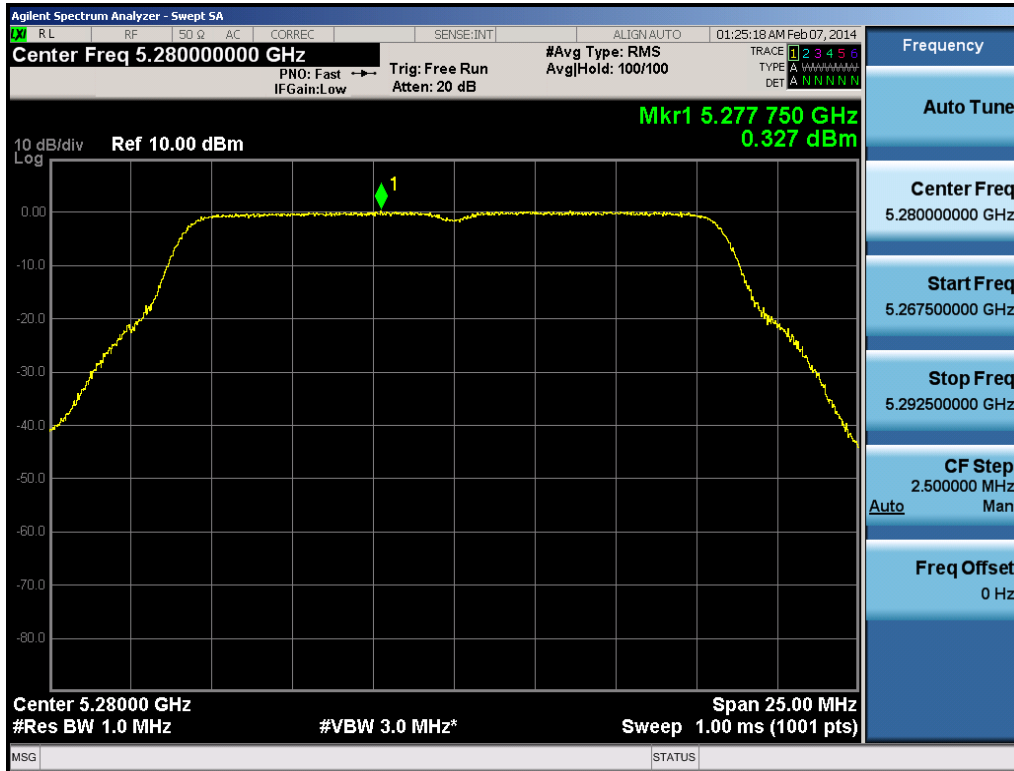
Plot 6-108. Peak Power Spectral Density Plot (802.11a (UNII Band 2A) – Ch. 56)
