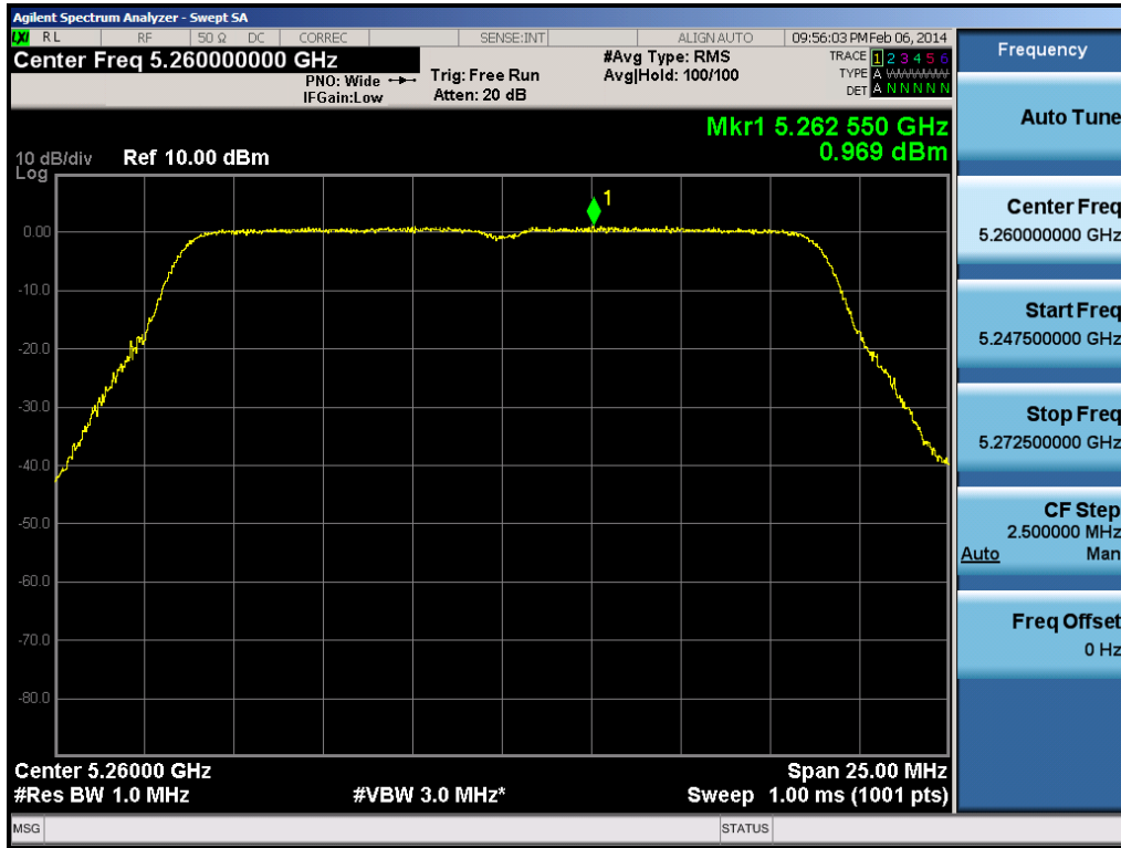
Plot 6-82. Peak Power Spectral Density Plot (20MHz BW 802.11n (UNII Band 2A) – Ch. 52)
