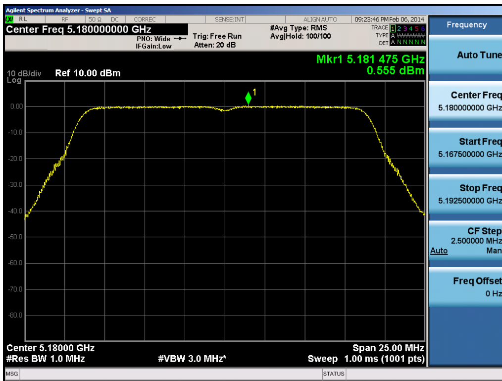
Plot 6-73. Peak Power Spectral Density Plot (20MHz BW 802.11n (UNII Band 1) – Ch. 36)
