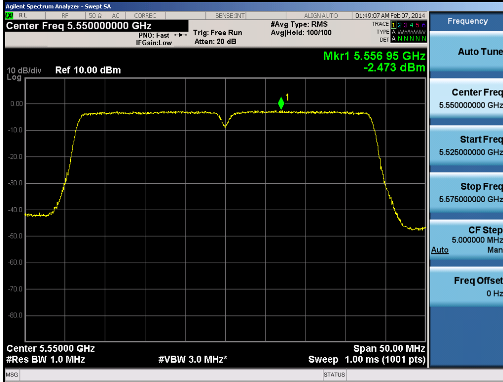
Plot 6-123. Peak Power Spectral Density Plot (40MHz BW 802.11n (UNII Band 2C) – Ch. 110)
