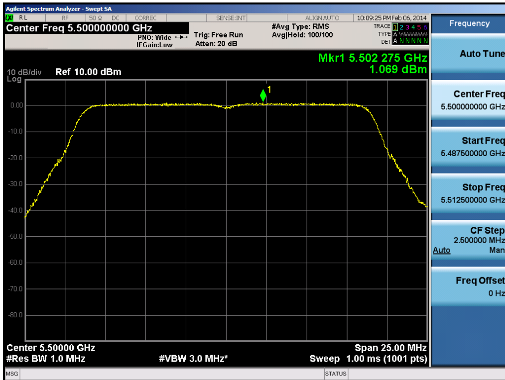
Plot 6-91. Peak Power Spectral Density Plot (20MHz BW 802.11n (UNII Band 2C) – Ch. 100)
