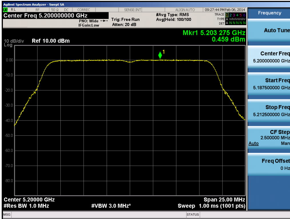
Plot 6-74. Peak Power Spectral Density Plot (20MHz BW 802.11n (UNII Band 1) – Ch. 40)
