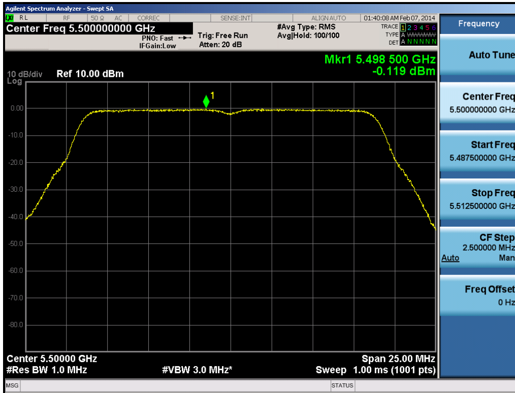
Plot 6-119. Peak Power Spectral Density Plot (20MHz BW 802.11n (UNII Band 2C) – Ch. 100)
