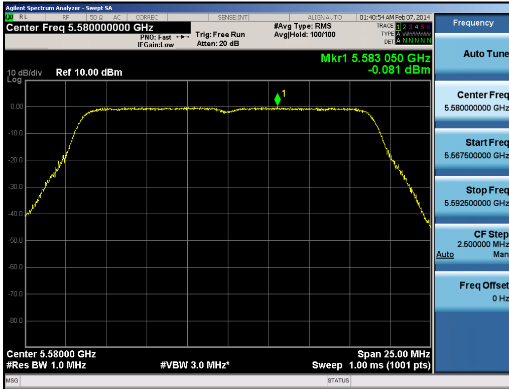
Plot 6-120. Peak Power Spectral Density Plot (20MHz BW 802.11n (UNII Band 2C) – Ch. 116)
