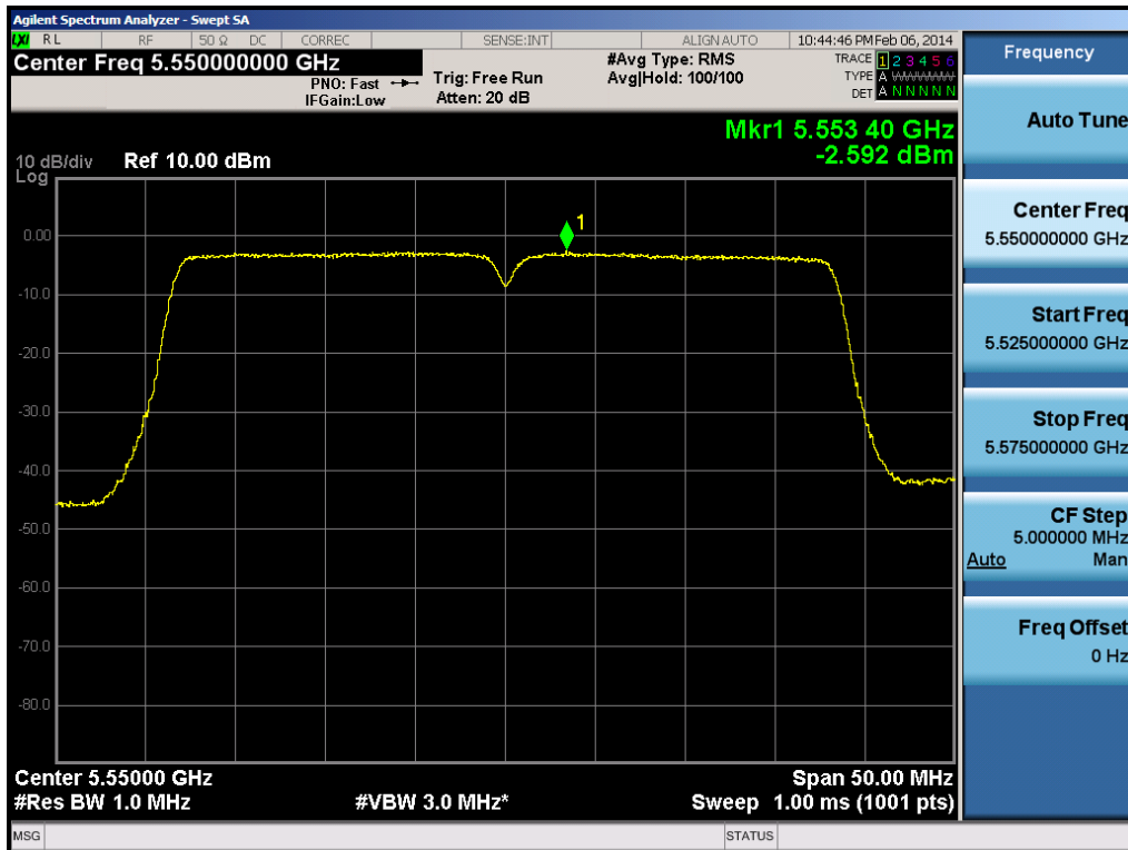
Plot 6-95. Peak Power Spectral Density Plot (40MHz BW 802.11n (UNII Band 2C) – Ch. 110)
