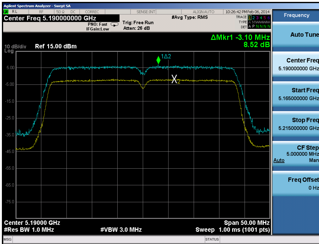
Plot 6-128. Peak Excursion Ratio Plot (40MHz BW 802.11n)
