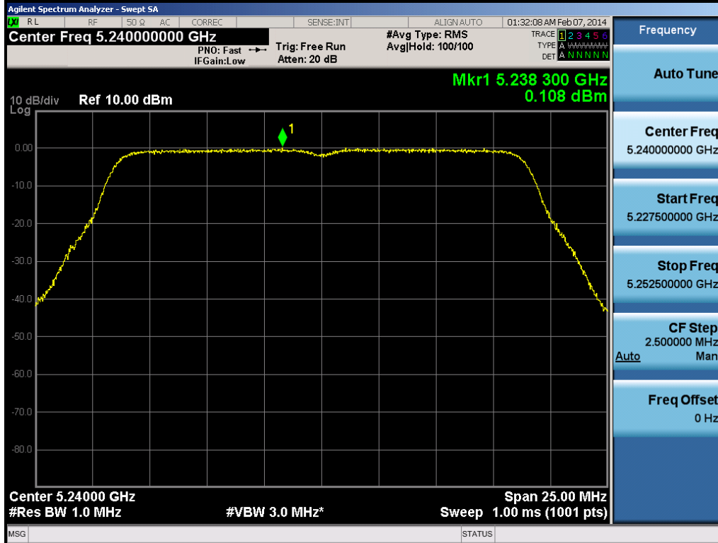
Plot 6-103. Peak Power Spectral Density Plot (20MHz BW 802.11n (UNII Band 1) – Ch. 48)
