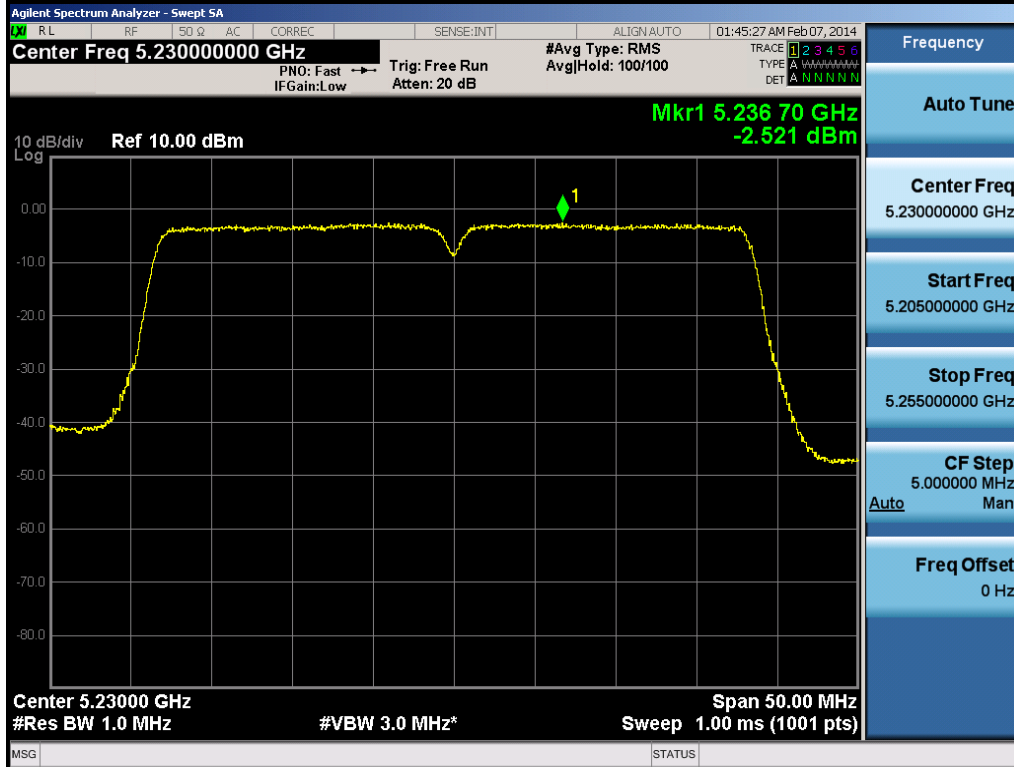
Plot 6-105. Peak Power Spectral Density Plot (40MHz BW 802.11n (UNII Band 1) – Ch. 46)
