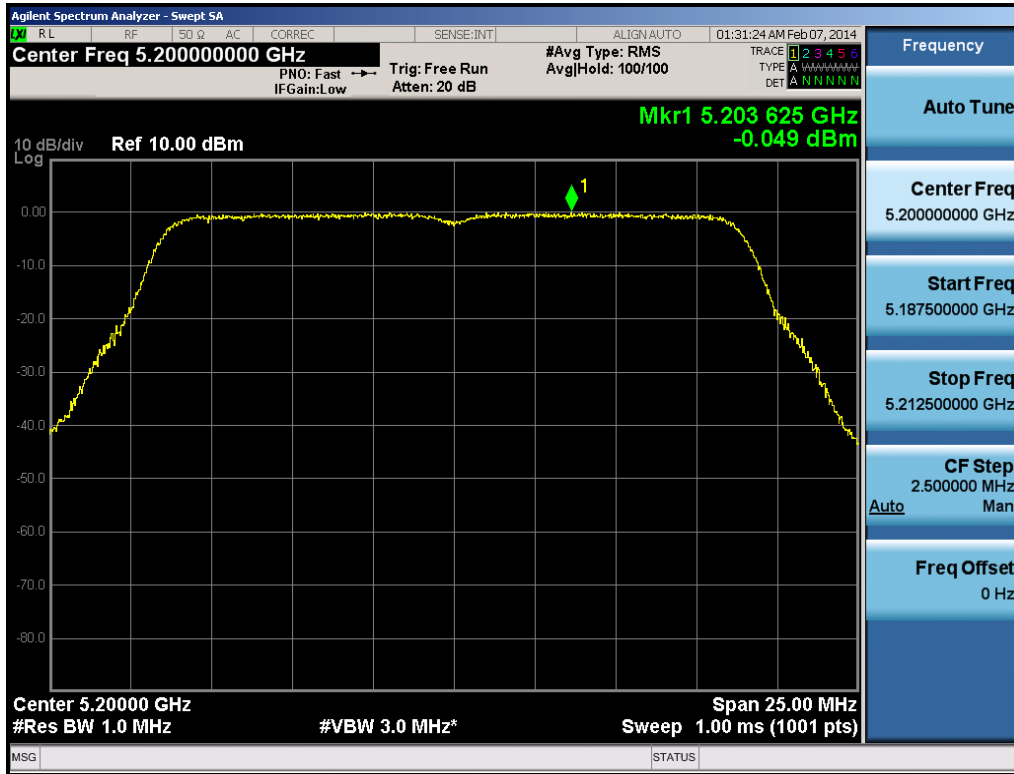
Plot 6-102. Peak Power Spectral Density Plot (20MHz BW 802.11n (UNII Band 1) – Ch. 40)
