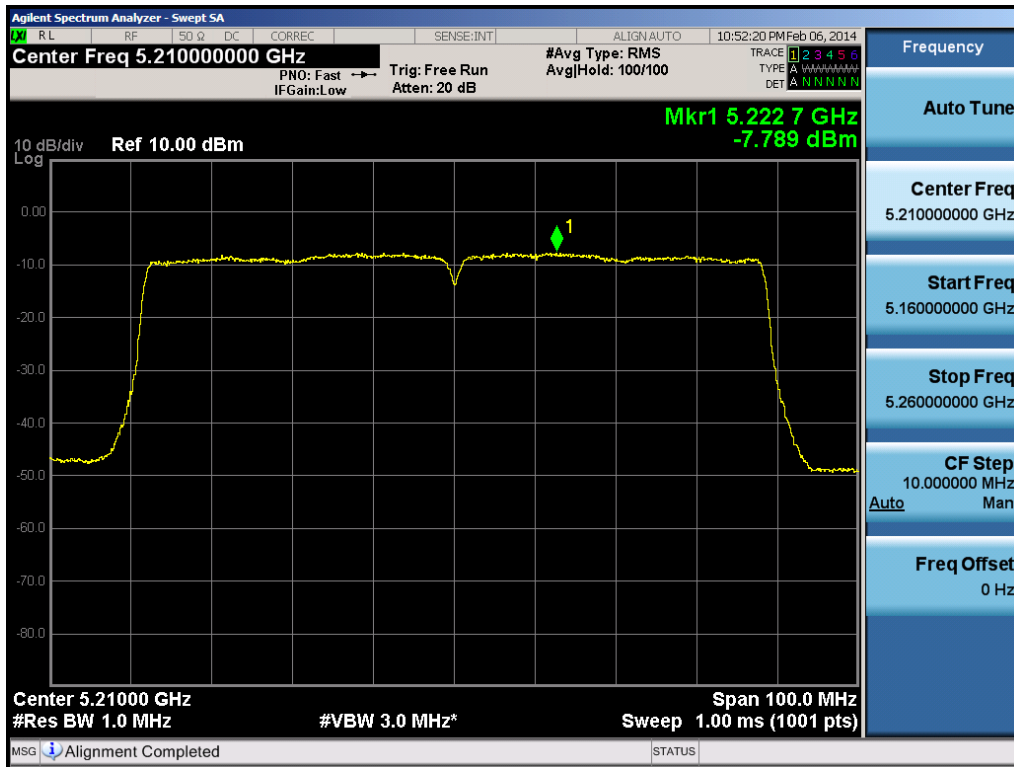
Plot 6-78. Peak Power Spectral Density Plot (80MHz BW 802.11ac (UNII Band 1) – Ch. 42)
