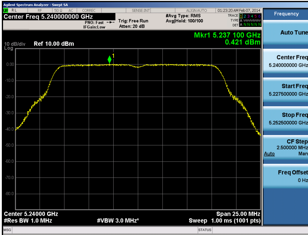
Plot 6-100. Peak Power Spectral Density Plot (802.11a (UNII Band 1) – Ch. 48)
