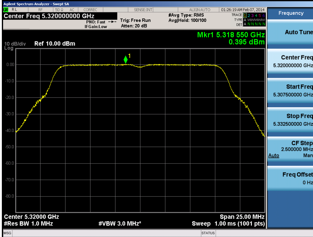
Plot 6-109. Peak Power Spectral Density Plot (802.11a (UNII Band 2A) – Ch. 64)
