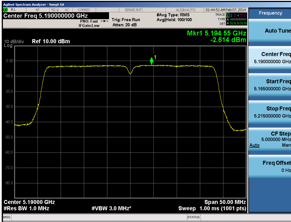
Plot 6-104. Peak Power Spectral Density Plot (40MHz BW 802.11n (UNII Band 1) – Ch. 38)
