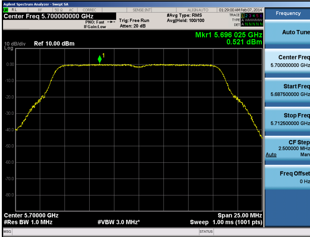
Plot 6-118. Peak Power Spectral Density Plot (802.11a (UNII Band 2C) – Ch. 140)
