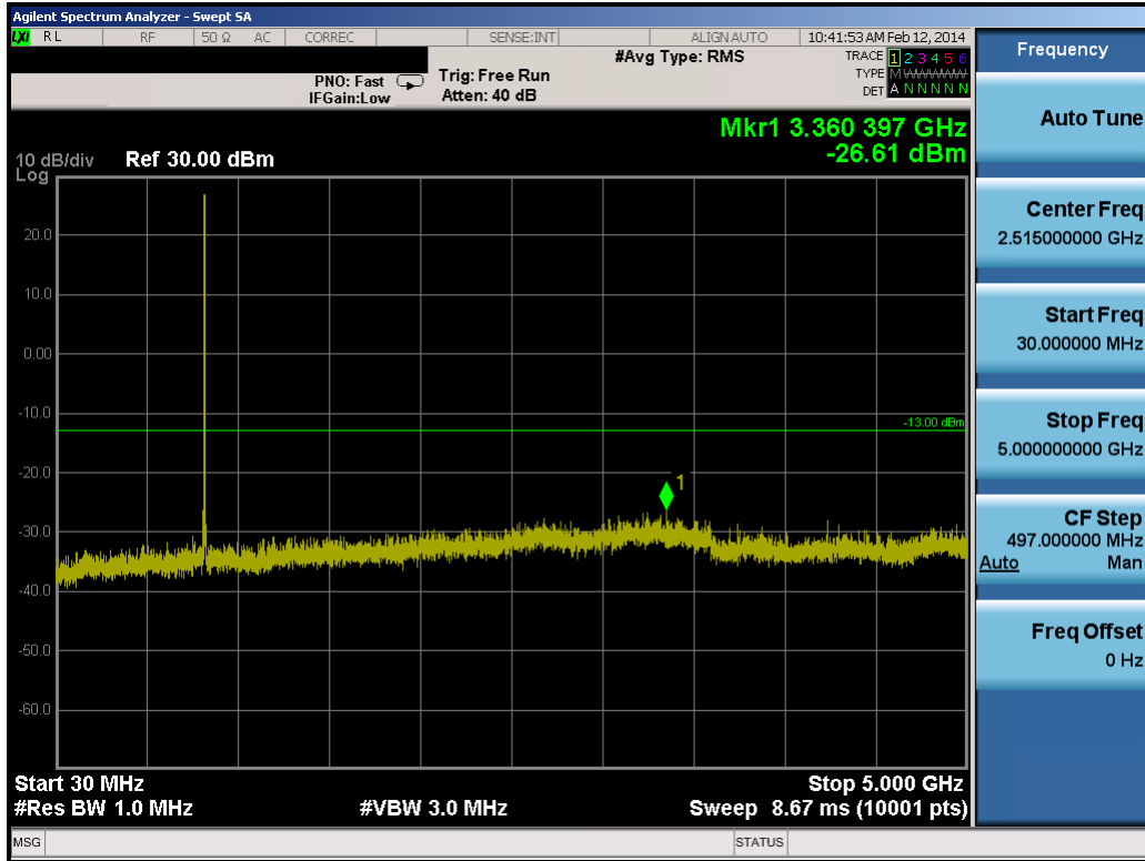
Plot 8-20. Conducted Spurious Plot (10.0MHz QPSK – RB Size 1, RB Offset 0 – High Channel)
