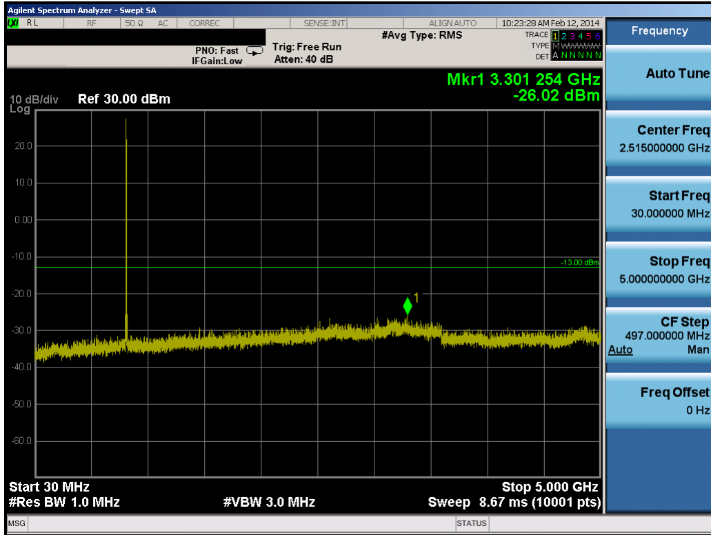
Plot 8-18. Conducted Spurious Plot (10.0MHz QPSK – RB Size 1, RB Offset 0 – Mid Channel)
