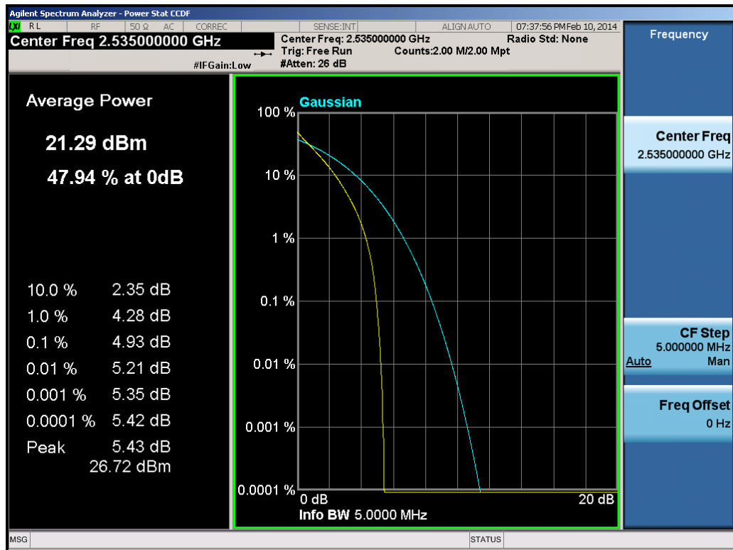
Plot 7-21. Peak-Average Ratio Plot (5.0MHz QPSK – RB Size 25)
