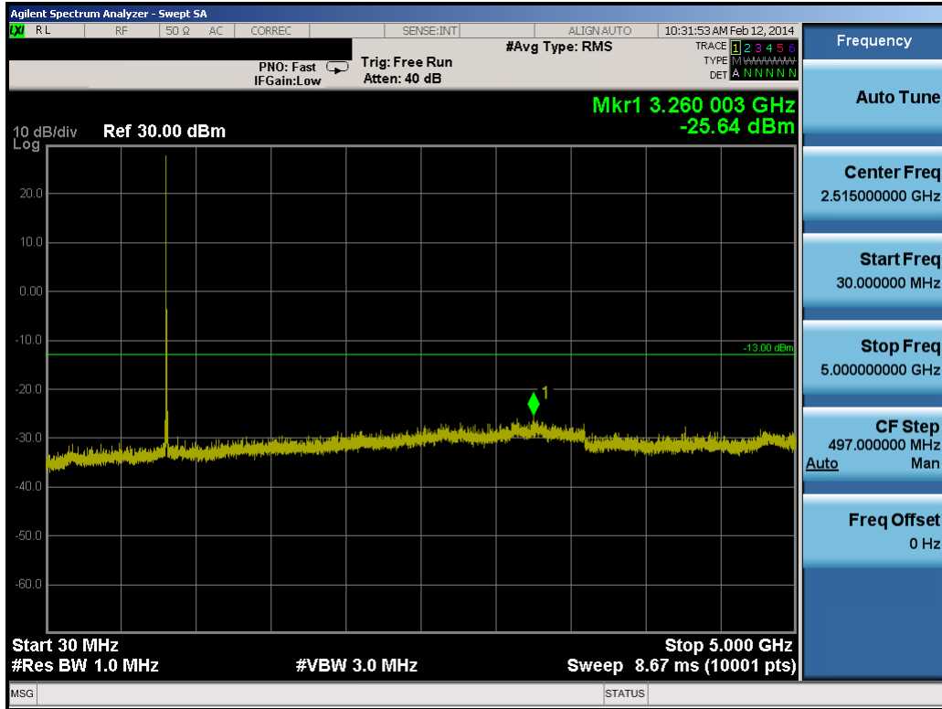
Plot 8-16. Conducted Spurious Plot (10.0MHz QPSK – RB Size 1, RB Offset 0– Low Channel)
