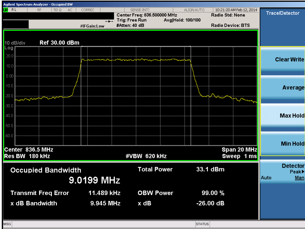
Plot 8-14. Occupied Bandwidth Plot (10.0MHz QPSK – RB Size 50)
