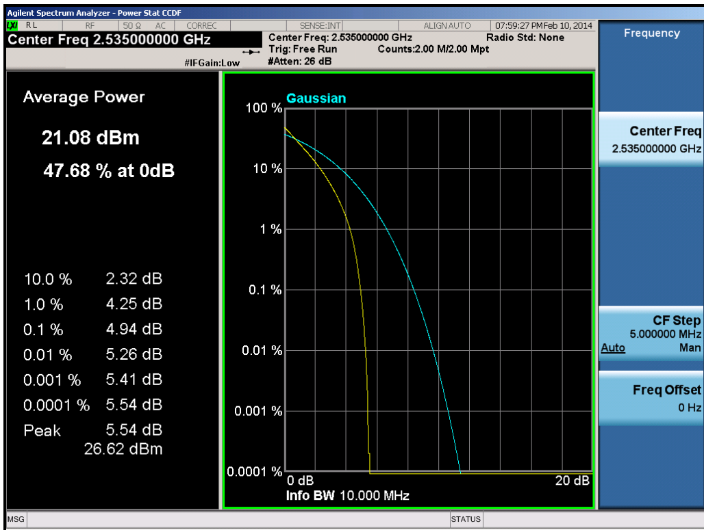
Plot 7-23. Peak-Average Ratio Plot (10.0MHz QPSK – RB Size 50)
