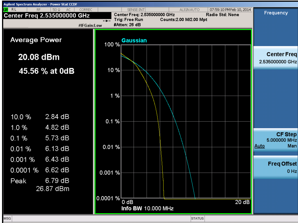
Plot 7-24. Peak-Average Ratio Plot (10.0Mhz 16QAM – RB Size 50)
