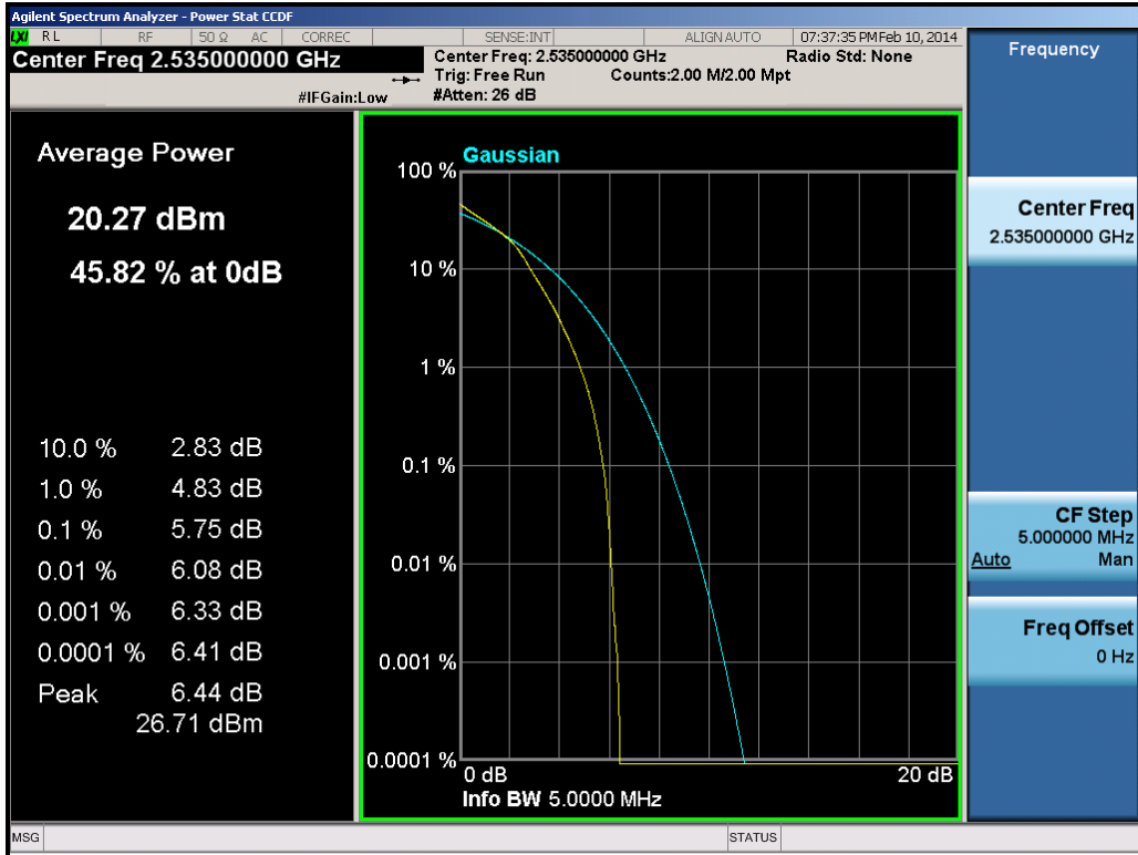
Plot 7-22. Peak-Average Ratio Plot (5.0MHz 16QAM – RB Size 25)
