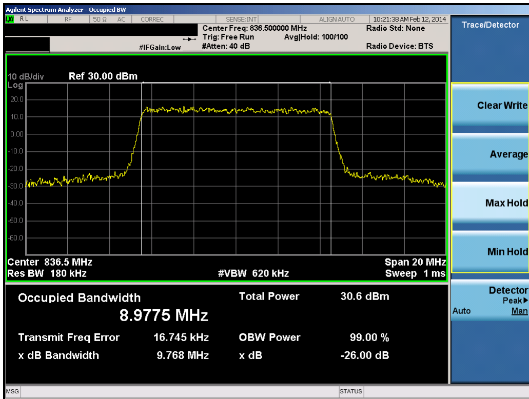
Plot 8-15. Occupied Bandwidth Plot (10.0MHz 16-QAM – RB Size 50)
