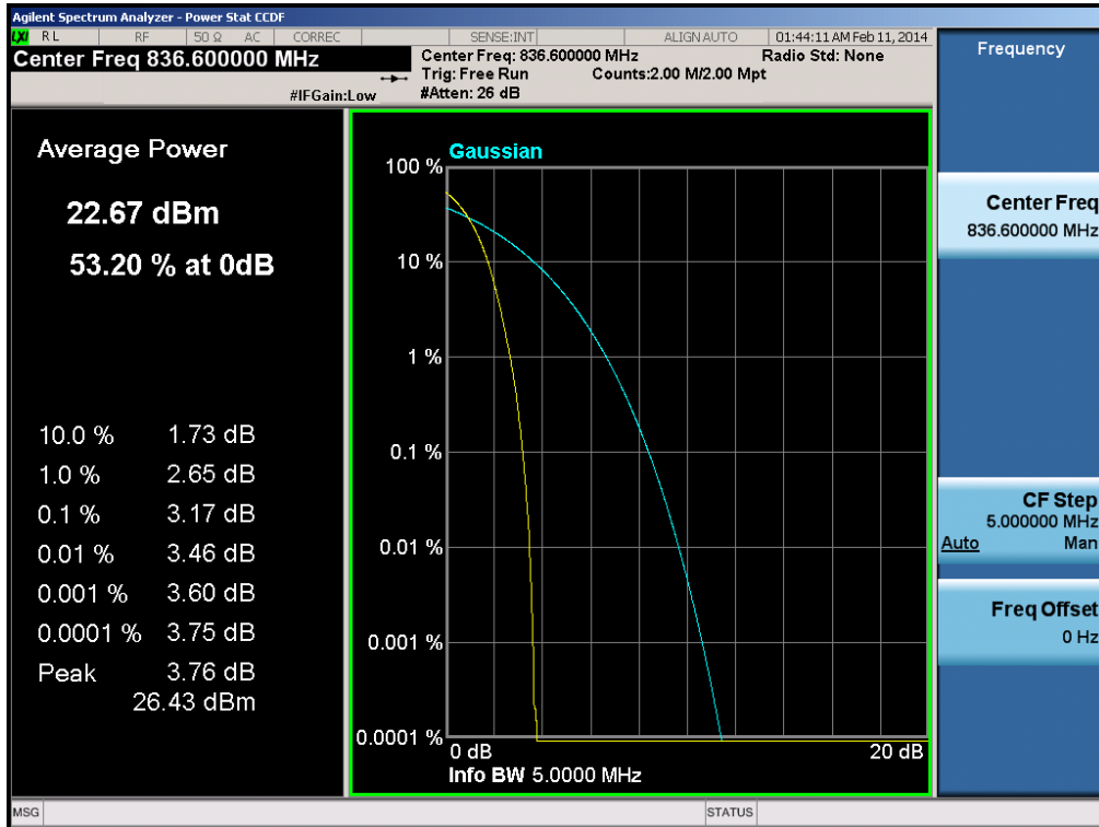
Plot 6-31. Peak-Average Ratio Plot (Cellular WCDMA Mode – Ch. 4183)
