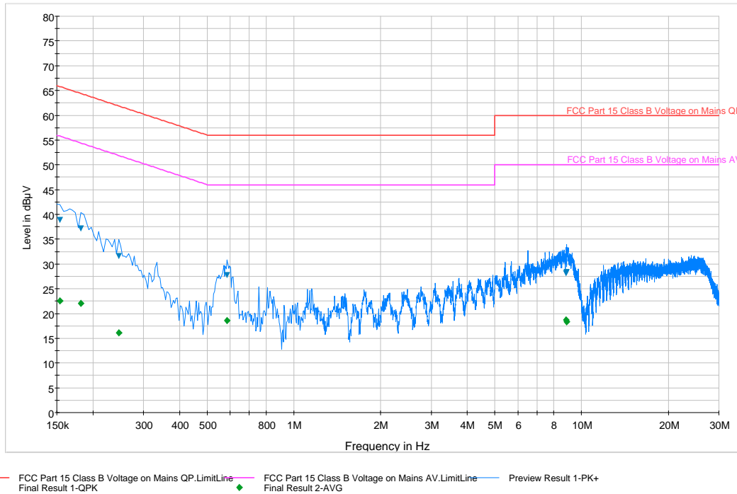
Plot 6-249. Line Conducted Plot with 802.11a UNII Band 2C (N)
