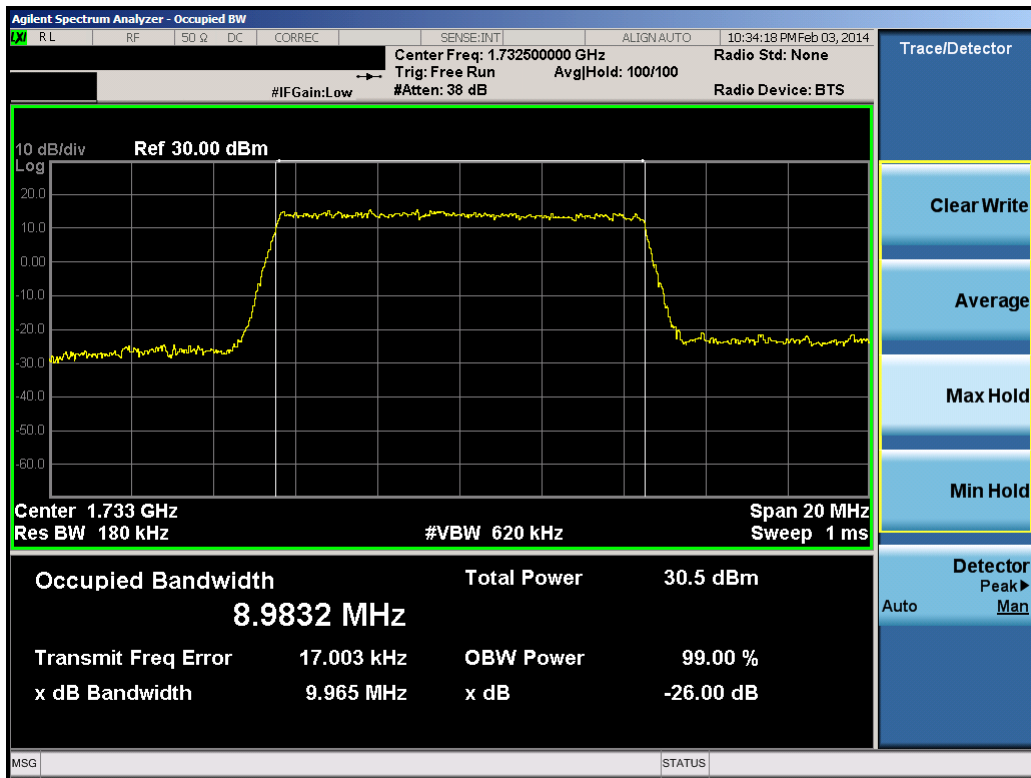
Plot 8-11. Occupied Bandwidth Plot (10.0MHz QPSK – RB Size 50)
