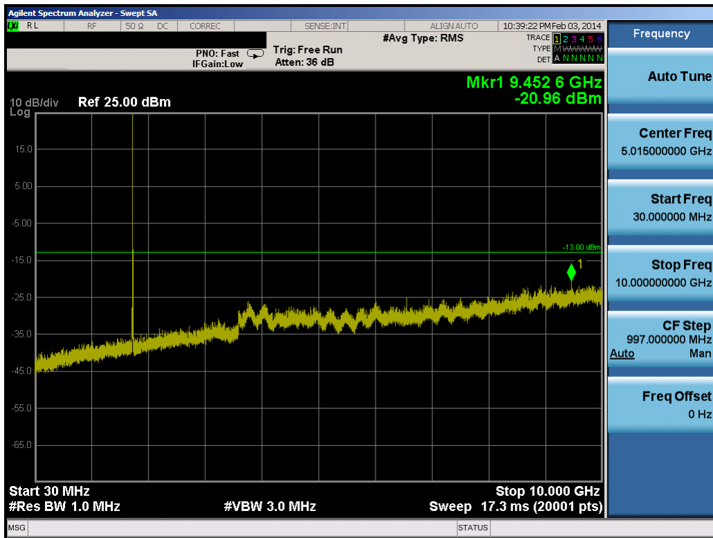
Plot 8-17. Conducted Spurious Plot (10.0MHz QPSK – RB Size 1, RB Offset 0 – High Channel)
