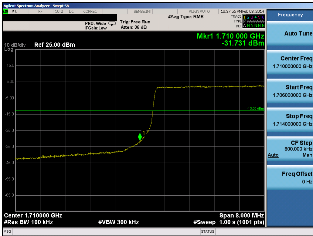
Plot 8-9. Lower Band Edge Plot (10.0MHz QPSK – RB Size 50)
