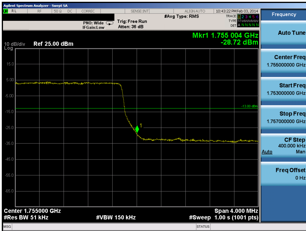
Plot 8-5. Upper Band Edge Plot (5.0MHz QPSK – RB Size 25)
