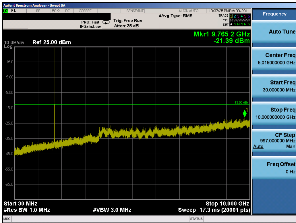
Plot 8-13. Conducted Spurious Plot (10.0MHz QPSK – RB Size 1, RB Offset 0– Low Channel)
