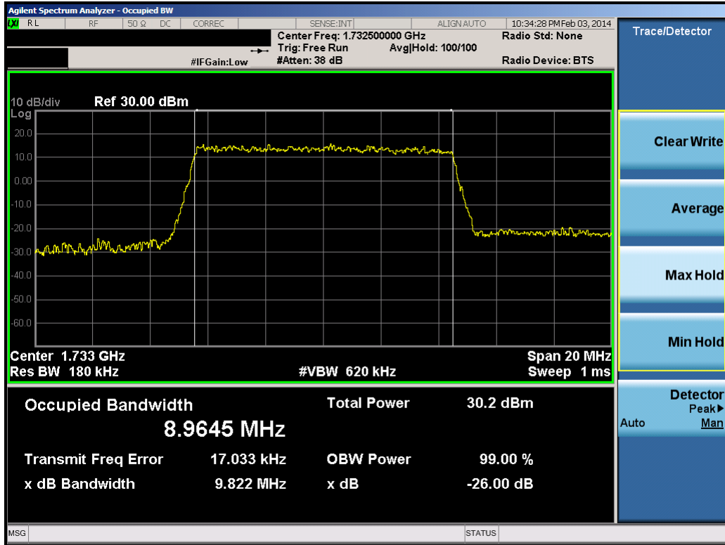
Plot 8-12. Occupied Bandwidth Plot (10.0MHz 16-QAM – RB Size 50)
