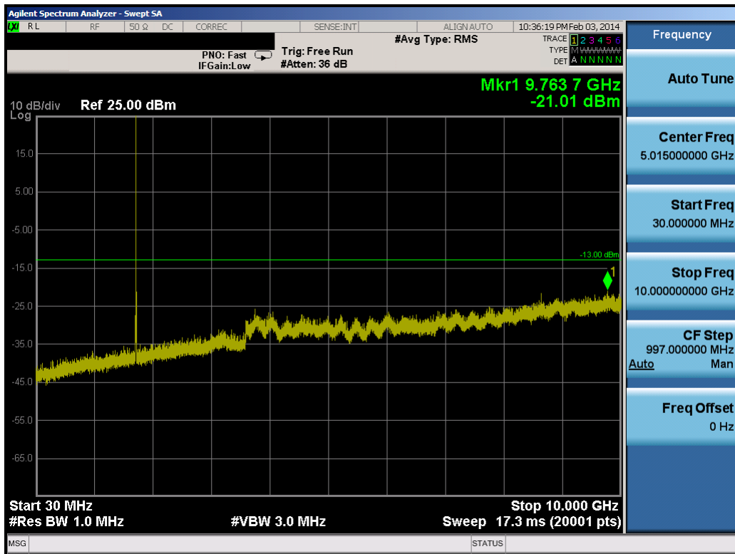
Plot 8-15. Conducted Spurious Plot (10.0MHz QPSK – RB Size 1, RB Offset 0 – Mid Channel)
