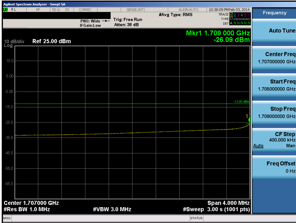
Plot 8-10. Lower Extended Band Edge Plot (10.0MHz QPSK – RB Size 50)
