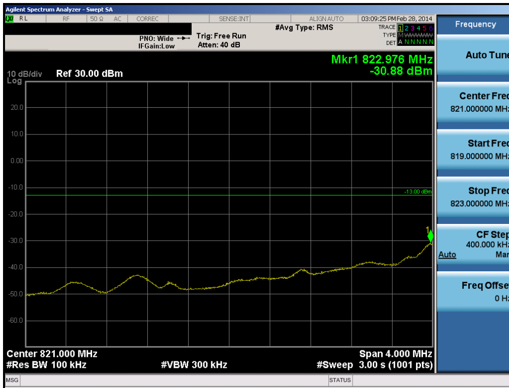
Plot 6-16. Extended Band Edge Plot (Cellular CDMA Mode – Ch. 1013)
