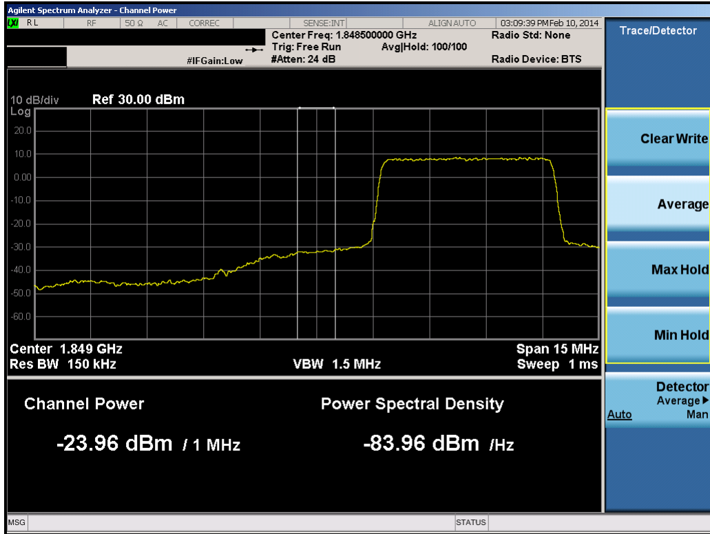
Plot 8-30. Lower Extended Band Edge Plot (5.0MHz QPSK – RB Size 25)
