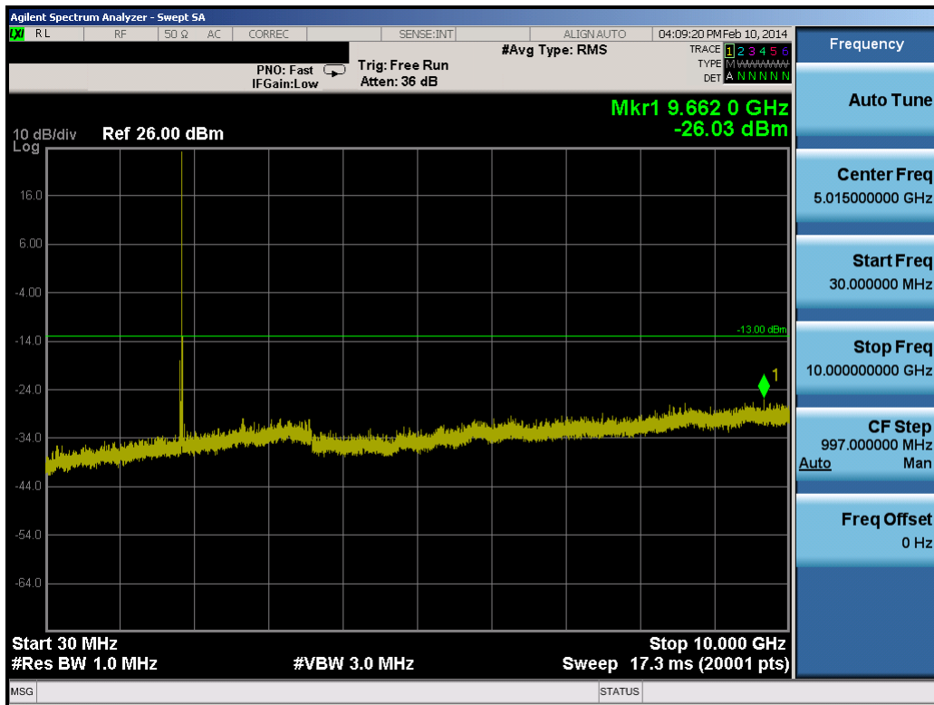
Plot 8-75. Conducted Spurious Plot (20.0MHz QPSK – RB Size 1, RB Offset 0– Low Channel)
