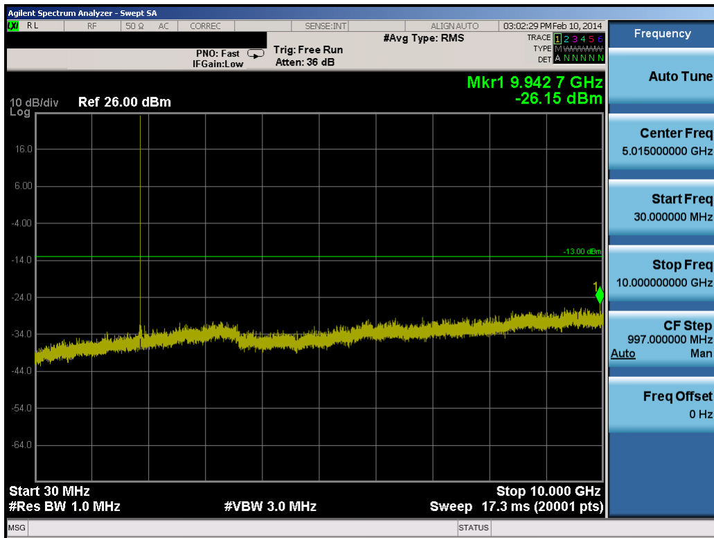
Plot 8-35. Conducted Spurious Plot (5.0MHz QPSK – RB Size 1, RB Offset 0 – Mid Channel)
