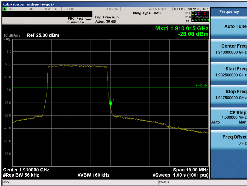
Plot 8-39. Upper Band Edge Plot (5.0MHz QPSK – RB Size 25)
