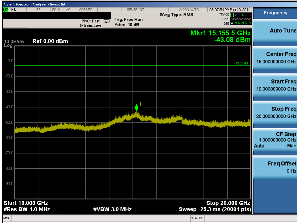
Plot 8-34. Conducted Spurious Plot (5.0MHz QPSK – RB Size 1, RB Offset 0 – Low Channel)
