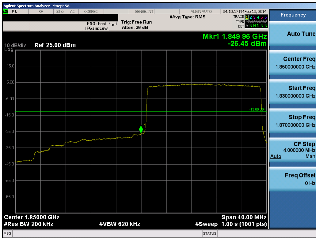
Plot 8-71. Lower Band Edge Plot (20.0MHz QPSK – RB Size 100)
