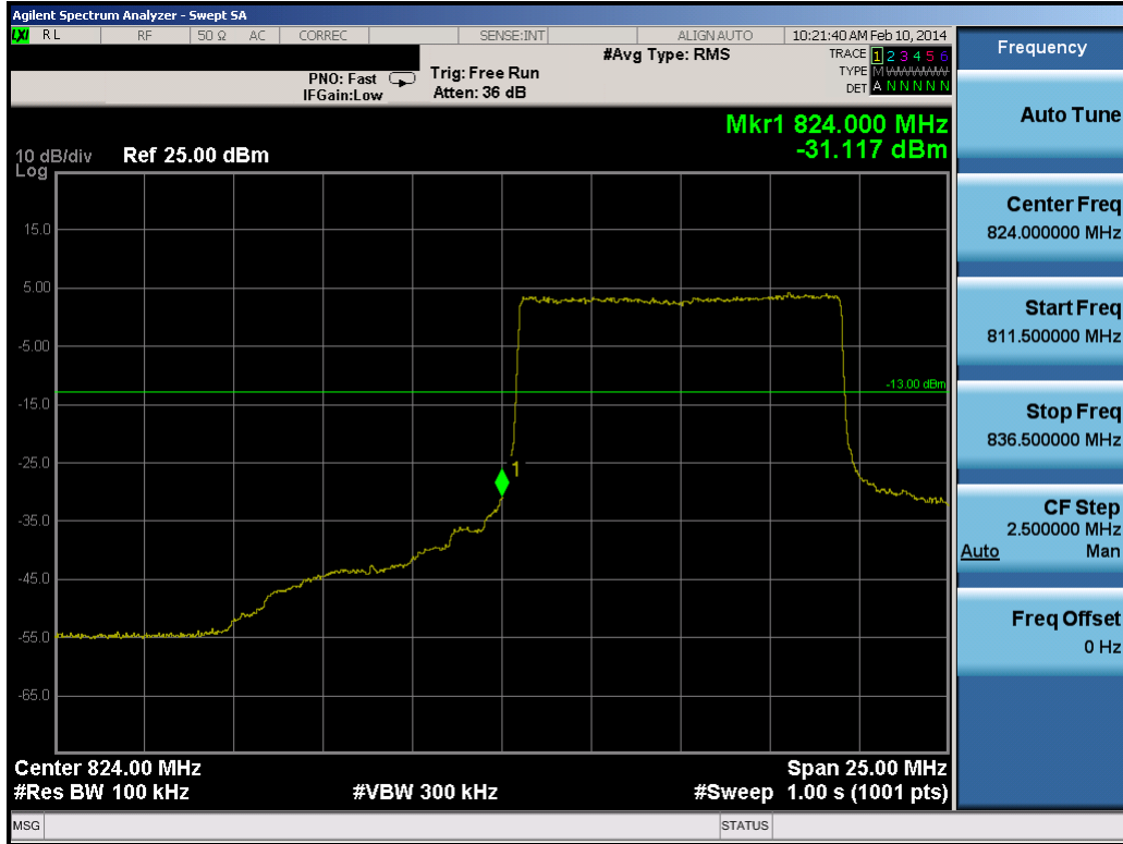
Plot 7-31. Lower Band Edge Plot (10.0MHz QPSK – RB Size 50)
