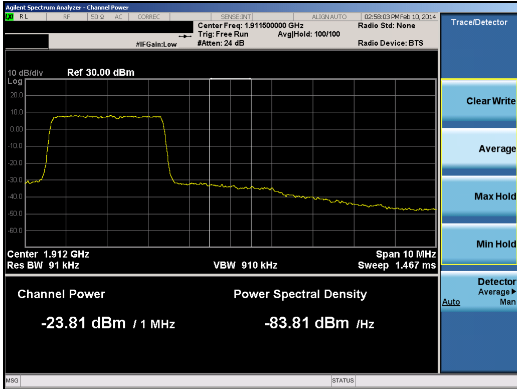
Plot 8-26. Upper Extended Band Edge Plot (3.0MHz QPSK – RB Size 15)
