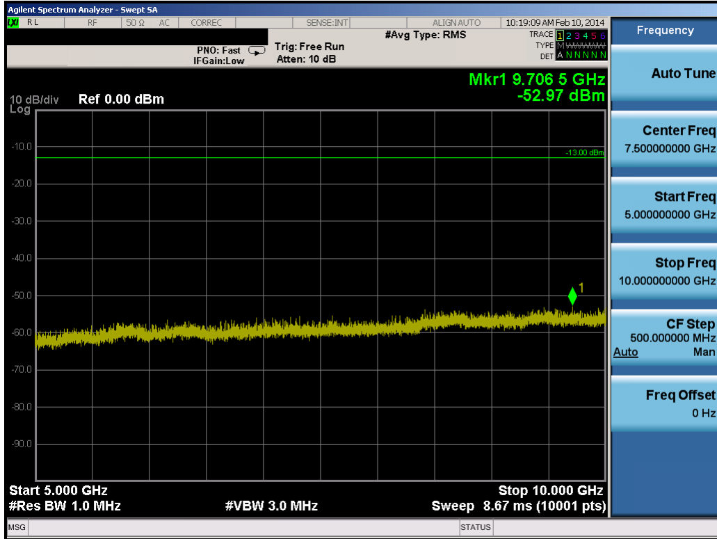
Plot 7-37. Conducted Spurious Plot (10.0MHz QPSK – RB Size 1, RB Offset 0 – Mid Channel)
