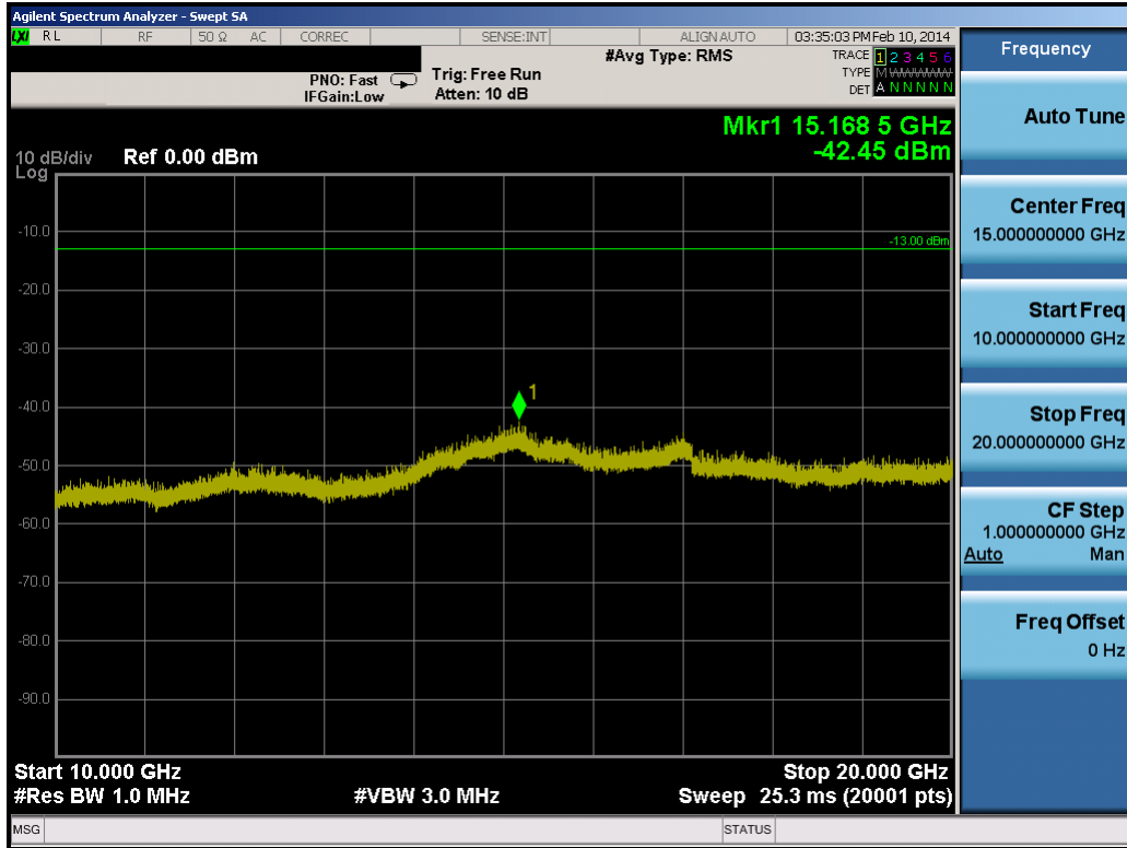
Plot 8-52. Conducted Spurious Plot (10.0MHz QPSK – RB Size 1, RB Offset 0 – High Channel)
