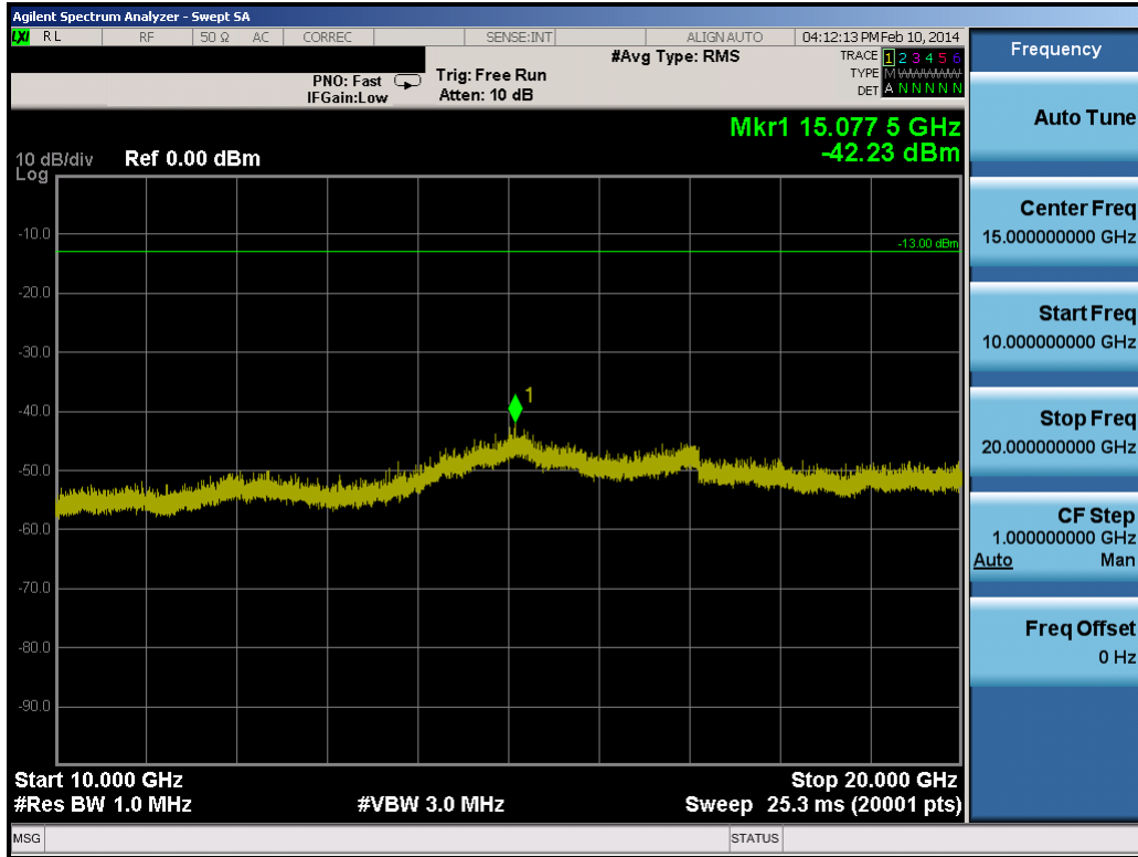
Plot 8-80. Conducted Spurious Plot (20.0MHz QPSK – RB Size 1, RB Offset 0 – High Channel)
