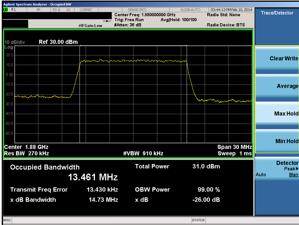
Plot 8-60. Occupied Bandwidth Plot (15.0MHz 16-QAM – RB Size 75)
