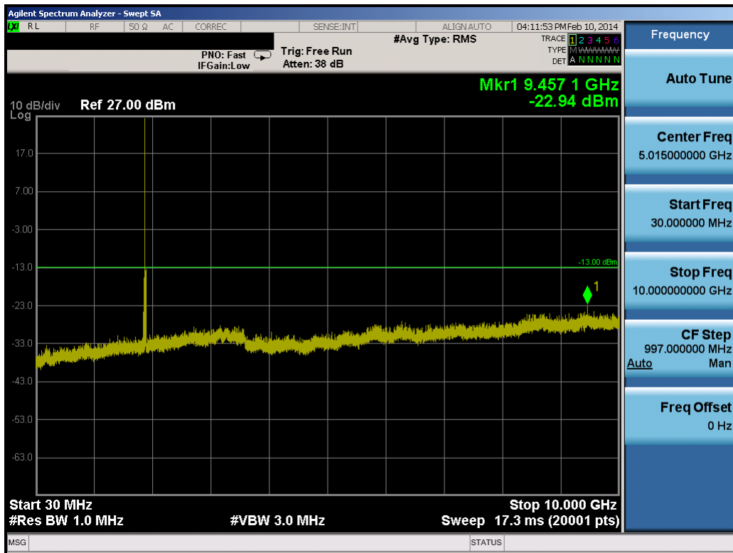
Plot 8-79. Conducted Spurious Plot (20.0MHz QPSK – RB Size 1, RB Offset 0 – High Channel)
