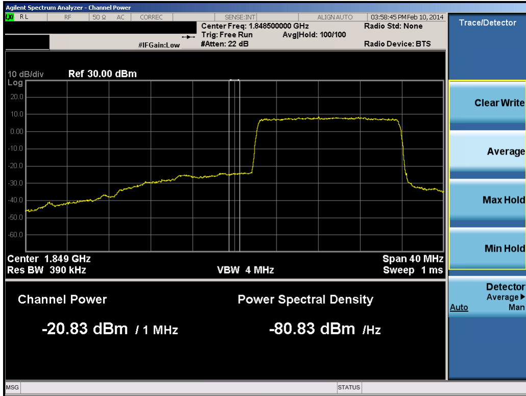
Plot 8-58. Lower Extended Band Edge Plot (15.0MHz QPSK – RB Size 75)
