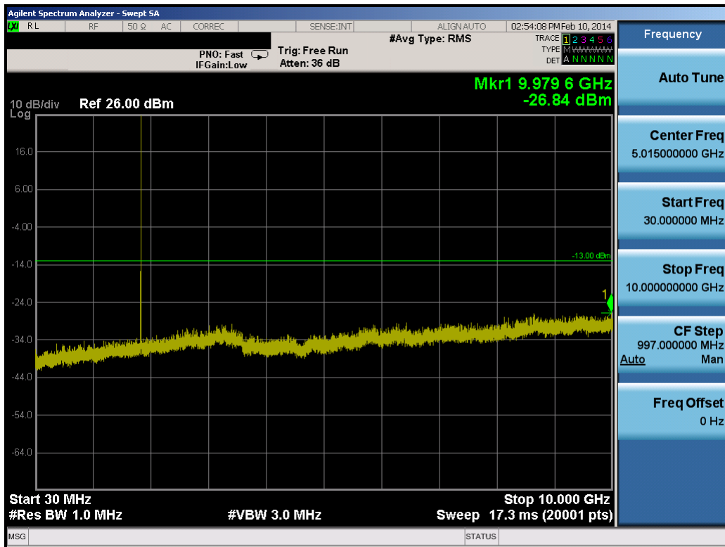
Plot 8-19. Conducted Spurious Plot (3.0MHz QPSK – RB Size 1, RB Offset 0 – Low Channel)
