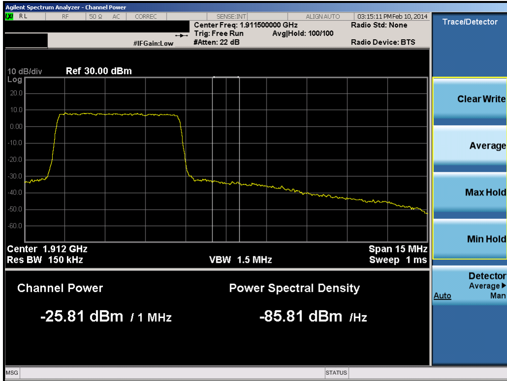
Plot 8-40. Upper Extended Band Edge Plot (5.0MHz QPSK – RB Size 25)
