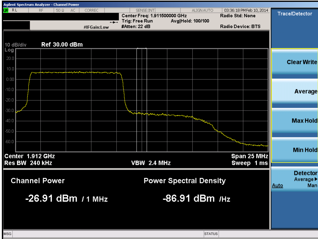
Plot 8-54. Upper Extended Band Edge Plot (10.0MHz QPSK – RB Size 50)
