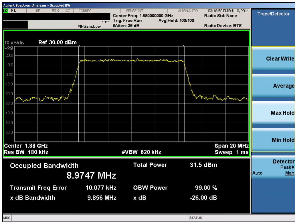
Plot 8-45. Occupied Bandwidth Plot (10.0MHz QPSK – RB Size 50)
