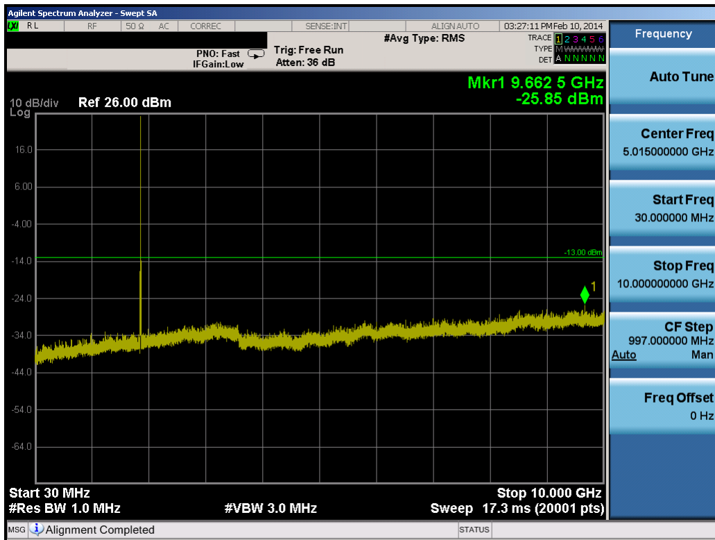
Plot 8-49. Conducted Spurious Plot (10.0MHz QPSK – RB Size 1, RB Offset 0 – Mid Channel)
