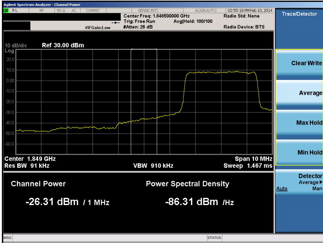
Plot 8-16. Lower Extended Band Edge Plot (3.0MHz QPSK – RB Size 15)
