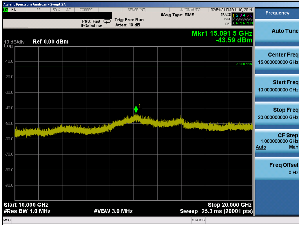
Plot 8-20. Conducted Spurious Plot (3.0MHz QPSK – RB Size 1, RB Offset 0 – Low Channel)
