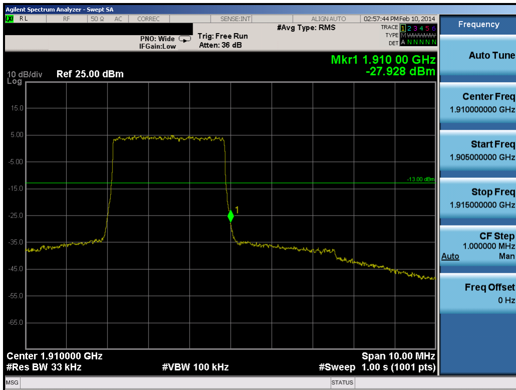
Plot 8-25. Upper Band Edge Plot (3.0MHz QPSK – RB Size 15)
