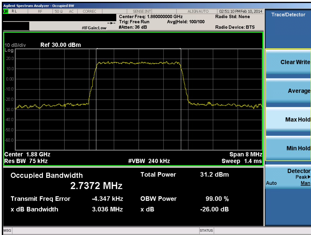
Plot 8-17. Occupied Bandwidth Plot (3.0MHz QPSK – RB Size 15)
