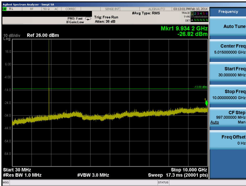
Plot 8-37. Conducted Spurious Plot (5.0MHz QPSK – RB Size 1, RB Offset 0 – High Channel)
