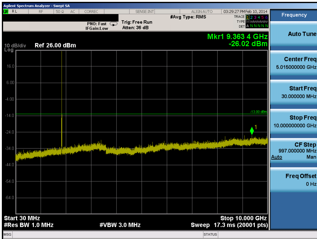
Plot 8-47. Conducted Spurious Plot (10.0MHz QPSK – RB Size 1, RB Offset 0– Low Channel)
