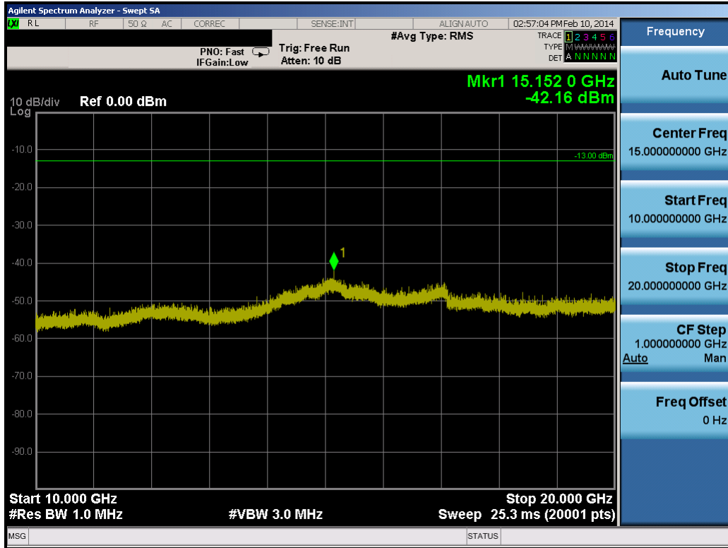
Plot 8-24. Conducted Spurious Plot (3.0MHz QPSK – RB Size 1, RB Offset 0 – High Channel)
