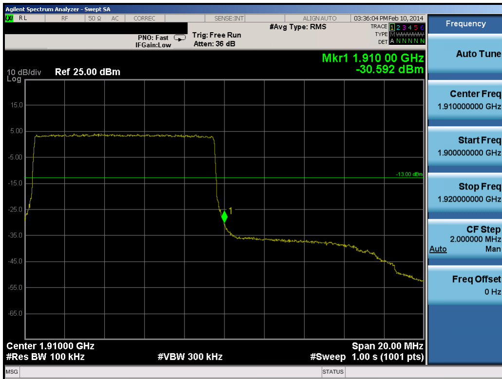
Plot 8-53. Upper Band Edge Plot (10.0MHz QPSK – RB Size 50)
