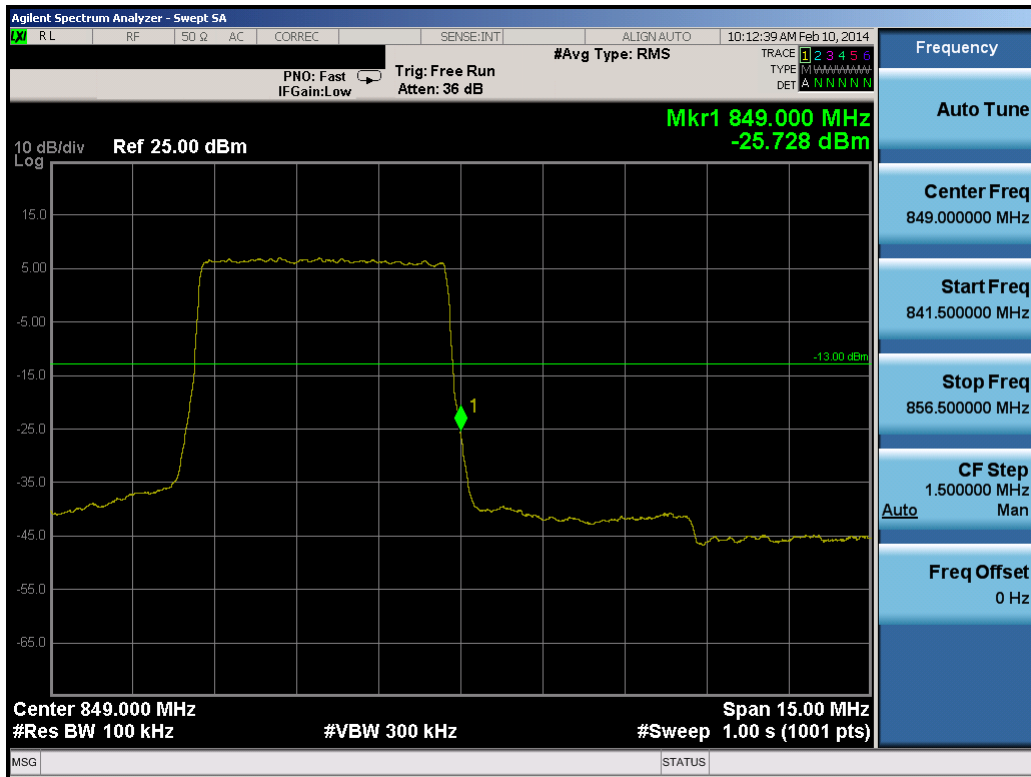
Plot 7-30. Upper Band Edge Plot (5.0MHz QPSK – RB Size 25)
