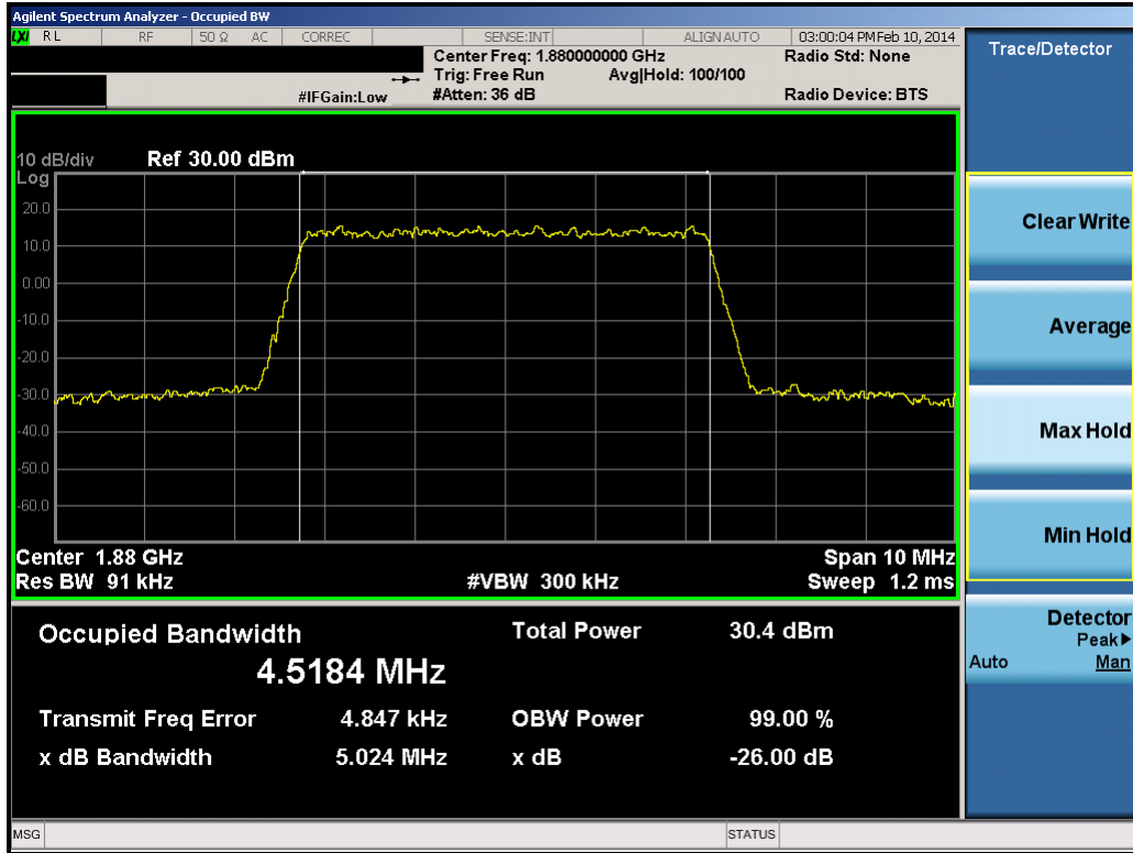
Plot 8-32. Occupied Bandwidth Plot (5.0MHz 16-QAM – RB Size 25)
