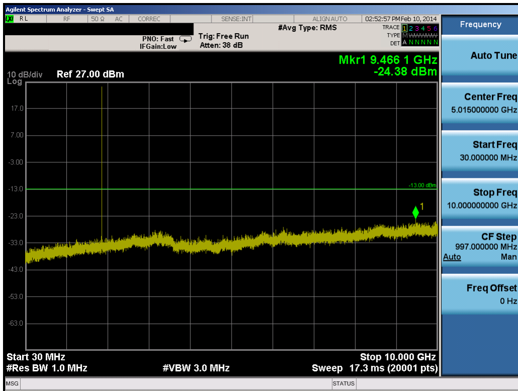
Plot 8-21. Conducted Spurious Plot (3.0MHz QPSK – RB Size 1, RB Offset 0 – Mid Channel)
