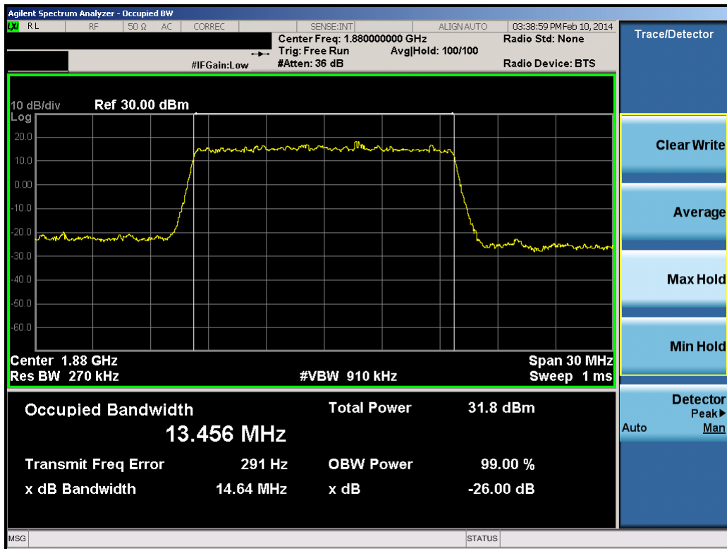
Plot 8-59. Occupied Bandwidth Plot (15.0MHz QPSK – RB Size 75)
