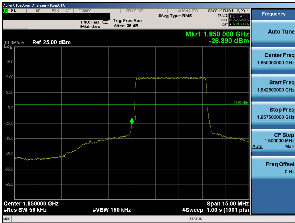
Plot 8-29. Lower Band Edge Plot (5.0MHz QPSK – RB Size 25)
