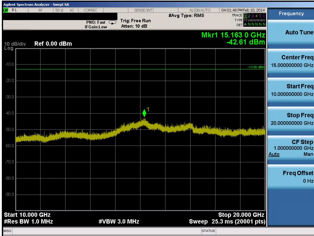
Plot 8-66. Conducted Spurious Plot (15.0MHz QPSK – RB Size 1, RB Offset 0 – High Channel)
