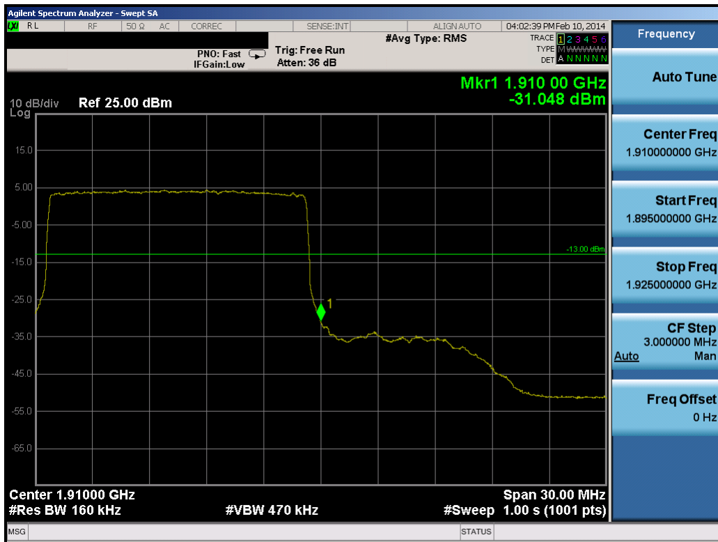
Plot 8-67. Upper Band Edge Plot (15.0MHz QPSK – RB Size 75)
