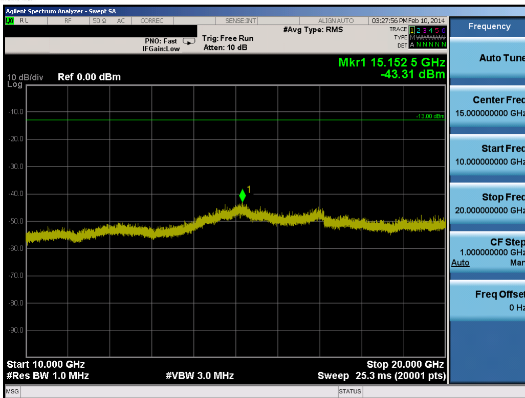
Plot 8-50. Conducted Spurious Plot (10.0MHz QPSK – RB Size 1, RB Offset 0 – Mid Channel)
