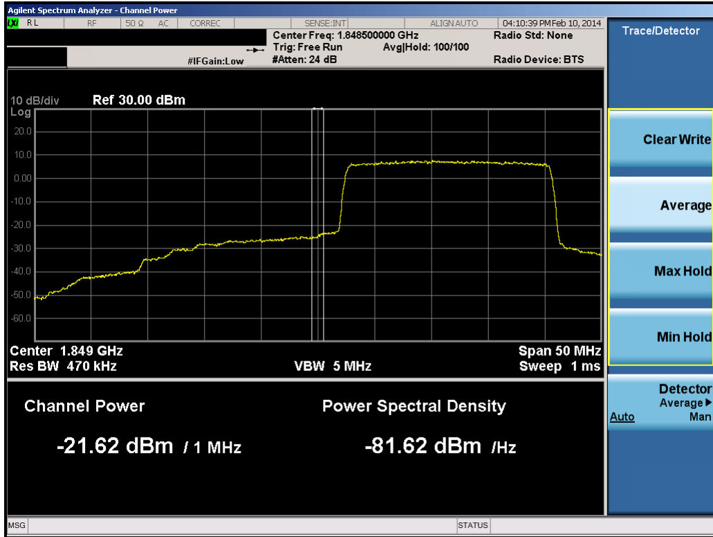
Plot 8-72. Lower Extended Band Edge Plot (20.0MHz QPSK – RB Size 100)
