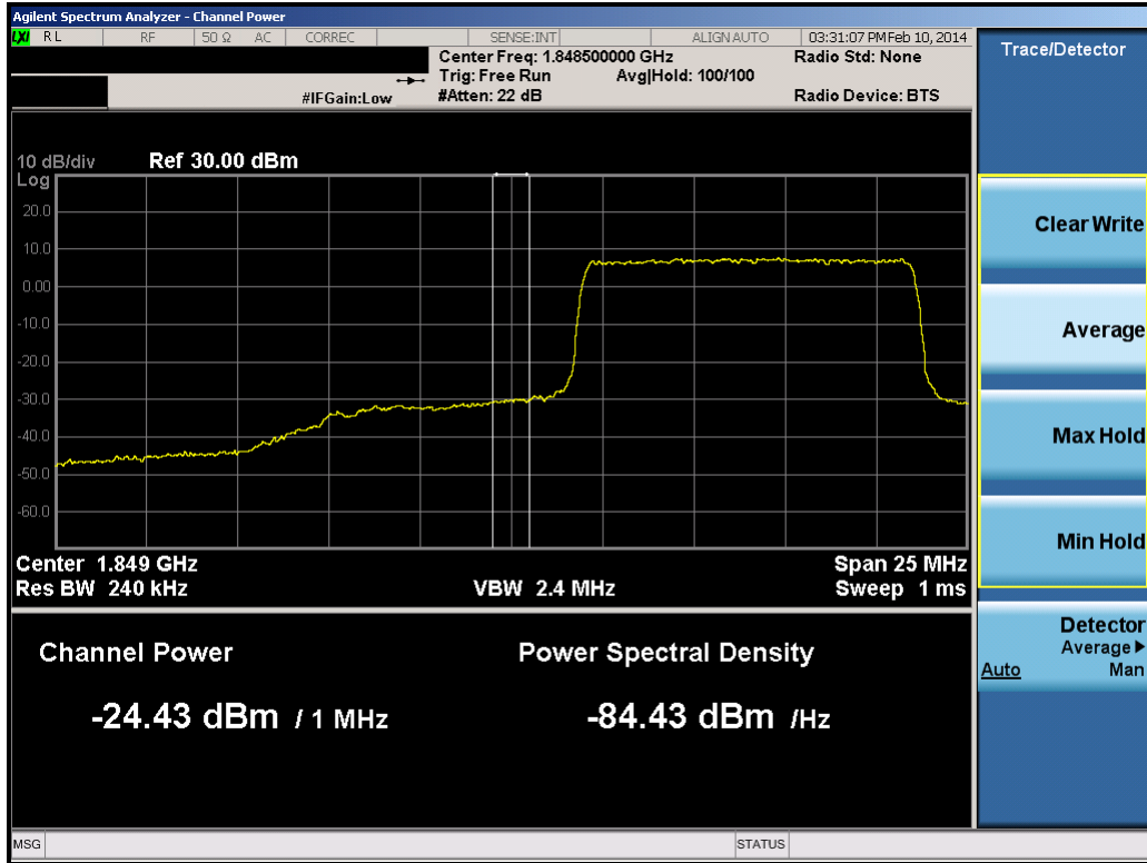
Plot 8-44. Lower Extended Band Edge Plot (10.0MHz QPSK – RB Size 50)
