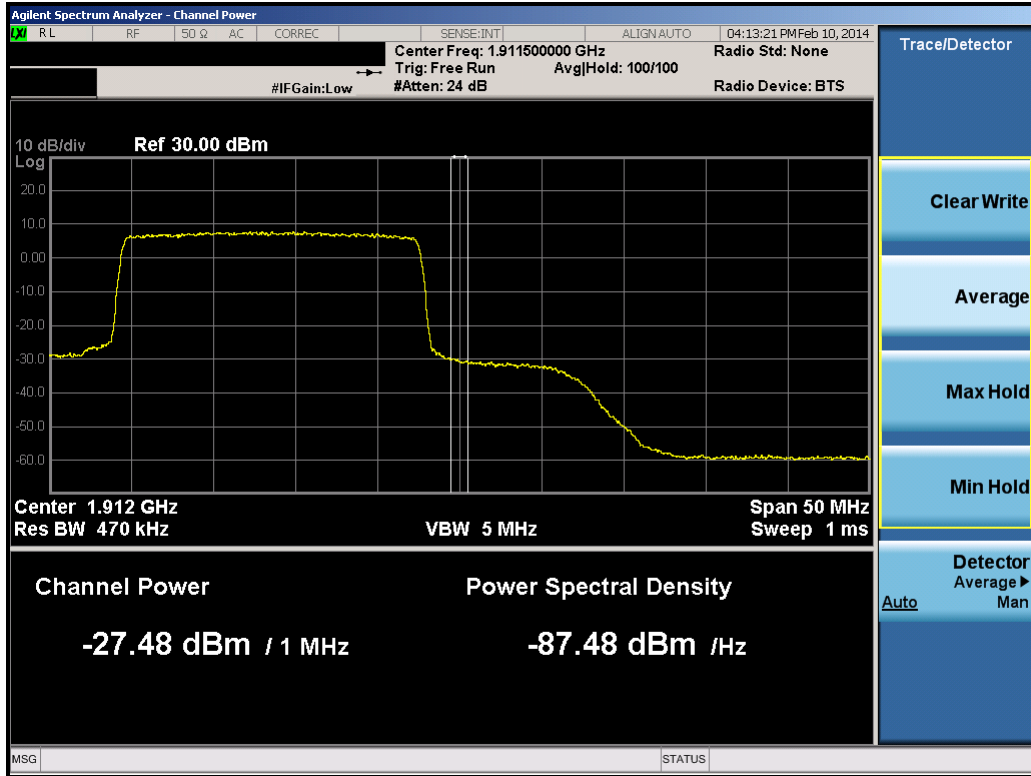
Plot 8-82. Upper Extended Band Edge Plot (20.0MHz QPSK – RB Size 100)
