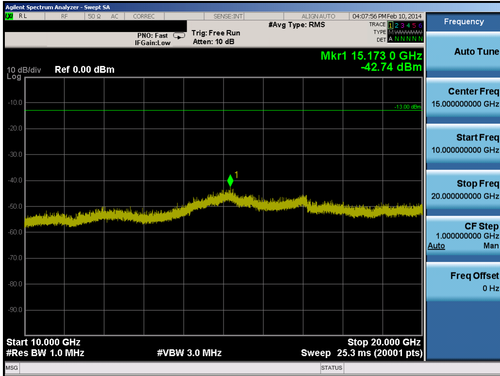
Plot 8-78. Conducted Spurious Plot (20.0MHz QPSK – RB Size 1, RB Offset 0 – Mid Channel)
