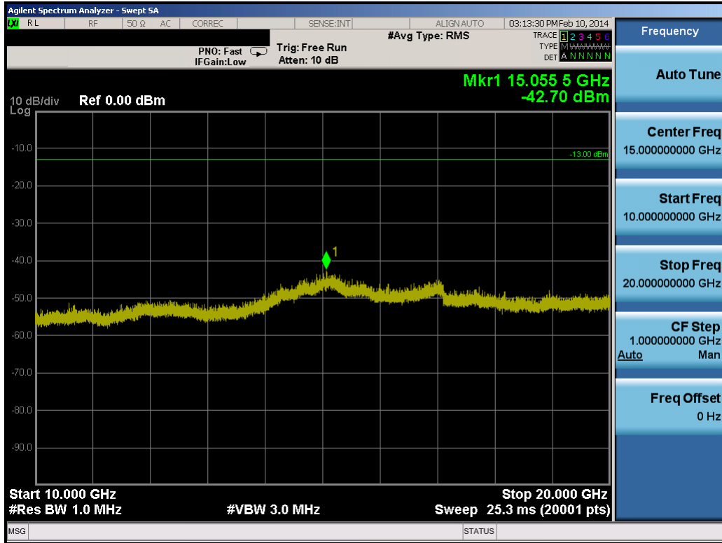
Plot 8-38. Conducted Spurious Plot (5.0MHz QPSK – RB Size 1, RB Offset 0 – High Channel)
