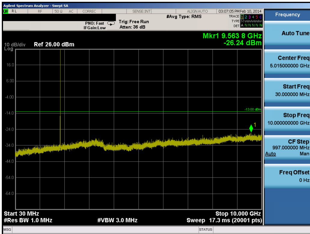
Plot 8-33. Conducted Spurious Plot (5.0MHz QPSK – RB Size 1, RB Offset 0 – Low Channel)
