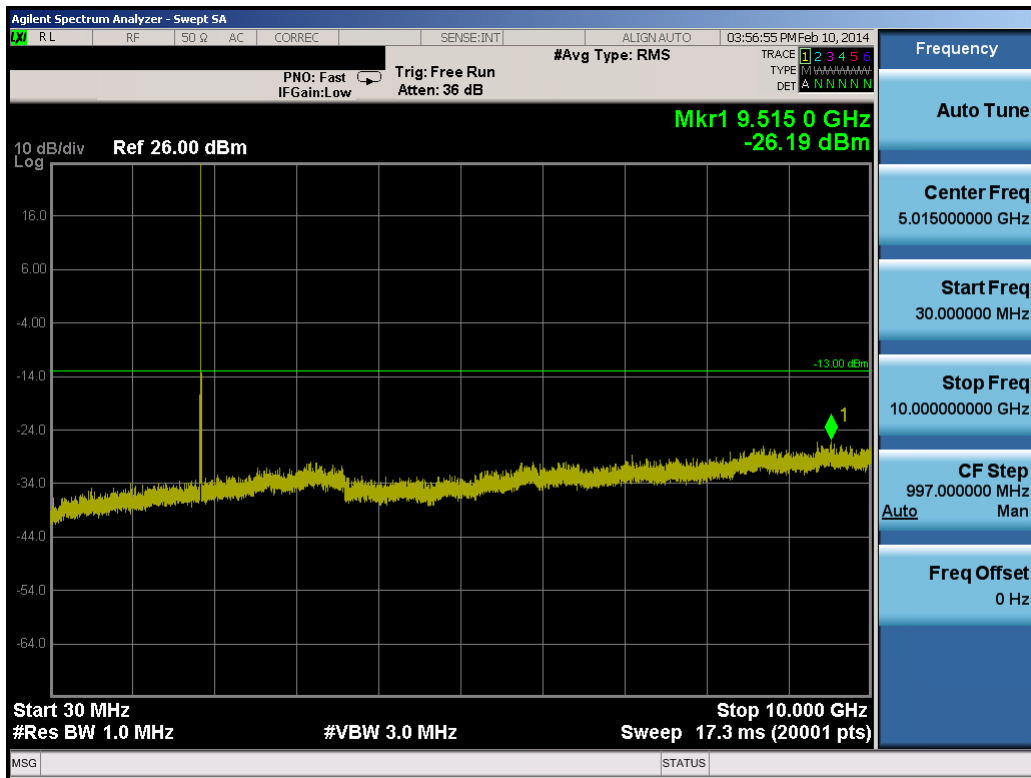
Plot 8-61. Conducted Spurious Plot (15.0MHz QPSK – RB Size 1, RB Offset 0 – Low Channel)
