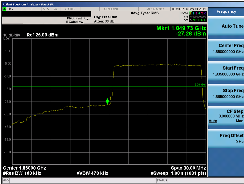
Plot 8-57. Lower Band Edge Plot (15.0MHz QPSK – RB Size 75)
