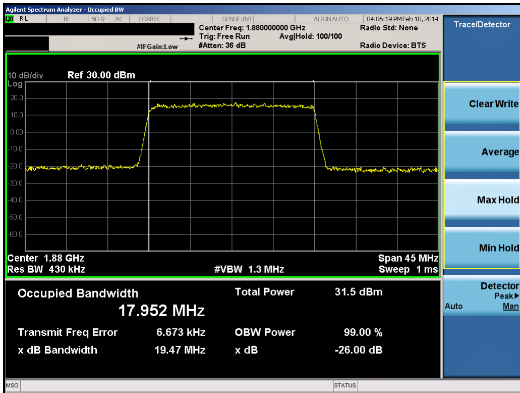
Plot 8-73. Occupied Bandwidth Plot (20.0MHz QPSK – RB Size 100)
