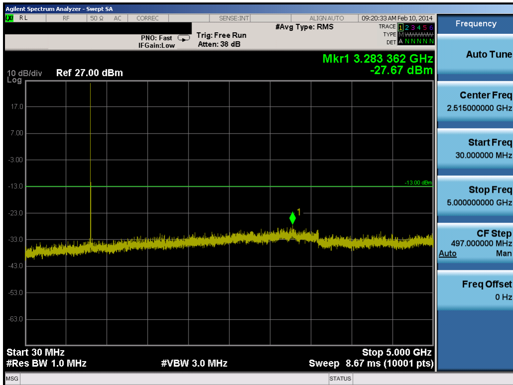
Plot 7-4. Conducted Spurious Plot (1.4MHz QPSK – RB Size 1, RB Offset 0 – Low Channel)
