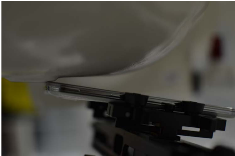
SAR Test Setup Photo 2 – Right Tilt, Standard Battery Cover
