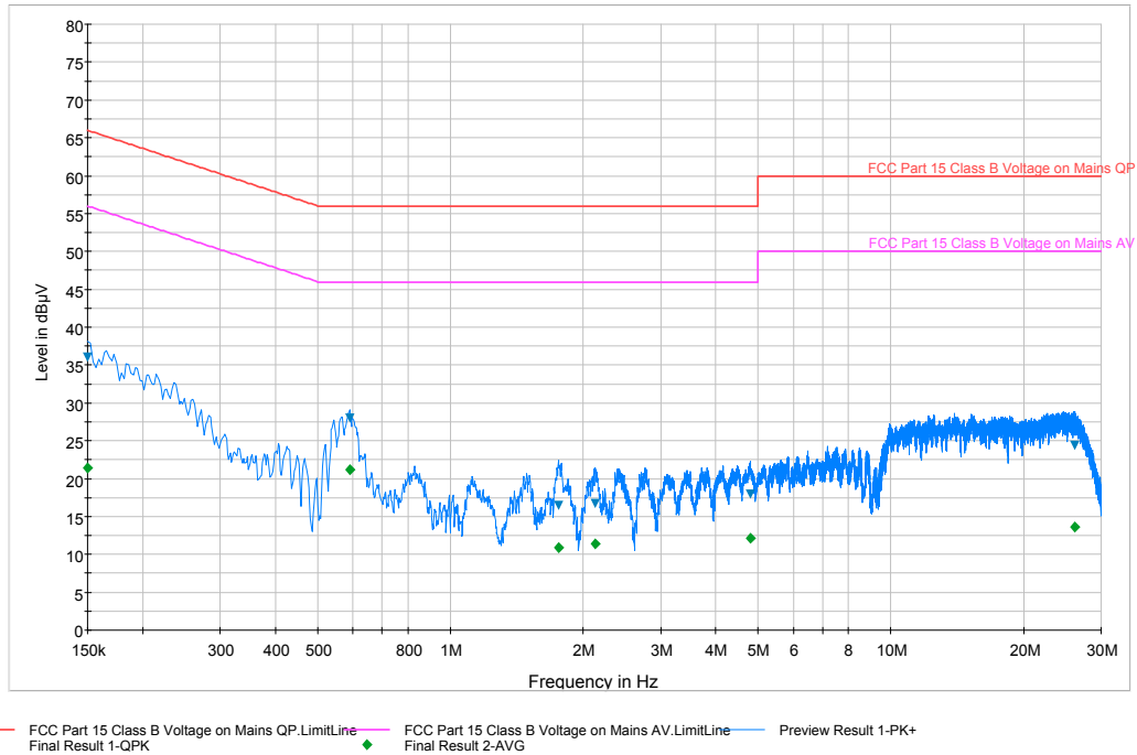
Plot 6-22. Line Conducted Plot with Bluetooth LE (L1)
