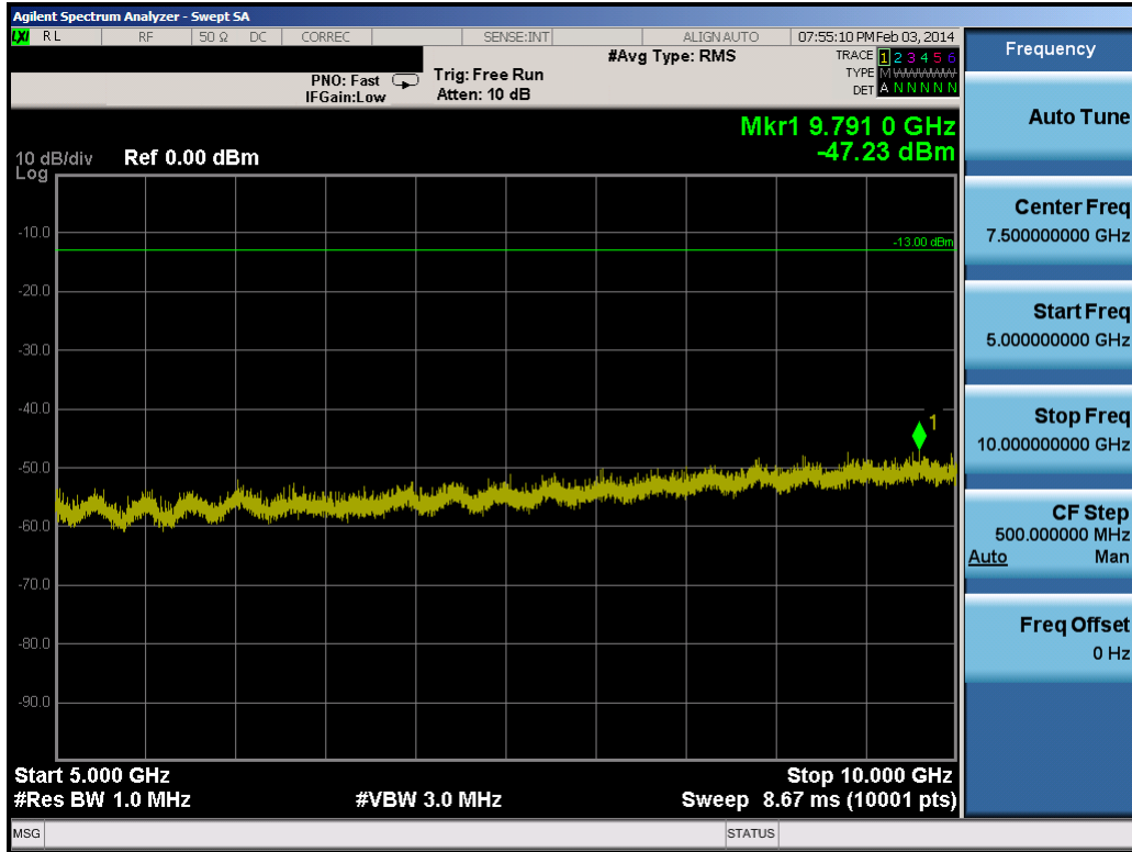
Plot 8-42. Conducted Spurious Plot (10.0MHz QPSK – RB Size 1, RB Offset 0 – Low Channel)
