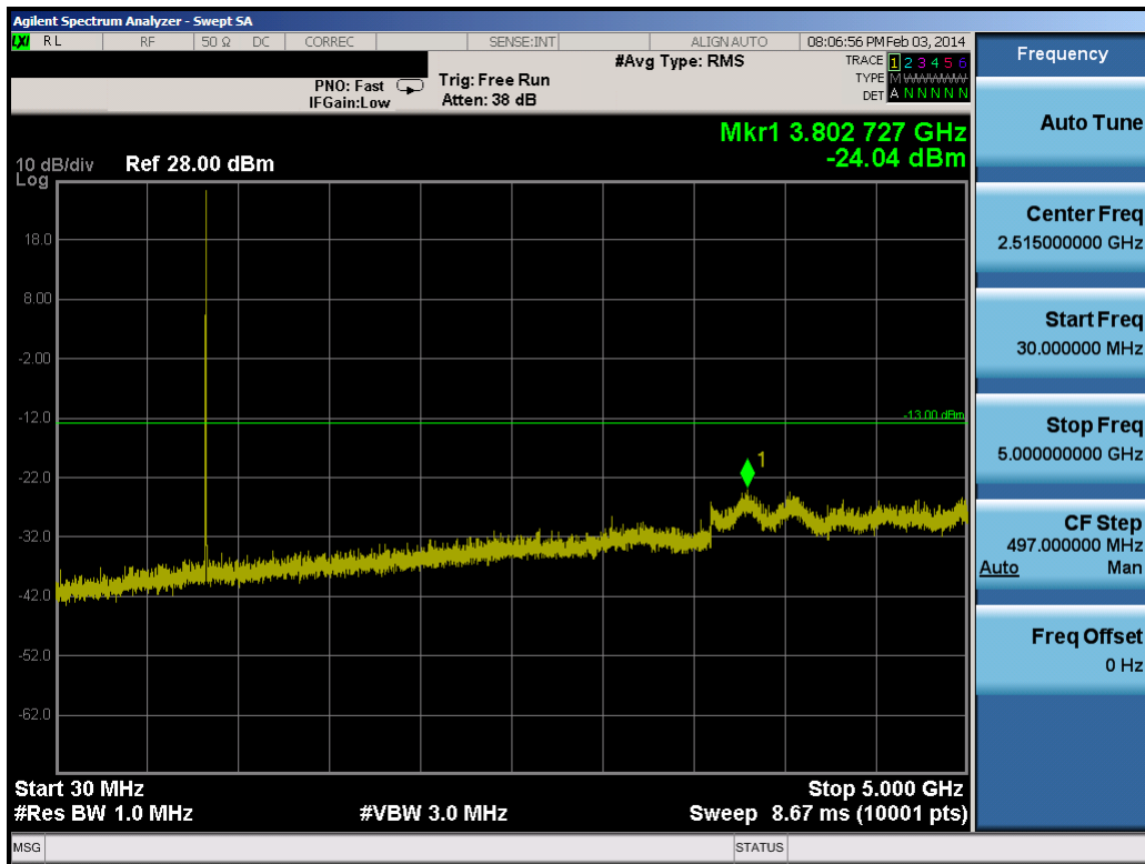
Plot 8-21. Conducted Spurious Plot (3.0MHz QPSK – RB Size 1, RB Offset 0 – High Channel)
