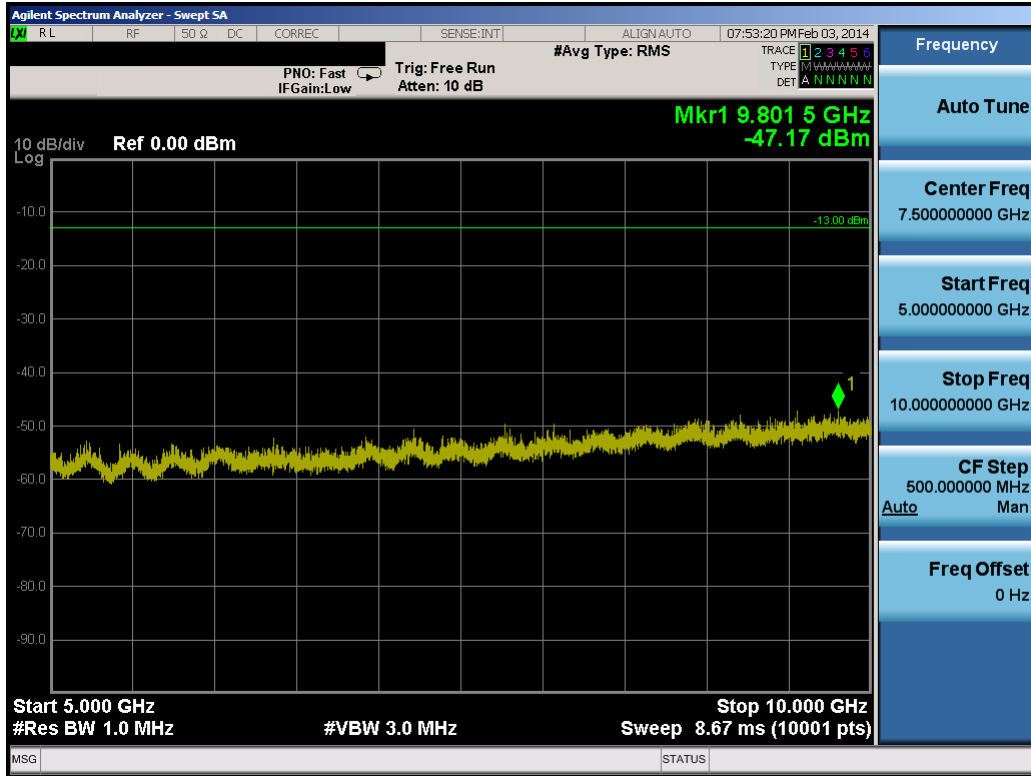
Plot 8-44. Conducted Spurious Plot (10.0MHz QPSK – RB Size 1, RB Offset 0 – Mid Channel)
