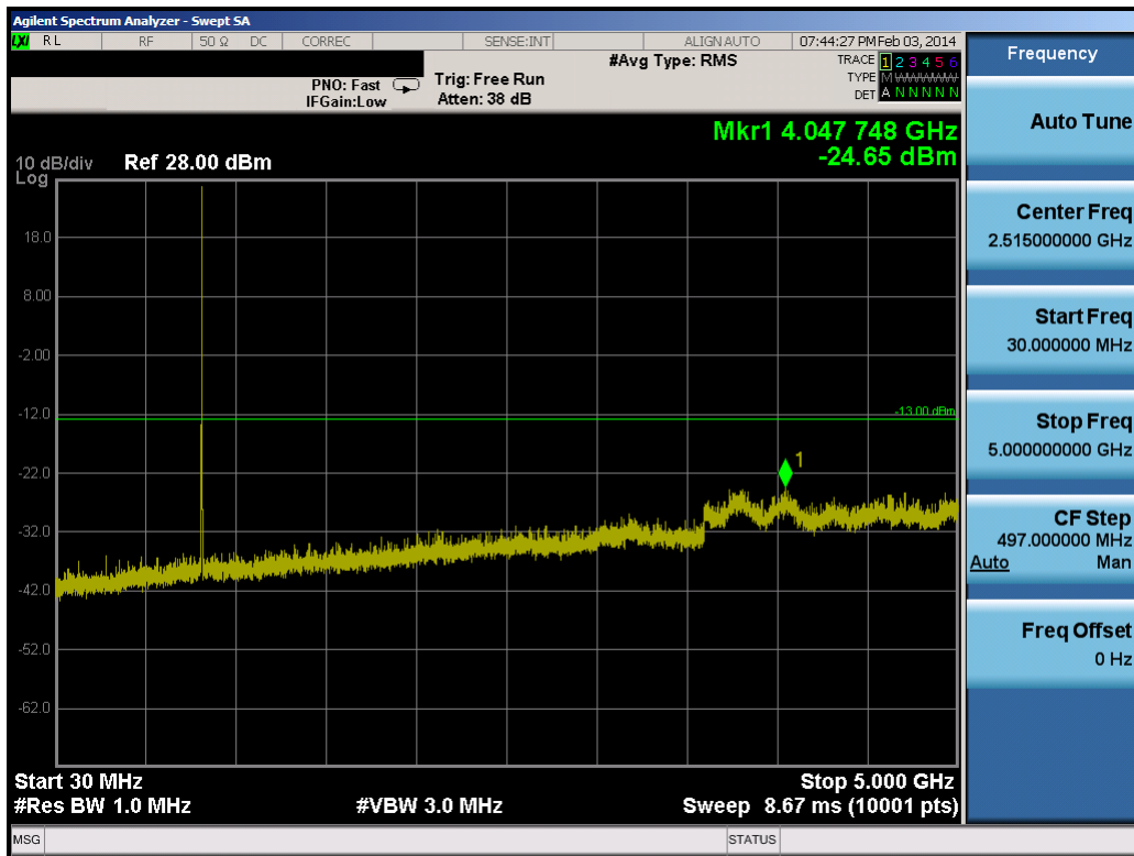
Plot 8-31. Conducted Spurious Plot (5.0MHz QPSK – RB Size 1, RB Offset 0 – Mid Channel)
