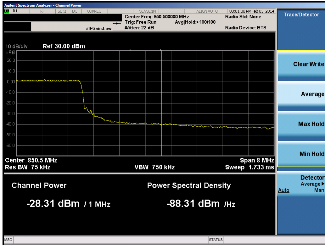
Plot 8-48. Upper Extended Band Edge Plot (10.0MHz QPSK – RB Size 50)
