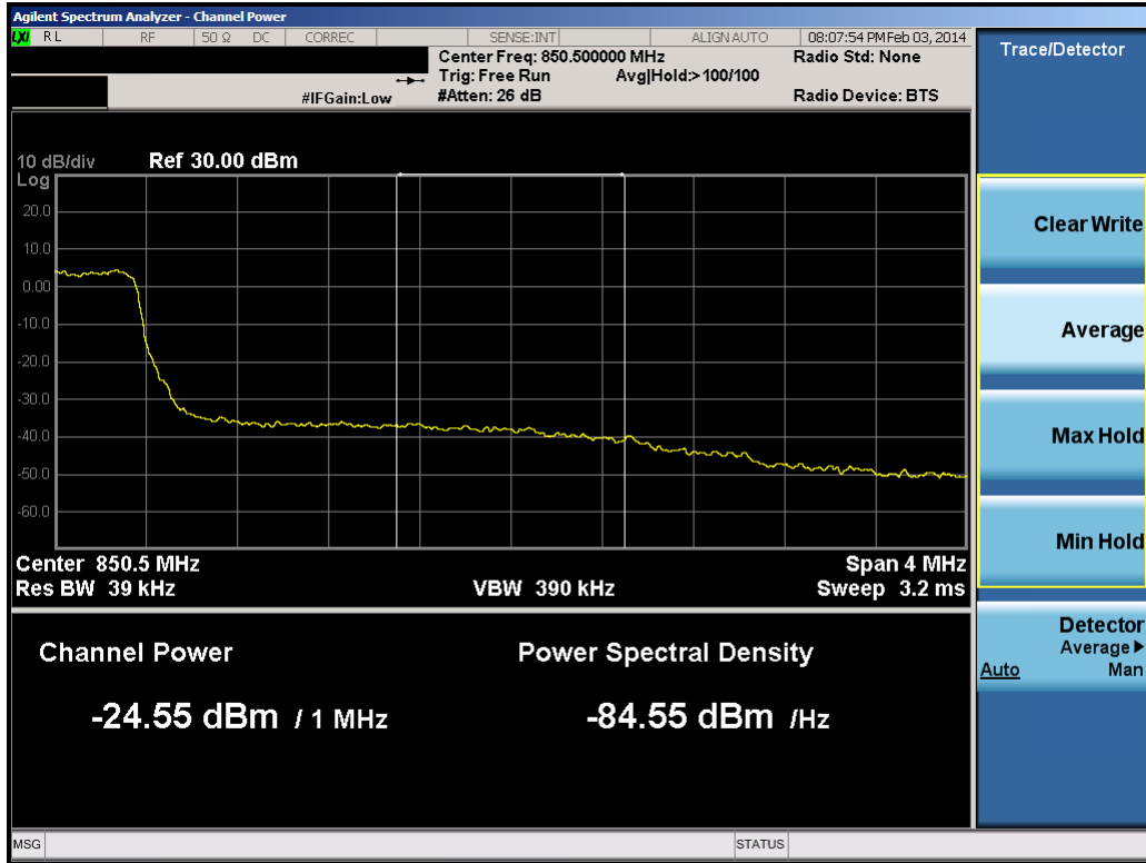
Plot 8-24. Upper Extended Band Edge Plot (3.0MHz QPSK – RB Size 15)
