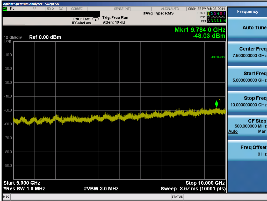
Plot 8-18. Conducted Spurious Plot (3.0MHz QPSK – RB Size 1, RB Offset 0 – Low Channel)
