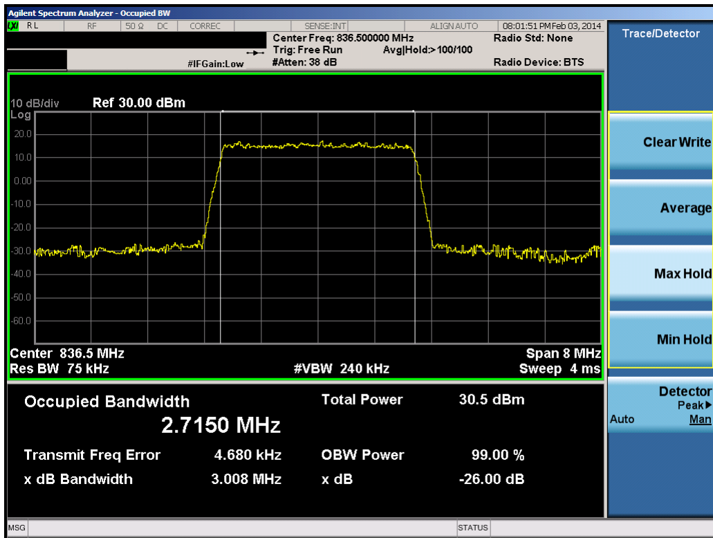
Plot 8-15. Occupied Bandwidth Plot (3.0MHz QPSK – RB Size 15)
