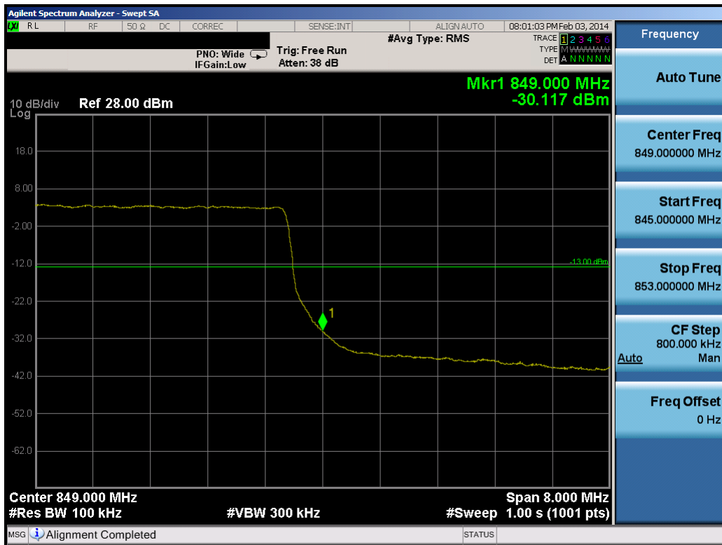
Plot 8-47. Upper Band Edge Plot (10.0MHz QPSK – RB Size 50)
