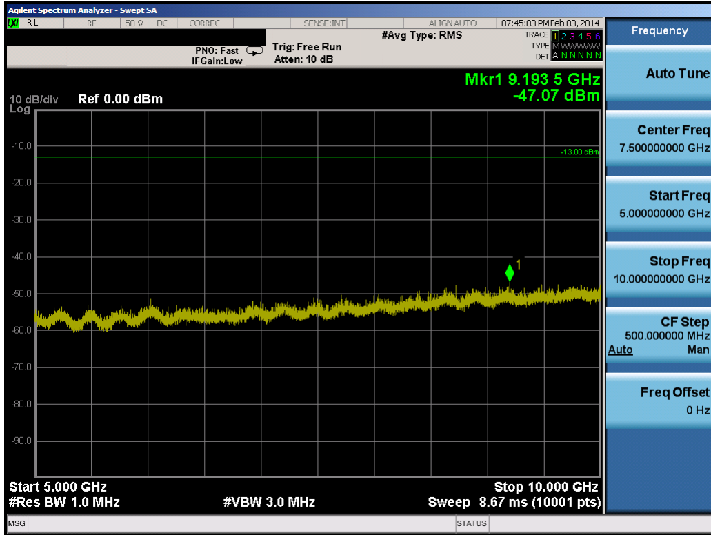
Plot 8-32. Conducted Spurious Plot (5.0MHz QPSK – RB Size 1, RB Offset 0 – Mid Channel)
