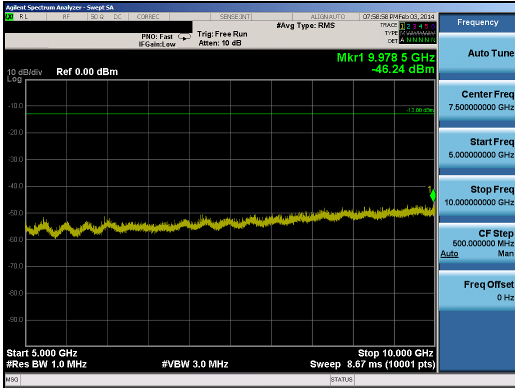
Plot 8-46. Conducted Spurious Plot (10.0MHz QPSK – RB Size 1, RB Offset 0 – High Channel)
