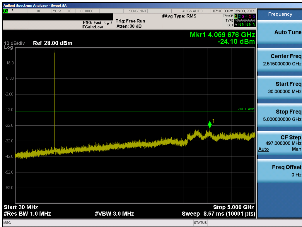
Plot 8-33. Conducted Spurious Plot (5.0MHz QPSK – RB Size 1, RB Offset 0 – High Channel)
