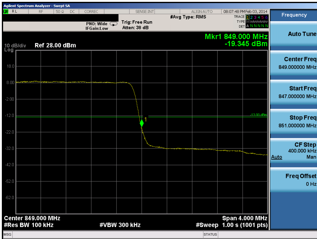
Plot 8-23. Upper Band Edge Plot (3.0MHz QPSK – RB Size 15)
