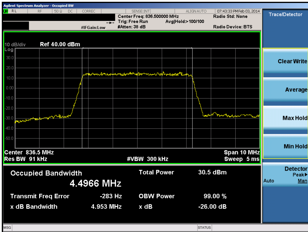
Plot 8-27. Occupied Bandwidth Plot (5.0MHz QPSK – RB Size 25)
