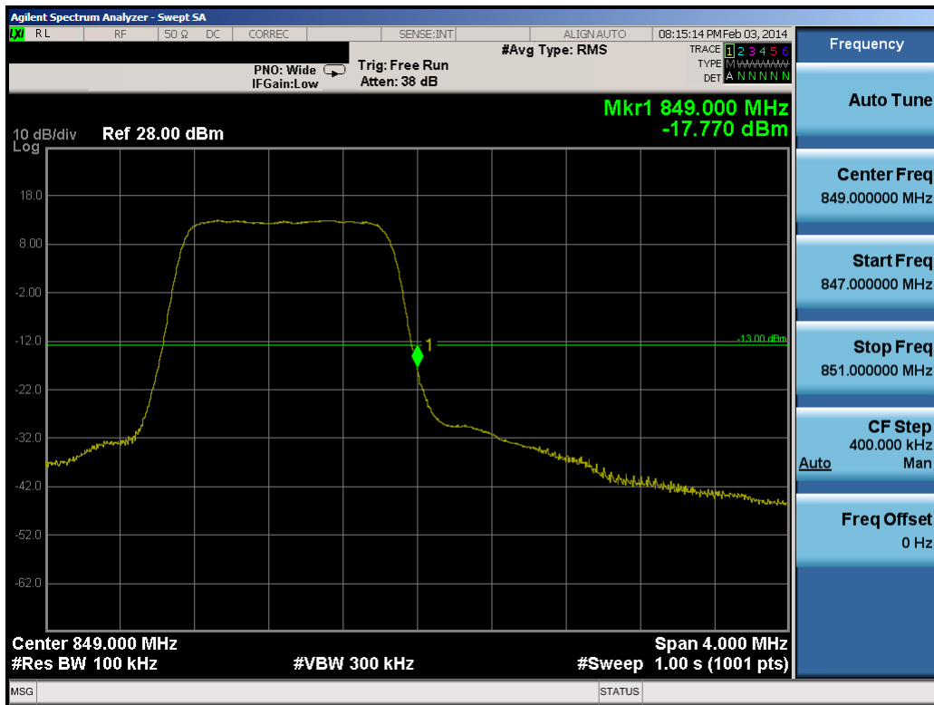
Plot 8-11. Upper Band Edge Plot (1.4MHz QPSK – RB Size 6)
