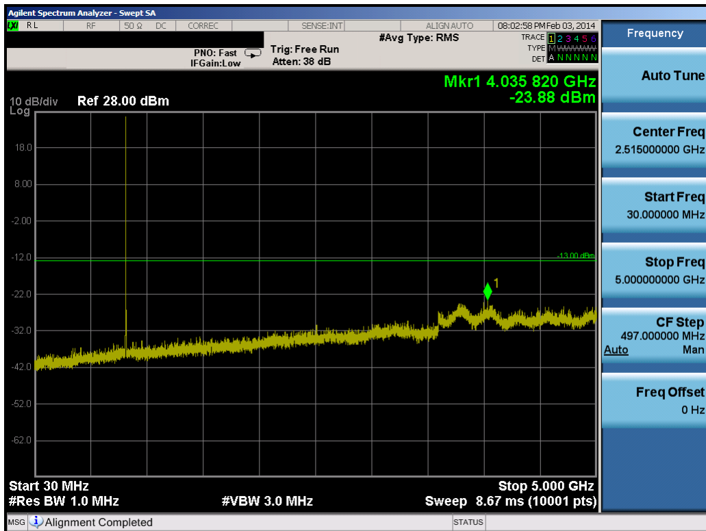
Plot 8-19. Conducted Spurious Plot (3.0MHz QPSK – RB Size 1, RB Offset 0 – Mid Channel)
