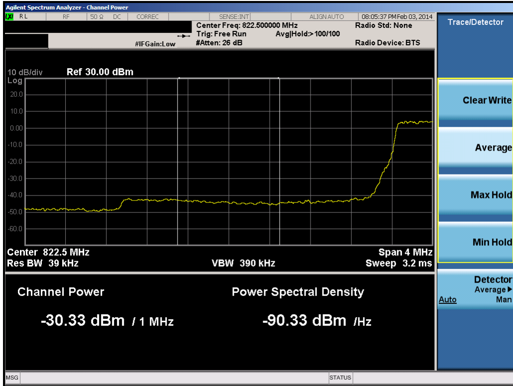
Plot 8-14. Lower Extended Band Edge Plot (3.0MHz QPSK – RB Size 15)
