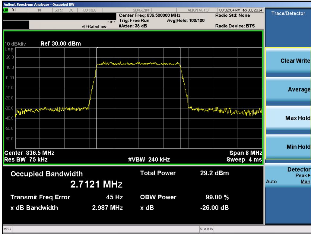
Plot 8-16. Occupied Bandwidth Plot (3.0MHz 16-QAM – RB Size 15)
