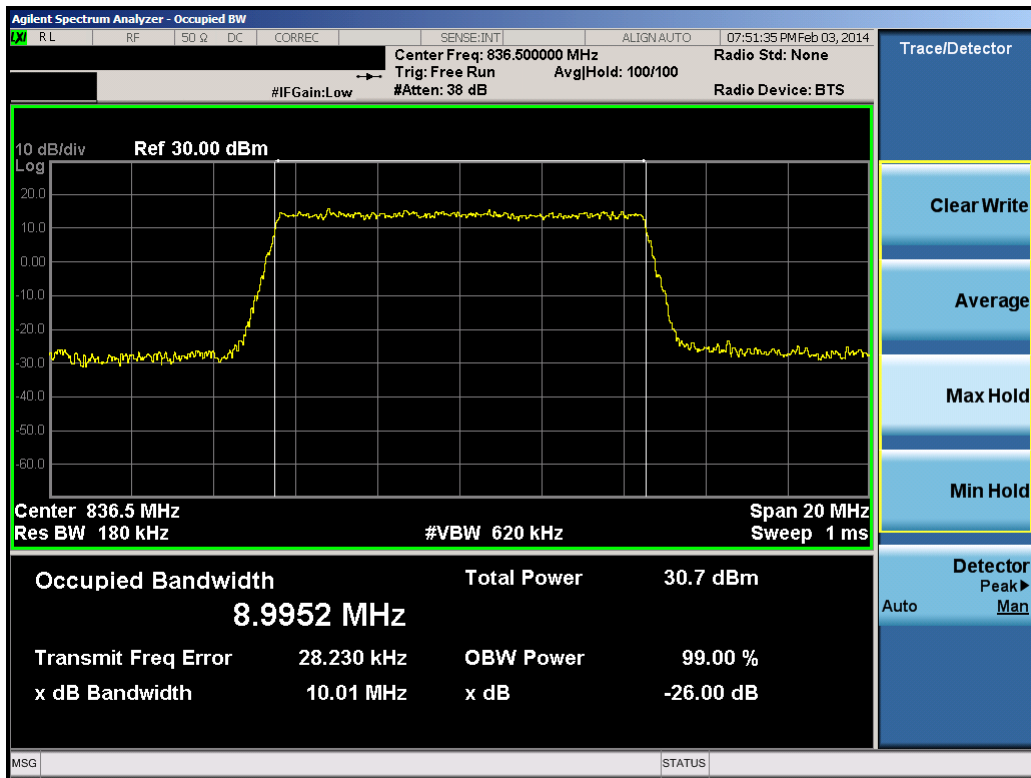
Plot 8-39. Occupied Bandwidth Plot (10.0MHz QPSK – RB Size 50)
