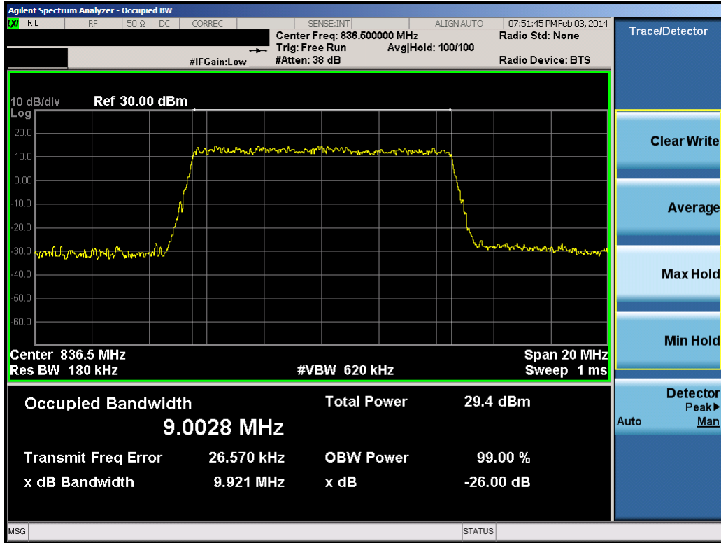
Plot 8-40. Occupied Bandwidth Plot (10.0MHz 16-QAM – RB Size 50)
