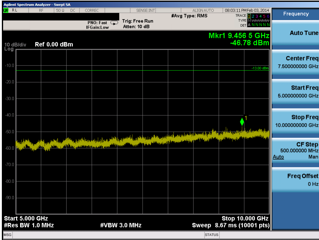
Plot 8-20. Conducted Spurious Plot (3.0MHz QPSK – RB Size 1, RB Offset 0 – Mid Channel)
