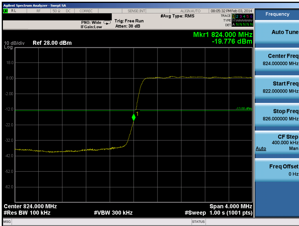
Plot 8-13. Lower Band Edge Plot (3.0MHz QPSK – RB Size 15)
