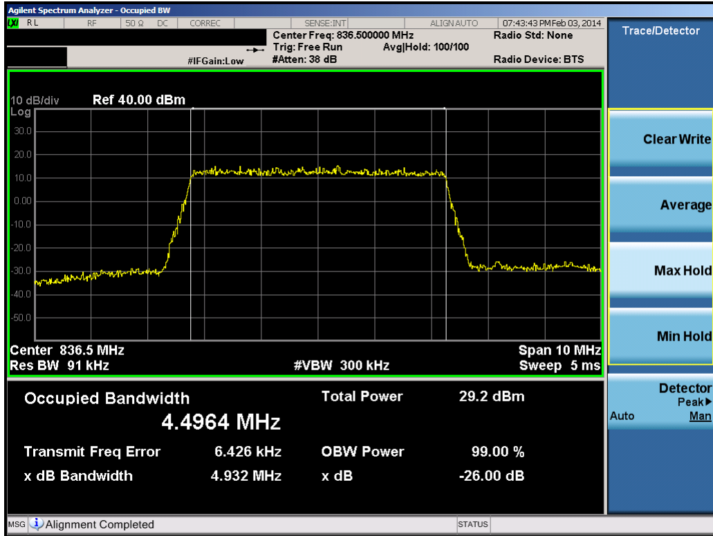
Plot 8-28. Occupied Bandwidth Plot (5.0MHz 16-QAM – RB Size 25)
