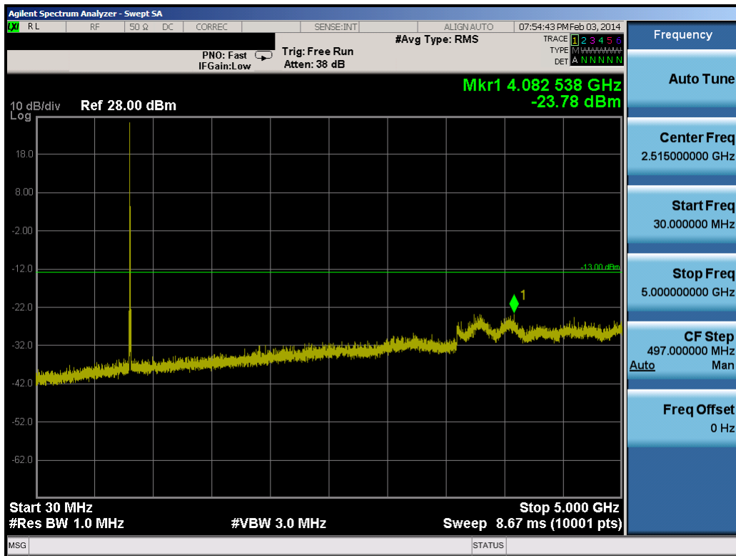
Plot 8-41. Conducted Spurious Plot (10.0MHz QPSK – RB Size 1, RB Offset 0– Low Channel)
