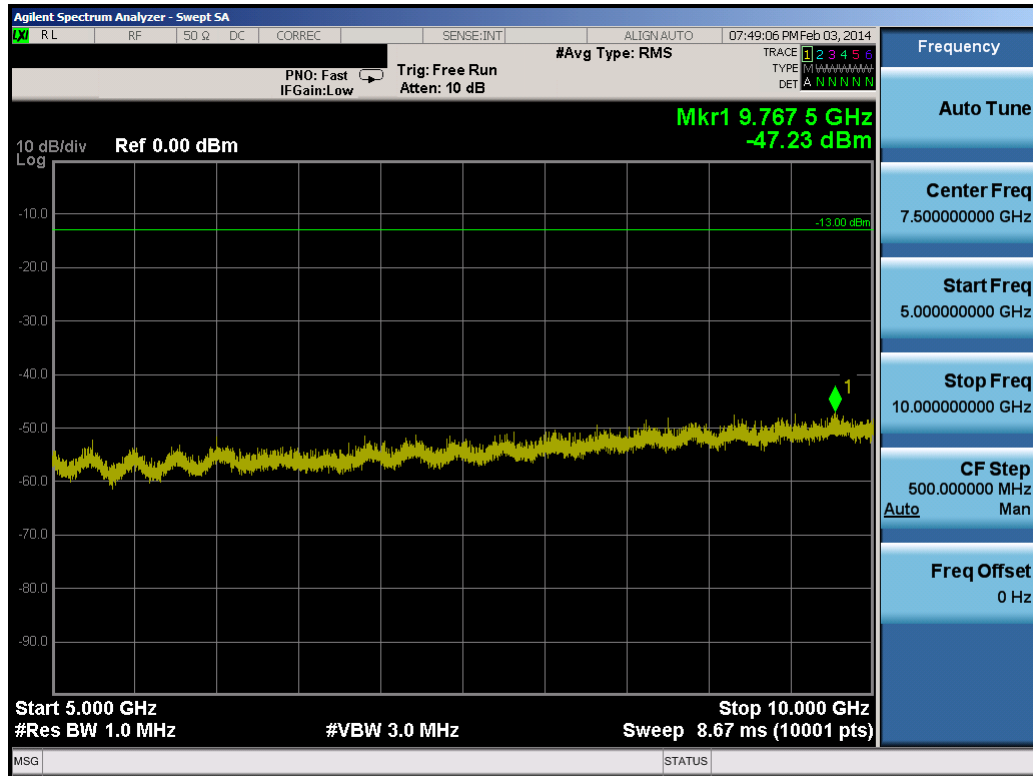
Plot 8-34. Conducted Spurious Plot (5.0MHz QPSK – RB Size 1, RB Offset 0 – High Channel)
