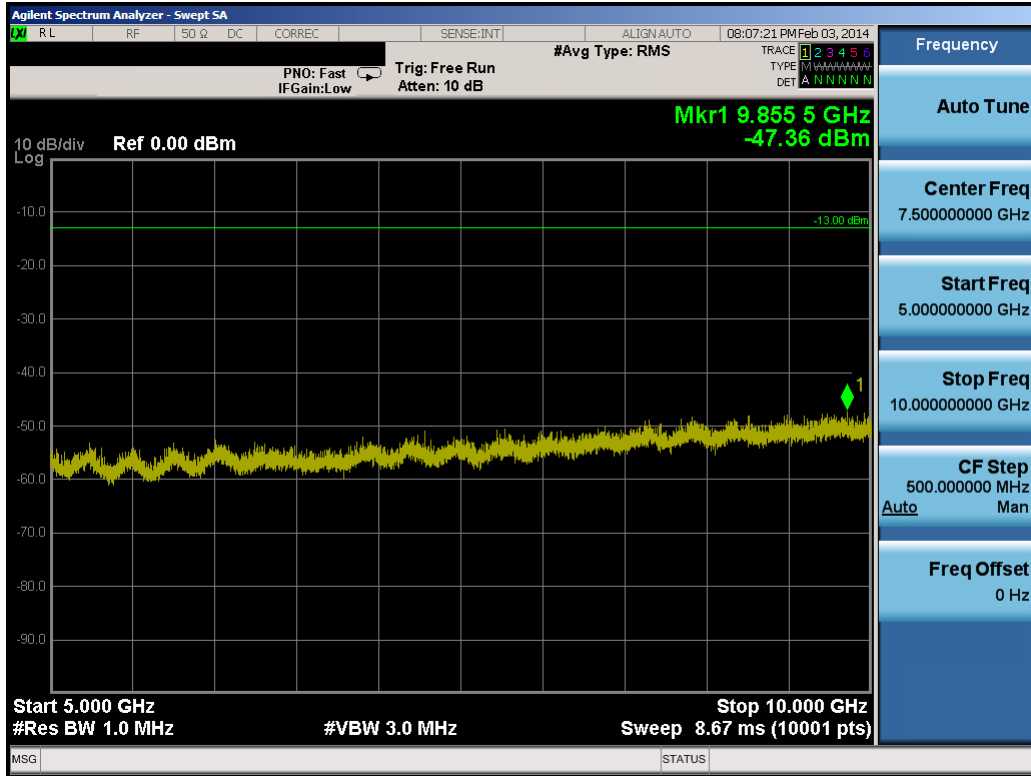
Plot 8-22. Conducted Spurious Plot (3.0MHz QPSK – RB Size 1, RB Offset 0 – High Channel)
