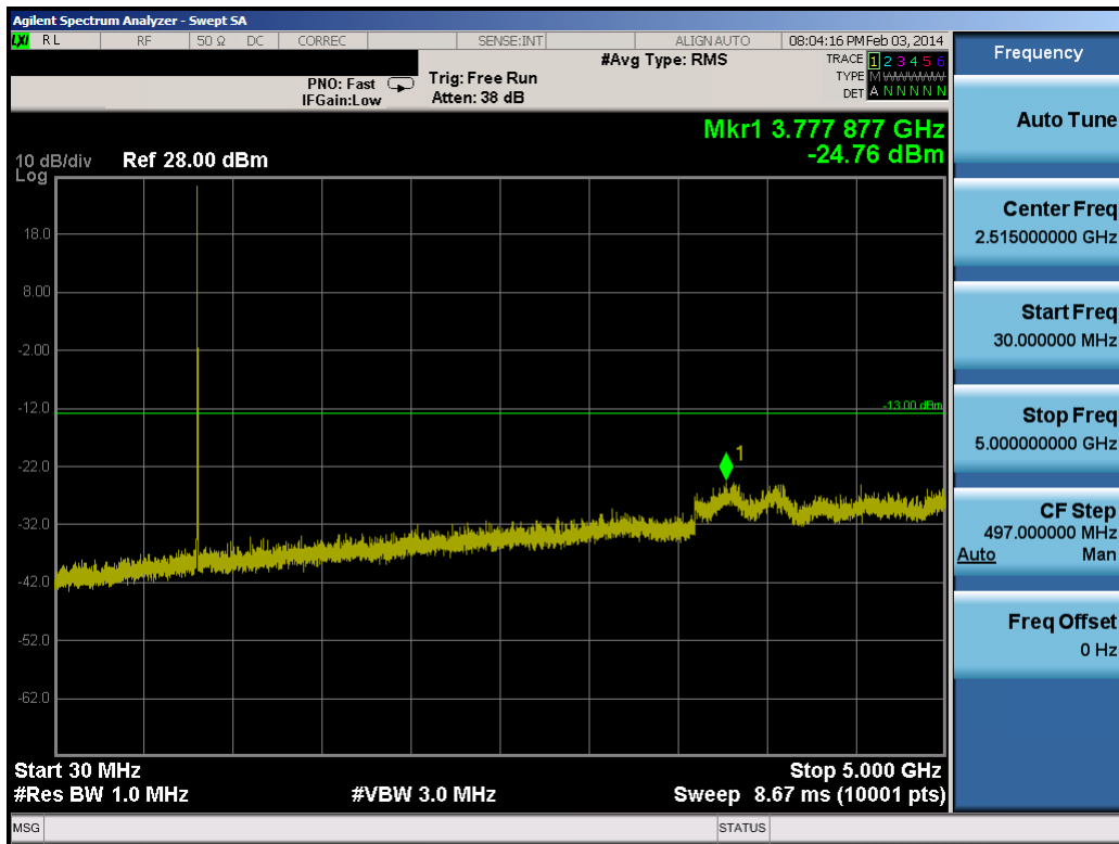
Plot 8-17. Conducted Spurious Plot (3.0MHz QPSK – RB Size 1, RB Offset 0 – Low Channel)
