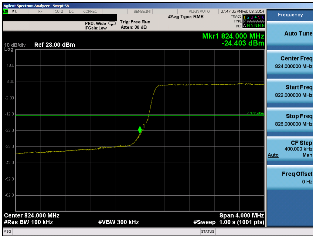
Plot 8-25. Lower Band Edge Plot (5.0MHz QPSK – RB Size 25)
