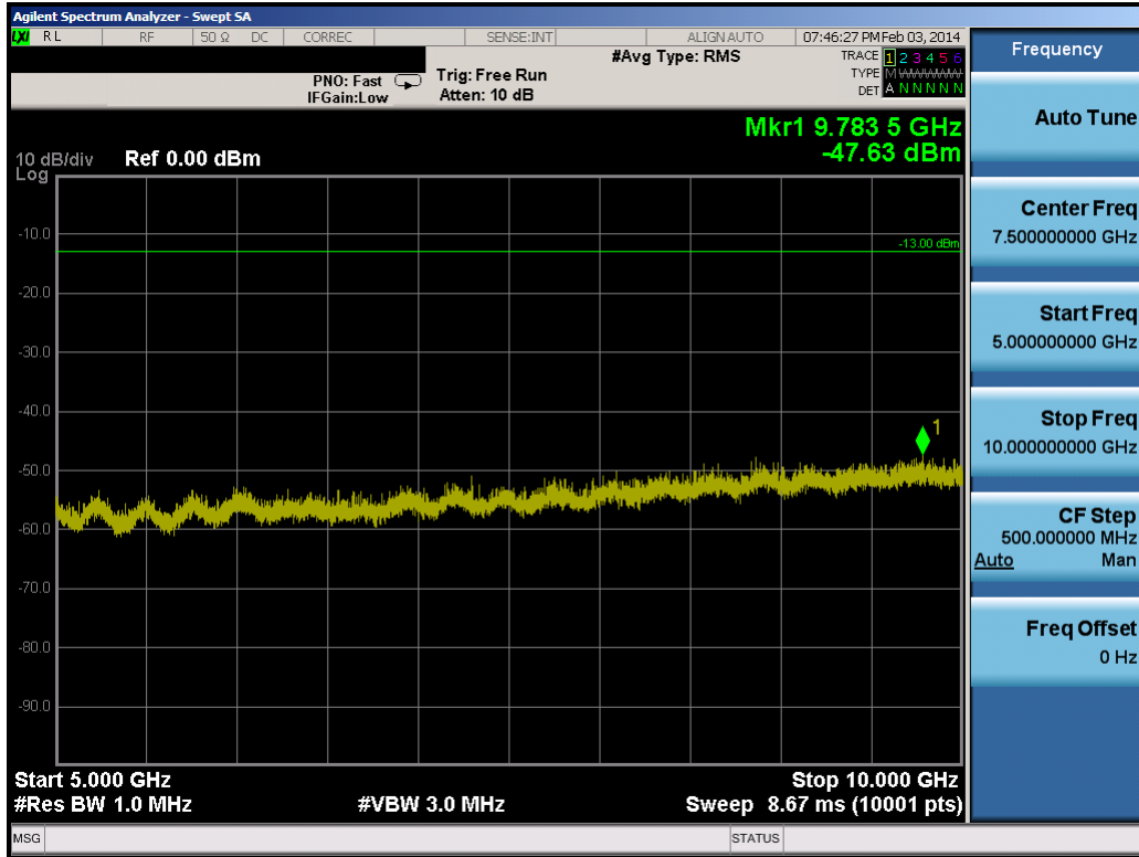
Plot 8-30. Conducted Spurious Plot (5.0MHz QPSK – RB Size 1, RB Offset 0 – Low Channel)
