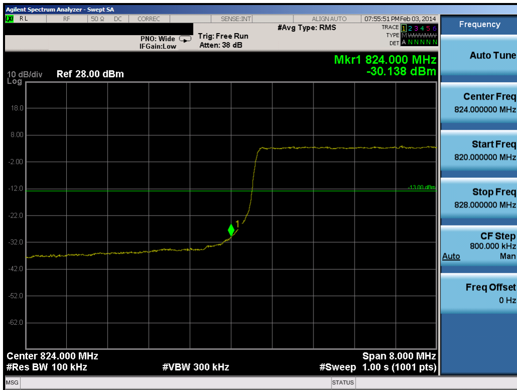
Plot 8-37. Lower Band Edge Plot (10.0MHz QPSK – RB Size 50)
