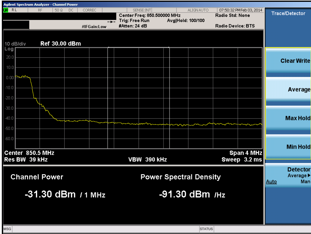
Plot 8-36. Upper Extended Band Edge Plot (5.0MHz QPSK – RB Size 25)
