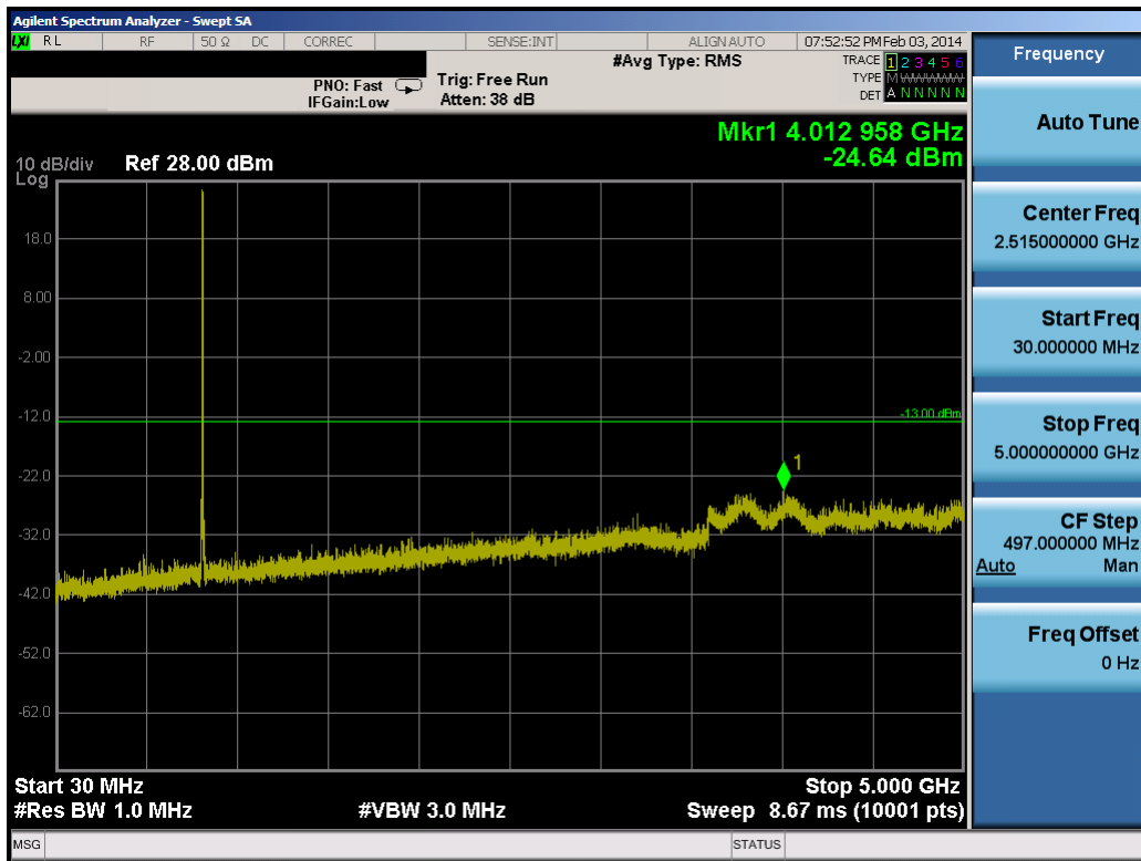
Plot 8-43. Conducted Spurious Plot (10.0MHz QPSK – RB Size 1, RB Offset 0 – Mid Channel)
