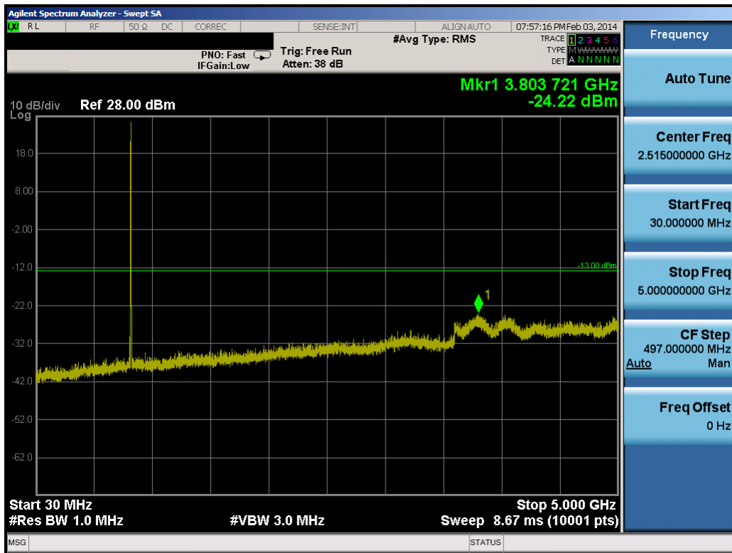
Plot 8-45. Conducted Spurious Plot (10.0MHz QPSK – RB Size 1, RB Offset 0 – High Channel)
