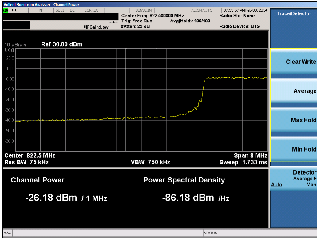
Plot 8-38. Lower Extended Band Edge Plot (10.0MHz QPSK – RB Size 50)
