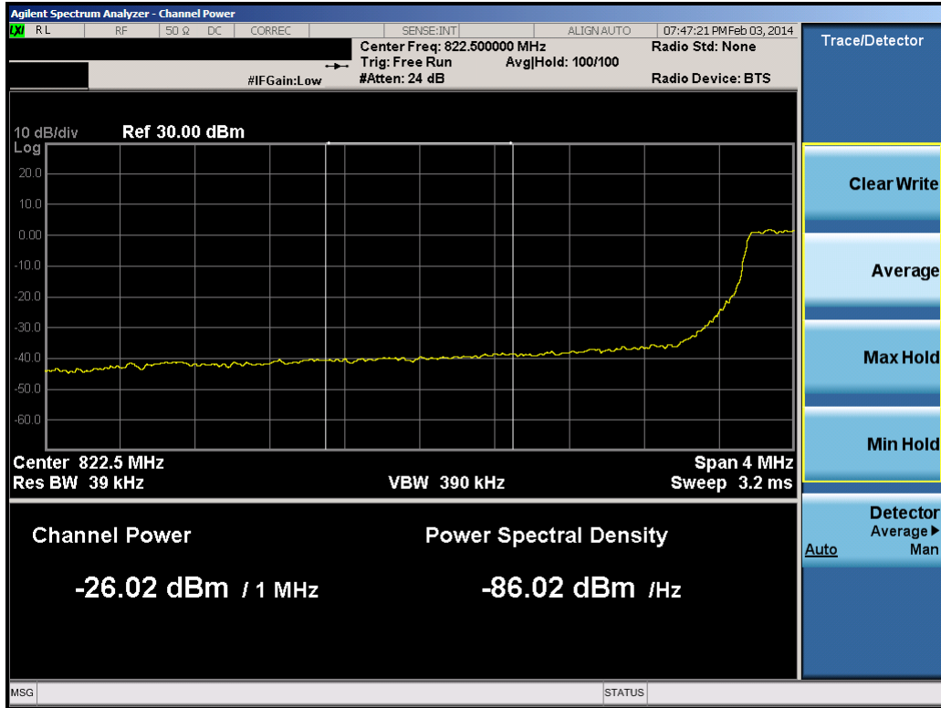
Plot 8-26. Lower Extended Band Edge Plot (5.0MHz QPSK – RB Size 25)
