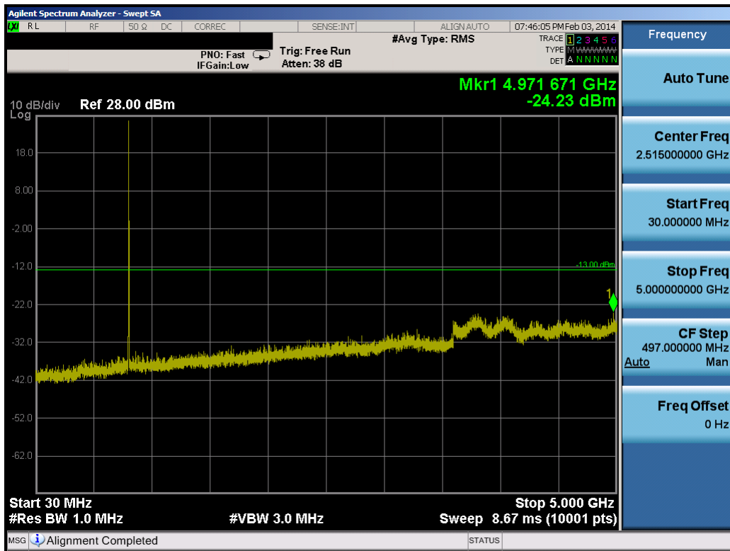
Plot 8-29. Conducted Spurious Plot (5.0MHz QPSK – RB Size 1, RB Offset 0 – Low Channel)
