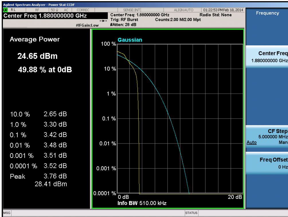
Plot 6-68. Peak-Average Ratio Plot (EDGE1900 Mode, Master – Ch. 661)
