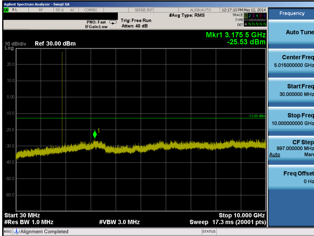
Plot 6-37. Conducted Spurious Plot (PCS GSM Mode, Slave – Ch. 661)
