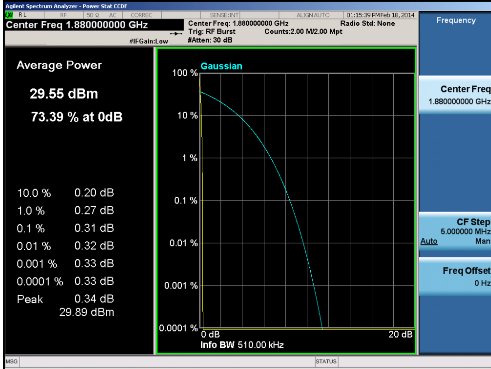
Plot 6-67. Peak-Average Ratio Plot (PCS GSM Mode, Master – Ch. 661)
