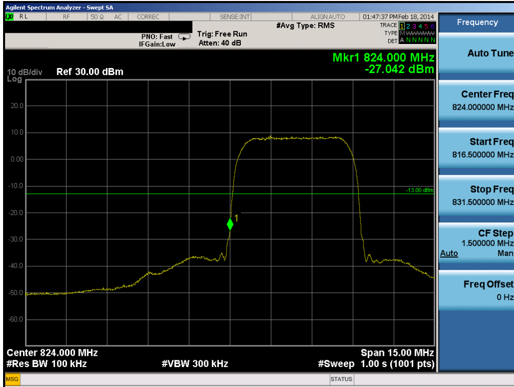
Plot 6-61. Band Edge Plot (Cellular WCDMA Mode – Ch. 4132)
