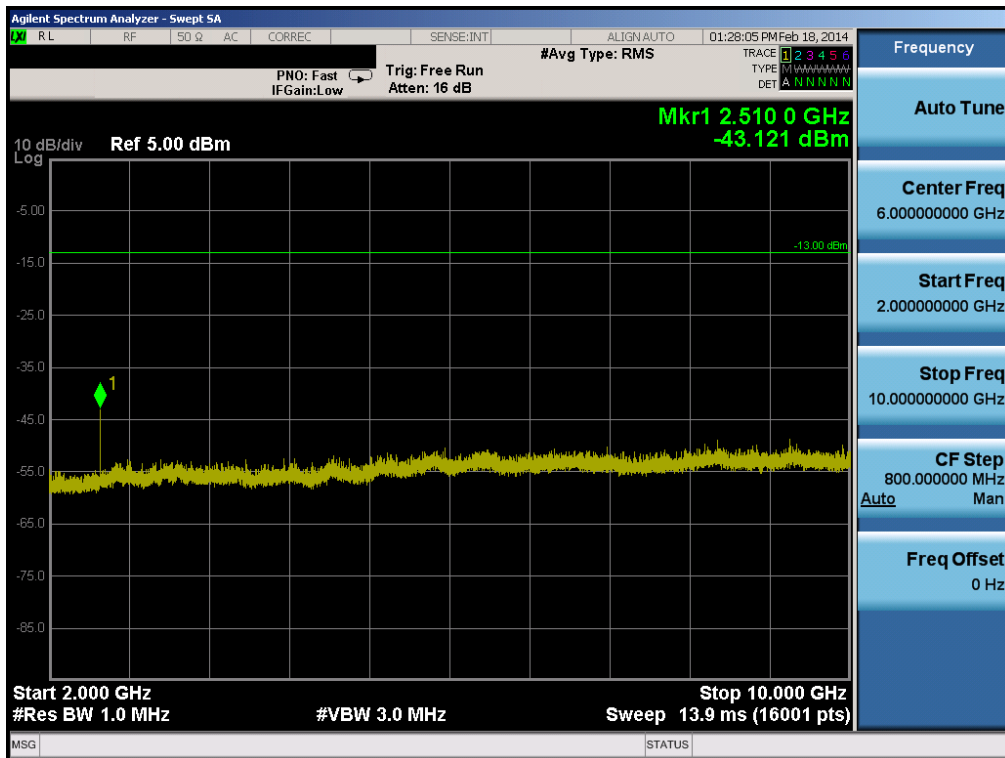
Plot 6-16. Conducted Spurious Plot (Cellular GSM Mode, Master – Ch. 190)
