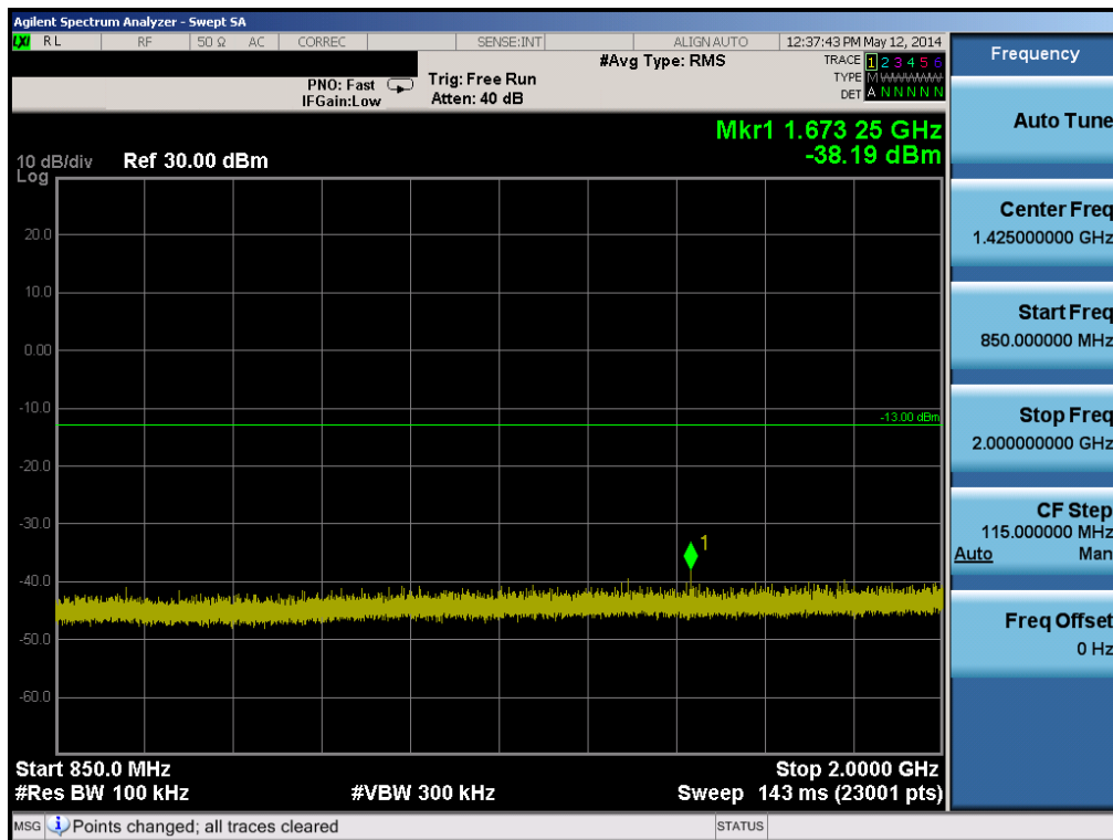
Plot 6-30. Conducted Spurious Plot (Cellular GSM Mode, Slave – Ch. 190)
