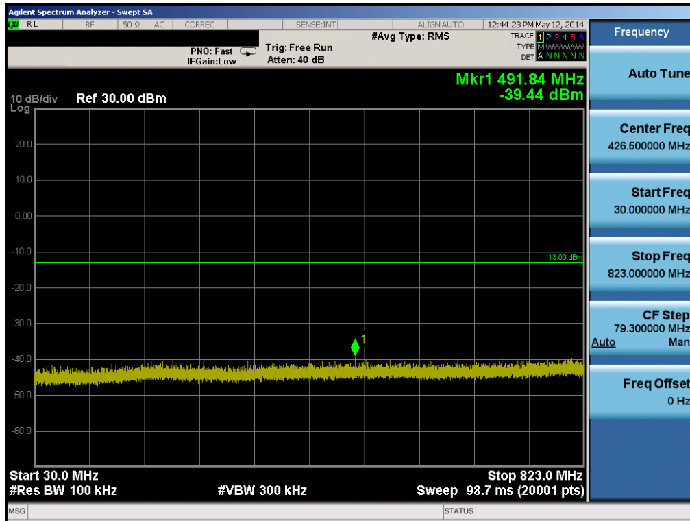
Plot 6-32. Conducted Spurious Plot (Cellular GSM Mode, Slave – Ch. 251)
