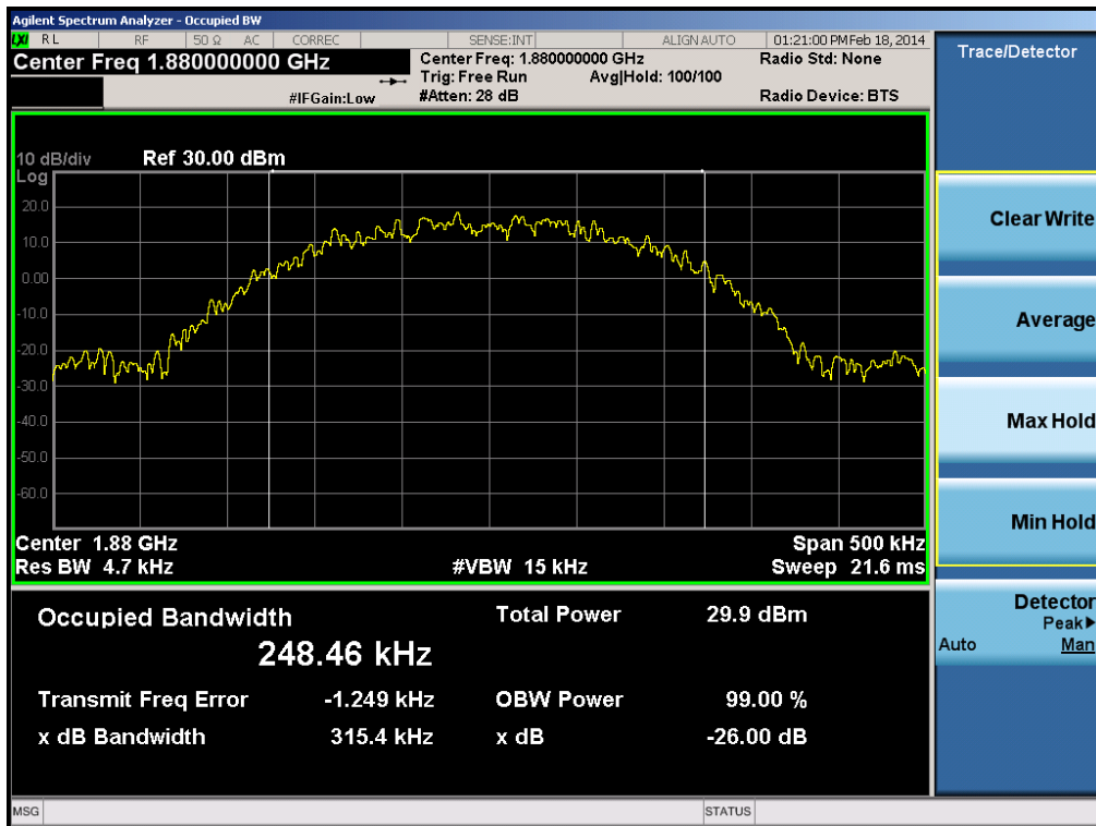
Plot 6-4. Occupied Bandwidth Plot (EDGE1900 Mode, Master – Ch. 661)
