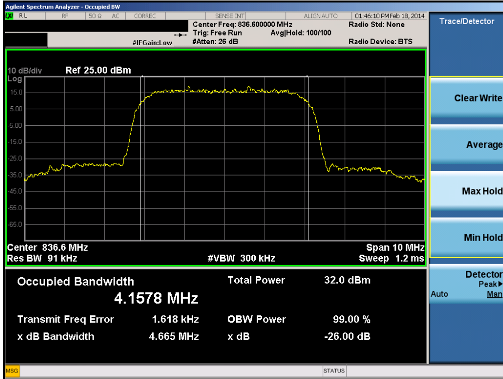
Plot 6-9. Occupied Bandwidth Plot (Cellular WCDMA Mode – Ch. 4183)
