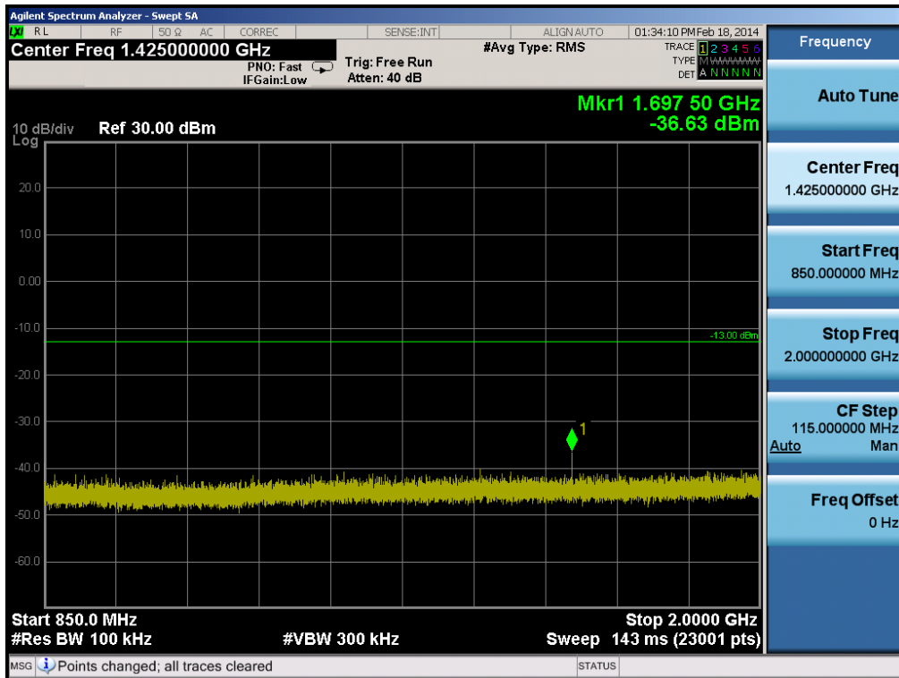
Plot 6-18. Conducted Spurious Plot (Cellular GSM Mode, Master – Ch. 251)
