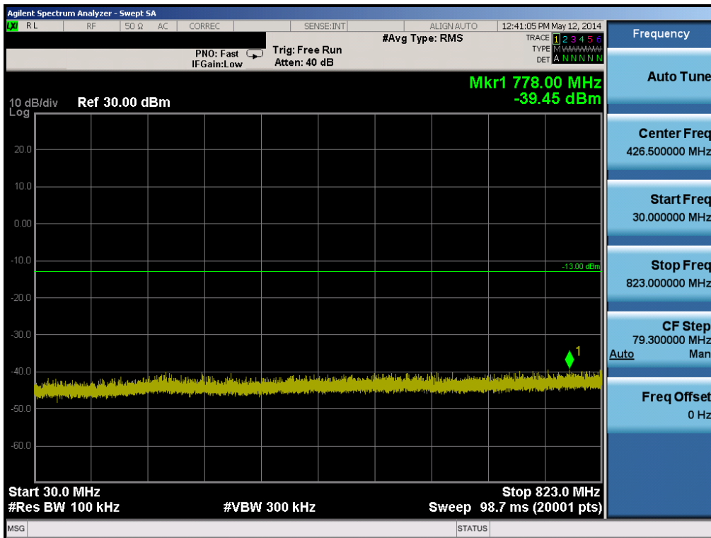
Plot 6-26. Conducted Spurious Plot (Cellular GSM Mode, Slave – Ch. 128)
