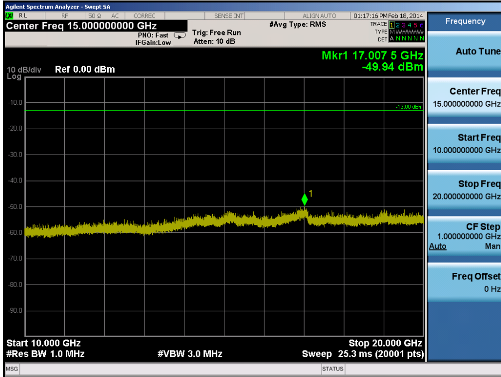
Plot 6-21. Conducted Spurious Plot (PCS GSM Mode, Master – Ch. 512)
