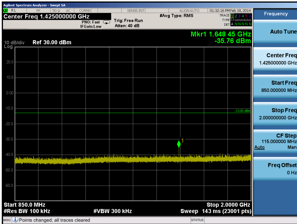
Plot 6-12. Conducted Spurious Plot (Cellular GSM Mode, Master – Ch. 128)
