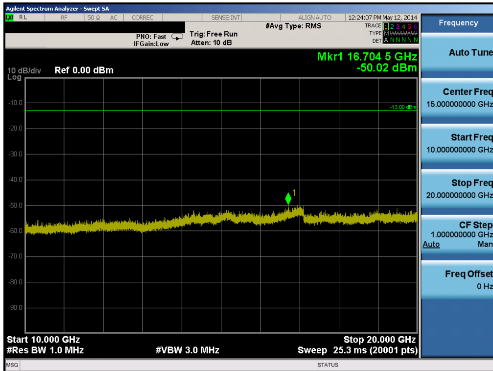
Plot 6-40. Conducted Spurious Plot (PCS GSM Mode, Slave – Ch. 810)
