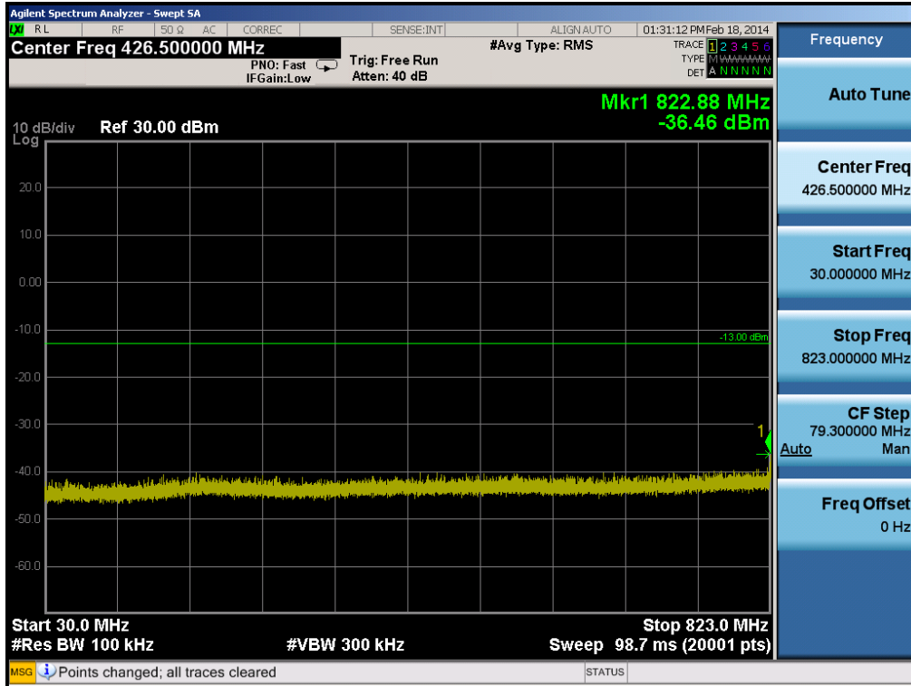
Plot 6-11. Conducted Spurious Plot (Cellular GSM Mode, Master – Ch. 128)
