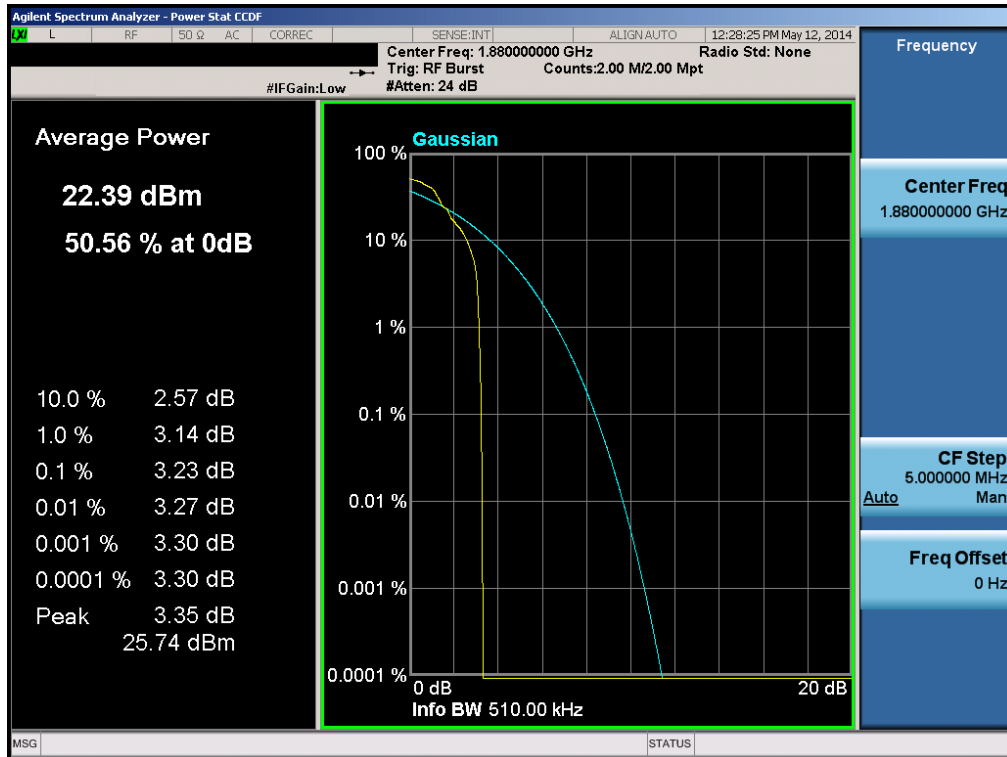
Plot 6-70. Peak-Average Ratio Plot (EDGE1900 Mode, Slave – Ch. 661)
