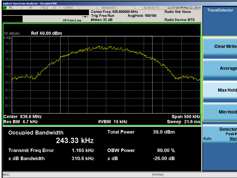
Plot 6-5. Occupied Bandwidth Plot (Cellular GSM Mode, Slave – Ch. 190)
