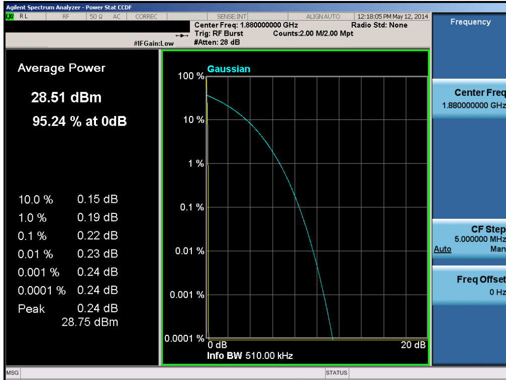
Plot 6-69. Peak-Average Ratio Plot (PCS GSM Mode, Slave – Ch. 661)
