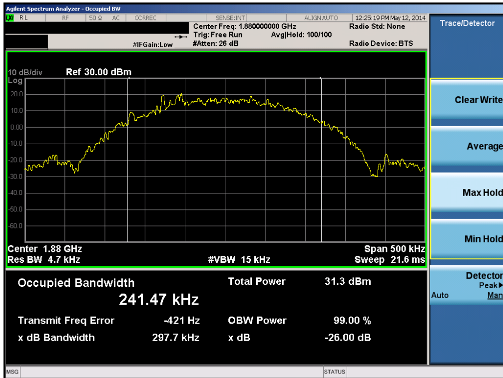
Plot 6-8. Occupied Bandwidth Plot (EDGE1900 Mode, Slave – Ch. 661)
