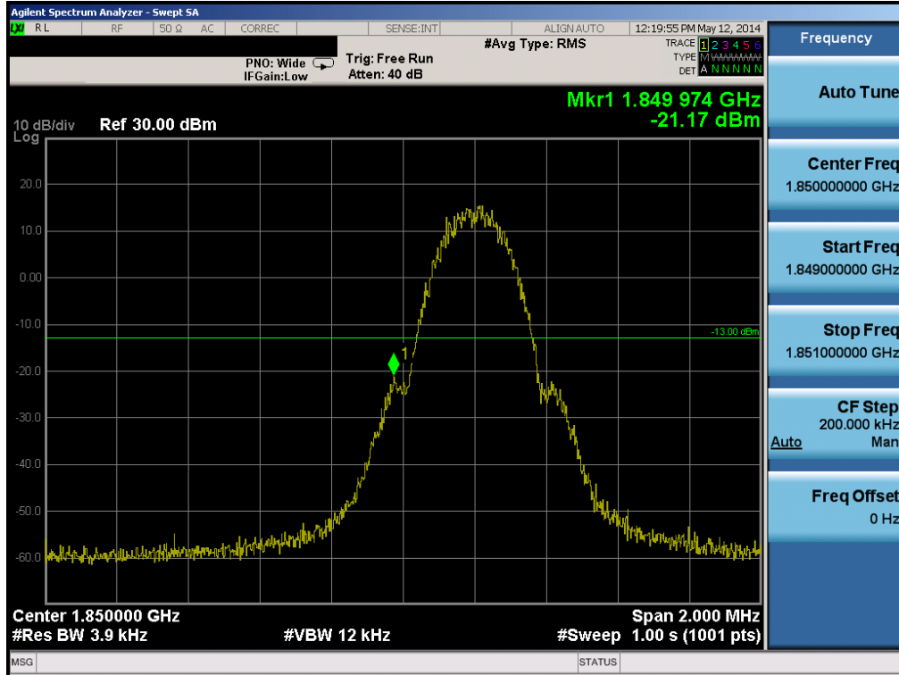
Plot 6-59. Band Edge Plot (PCS GSM Mode, Slave – Ch. 512)
