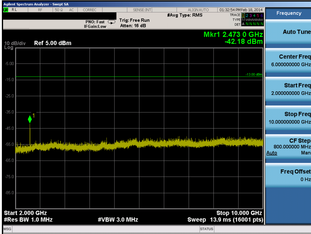
Plot 6-13. Conducted Spurious Plot (Cellular GSM Mode, Master – Ch. 128)
