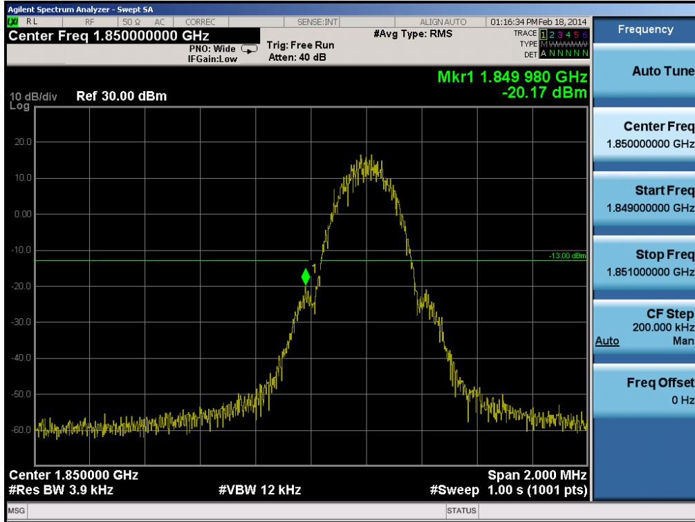
Plot 6-55. Band Edge Plot (PCS GSM Mode, Master – Ch. 512)
