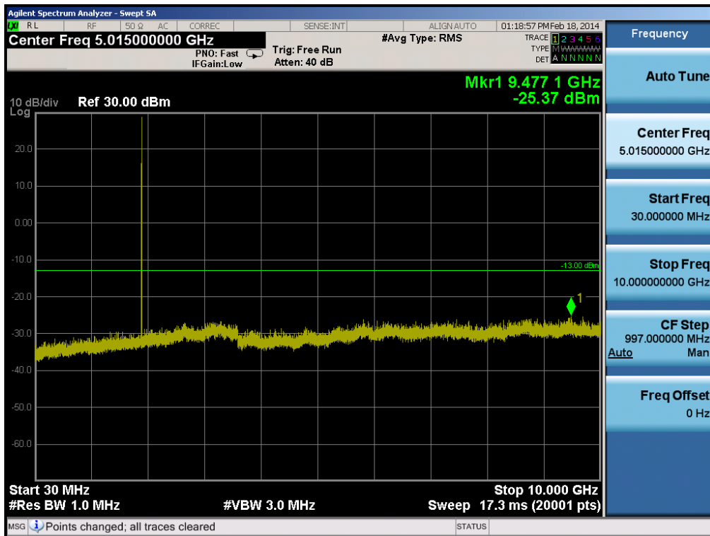
Plot 6-24. Conducted Spurious Plot (PCS GSM Mode, Master – Ch. 810)
