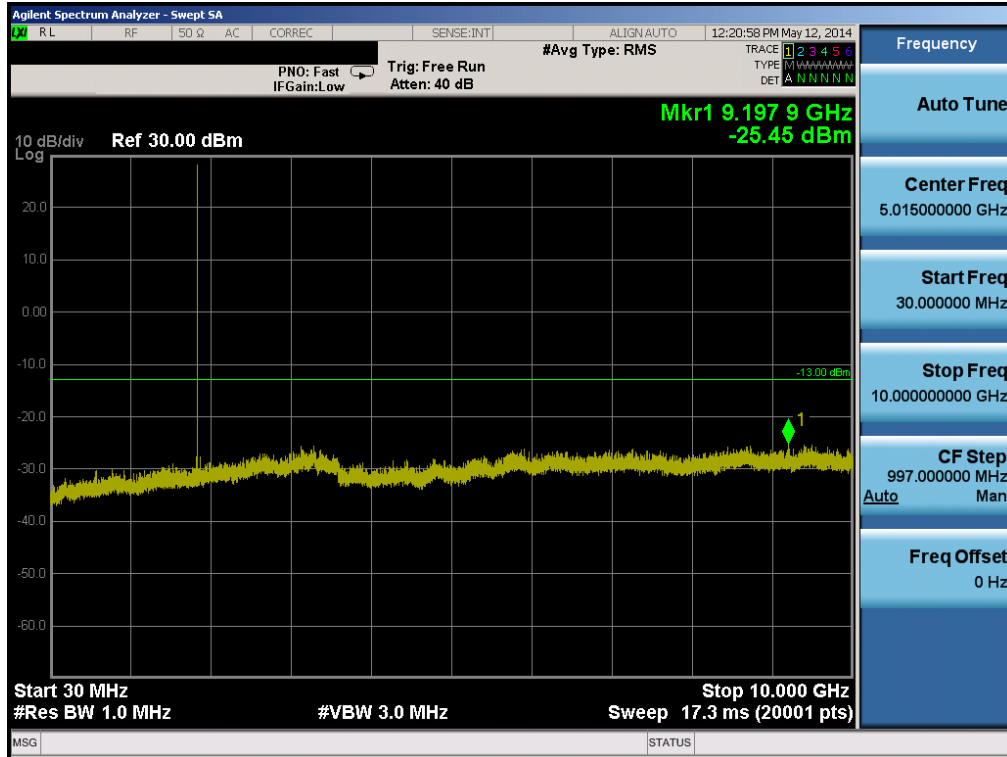
Plot 6-35. Conducted Spurious Plot (PCS GSM Mode, Slave – Ch. 512)
