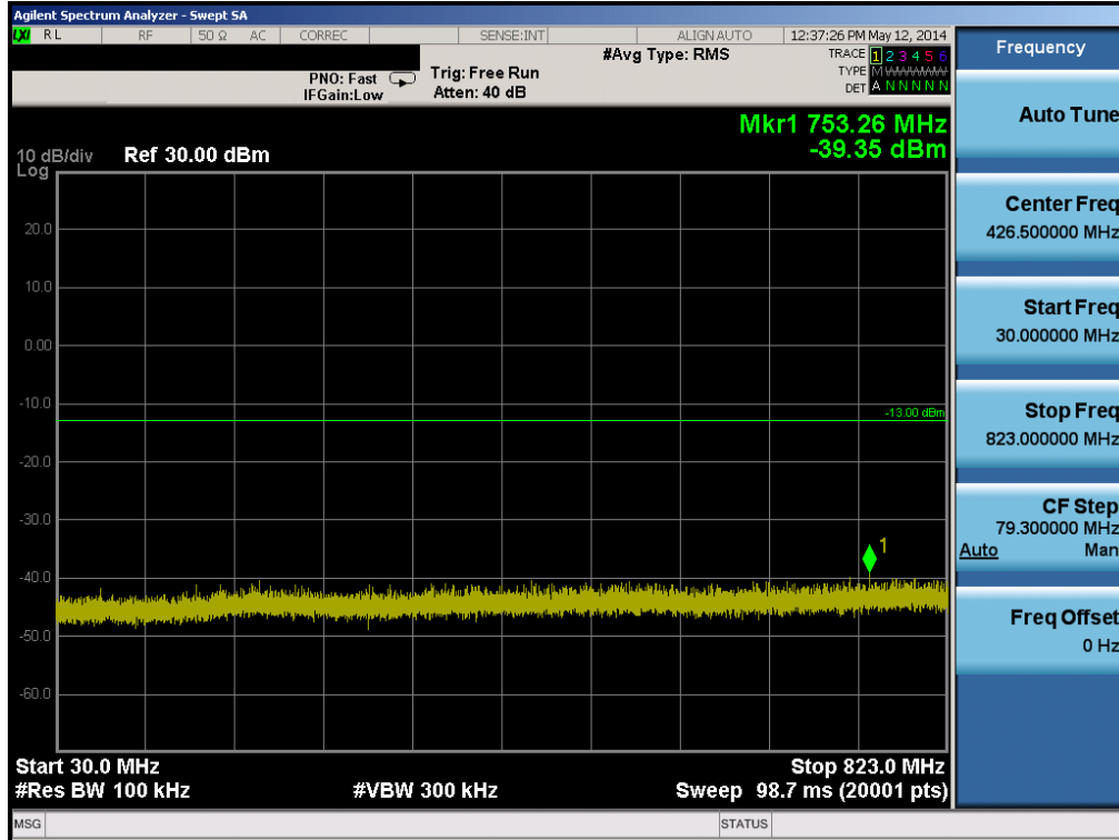
Plot 6-29. Conducted Spurious Plot (Cellular GSM Mode, Slave – Ch. 190)
