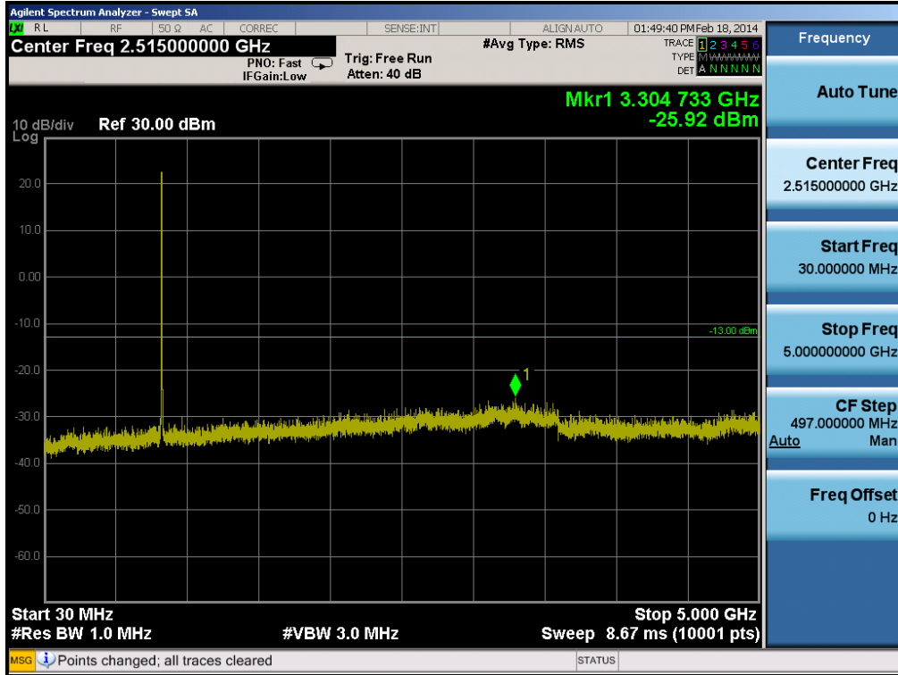
Plot 6-45. Conducted Spurious Plot (Cellular WCDMA Mode – Ch. 4233)
