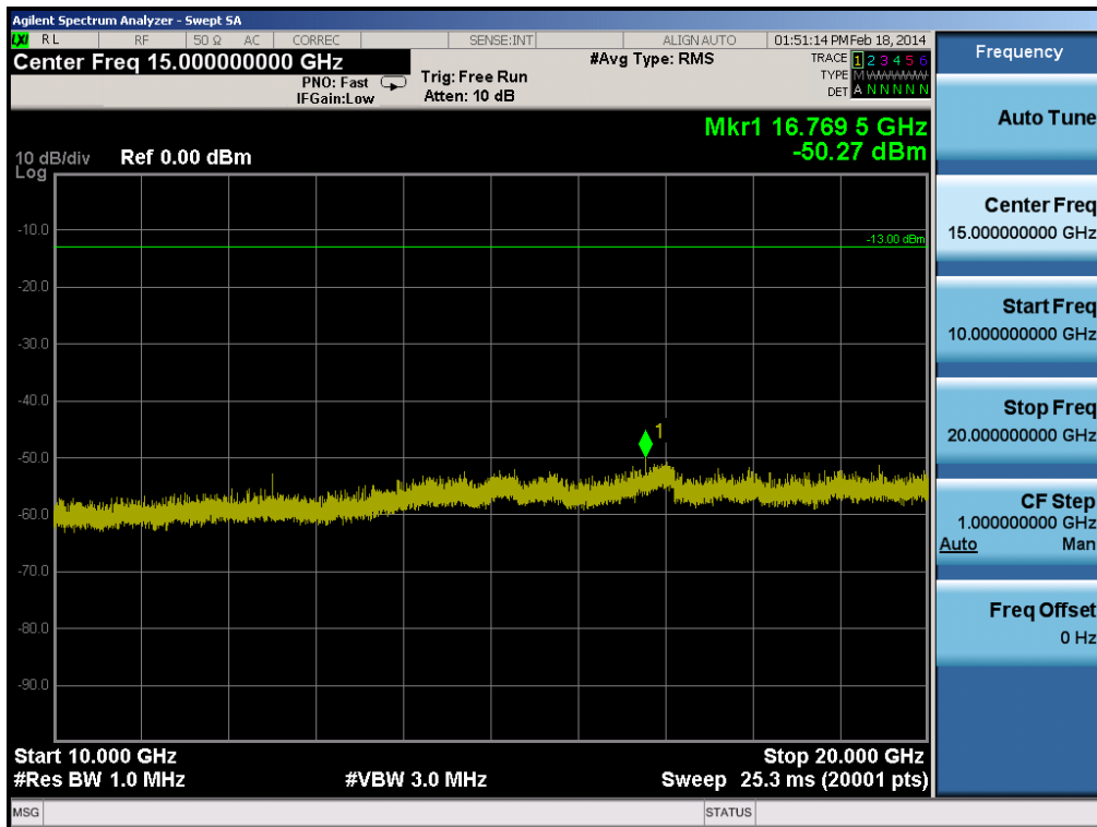
Plot 6-50. Conducted Spurious Plot (PCS WCDMA Mode – Ch. 9400)
