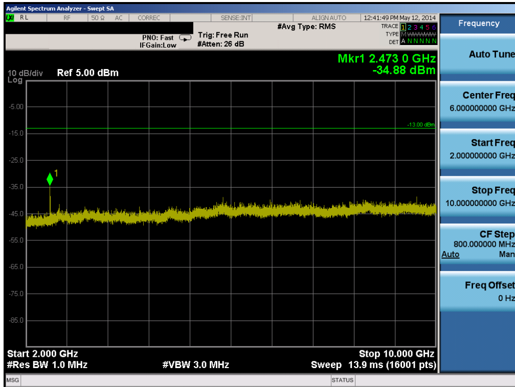
Plot 6-28. Conducted Spurious Plot (Cellular GSM Mode, Slave – Ch. 128)
