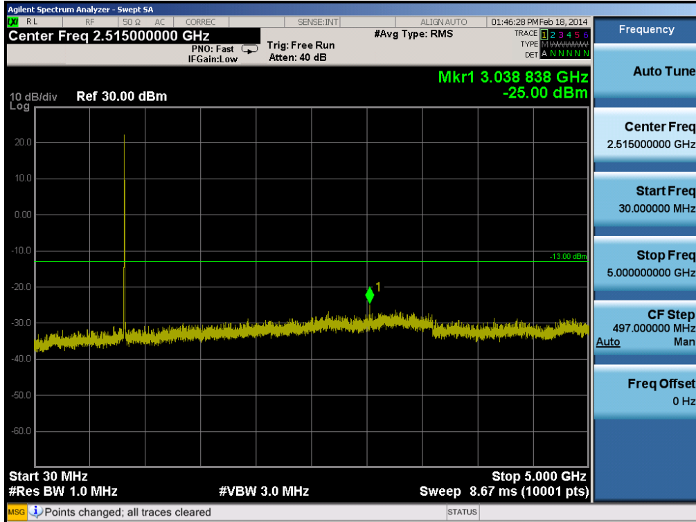
Plot 6-43. Conducted Spurious Plot (Cellular WCDMA Mode – Ch. 4183)
