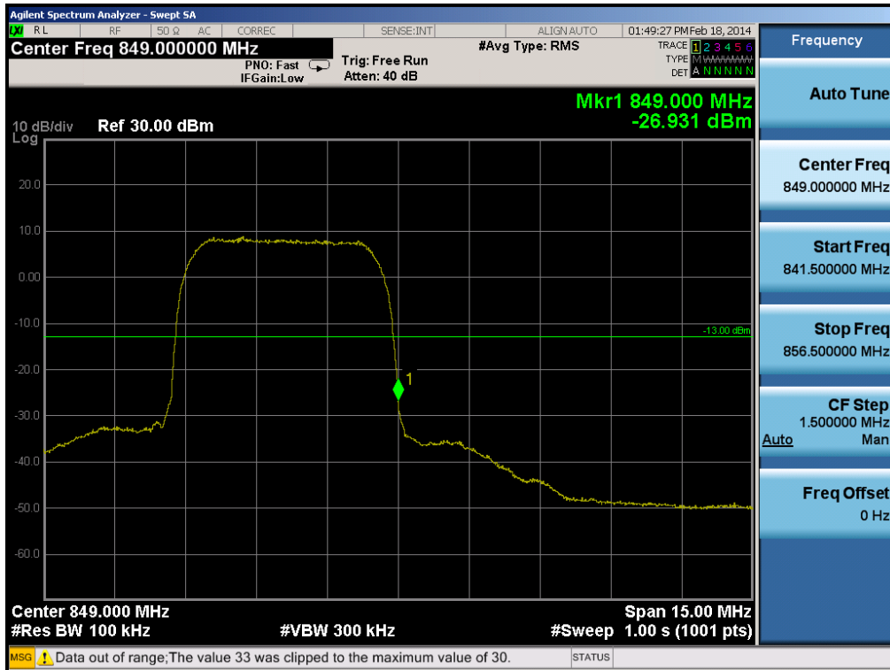
Plot 6-62. Band Edge Plot (Cellular WCDMA Mode – Ch. 4233)
