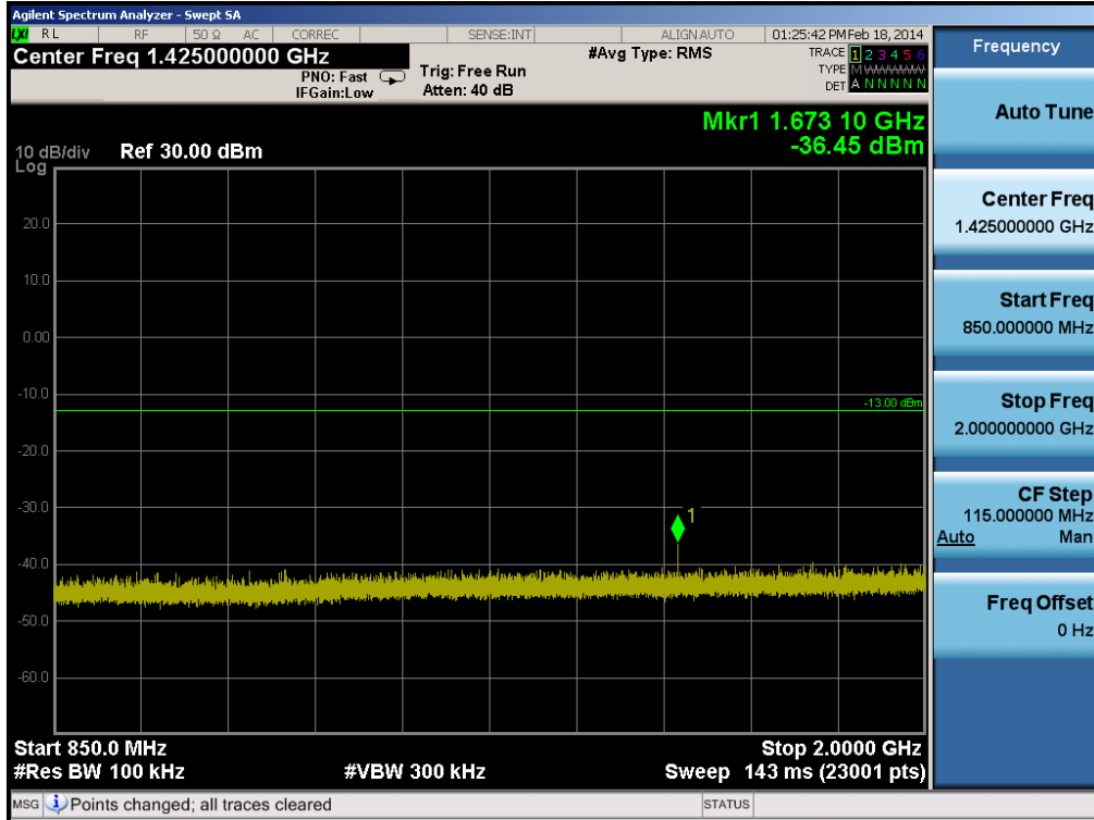
Plot 6-15. Conducted Spurious Plot (Cellular GSM Mode, Master – Ch. 190)
