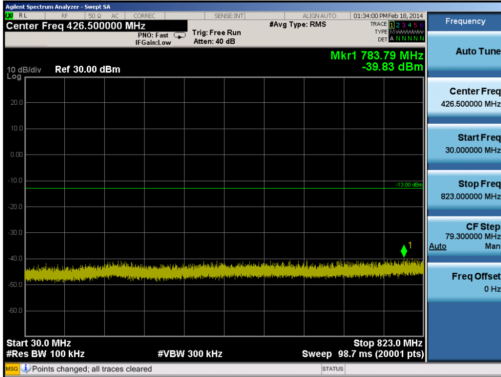
Plot 6-17. Conducted Spurious Plot (Cellular GSM Mode, Master – Ch. 251)
