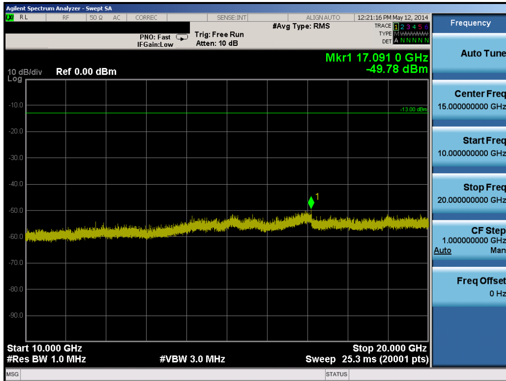
Plot 6-36. Conducted Spurious Plot (PCS GSM Mode, Slave – Ch. 512)
