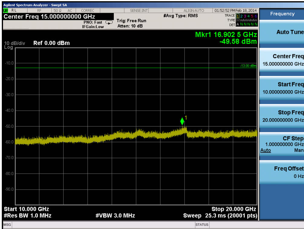
Plot 6-48. Conducted Spurious Plot (PCS WCDMA Mode – Ch. 9262)
