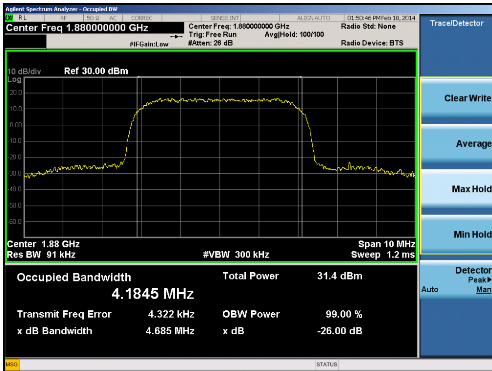
Plot 6-10. Occupied Bandwidth Plot (PCS WCDMA Mode – Ch. 9400)
