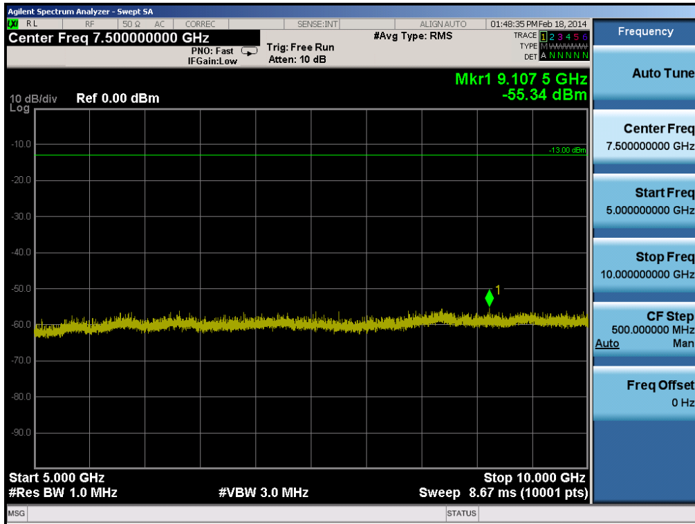
Plot 6-42. Conducted Spurious Plot (Cellular WCDMA Mode – Ch. 4132)
