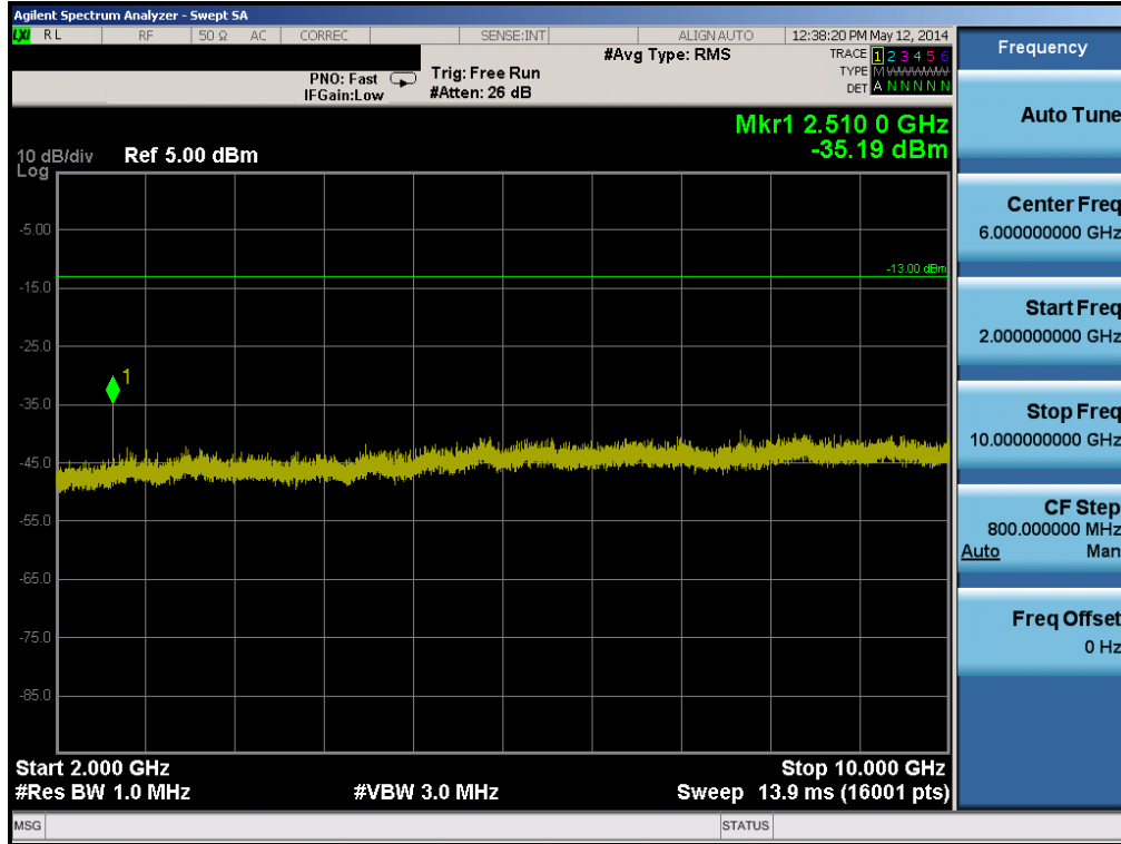
Plot 6-31. Conducted Spurious Plot (Cellular GSM Mode, Slave – Ch. 190)
