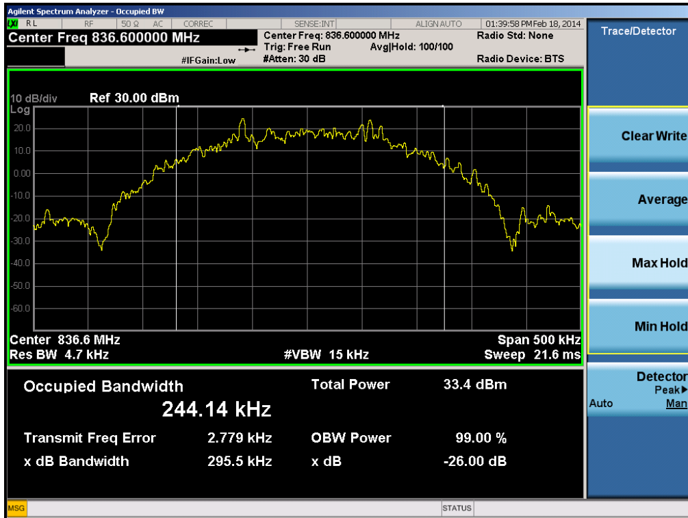
Plot 6-2. Occupied Bandwidth Plot (EDGE850 Mode, Master – Ch. 190)
