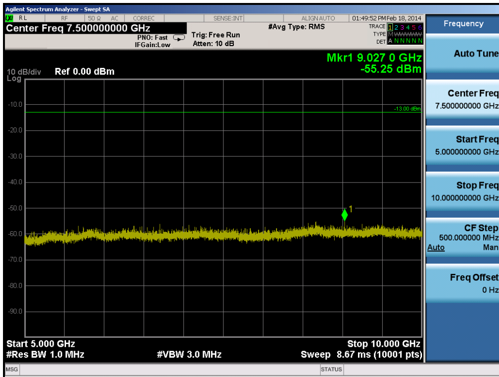
Plot 6-46. Conducted Spurious Plot (Cellular WCDMA Mode – Ch. 4233)
