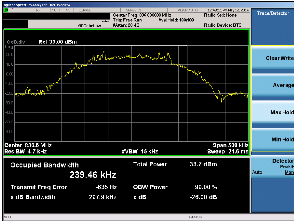
Plot 6-6. Occupied Bandwidth Plot (EDGE850 Mode, Slave – Ch. 190)
