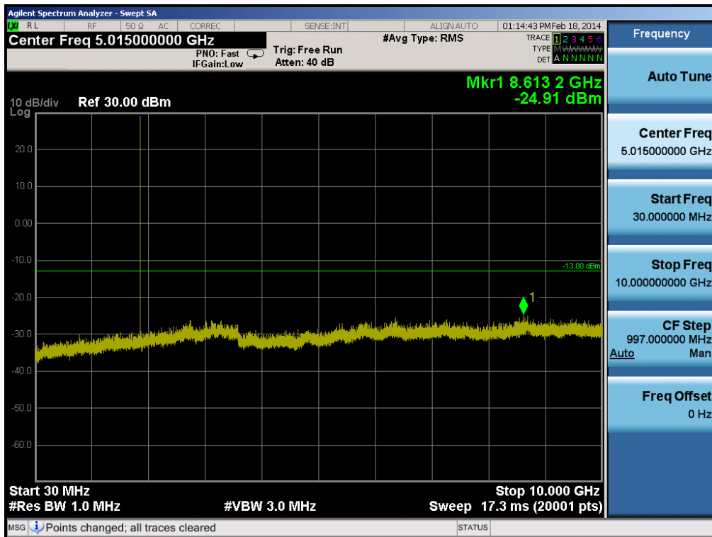
Plot 6-22. Conducted Spurious Plot (PCS GSM Mode, Master – Ch. 661)
