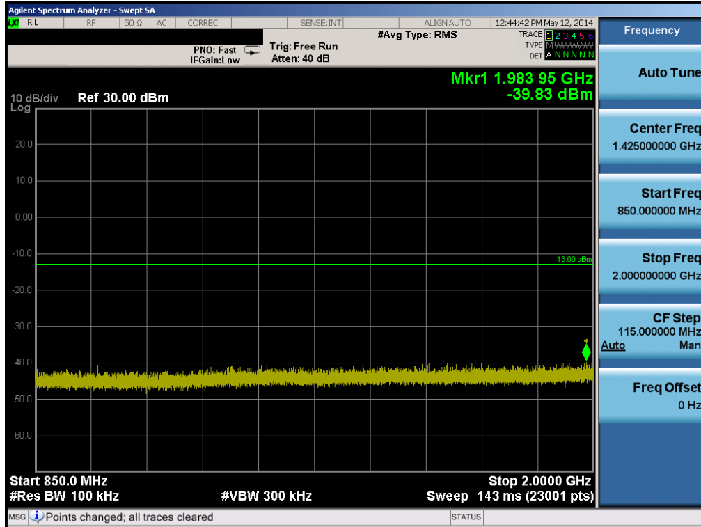
Plot 6-33. Conducted Spurious Plot (Cellular GSM Mode, Slave – Ch. 251)
