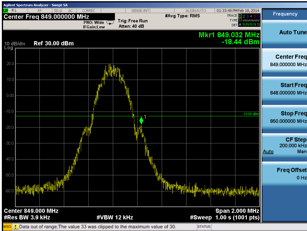
Plot 6-54. Band Edge Plot (Cellular GSM Mode, Master – Ch. 251)
