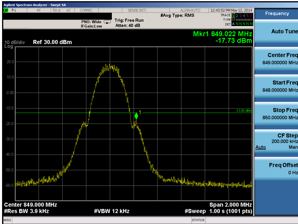
Plot 6-58. Band Edge Plot (Cellular GSM Mode, Slave – Ch. 251)
