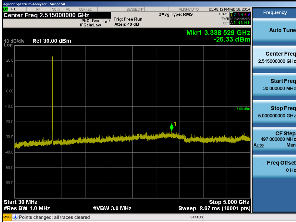
Plot 6-41. Conducted Spurious Plot (Cellular WCDMA Mode – Ch. 4132)
