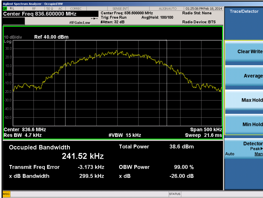
Plot 6-1. Occupied Bandwidth Plot (Cellular GSM Mode, Master – Ch. 190)
