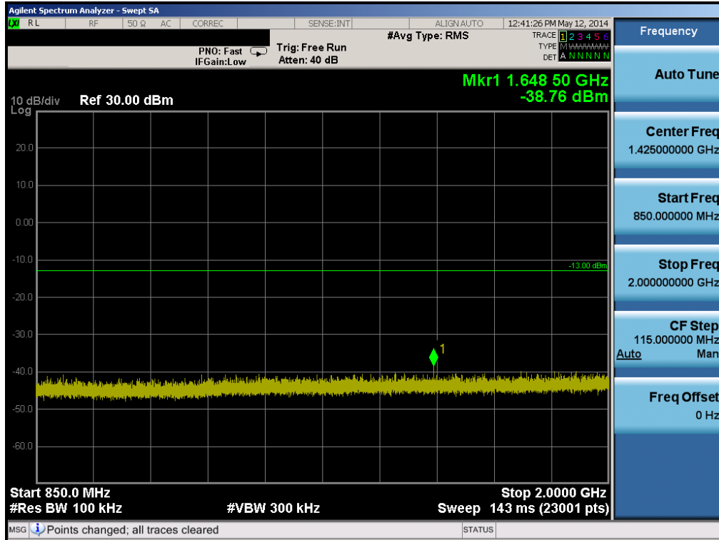
Plot 6-27. Conducted Spurious Plot (Cellular GSM Mode, Slave – Ch. 128)
