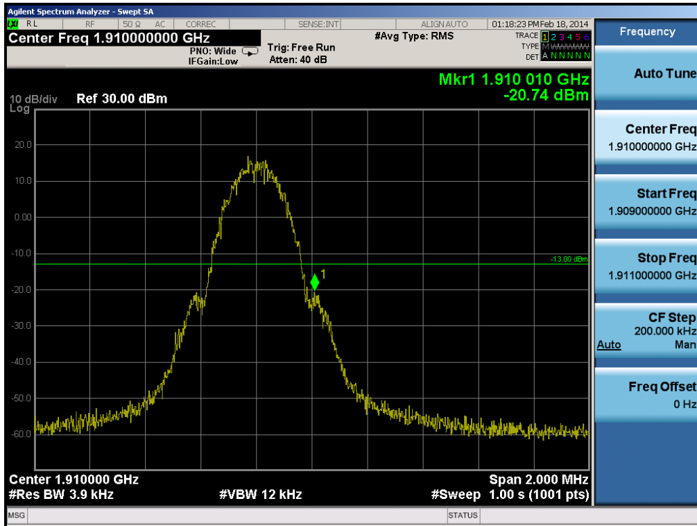
Plot 6-56. Band Edge Plot (PCS GSM Mode, Master – Ch. 810)
