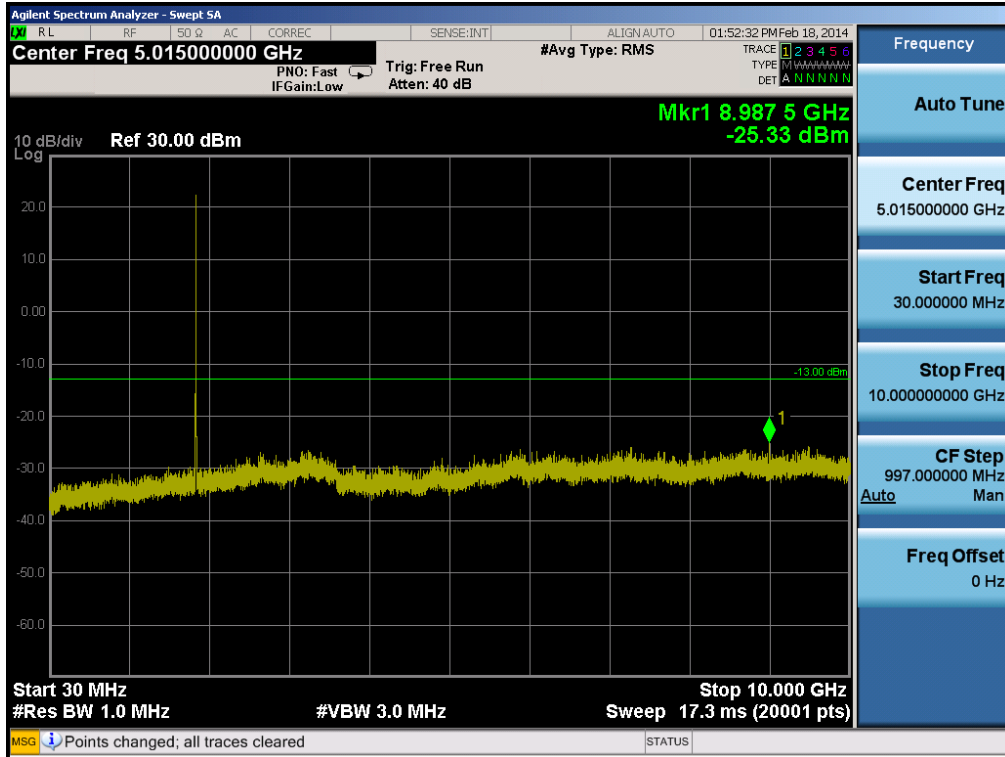
Plot 6-47. Conducted Spurious Plot (PCS WCDMA Mode – Ch. 9262)
