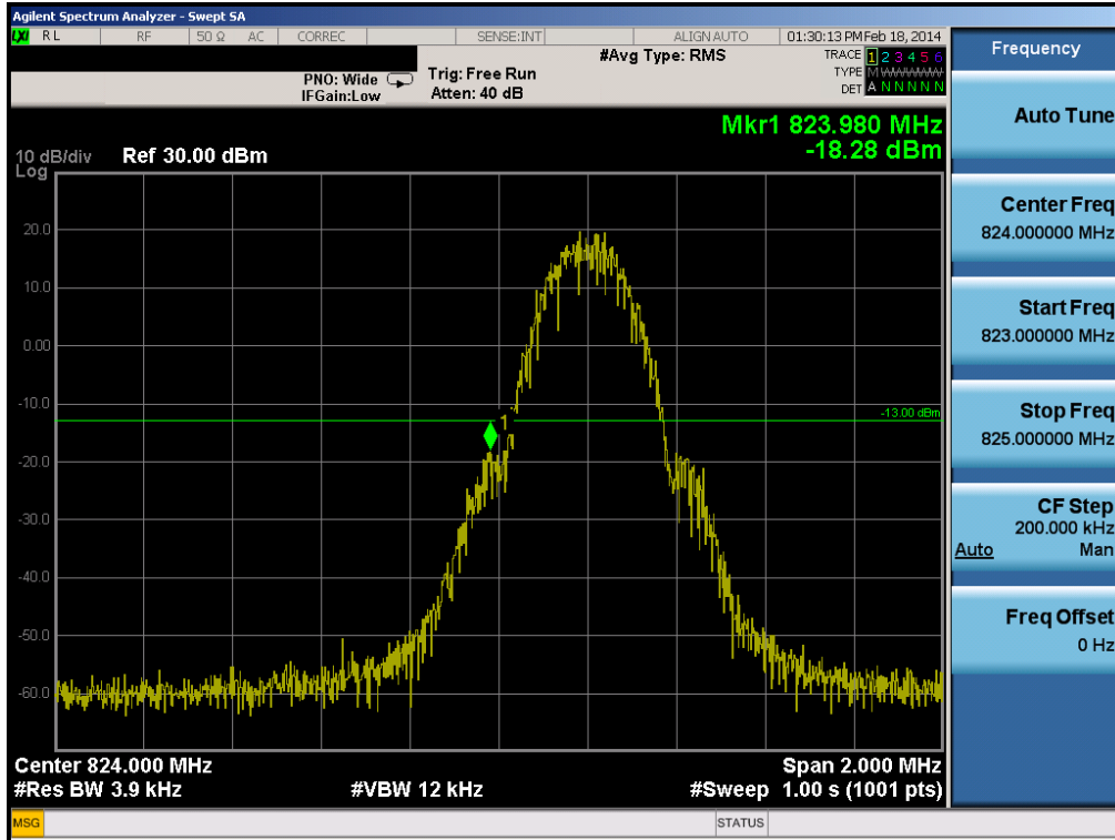
Plot 6-53. Band Edge Plot (Cellular GSM Mode, Master – Ch. 128)
