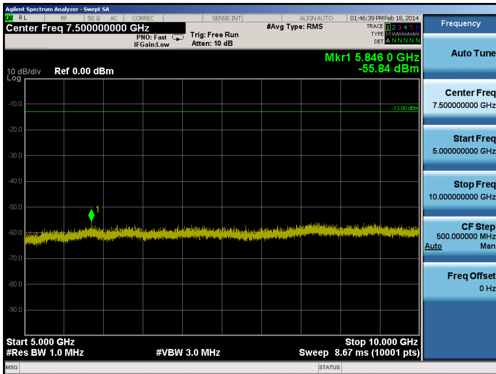
Plot 6-44. Conducted Spurious Plot (Cellular WCDMA Mode – Ch. 4183)
