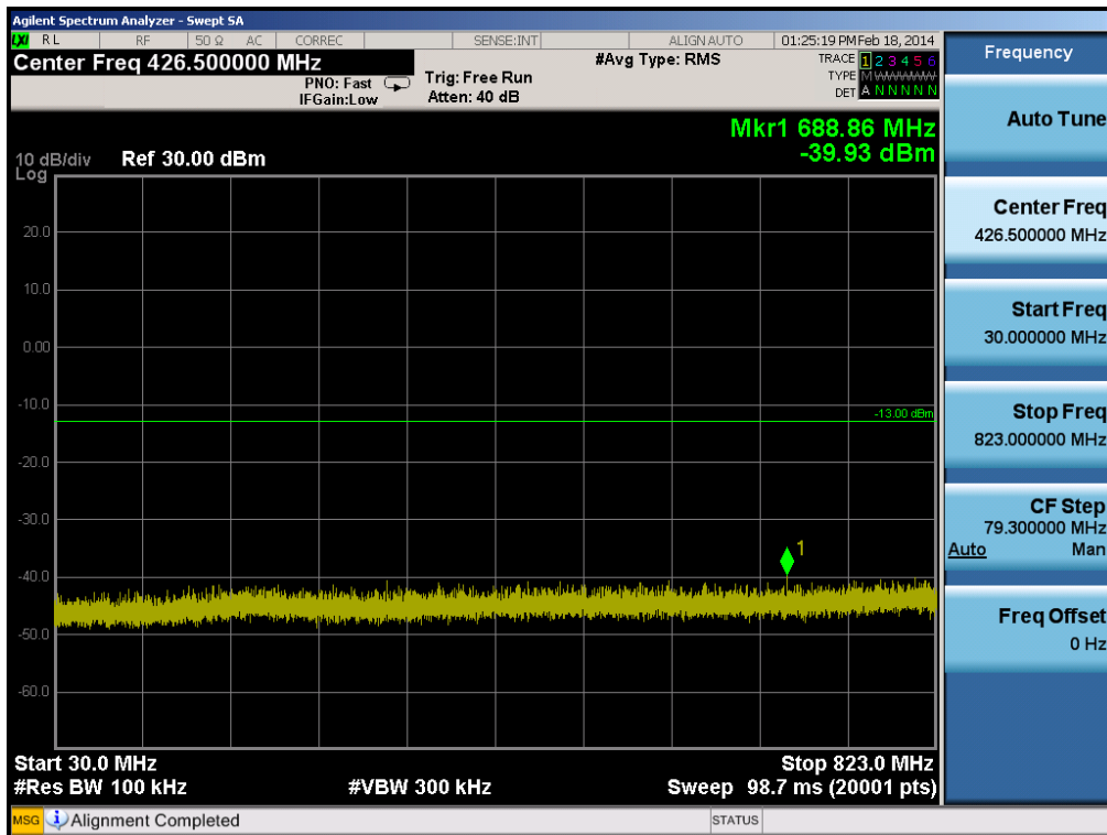
Plot 6-14. Conducted Spurious Plot (Cellular GSM Mode, Master – Ch. 190)
