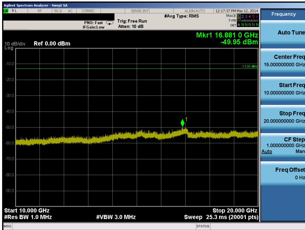
Plot 6-38. Conducted Spurious Plot (PCS GSM Mode, Slave – Ch. 661)
