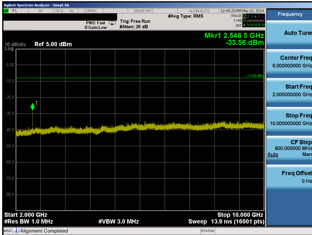
Plot 6-34. Conducted Spurious Plot (Cellular GSM Mode, Slave – Ch. 251)
