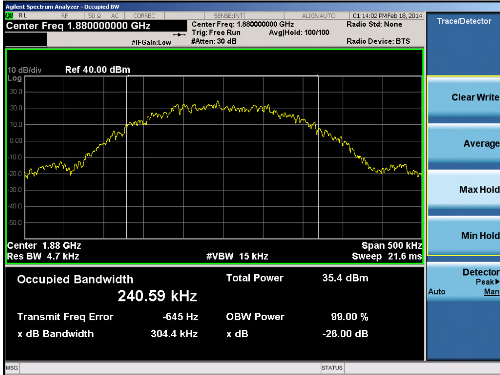
Plot 6-3. Occupied Bandwidth Plot (PCS GSM Mode, Master – Ch. 661)
