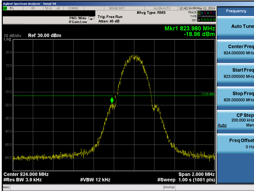
Plot 6-57. Band Edge Plot (Cellular GSM Mode, Slave – Ch. 128)
