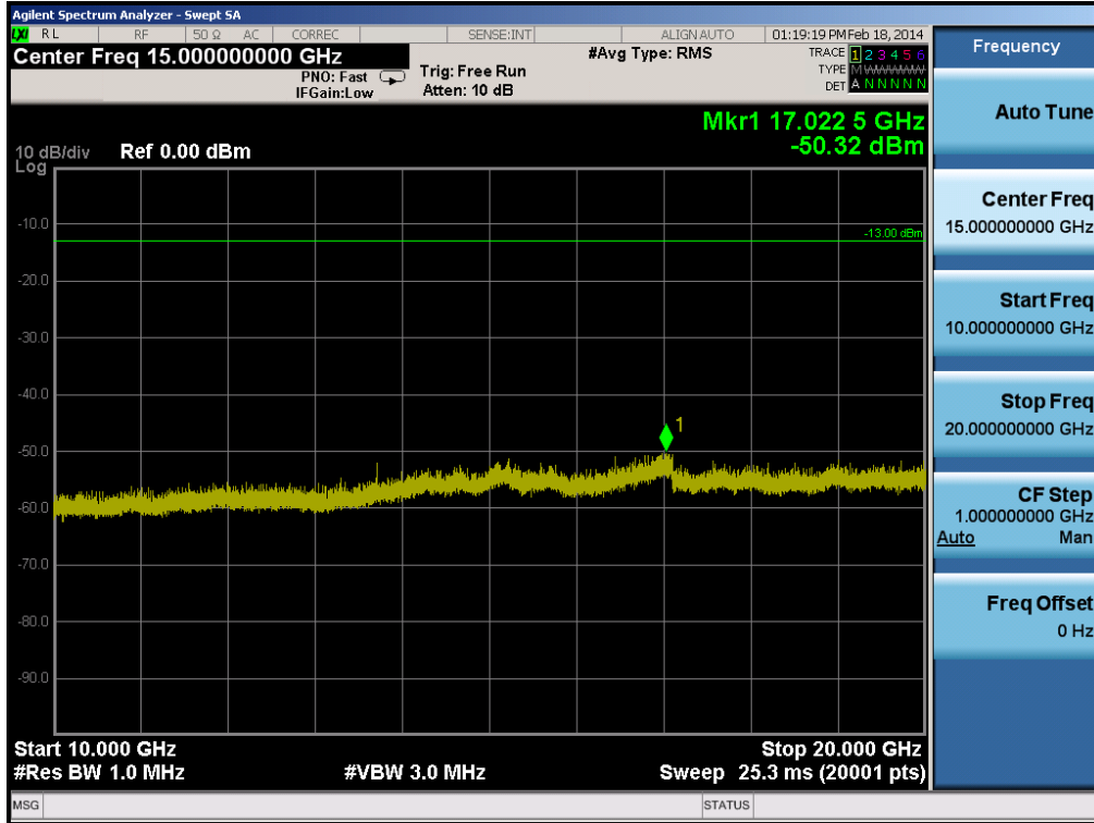
Plot 6-25. Conducted Spurious Plot (PCS GSM Mode, Master – Ch. 810)
