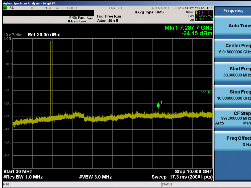
Plot 6-39. Conducted Spurious Plot (PCS GSM Mode, Slave – Ch. 810)
