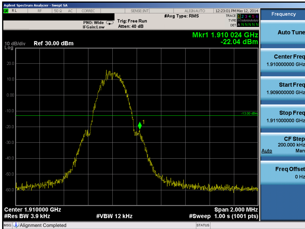
Plot 6-60. Band Edge Plot (PCS GSM Mode, Slave – Ch. 810)
