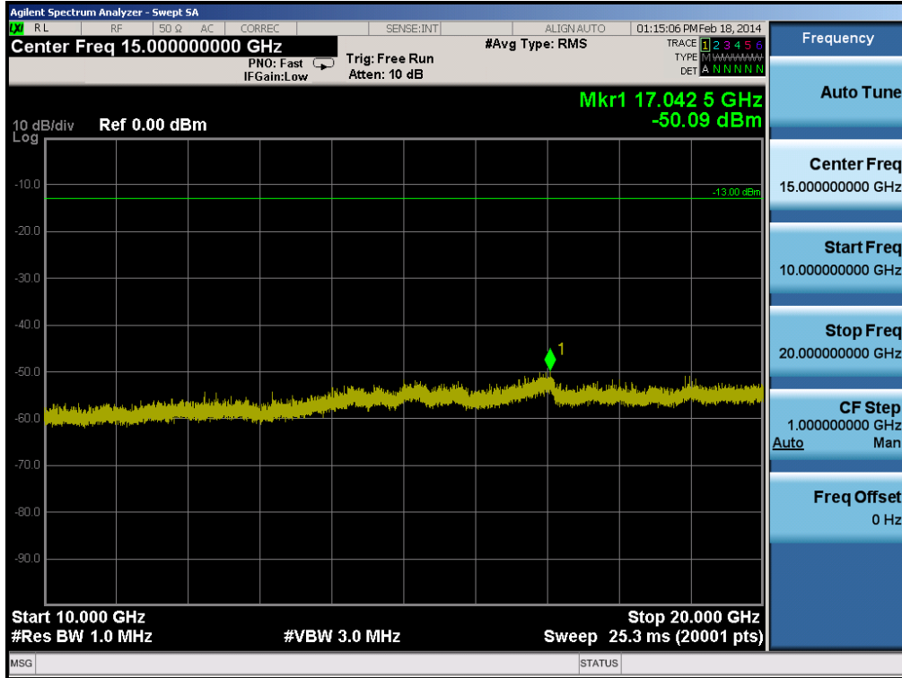
Plot 6-23. Conducted Spurious Plot (PCS GSM Mode, Master – Ch. 661)
