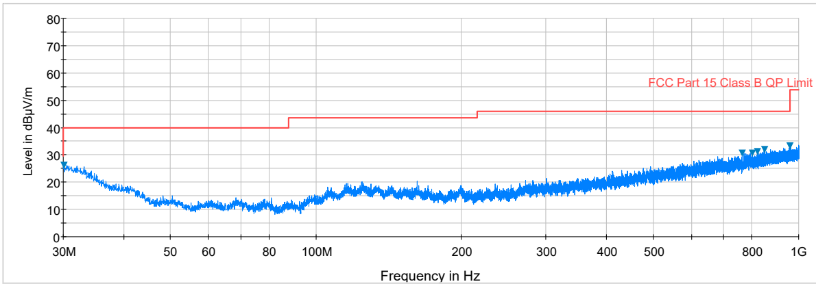
Plot 7-1. Radiated Spurious Plot below 1GHz (Pol. H)
