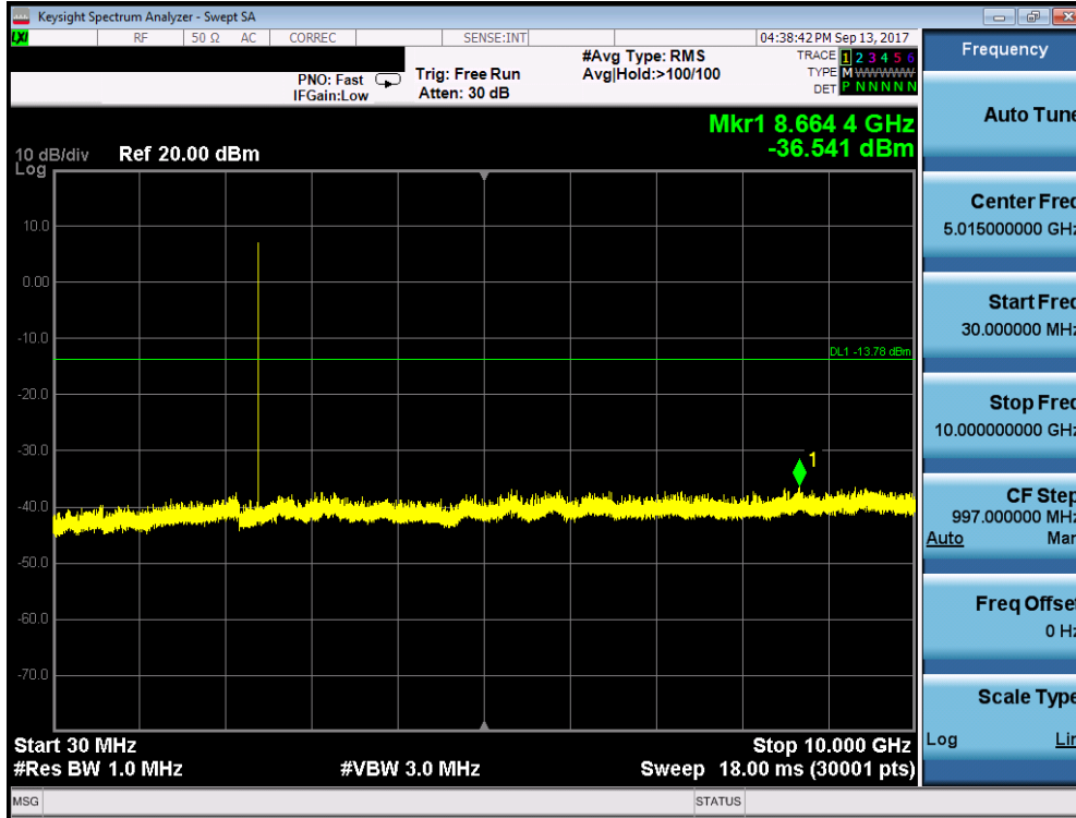
Plot 7-29. Conducted Spurious Plot (Bluetooth (LE), 2Mbps – Ch. 0)
