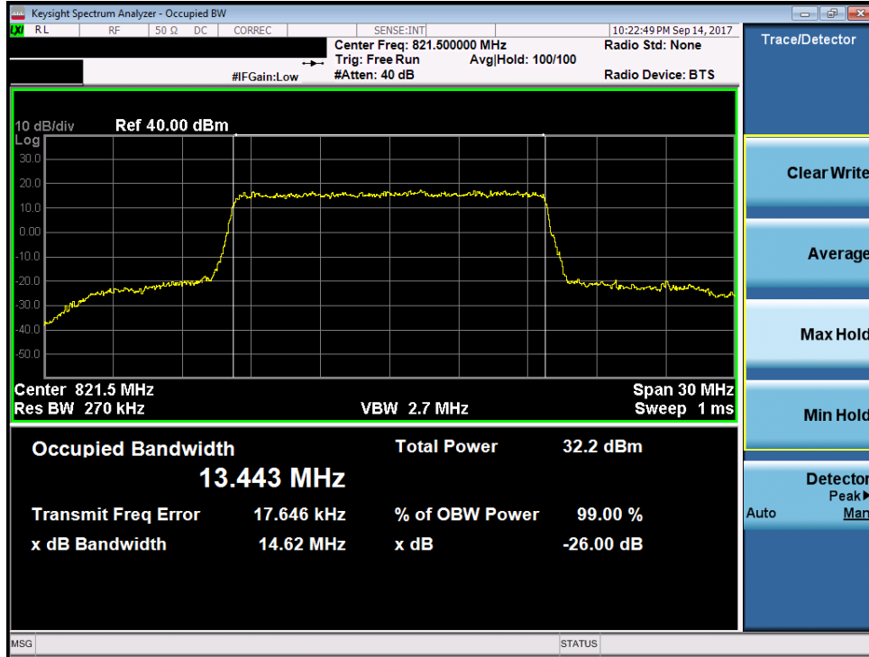
Plot 7-15. Occupied Bandwidth Plot (15MHz QPSK – RB Size 75)
