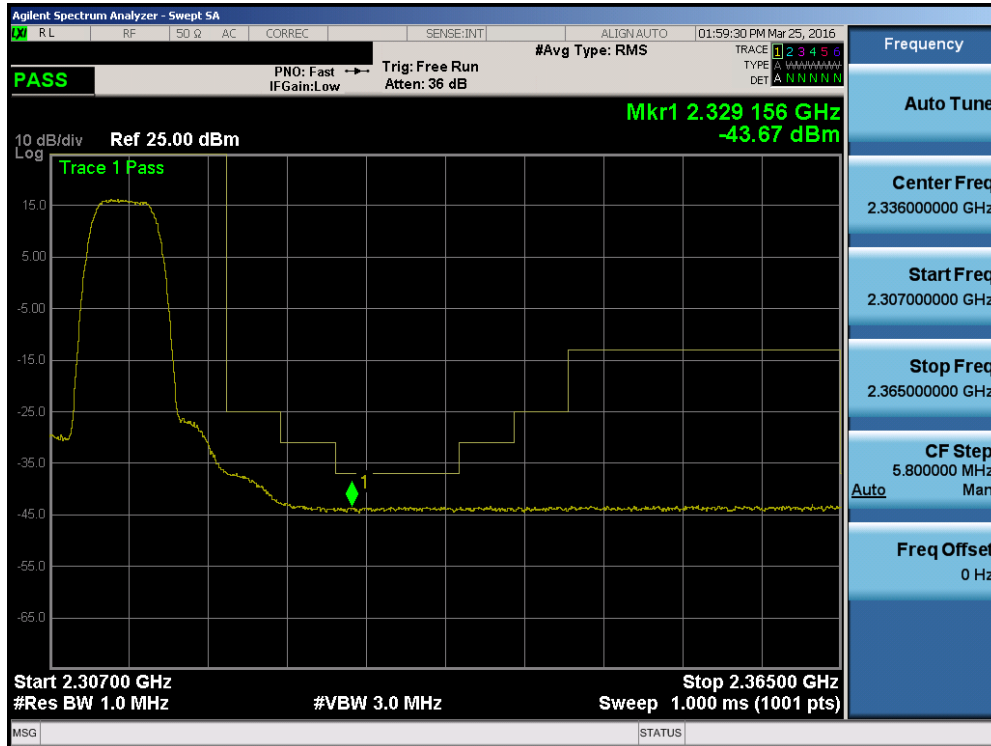
Plot 7-186. Upper Extended Band Edge Plot (Band 30 – 5.0MHz QPSK – RB Size 50)
