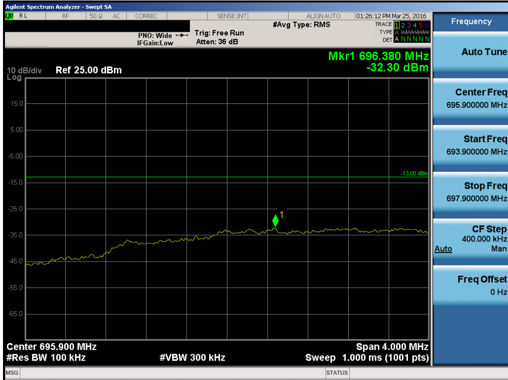
Plot 7-116. Lower Extended Band Edge Plot (Band 12 – 5.0MHz QPSK – RB Size 25)
