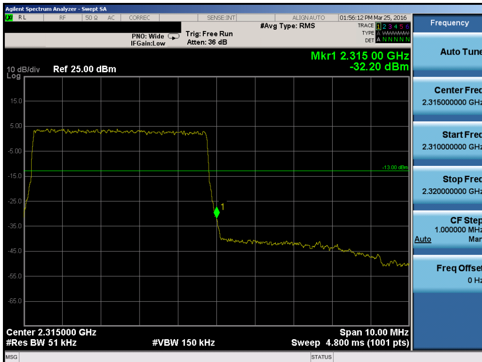
Plot 7-185. Upper Band Edge Plot (Band 30 – 5.0MHz QPSK – RB Size 50)
