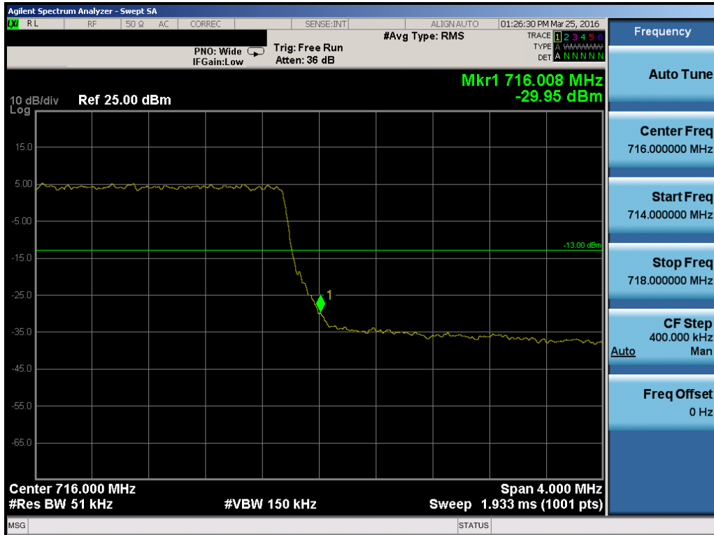
Plot 7-117. Upper Band Edge Plot (Band 12 – 5.0MHz QPSK – RB Size 25)
