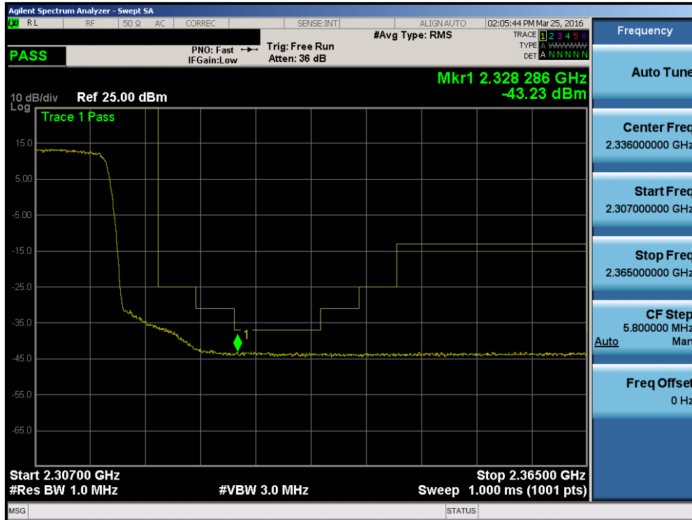
Plot 7-190. Upper Extended Band Edge Plot (Band 30 – 10.0MHz QPSK – RB Size 50)
