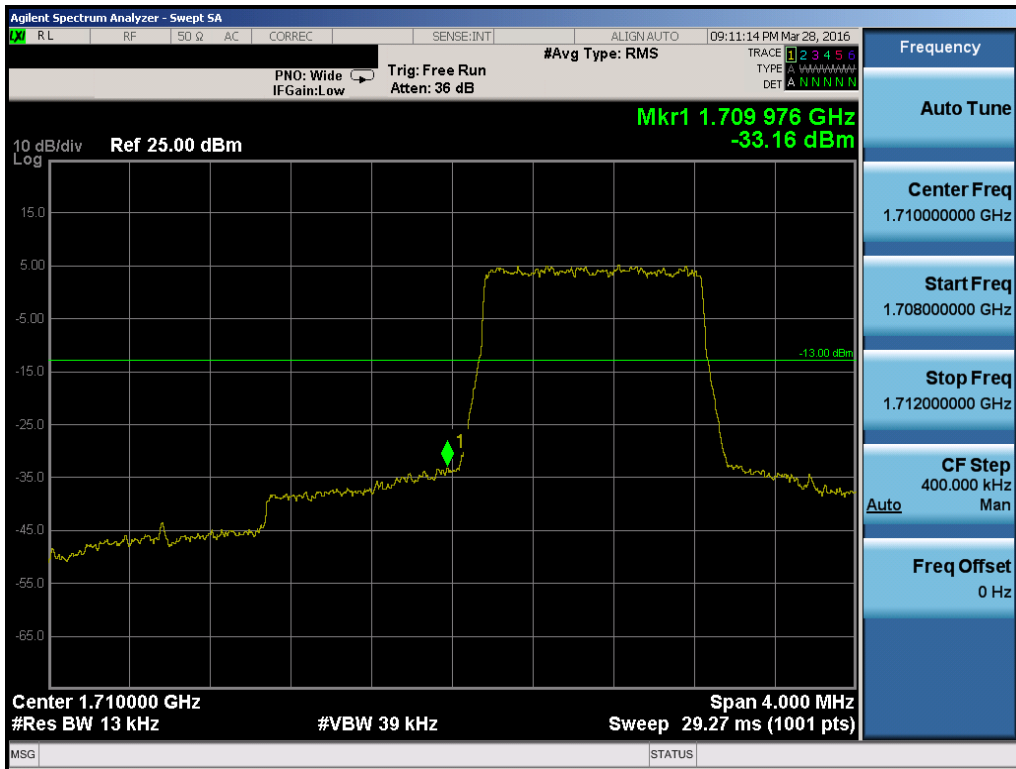
Plot 7-135. Lower Band Edge Plot (Band 4 – 1.4MHz QPSK – RB Size 6)
