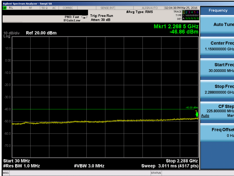
Plot 7-95. Conducted Spurious Plot (Band 30 – 10.0MHz QPSK – RB Size 1, RB Offset 0 – High Channel)
