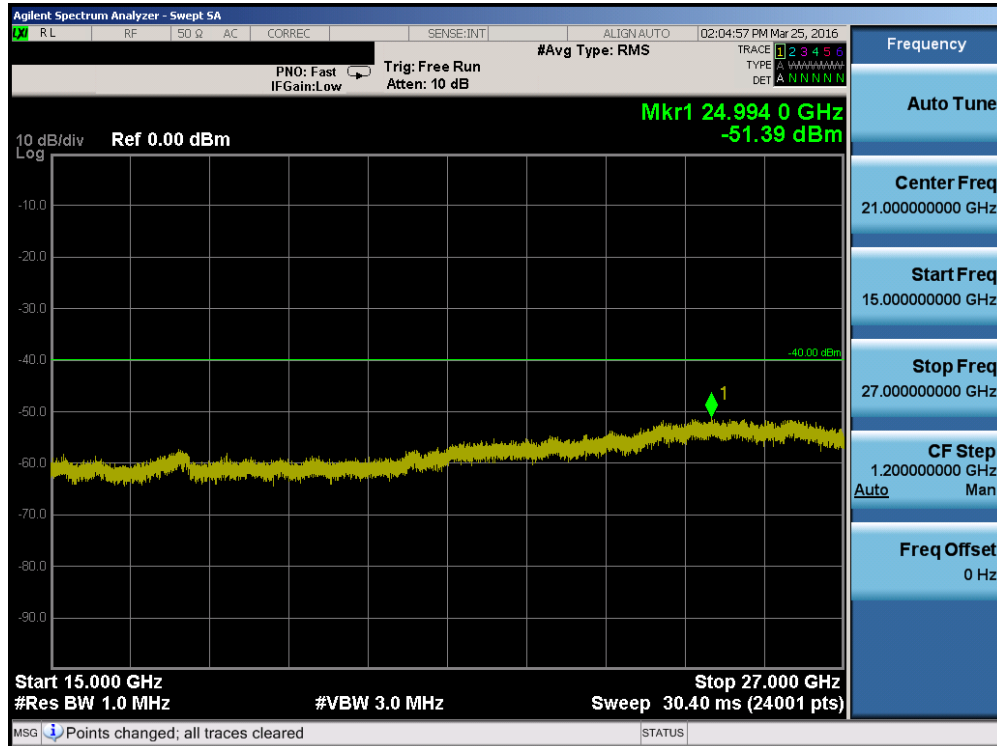
Plot 7-97. Conducted Spurious Plot (Band 30 – 10.0MHz QPSK – RB Size 1, RB Offset 0 – High Channel)
