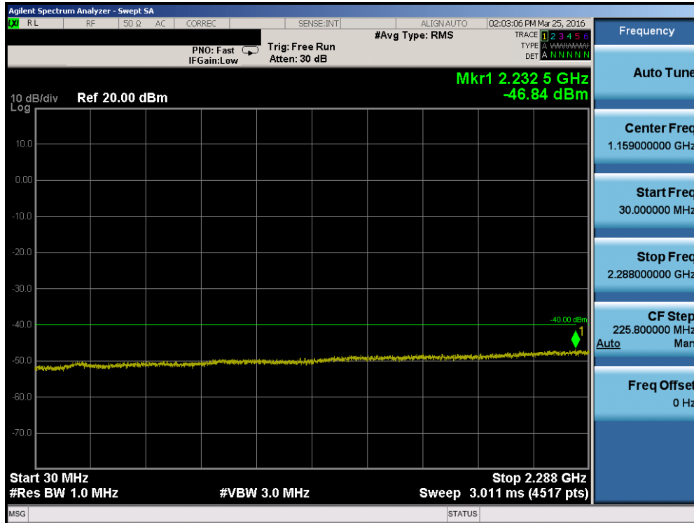
Plot 7-89. Conducted Spurious Plot (Band 30 – 10.0MHz QPSK – RB Size 1, RB Offset 0– Low Channel)
