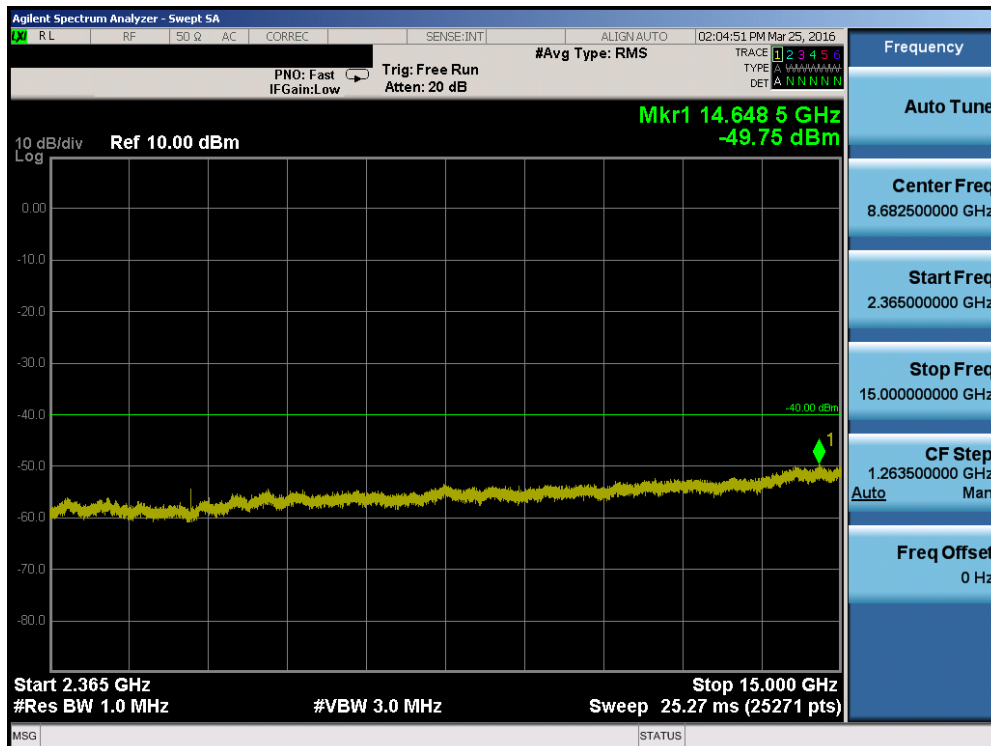
Plot 7-96. Conducted Spurious Plot (Band 30 – 10.0MHz QPSK – RB Size 1, RB Offset 0 – High Channel)
