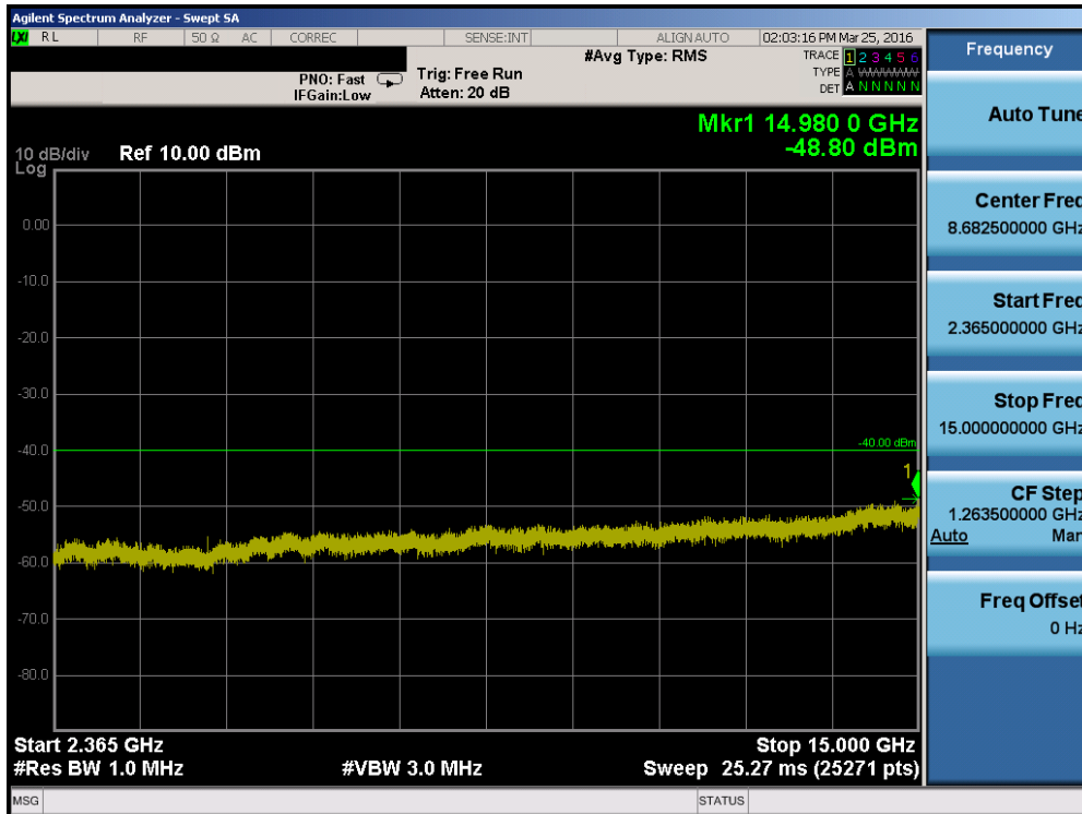
Plot 7-90. Conducted Spurious Plot (Band 30 – 10.0MHz QPSK – RB Size 1, RB Offset 0 – Low Channel)
