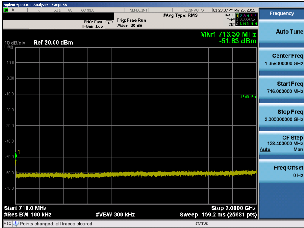
Plot 7-57. Conducted Spurious Plot (Band 12 – 10.0MHz QPSK – RB Size 1, RB Offset 0 – Mid Channel)
