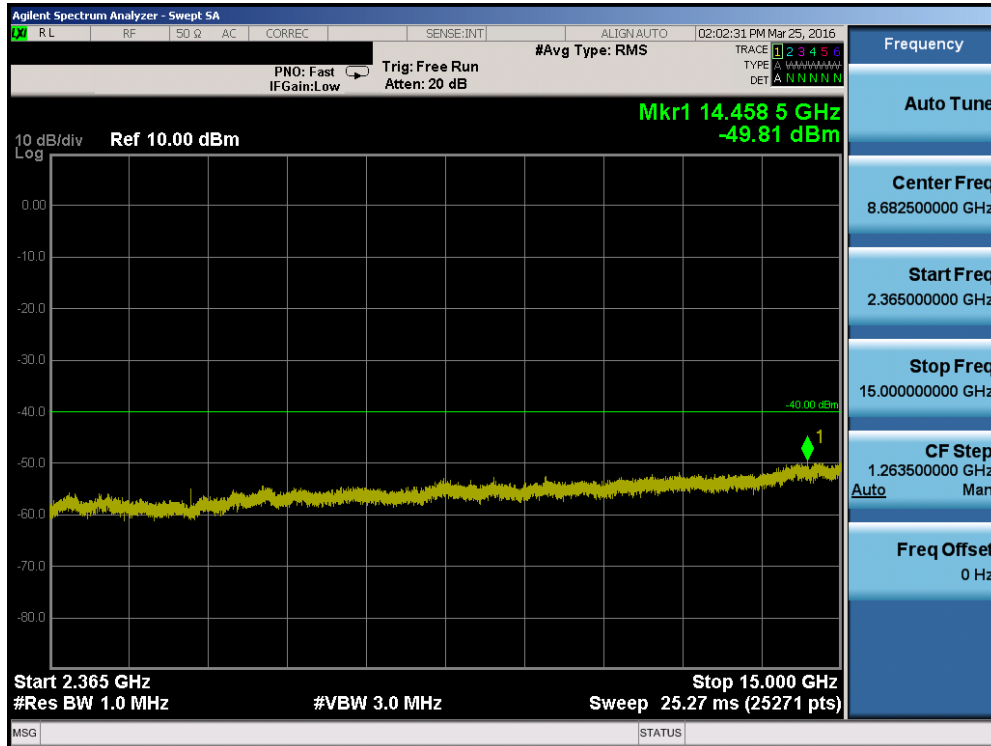
Plot 7-93. Conducted Spurious Plot (Band 30 – 10.0MHz QPSK – RB Size 1, RB Offset 0 – Mid Channel)
