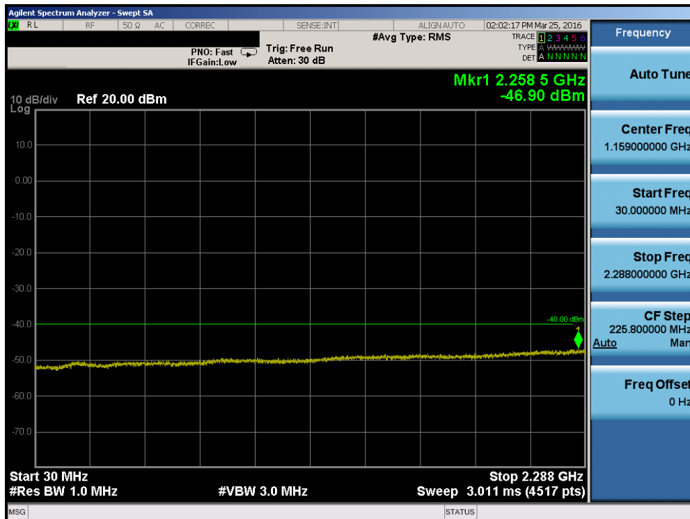
Plot 7-92. Conducted Spurious Plot (Band 30 – 10.0MHz QPSK – RB Size 1, RB Offset 0 – Mid Channel)
