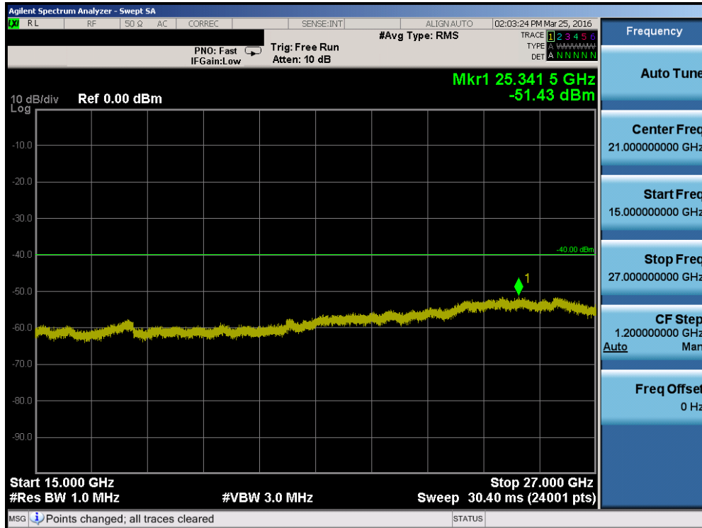
Plot 7-91. Conducted Spurious Plot (Band 30 – 10.0MHz QPSK – RB Size 1, RB Offset 0 – Low Channel)
