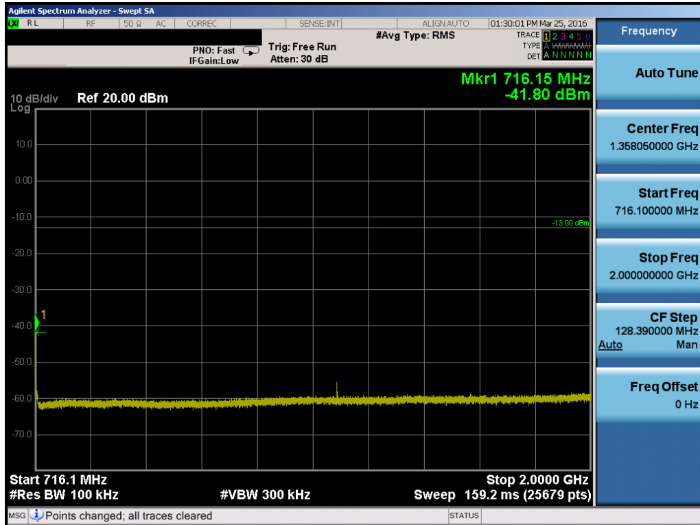
Plot 7-60. Conducted Spurious Plot (Band 12 – 10.0MHz QPSK – RB Size 1, RB Offset 0 – High Channel)
