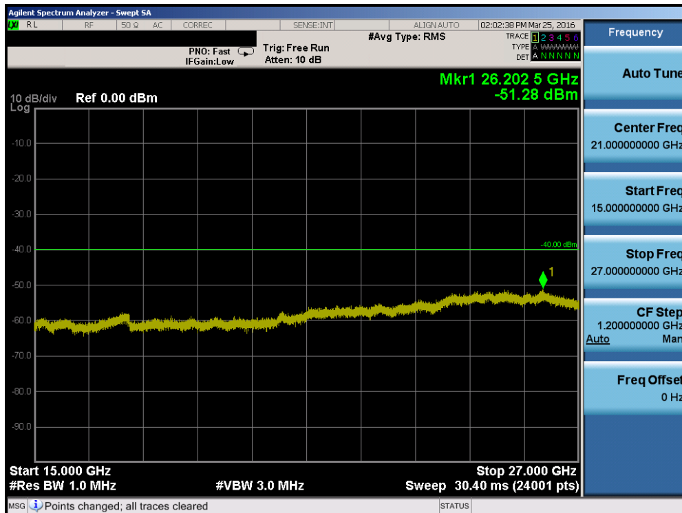
Plot 7-94. Conducted Spurious Plot (Band 30 – 10.0MHz QPSK – RB Size 1, RB Offset 0 – Mid Channel)
