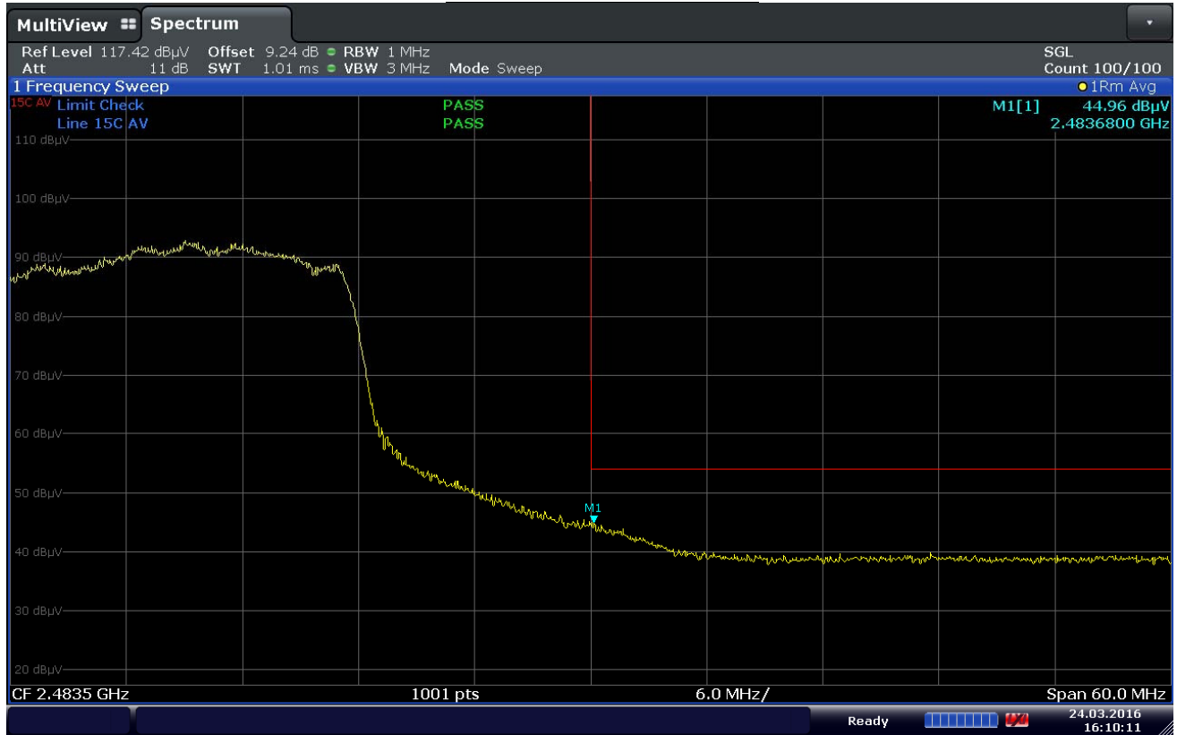
Plot 7-85. Radiated Restricted Upper Band Edge Measurement (Average)
