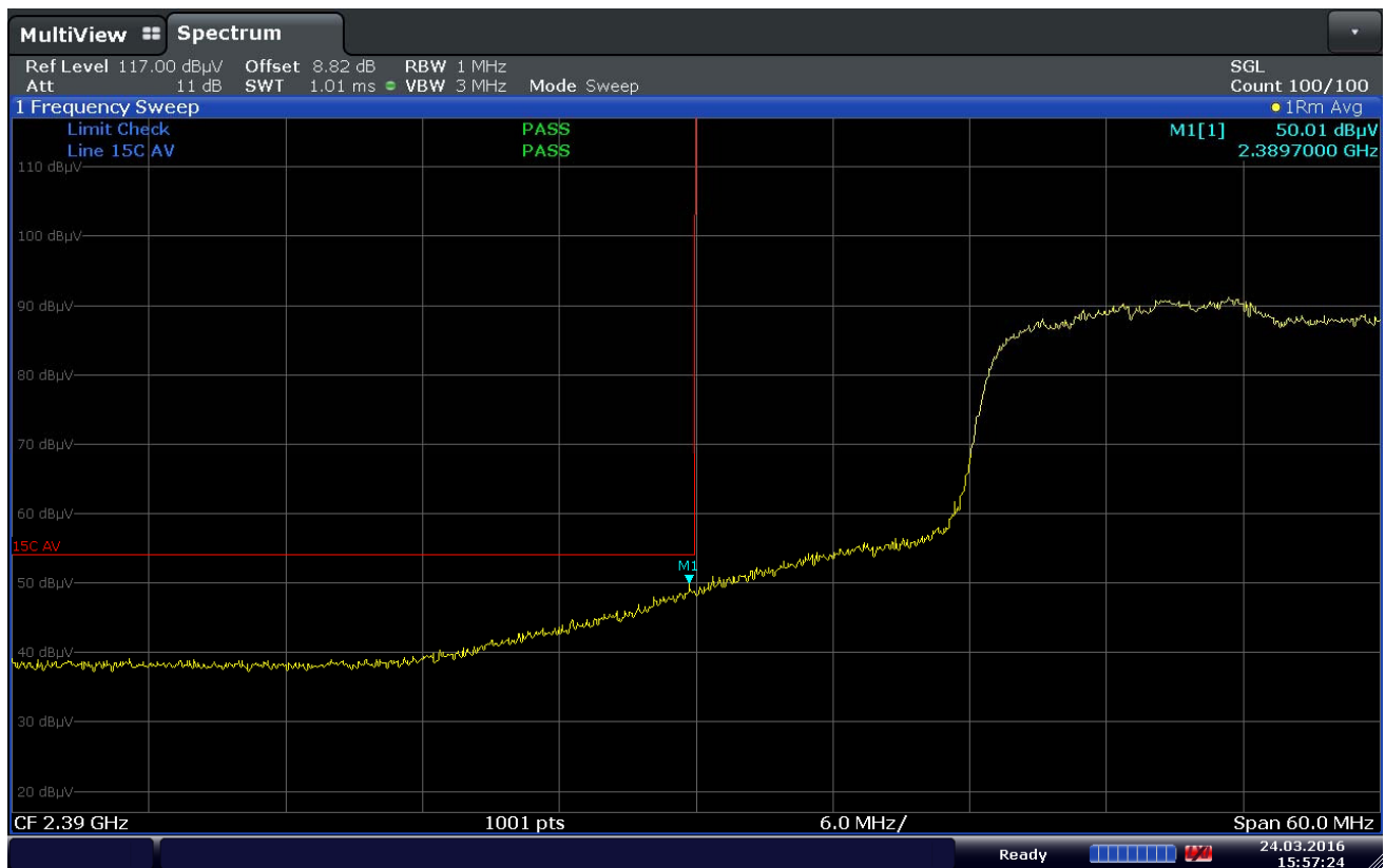
Plot 7-83. Radiated Restricted Lower Band Edge Measurement (Average)
