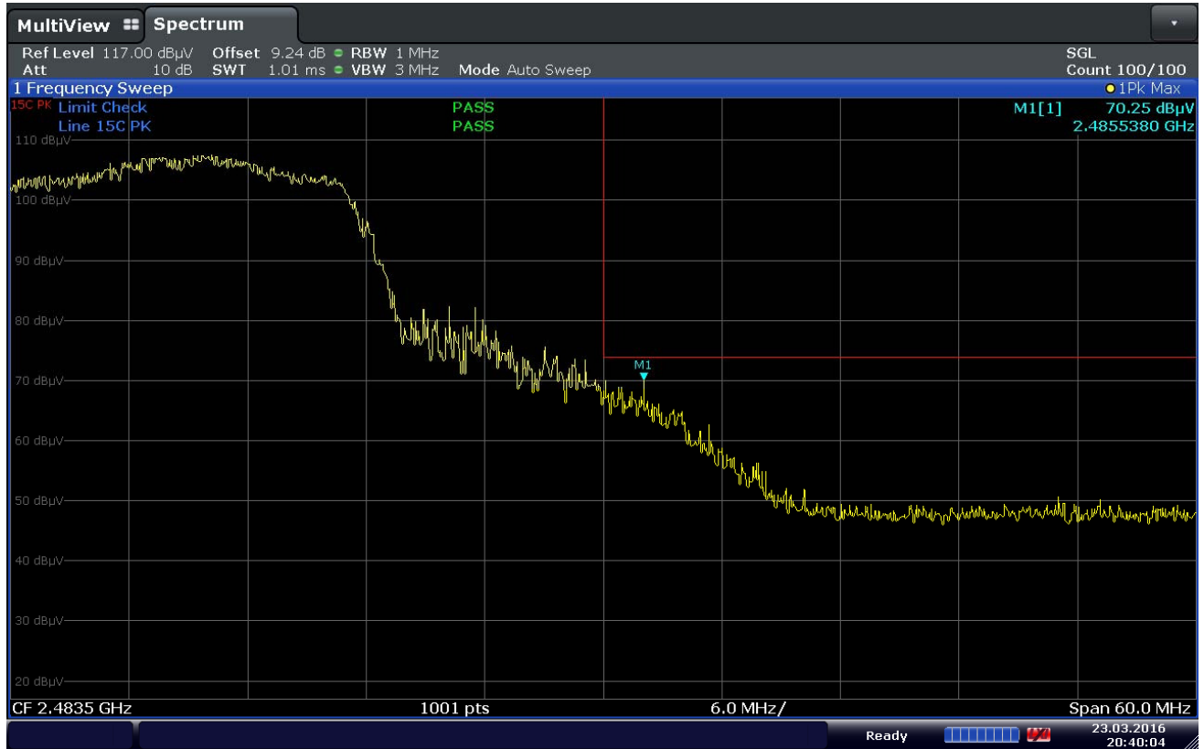
Plot 7-80. Radiated Restricted Upper Band Edge Measurement (Peak)
