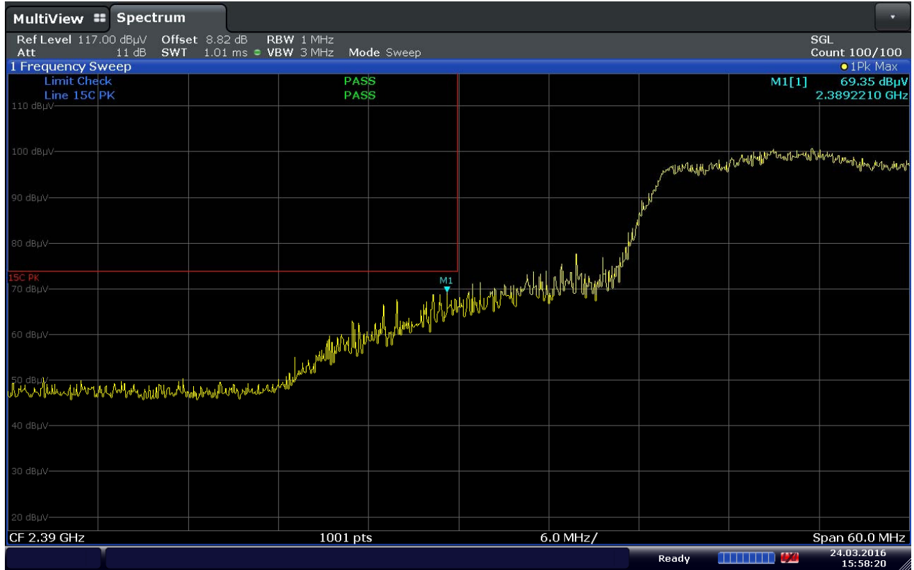
Plot 7-84. Radiated Restricted Lower Band Edge Measurement (Peak)
