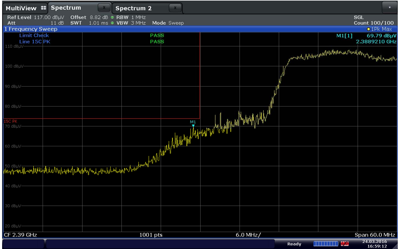
Plot 7-90. Radiated Restricted Lower Band Edge Measurement (Peak)
