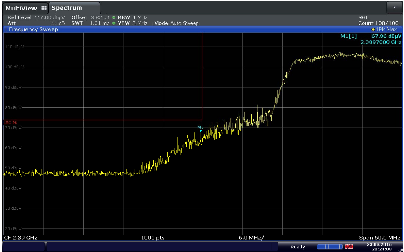
Plot 7-78. Radiated Restricted Lower Band Edge Measurement (Peak)
