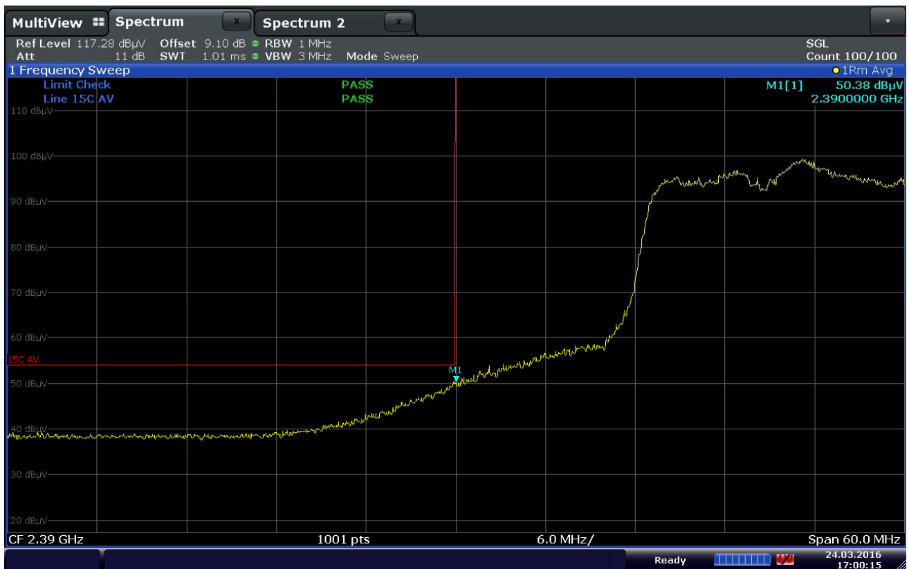
Plot 7-89. Radiated Restricted Lower Band Edge Measurement (Average)
