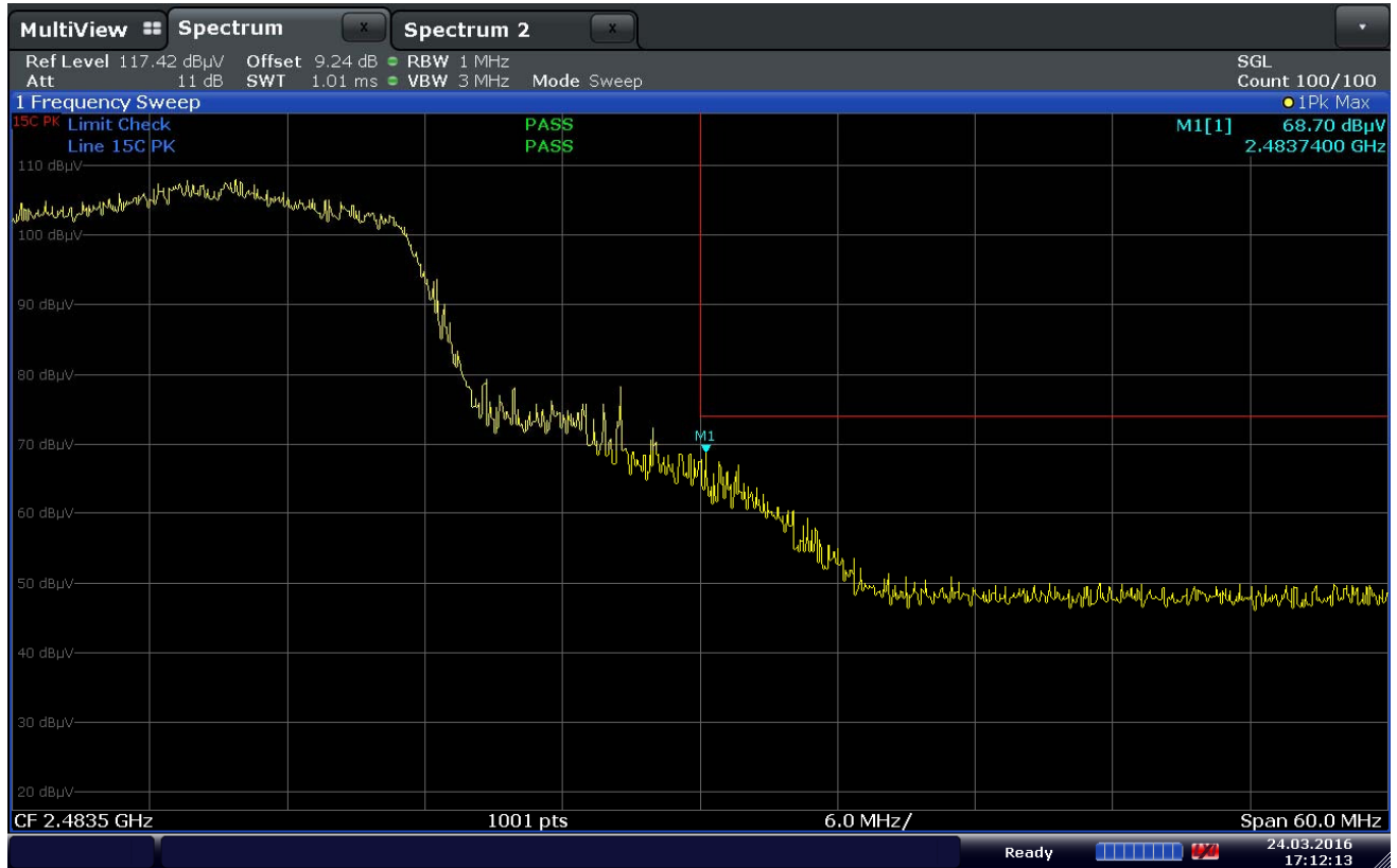
Plot 7-92. Radiated Restricted Upper Band Edge Measurement (Peak)
