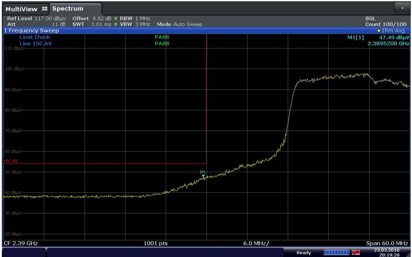
Plot 7-77. Radiated Restricted Lower Band Edge Measurement (Average)
