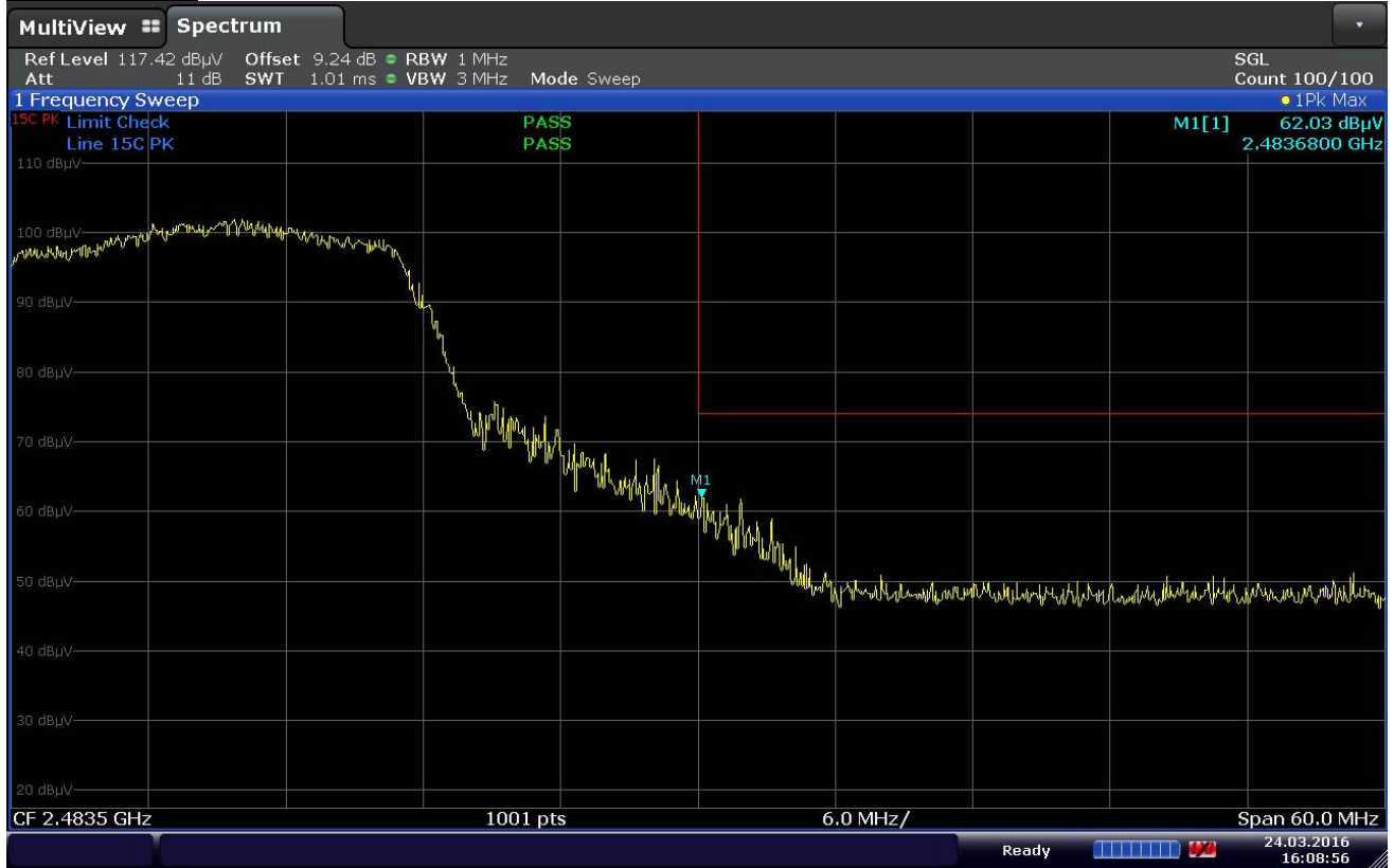
Plot 7-86. Radiated Restricted Upper Band Edge Measurement (Peak)
