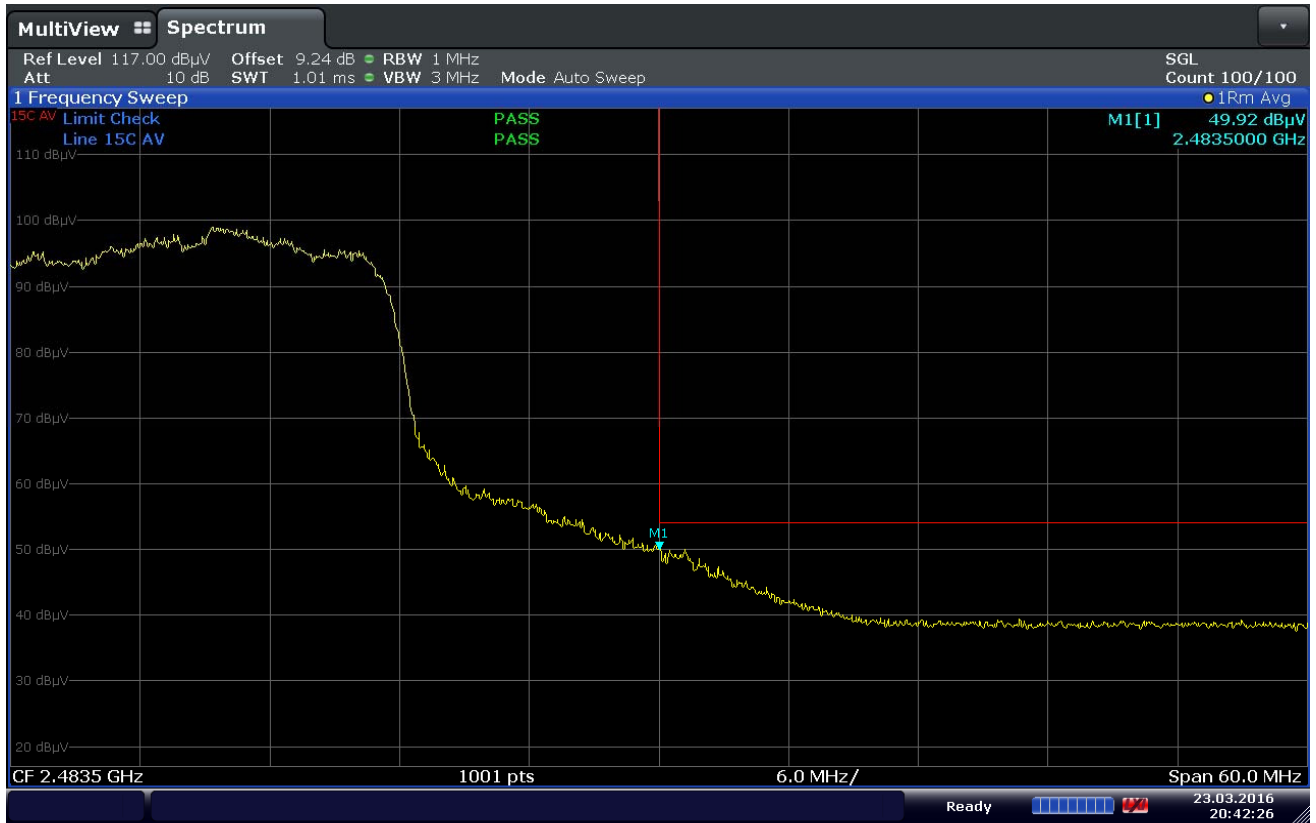
Plot 7-79. Radiated Restricted Upper Band Edge Measurement (Average)
