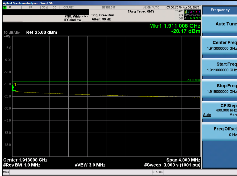
Plot 6-151. Upper Extended Band Edge Plot (Band 2 – 10.0MHz QPSK – RB Size 50)
