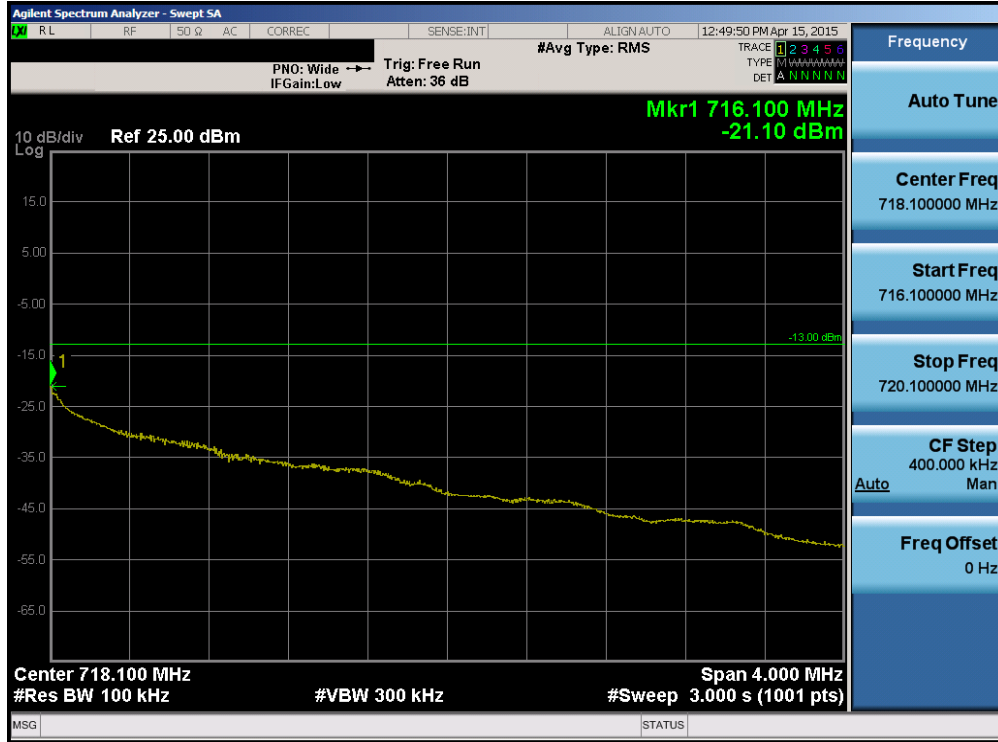
Plot 6-87. Upper Extended Band Edge Plot (Band 12 – 1.4MHz QPSK – RB Size 6)
