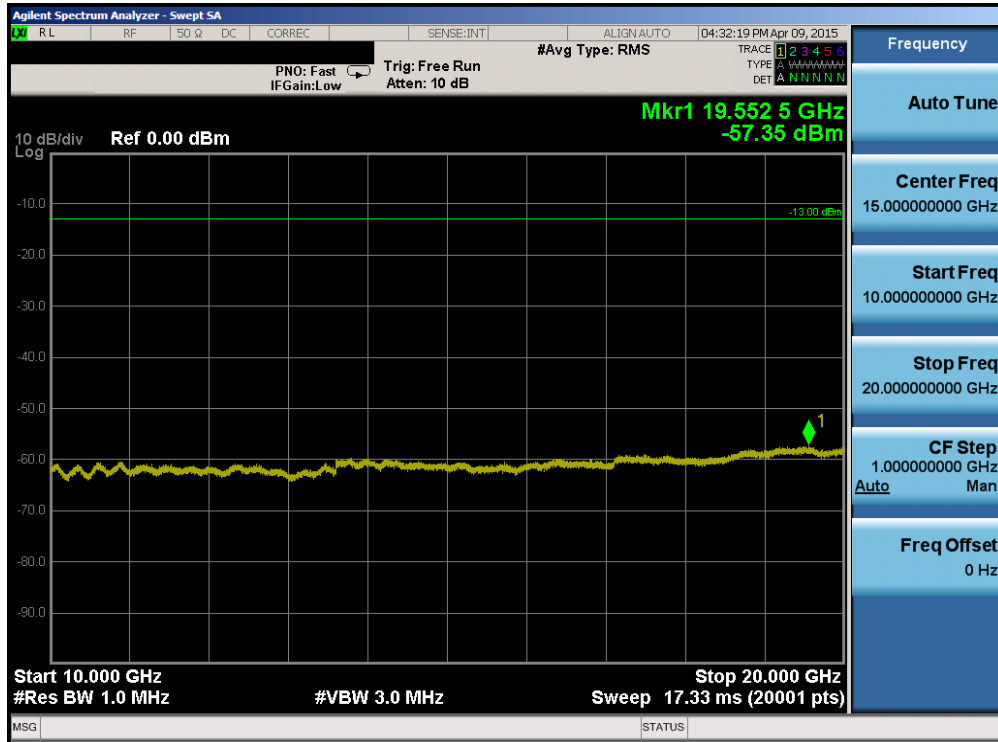
Plot 6-77. Conducted Spurious Plot (Band 2 – 1.4MHz QPSK – RB Size 1, RB Offset 0 – Mid Channel)
