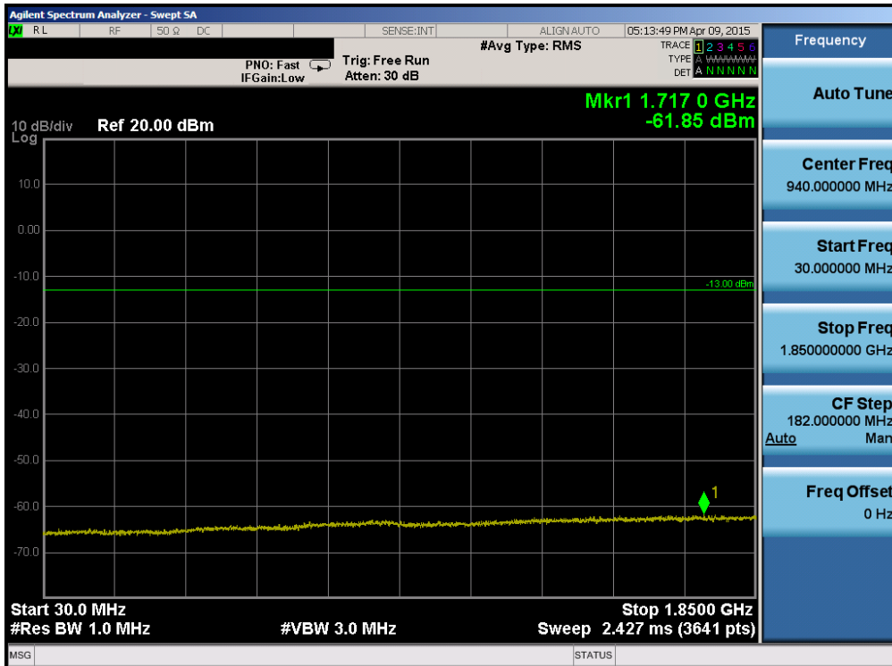
Plot 6-78. Conducted Spurious Plot (Band 2 – 1.4MHz QPSK – RB Size 1, RB Offset 0 – High Channel)
