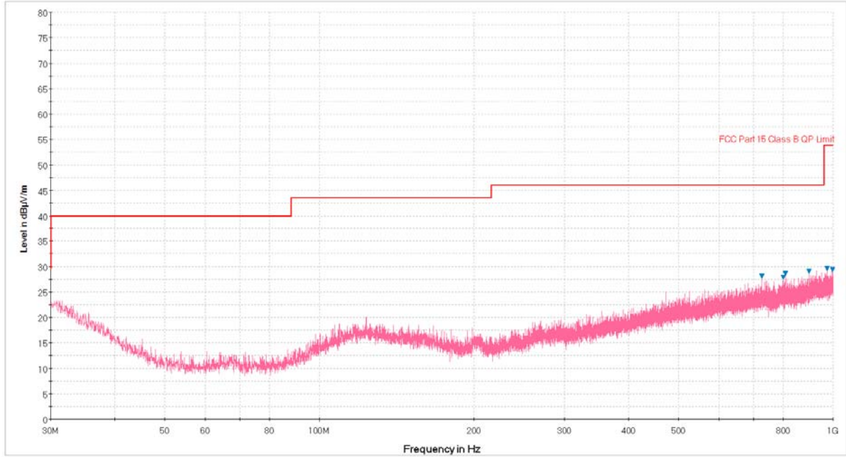
Plot 6-28. Radiated Spurious Plot below 1GHz (Pol. H)
