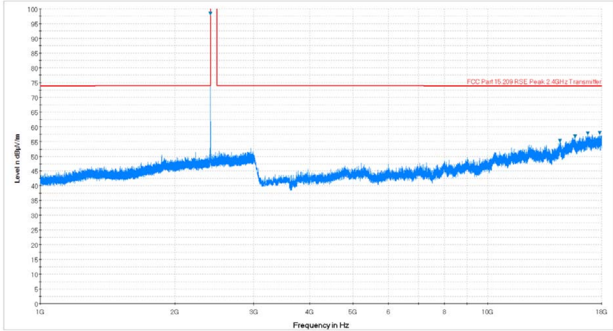
Plot 6-18. Radiated Spurious Plot above 1GHz (BTLE – Ch. 0, Ant. Pol. H)
