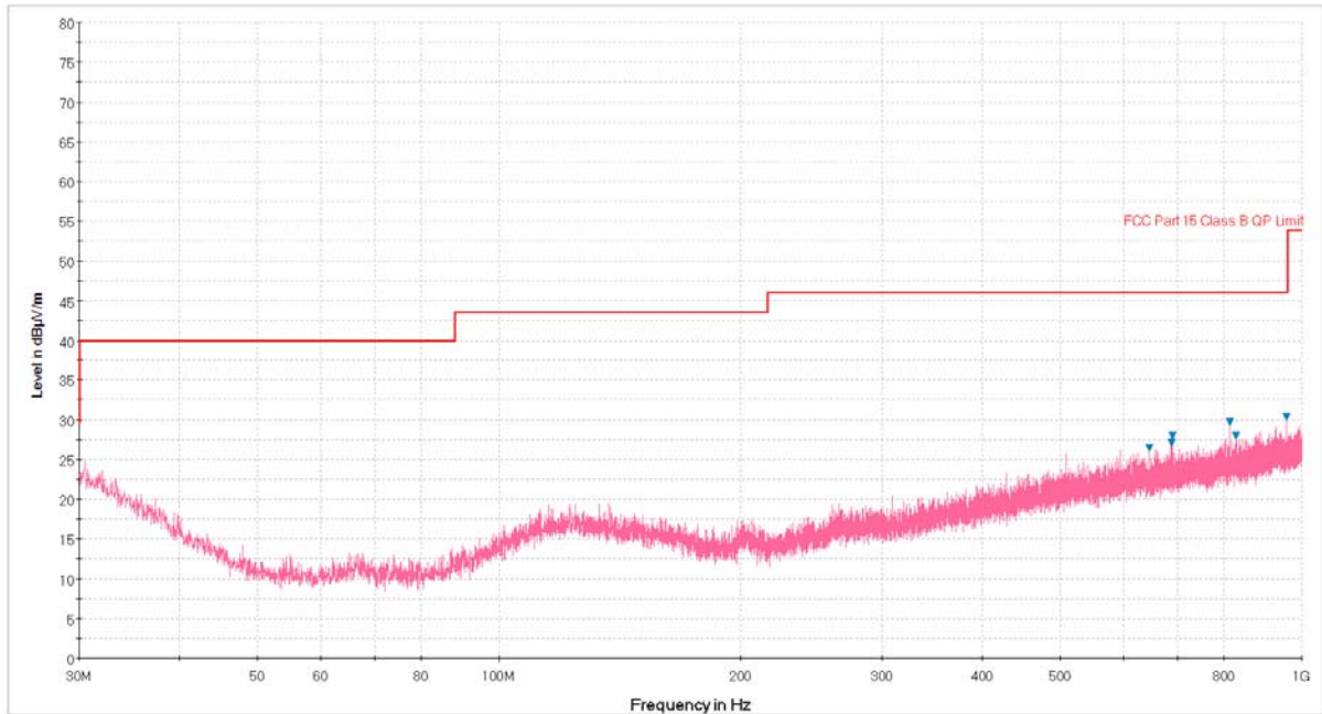
Plot 6-29. Radiated Spurious Plot below 1GHz (Pol. V)
