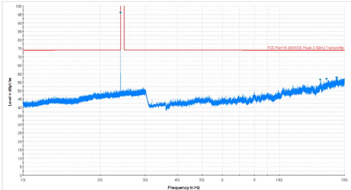
Plot 6-19. Radiated Spurious Plot above 1GHz (BTLE – Ch. 0, Ant. Pol. V)
