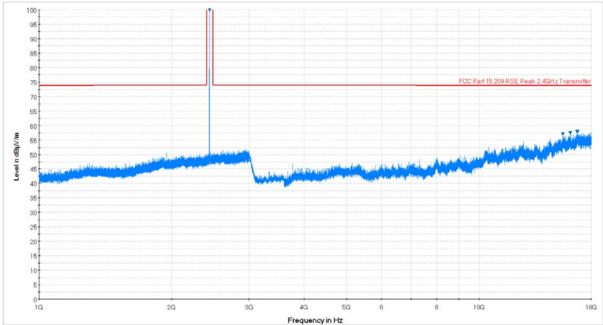
Plot 6-21. Radiated Spurious Plot above 1GHz (BTLE – Ch. 19, Ant. Pol. V)
