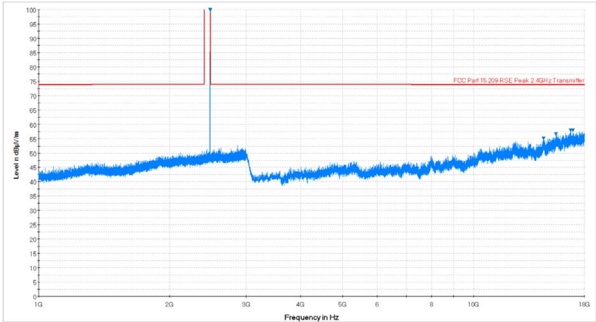
Plot 6-23. Radiated Spurious Plot above 1GHz (BTLE – Ch. 39, Ant. Pol. V)
