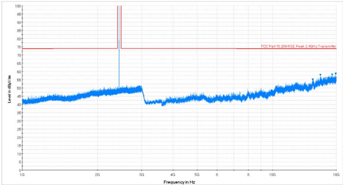
Plot 6-20. Radiated Spurious Plot above 1GHz (BTLE – Ch. 19, Ant. Pol. H)
