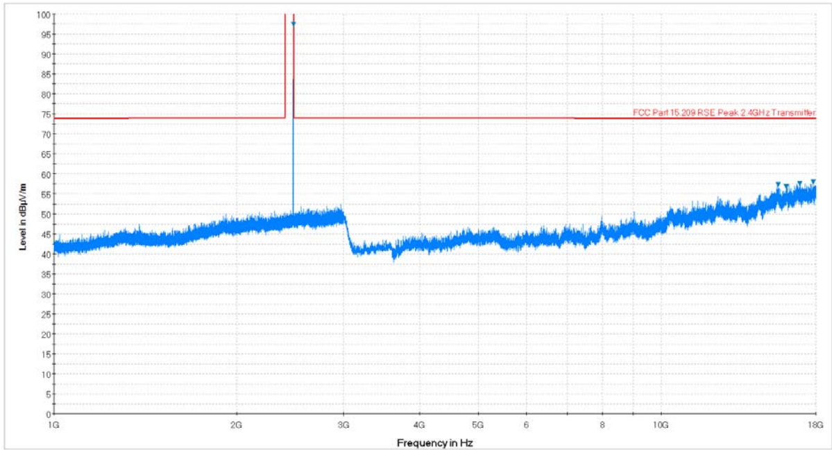
Plot 6-22. Radiated Spurious Plot above 1GHz (BTLE – Ch. 39, Ant. Pol. H)
