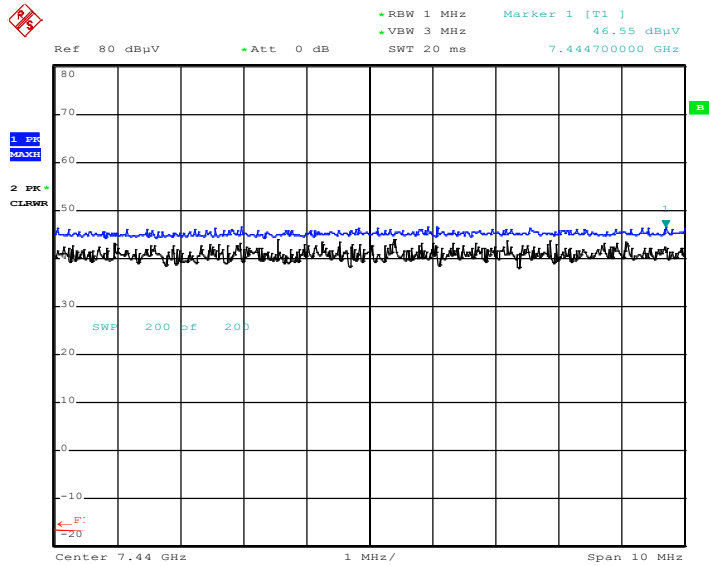
Radiated Spurious Emissions plot – Peak Reading (Ch.78 3rd Harmonic)
