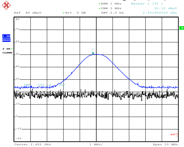
Fundamental Field Strength plot (Ch.0)
