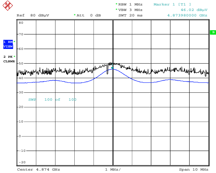
Radiated Spurious Emissions plot – Average Reading (802.11b, Ch.6 2nd Harmonic) [Ant1]
