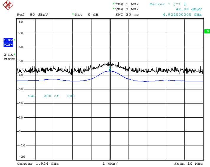
Radiated Spurious Emissions plot – Average Reading (802.11b, Ch.11 2nd Harmonic) [RSDB]
