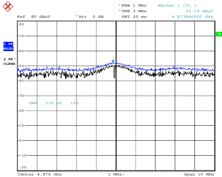
Radiated Spurious Emissions plot – Peak Reading (802.11b, Ch.6 2nd Harmonic) [Ant1]
