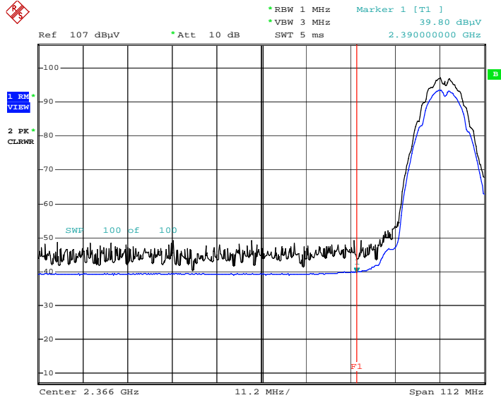
Radiated Restricted Band Edges plot – Average Reading (802.11b Ch.1) [Ant1]
