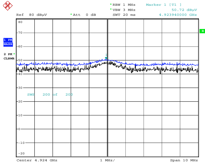
Radiated Spurious Emissions plot – Peak Reading (802.11b, Ch.11 2nd Harmonic) [RSDB]
