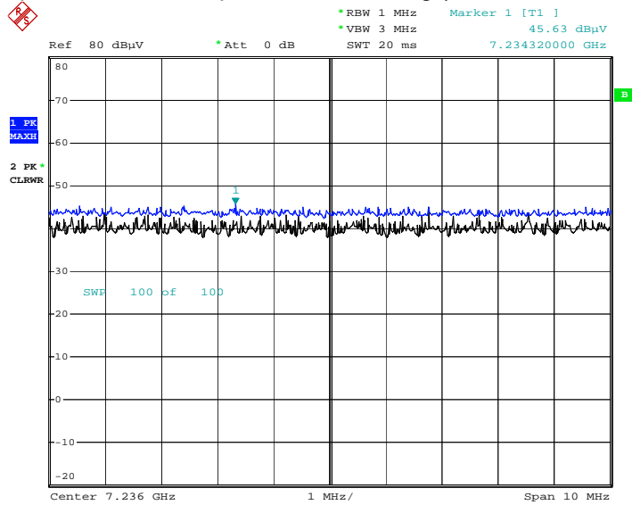
Radiated Spurious Emissions plot – Peak Reading (802.11b, Ch.1 3rd Harmonic) [Ant2]
