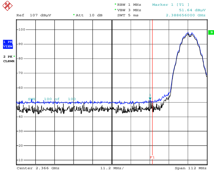
Radiated Restricted Band Edges plot – Peak Reading (802.11b Ch.1) [Ant1]
