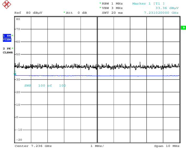
Radiated Spurious Emissions plot – Average Reading (802.11b, Ch.1 3rd Harmonic) [Ant2]
