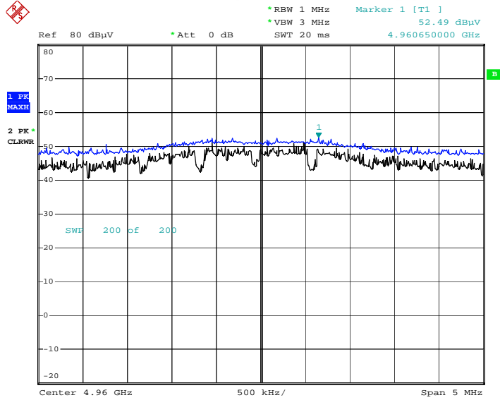
Radiated Spurious Emissions plot – Peak Reading (Ch.39 2nd Harmonic)
