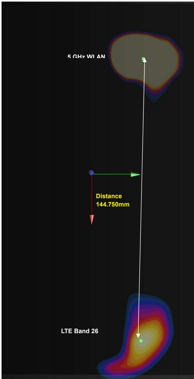
Plot: #7 Phablet SAR Rear Side: LTE Band 26 & 5GHz WLAN
