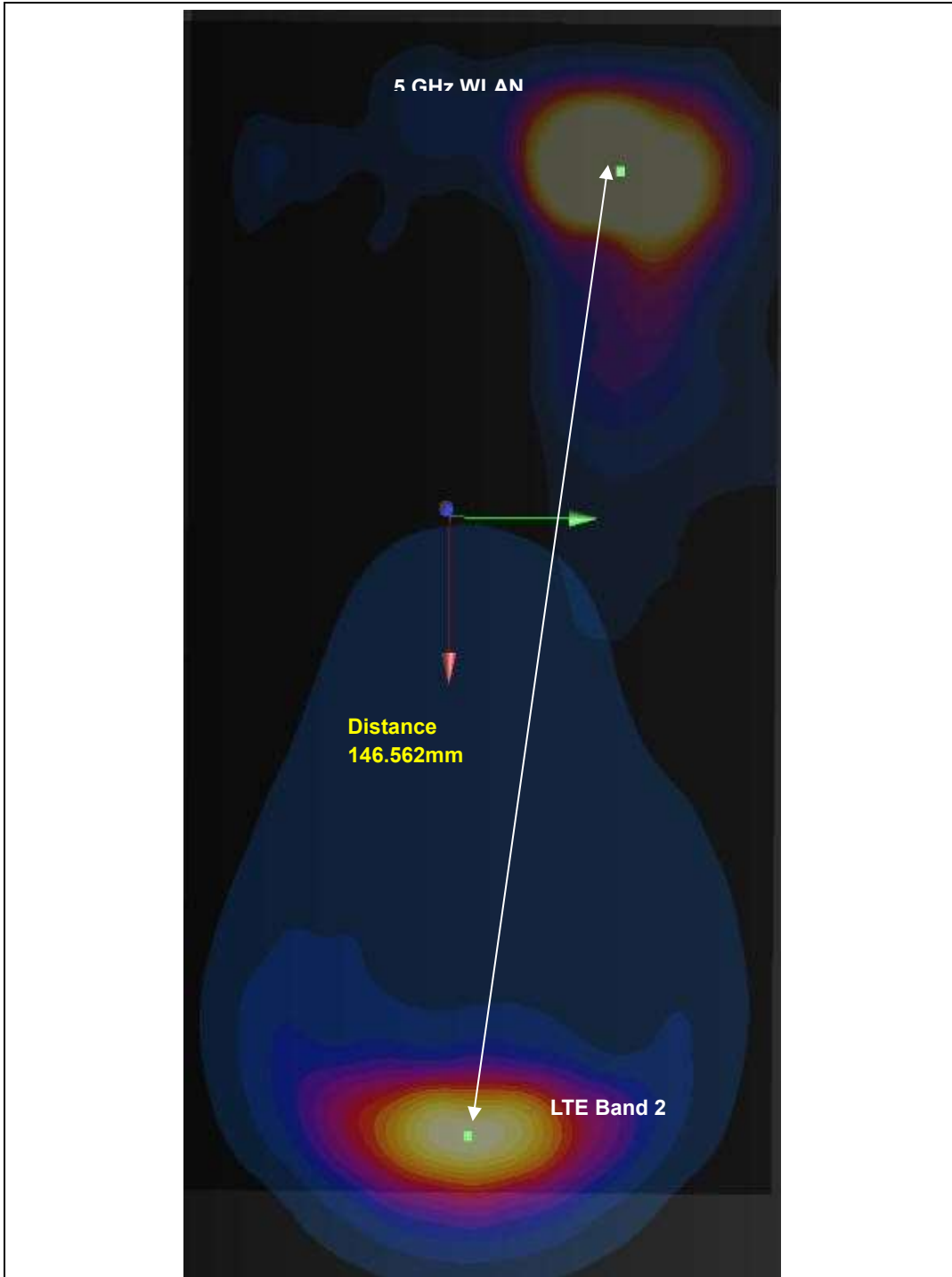
Plot: #5 Phablet SAR Rear Side: LTE Band 2 & 5GHz WLAN
