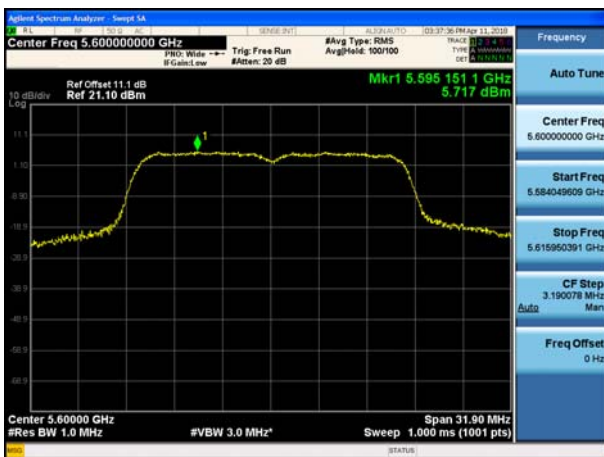
802.11n_HT20 UNII 2C BAND PSD CH 120
