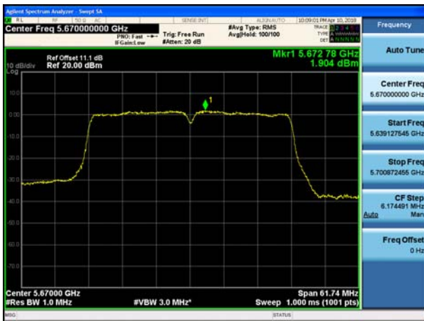
802.11n_HT40 UNII 2C BAND PSD CH 134
