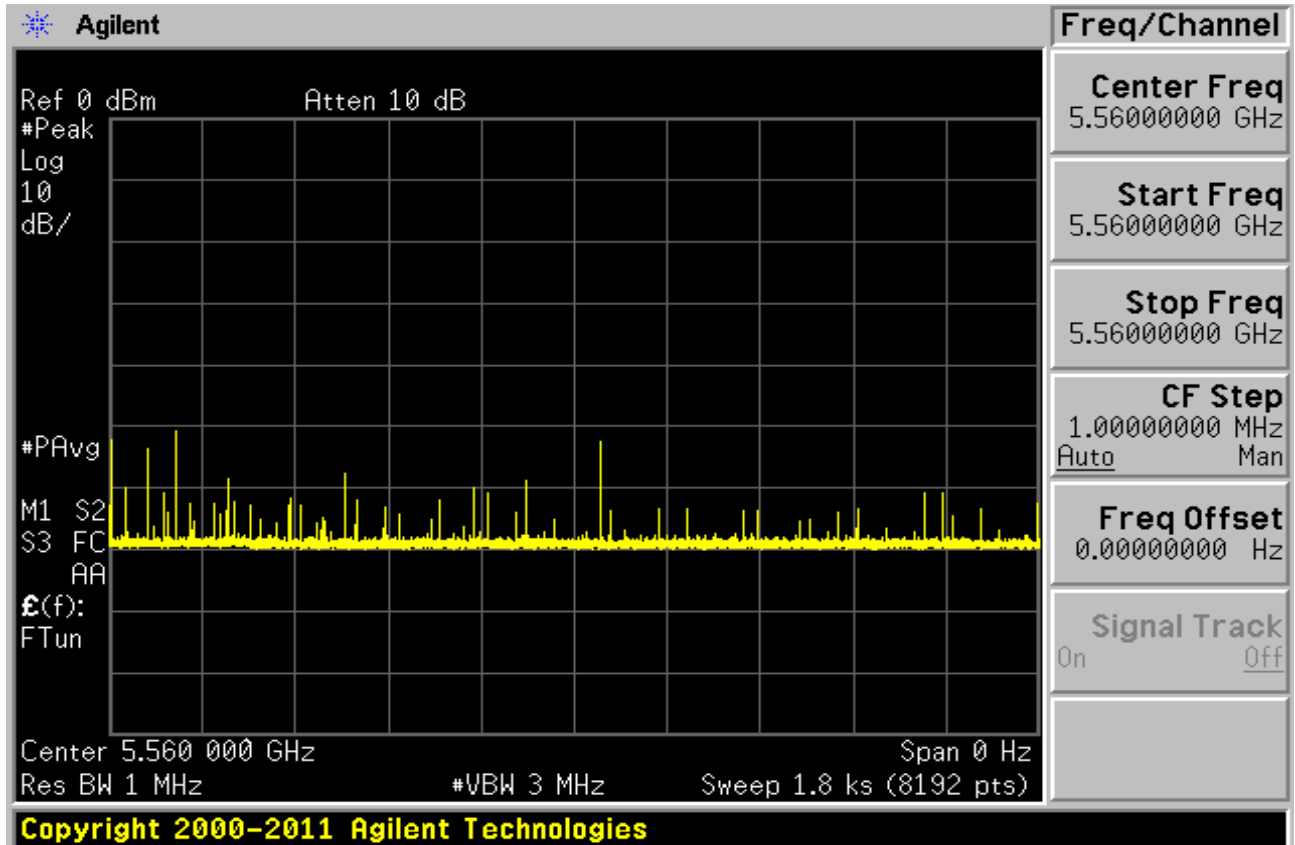
Figure 5-4. Band 2C Non-occupancy Period - Monitoring live spectrum - Elapse time 30 minutes
