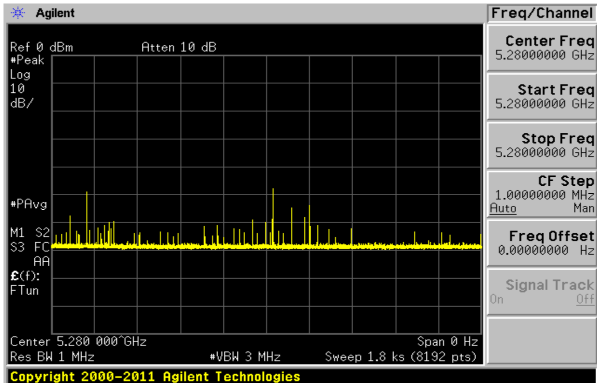
Figure 5-3. Band 2A Non-occupancy Period - Monitoring live spectrum - Elapse time 30 minutes
