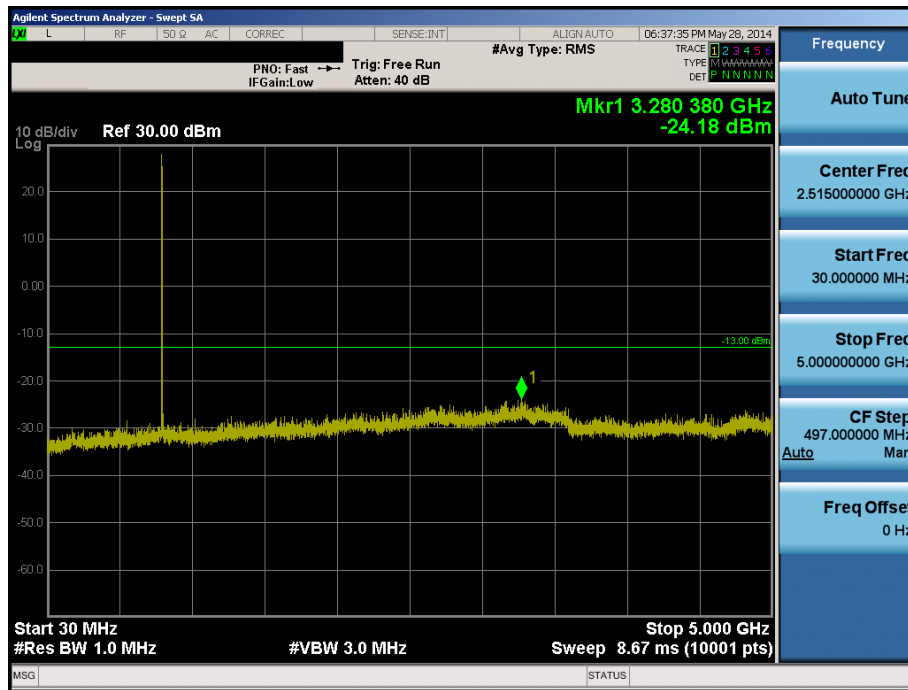
Plot 8-1. Conducted Spurious Plot (1.4MHz QPSK – RB Size 1, RB Offset 0 – Low Channel)
