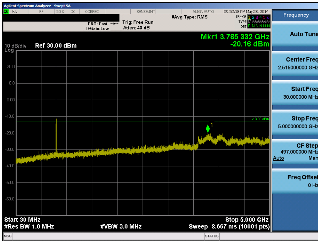
Plot 7-1. Conducted Spurious Plot (Ch. 476)
