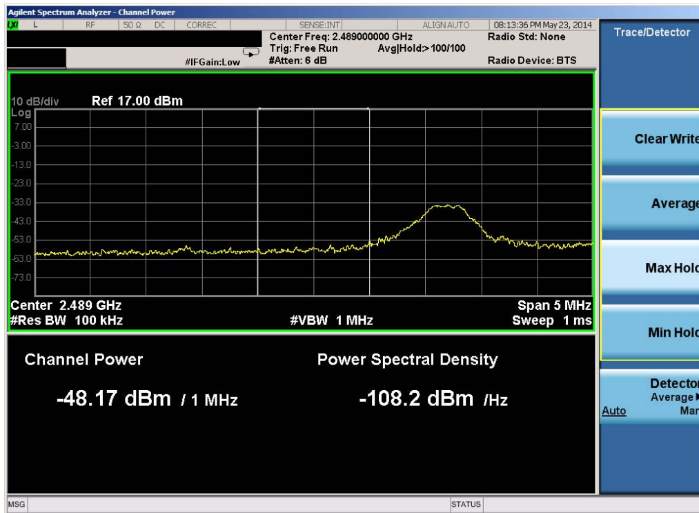
Plot 6-42. Lower Band Edge Plot 1 MHz Integration (Band 41 - 5 MHz QPSK - RB Size 1, Offset 0)
