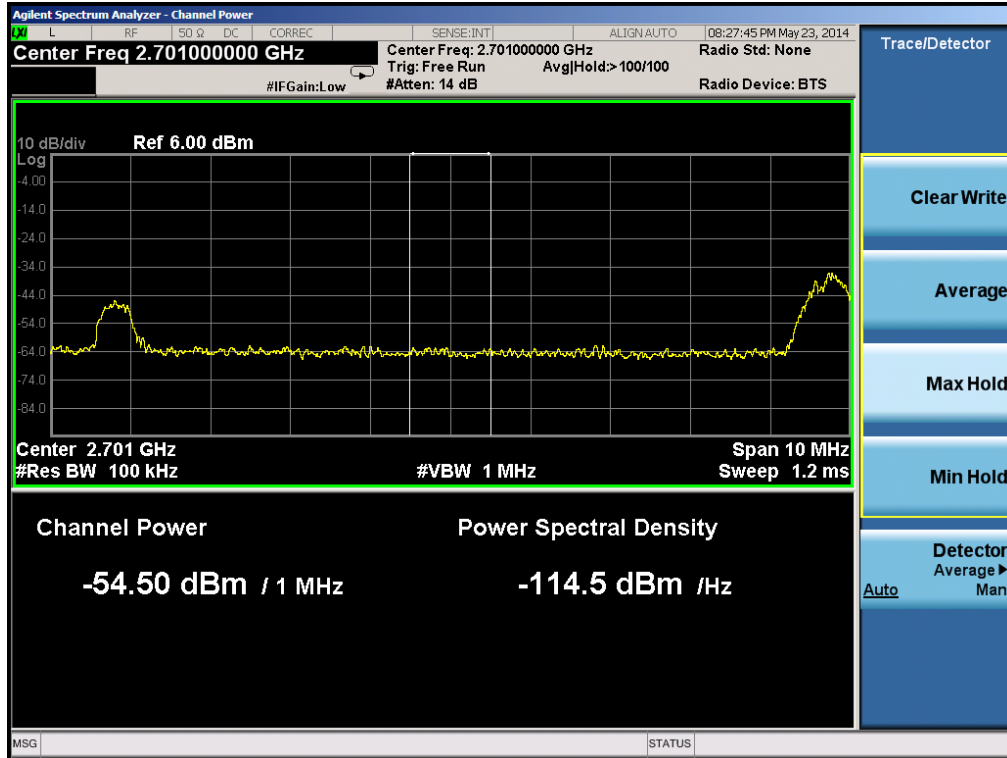
Plot 6-55. Upper Band Edge Plot 1 MHz Integration (Band 41 - 5 MHz QPSK - RB Size 1, Offset 0)
