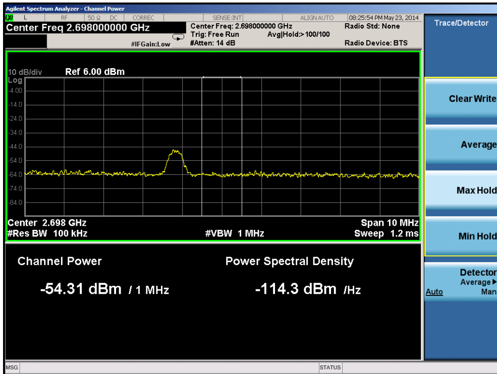
Plot 6-52. Upper Band Edge Plot 1 MHz Integration (Band 41 - 5 MHz QPSK - RB Size 1, Offset 0)
