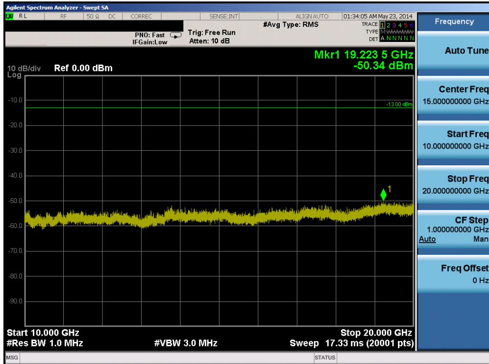
Plot 6-40. Conducted Spurious Plot (Band 25 – 1.4MHz QPSK – RB Size 1, RB Offset 0 – High Channel)
