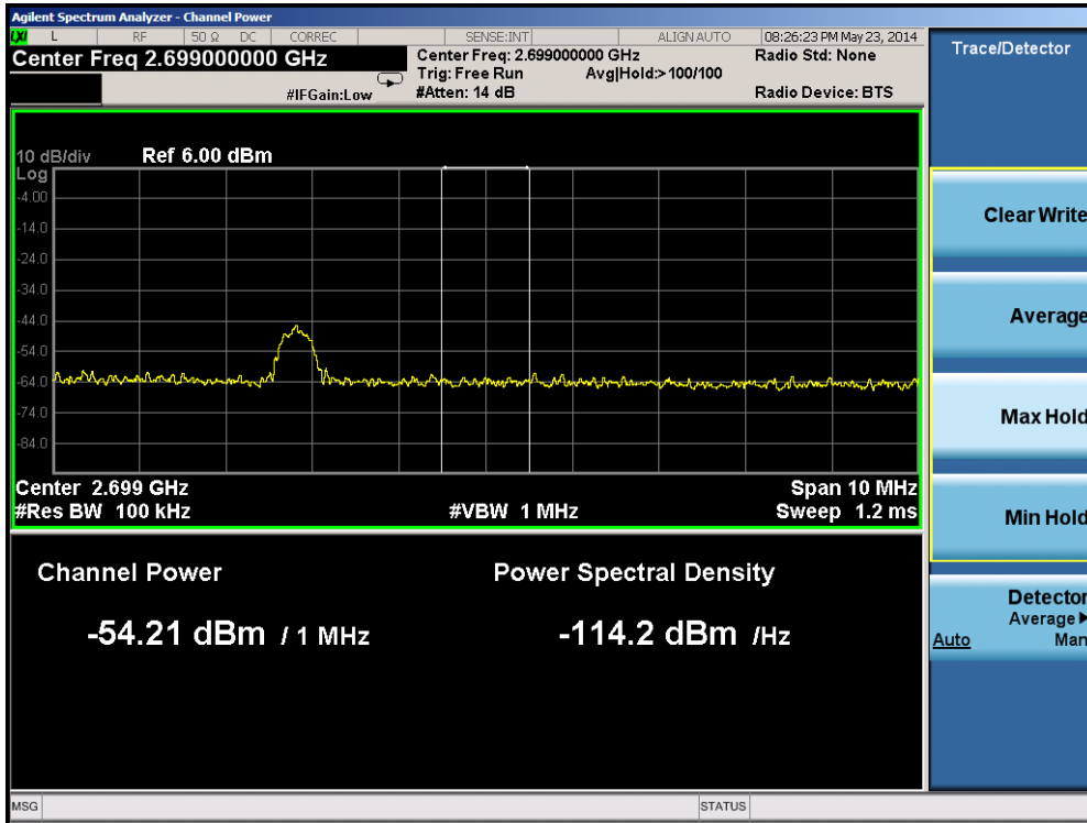
Plot 6-53. Upper Band Edge Plot 1 MHz Integration (Band 41 - 5 MHz QPSK - RB Size 1, Offset 0)
