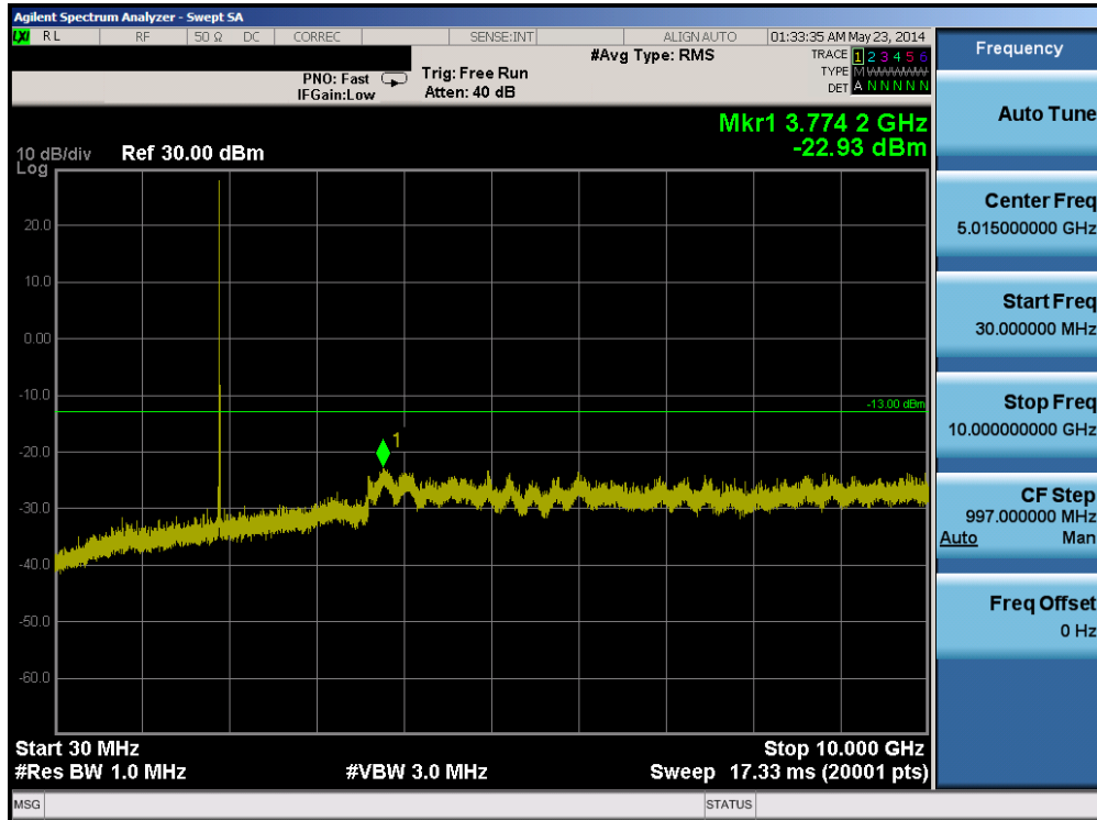
Plot 6-39. Conducted Spurious Plot (Band 25 – 1.4MHz QPSK – RB Size 1, RB Offset 0 – High Channel)
