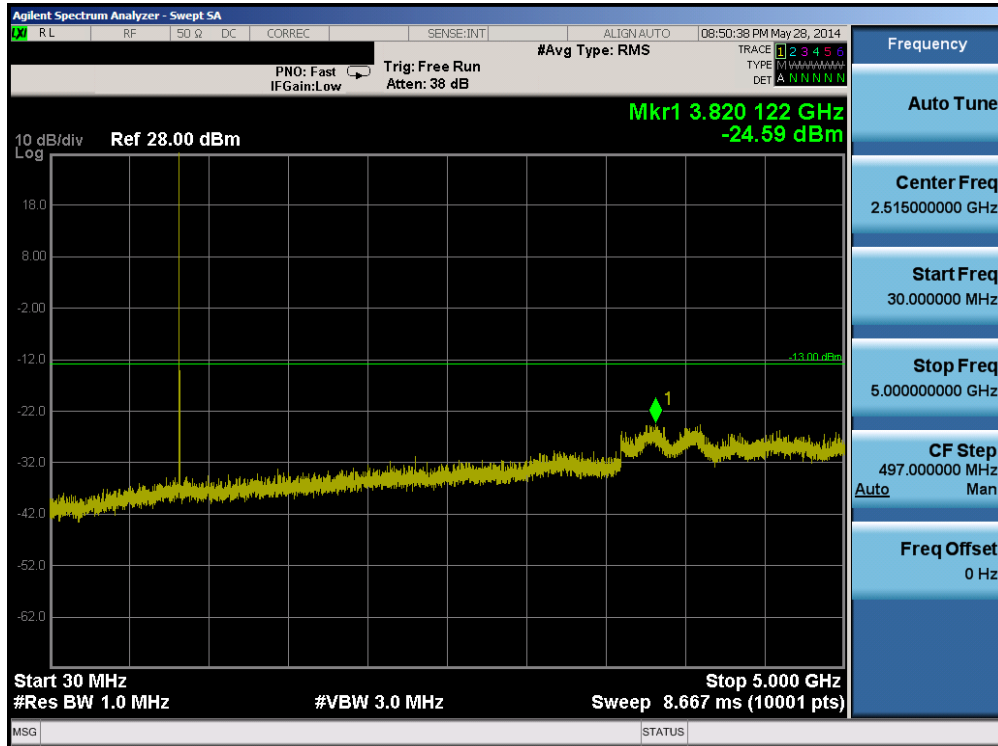
Plot 6-31. Conducted Spurious Plot (Band 26 – 3.0MHz QPSK – RB Size 1, RB Offset 0 – Mid Channel)
