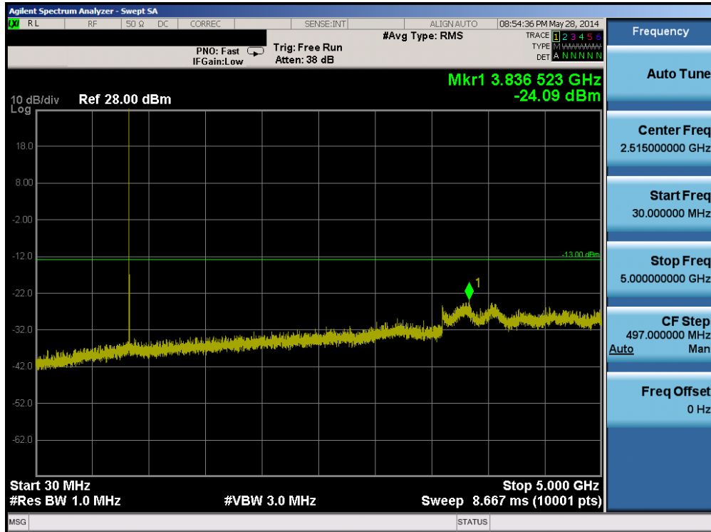
Plot 6-33. Conducted Spurious Plot (Band 26 – 3.0MHz QPSK – RB Size 1, RB Offset 0 – High Channel)
