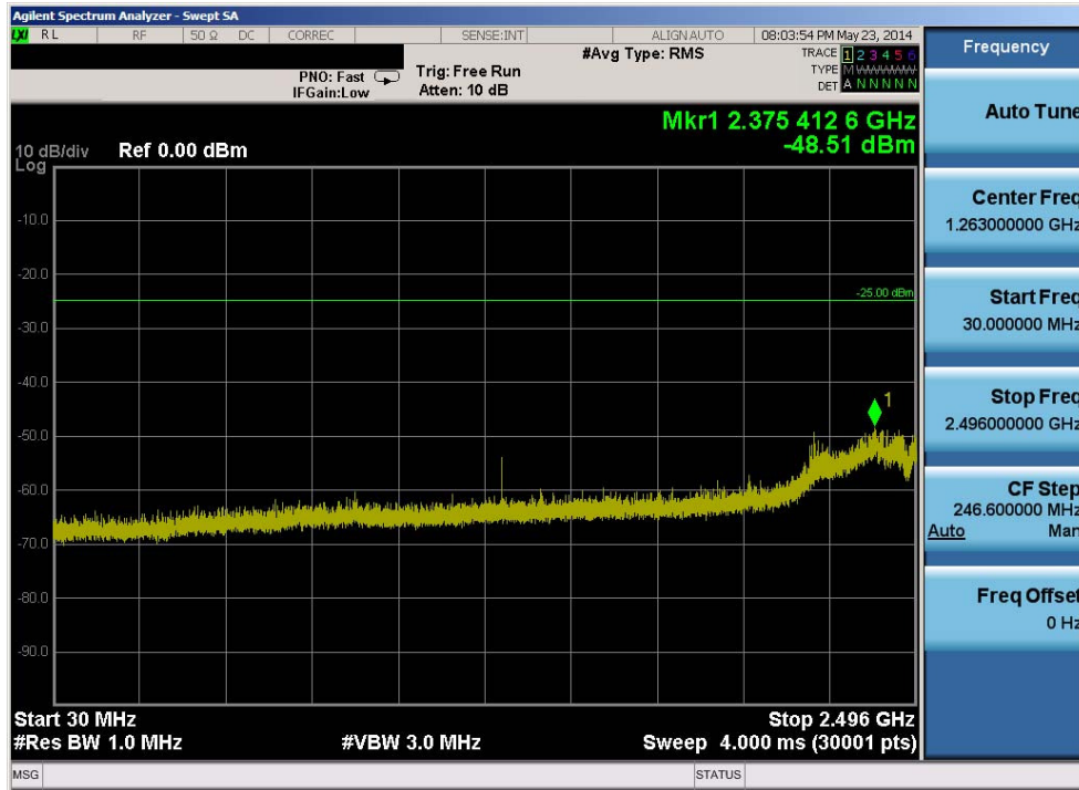
Plot 6-47. Conducted Spurious Plot (Band 41 – 5.0MHz QPSK – RB Size 1, RB Offset 0 – Mid Channel)
