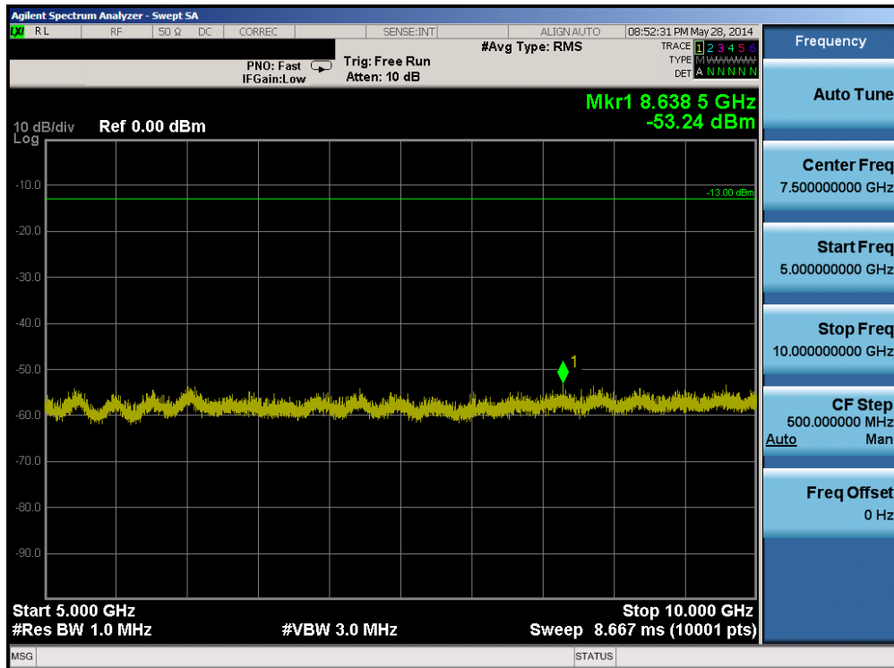
Plot 6-30. Conducted Spurious Plot (Band 26 – 3.0MHz QPSK – RB Size 1, RB Offset 0 – Low Channel)
