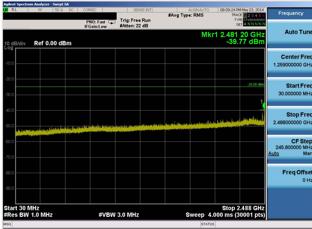
Plot 6-41. Conducted Spurious Plot (Band 41 – 5.0MHz QPSK – RB Size 1, RB Offset 0 – Low Channel)
