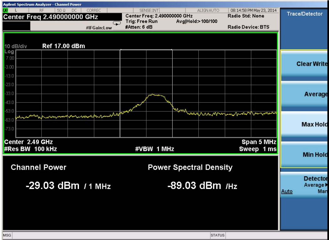
Plot 6-43. Lower Band Edge Plot 1 MHz Integration (Band 41 - 5 MHz QPSK - RB Size 1, Offset 0)
