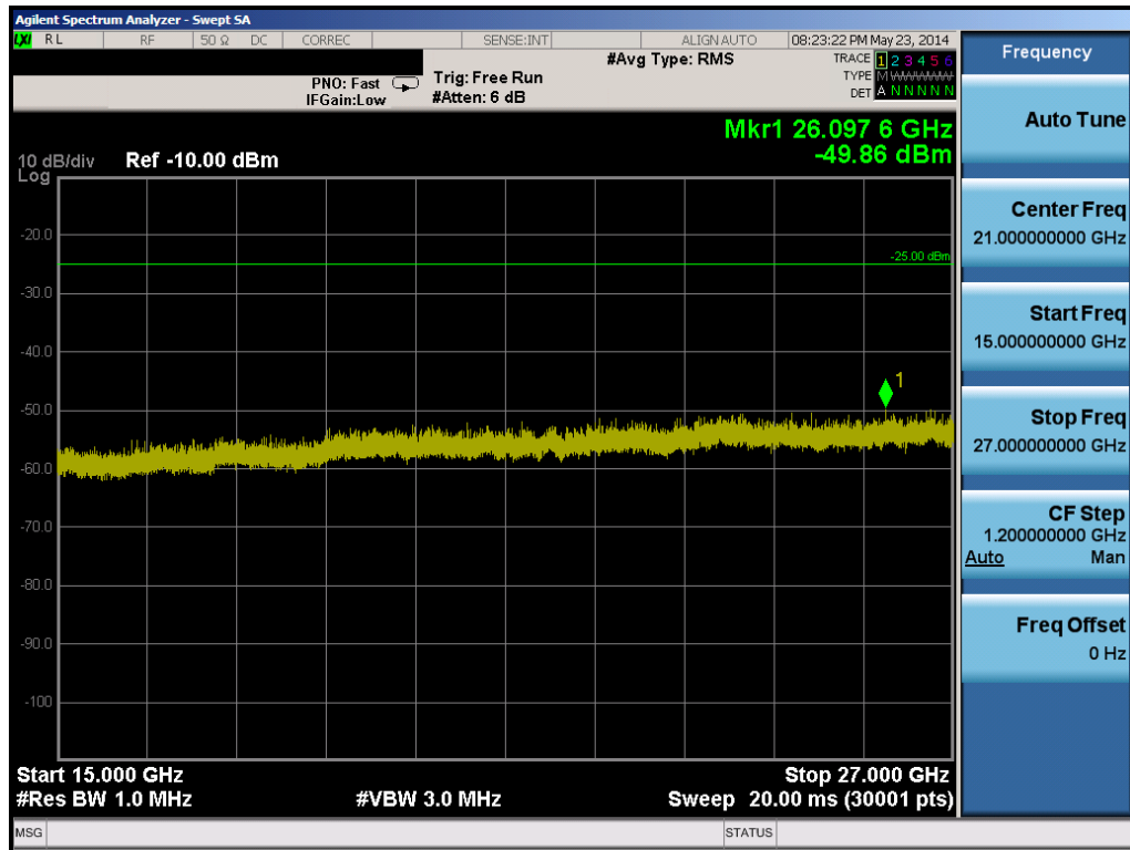
Plot 6-58. Conducted Spurious Plot (Band 41 – 5.0MHz QPSK – RB Size 1, RB Offset 0 – High Channel)
