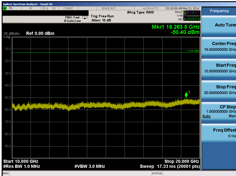
Plot 6-36. Conducted Spurious Plot (Band 25 – 1.4MHz QPSK – RB Size 1, RB Offset 0 – Low Channel)
