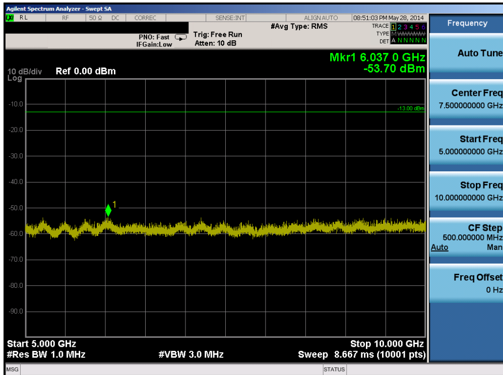
Plot 6-32. Conducted Spurious Plot (Band 26 – 3.0MHz QPSK – RB Size 1, RB Offset 0 – Mid Channel)
