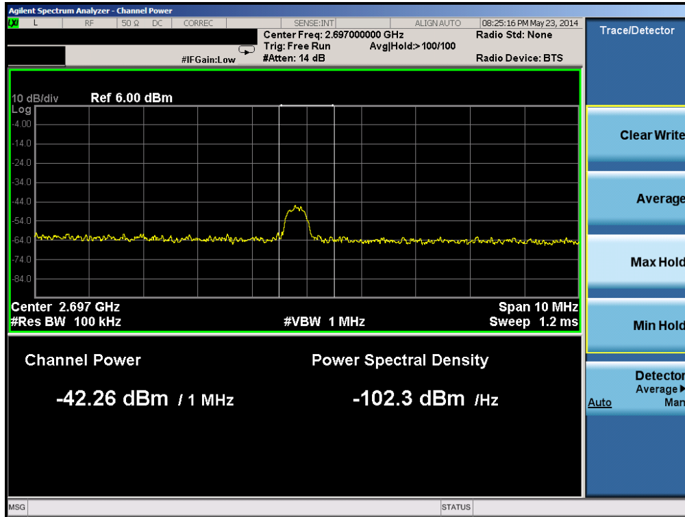
Plot 6-51. Upper Band Edge Plot 1 MHz Integration (Band 41 - 5 MHz QPSK - RB Size 1, Offset 0)
