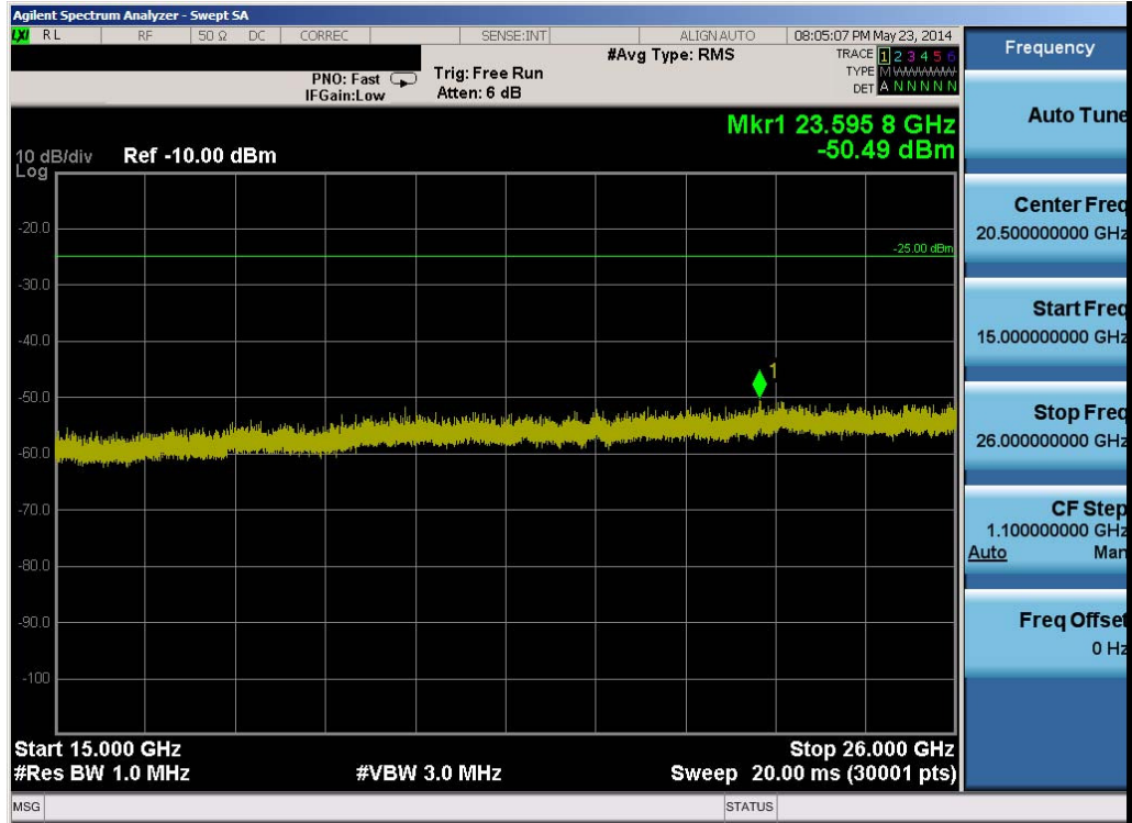
Plot 6-49. Conducted Spurious Plot (Band 41 – 5.0MHz QPSK – RB Size 1, RB Offset 0 – Mid Channel)
