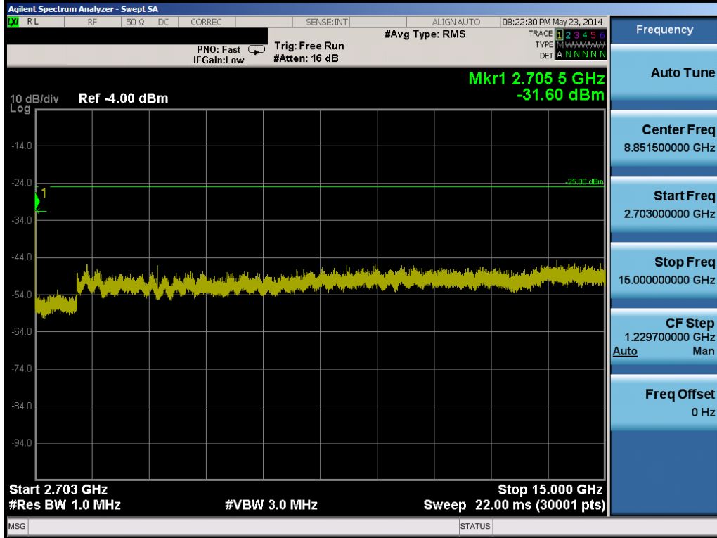
Plot 6-57. Conducted Spurious Plot (Band 41 – 5.0MHz QPSK – RB Size 1, RB Offset 0 – High Channel)
