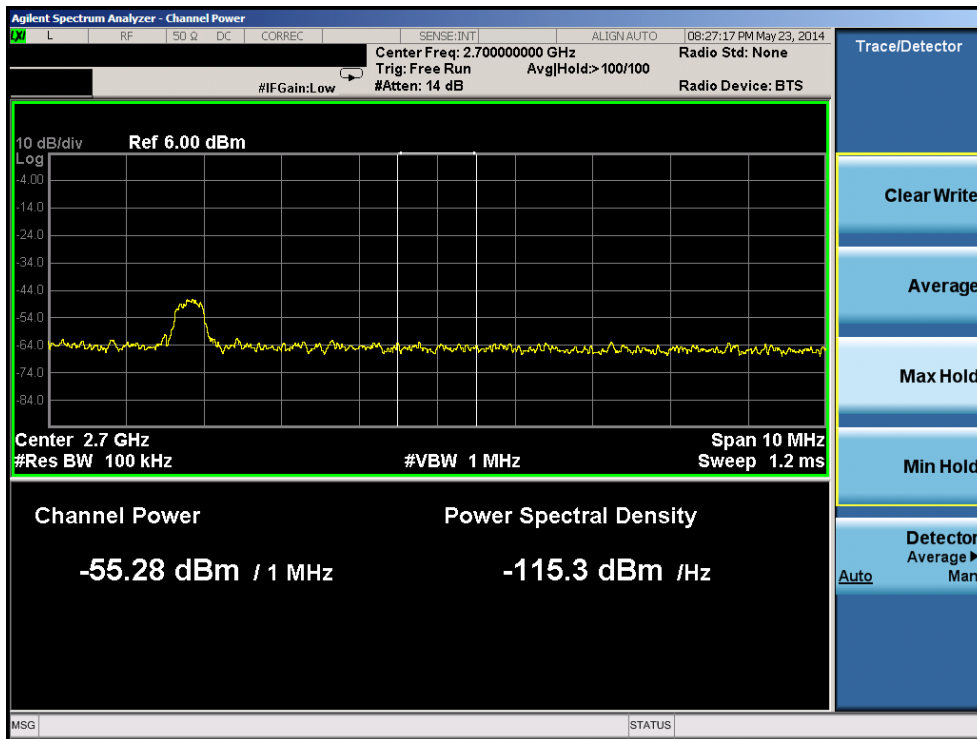
Plot 6-54. Upper Band Edge Plot 1 MHz Integration (Band 41 - 5 MHz QPSK - RB Size 1, Offset 0)
