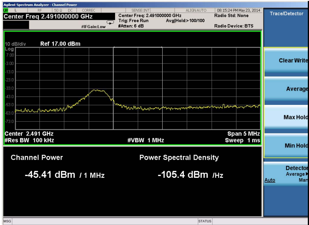
Plot 6-44. Lower Band Edge Plot 1 MHz Integration (Band 41 - 5 MHz QPSK - RB Size 1, Offset 0)
