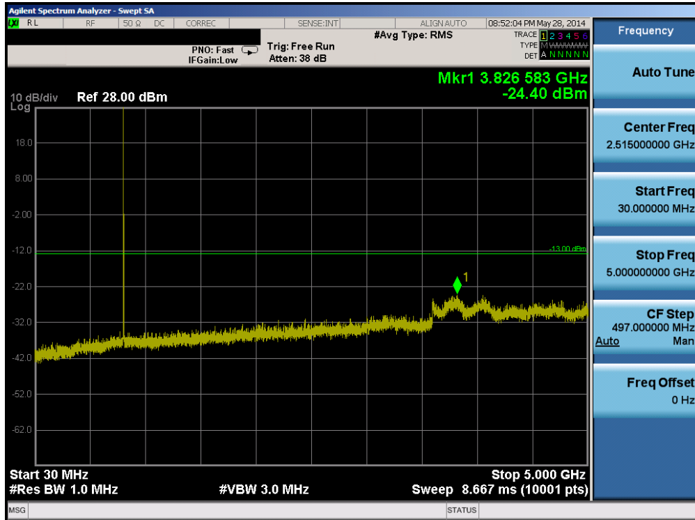
Plot 6-29. Conducted Spurious Plot (Band 26 – 3.0MHz QPSK – RB Size 1, RB Offset 0 – Low Channel)
