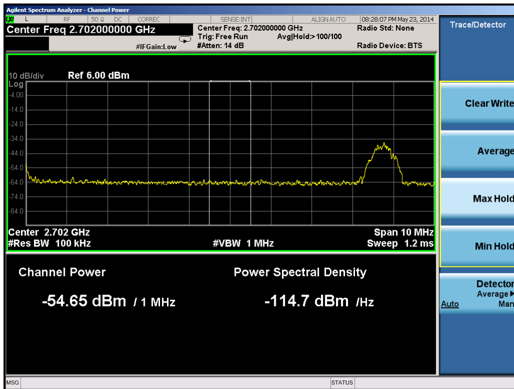
Plot 6-56. Upper Band Edge Plot 1 MHz Integration (Band 41 - 5 MHz QPSK - RB Size 1, Offset 0)
