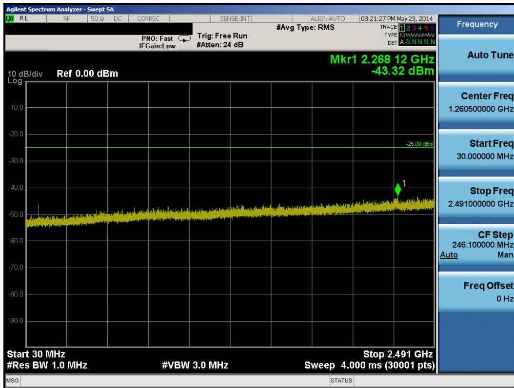
Plot 6-50. Conducted Spurious Plot (Band 41 – 5.0MHz QPSK – RB Size 1, RB Offset 0 – High Channel)
