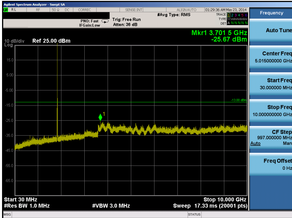
Plot 6-35. Conducted Spurious Plot (Band 25 – 1.4MHz QPSK – RB Size 1, RB Offset 0 – Low Channel)
