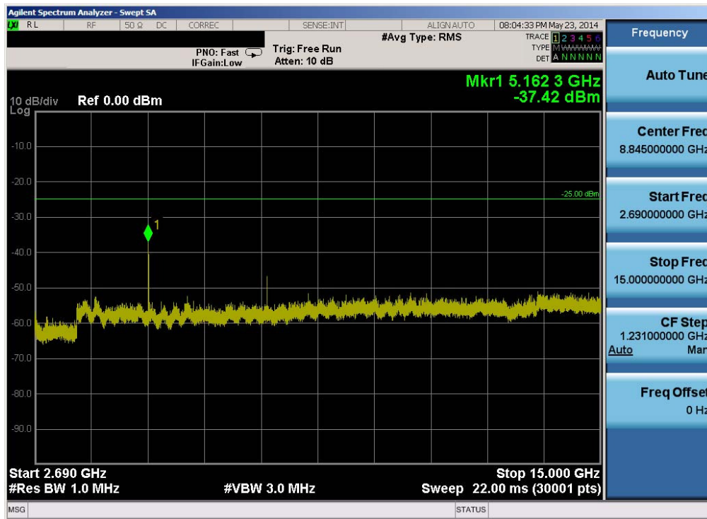
Plot 6-48. Conducted Spurious Plot (Band 41 – 5.0MHz QPSK – RB Size 1, RB Offset 0 – Mid Channel)
