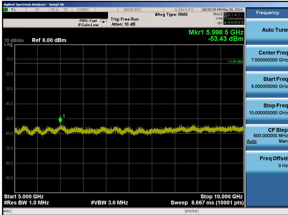
Plot 6-34. Conducted Spurious Plot (Band 26 – 3.0MHz QPSK – RB Size 1, RB Offset 0 – High Channel)
