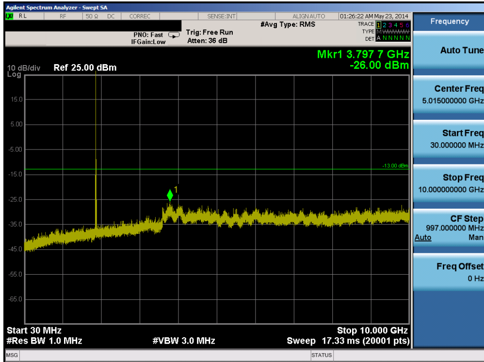
Plot 6-37. Conducted Spurious Plot (Band 25 – 1.4MHz QPSK – RB Size 1, RB Offset 0 – Mid Channel)
