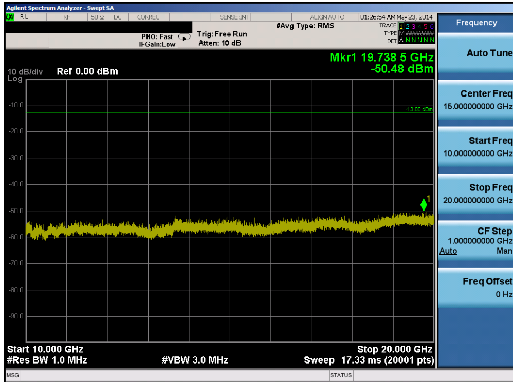
Plot 6-38. Conducted Spurious Plot (Band 25 – 1.4MHz QPSK – RB Size 1, RB Offset 0 – Mid Channel)
