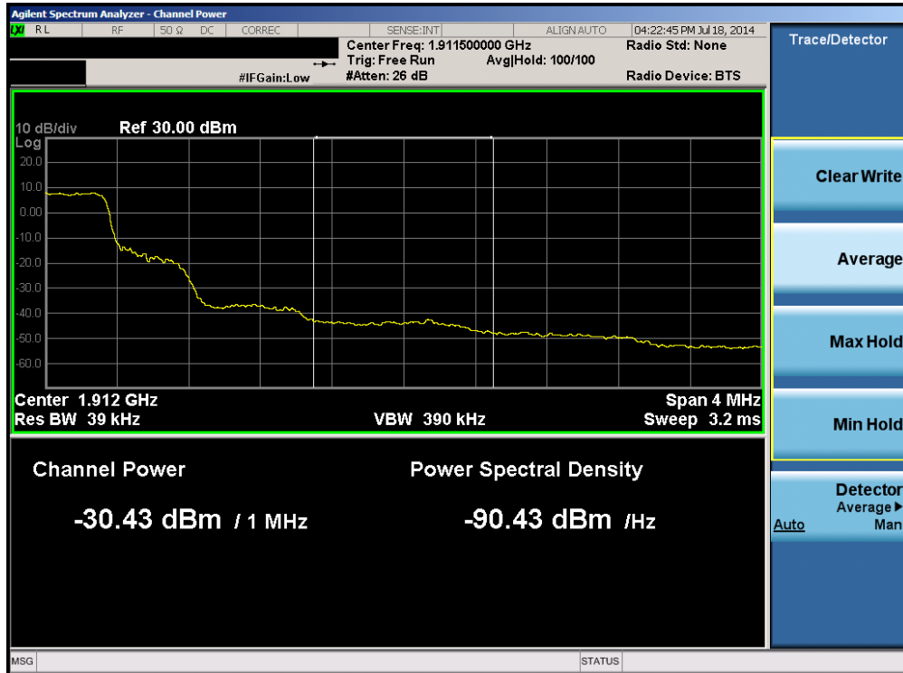
Plot 6-52. Upper Extended Band Edge Plot (Band 2 – 1.4MHz QPSK – RB Size 6)
