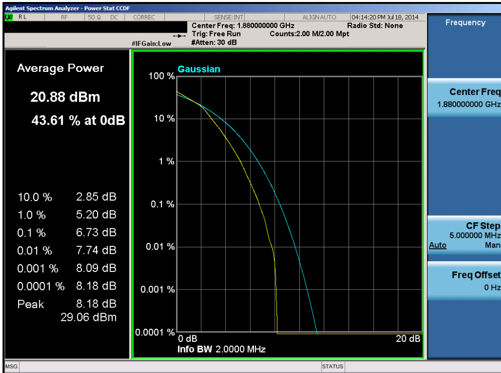
Plot 6-74. PAR Plot (Band 2 – 1.4MHz 16-QAM – RB Size 6)
