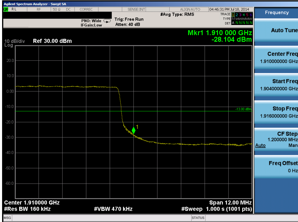
Plot 6-67. Upper Band Edge Plot (Band 2 – 15.0MHz QPSK – RB Size 75)
