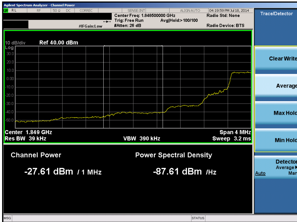
Plot 6-50. Lower Extended Band Edge Plot (Band 2 – 1.4MHz QPSK – RB Size 6)
