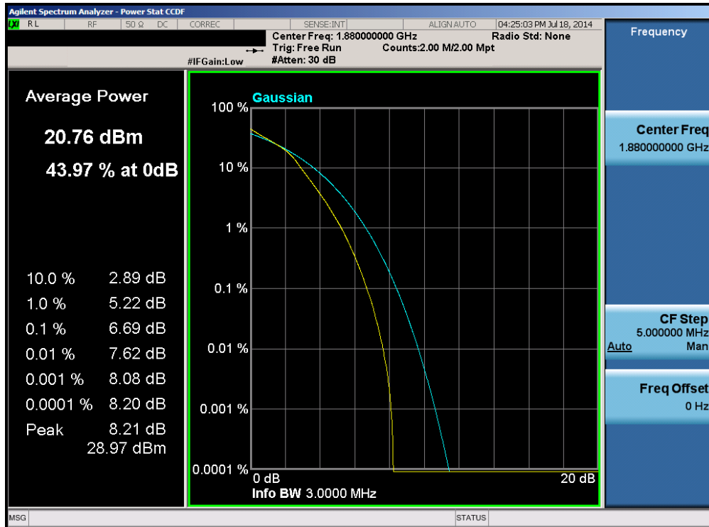
Plot 6-76. PAR Plot (Band 2 – 3.0MHz 16-QAM – RB Size 15)
