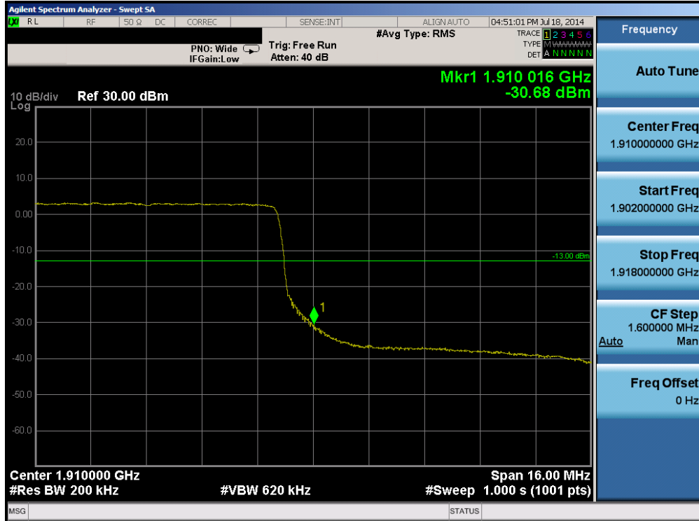
Plot 6-71. Upper Band Edge Plot (Band 2 – 20.0MHz QPSK – RB Size 100)
