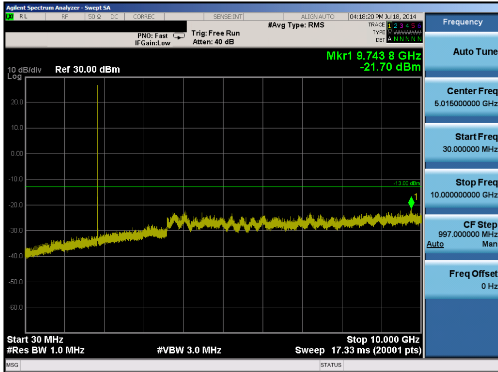
Plot 6-27. Conducted Spurious Plot (Band 2 – 1.4MHz QPSK – RB Size 1, RB Offset 0 – Low Channel)
