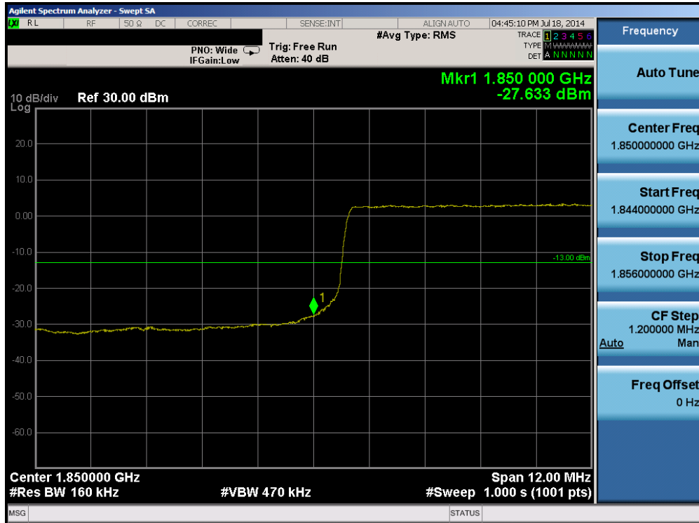
Plot 6-65. Lower Band Edge Plot (Band 2 – 15.0MHz QPSK – RB Size 75)
