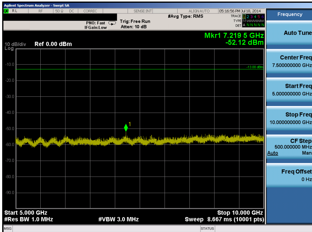
Plot 6-24. Conducted Spurious Plot (Band 5 – 3.0MHz QPSK – RB Size 1, RB Offset 0 – Mid Channel)
