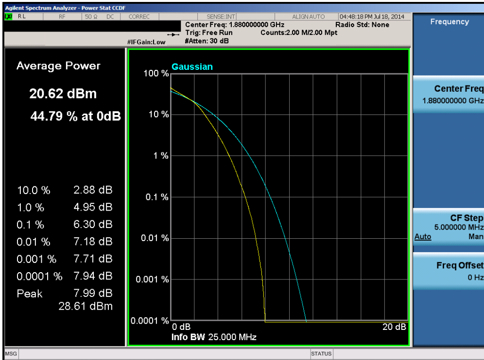
Plot 6-84. PAR Plot (Band 2 – 20.0MHz 16-QAM – RB Size 100)
