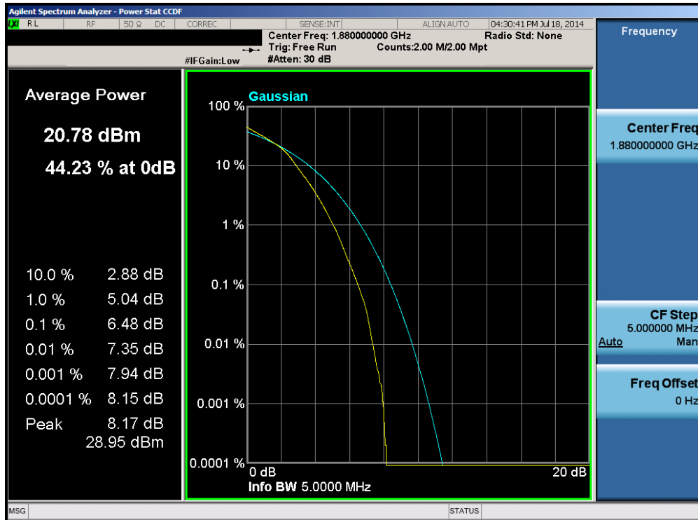
Plot 6-78. PAR Plot (Band 2 – 5.0MHz 16-QAM – RB Size 25)
