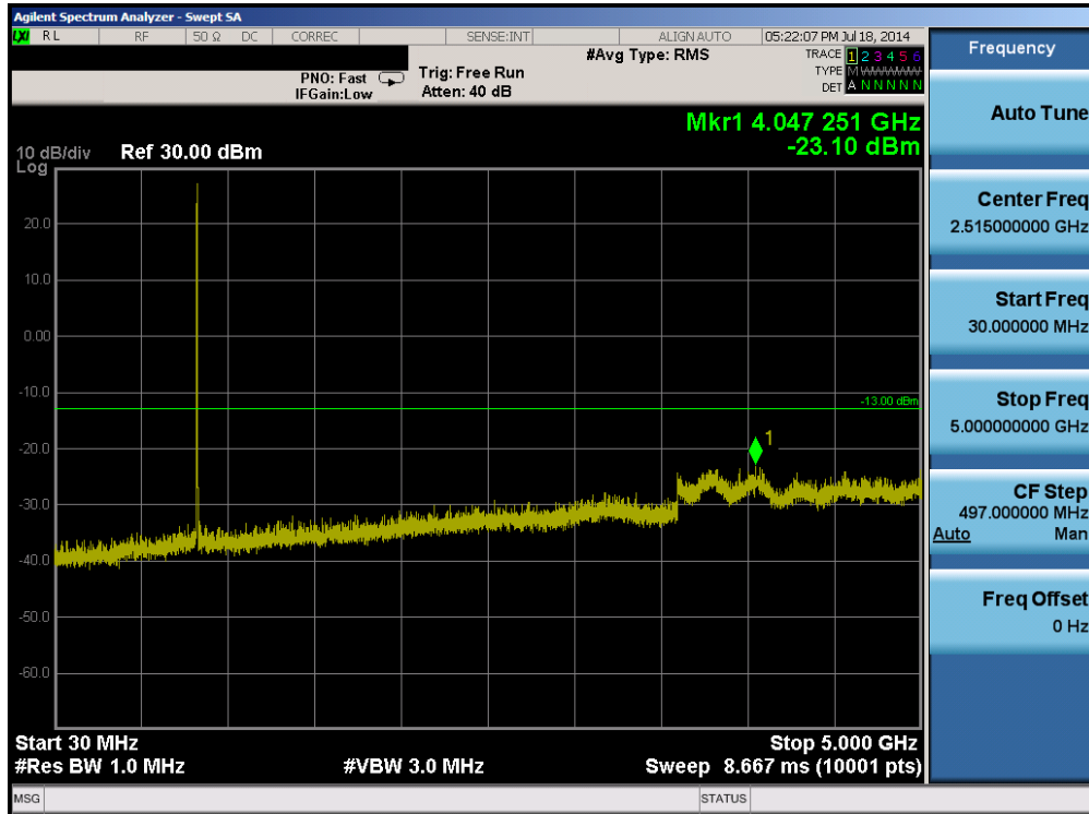
Plot 6-25. Conducted Spurious Plot (Band 5 – 3.0MHz QPSK – RB Size 1, RB Offset 0 – High Channel)
