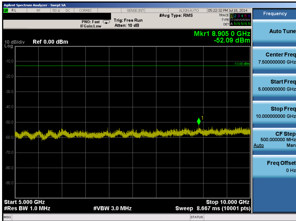
Plot 6-26. Conducted Spurious Plot (Band 5 – 3.0MHz QPSK – RB Size 1, RB Offset 0 – High Channel)
