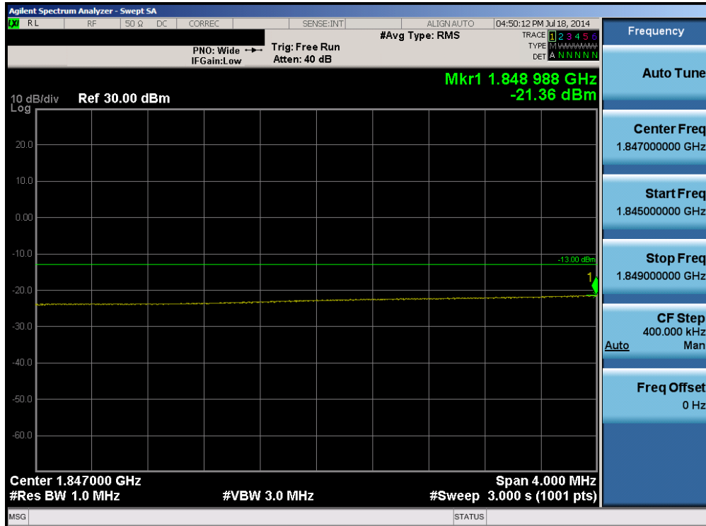
Plot 6-70. Lower Extended Band Edge Plot (Band 2 – 20.0MHz QPSK – RB Size 100)
