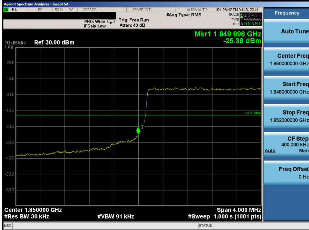
Plot 6-53. Lower Band Edge Plot (Band 2 – 3.0MHz QPSK – RB Size 15)
