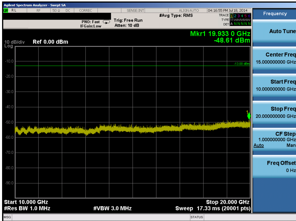
Plot 6-30. Conducted Spurious Plot (Band 2 – 1.4MHz QPSK – RB Size 1, RB Offset 0 – Mid Channel)
