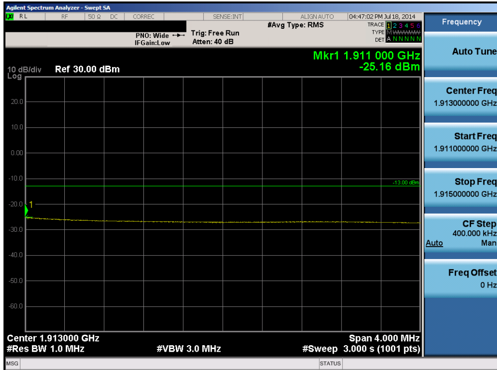
Plot 6-68. Upper Extended Band Edge Plot (Band 2 – 15.0MHz QPSK – RB Size 75)
