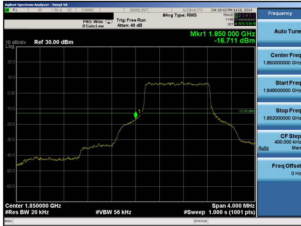
Plot 6-49. Lower Band Edge Plot (Band 2 – 1.4MHz QPSK – RB Size 6)
