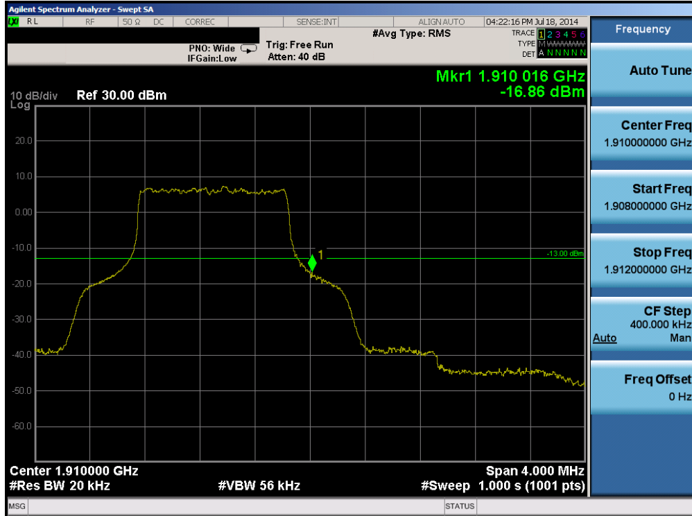
Plot 6-51. Upper Band Edge Plot (Band 2 – 1.4MHz QPSK – RB Size 6)
