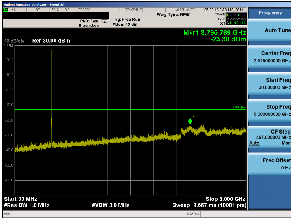
Plot 6-21. Conducted Spurious Plot (Band 5 – 3.0MHz QPSK – RB Size 1, RB Offset 0 – Low Channel)
