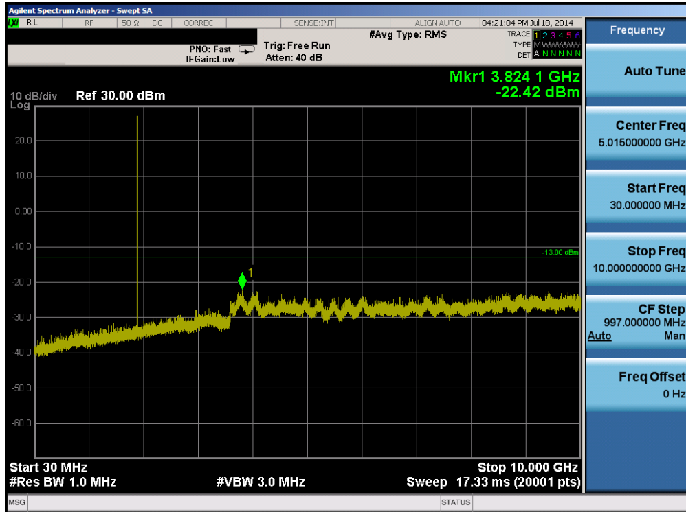
Plot 6-31. Conducted Spurious Plot (Band 2 – 1.4MHz QPSK – RB Size 1, RB Offset 0 – High Channel)
