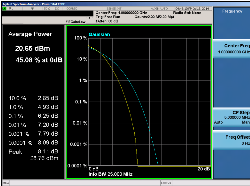
Plot 6-82. PAR Plot (Band 2 – 15.0MHz 16-QAM – RB Size 75)
