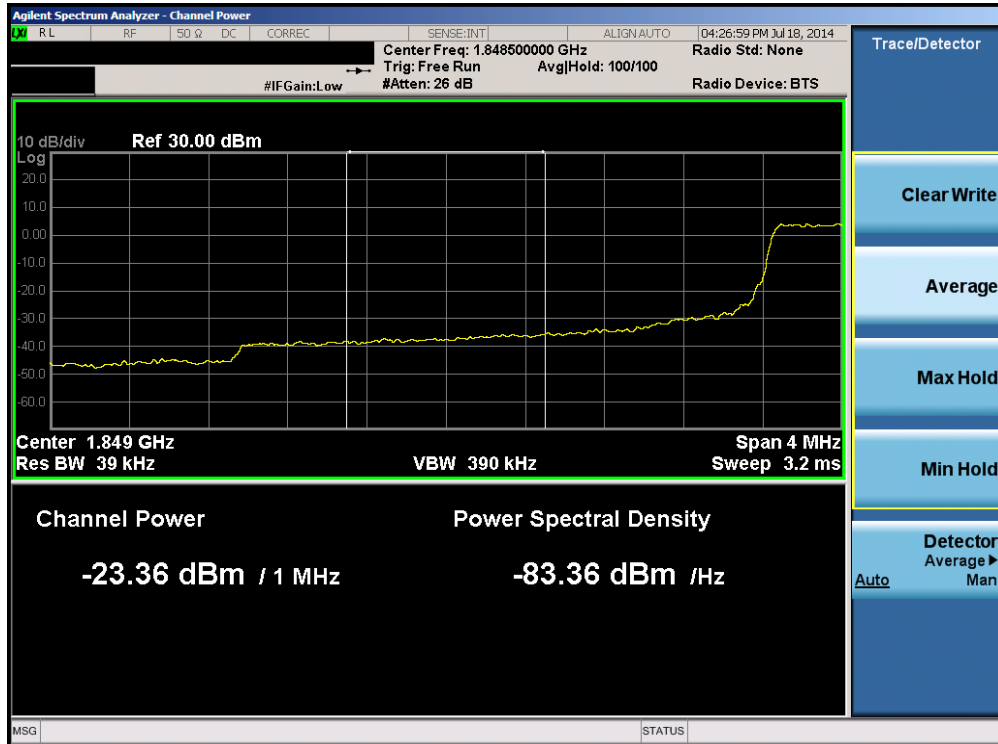
Plot 6-54. Lower Extended Band Edge Plot (Band 2 – 3.0MHz QPSK – RB Size 15)
