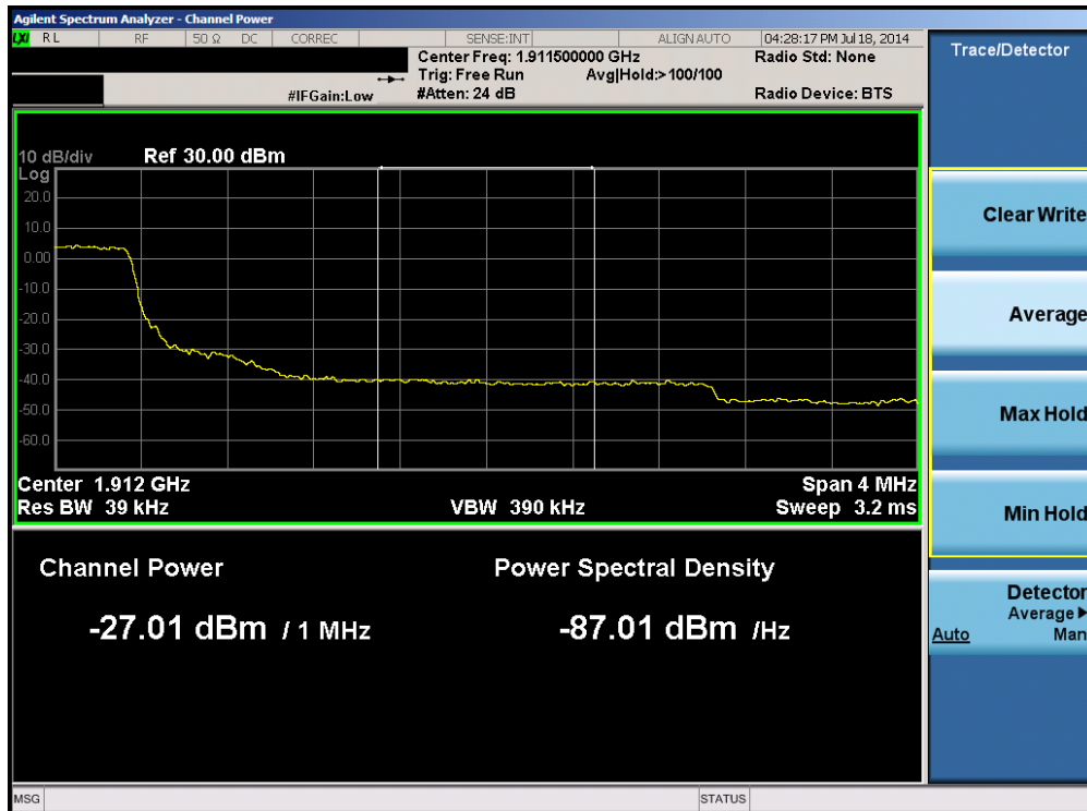
Plot 6-56. Upper Extended Band Edge Plot (Band 2 – 3.0MHz QPSK – RB Size 15)
