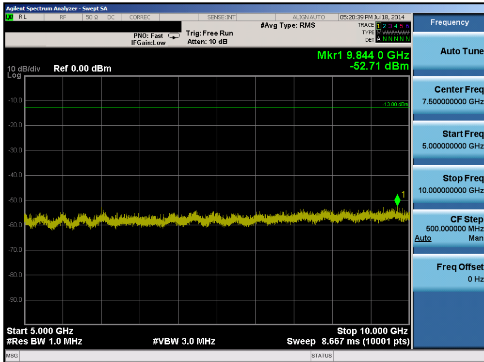
Plot 6-22. Conducted Spurious Plot (Band 5 – 3.0MHz QPSK – RB Size 1, RB Offset 0 – Low Channel)
