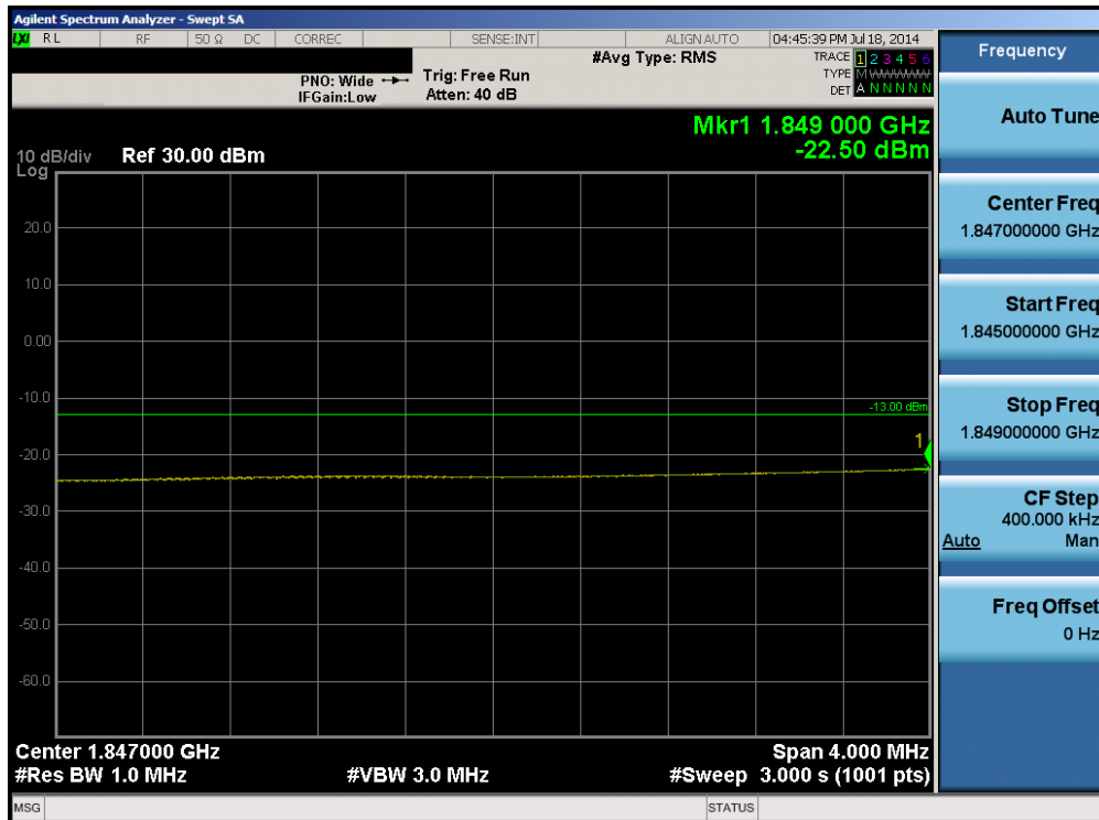
Plot 6-66. Lower Extended Band Edge Plot (Band 2 – 15.0MHz QPSK – RB Size 75)
