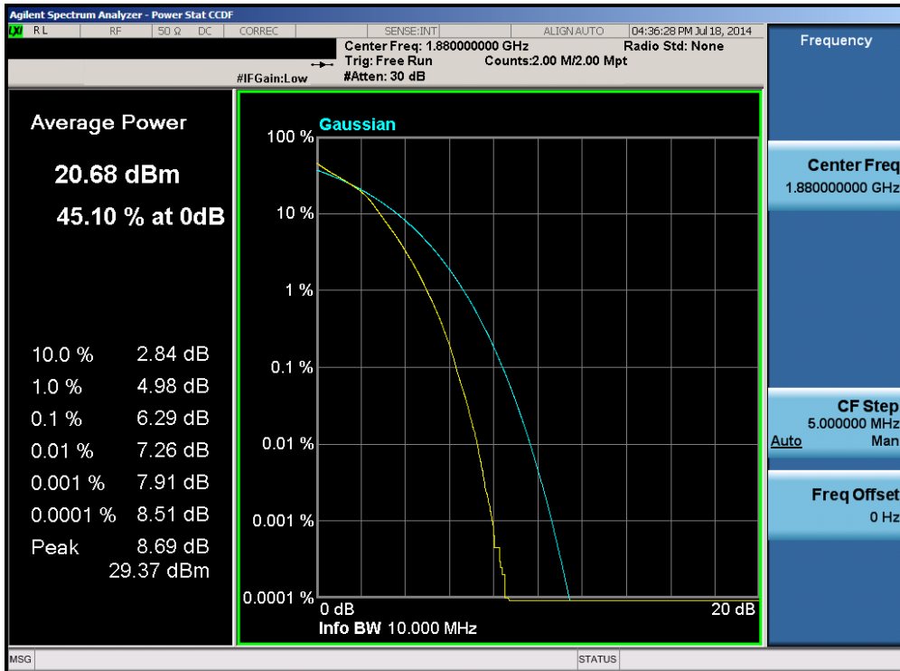
Plot 6-80. PAR Plot (Band 2 – 10.0MHz 16-QAM – RB Size 50)
