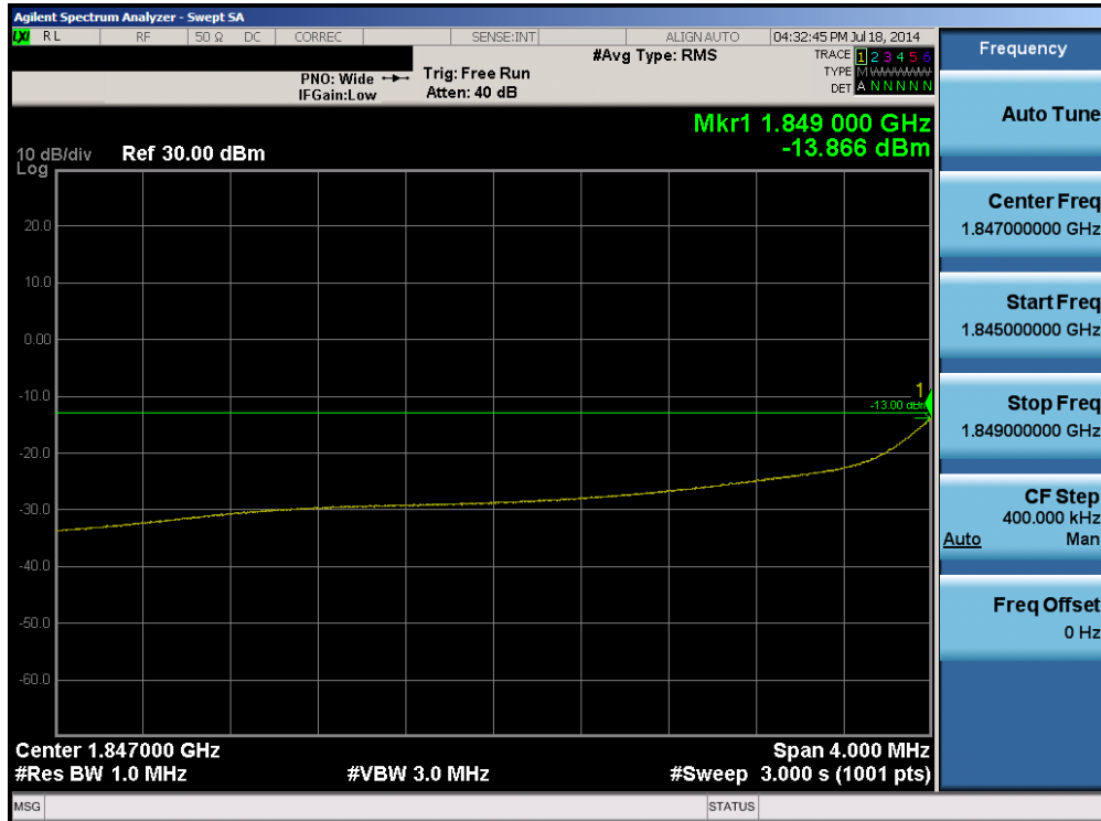
Plot 6-58. Lower Extended Band Edge Plot (Band 2 – 5.0MHz QPSK – RB Size 25)
