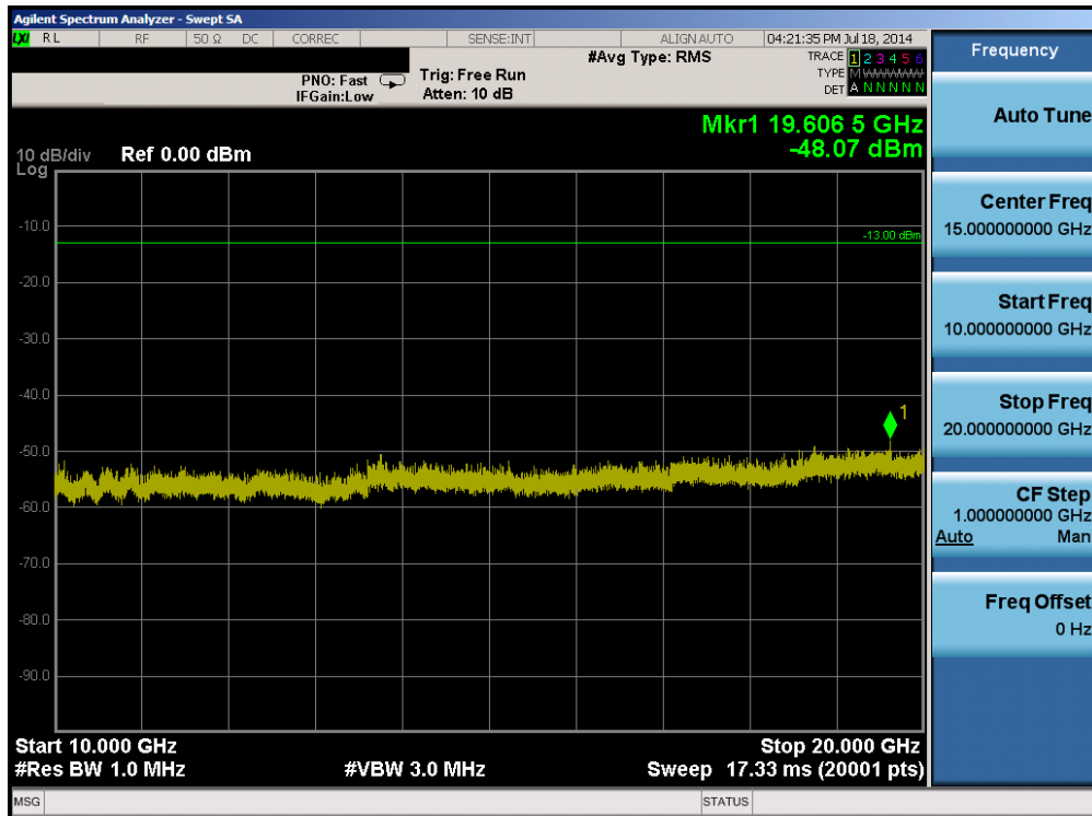
Plot 6-32. Conducted Spurious Plot (Band 2 – 1.4MHz QPSK – RB Size 1, RB Offset 0 – High Channel)
