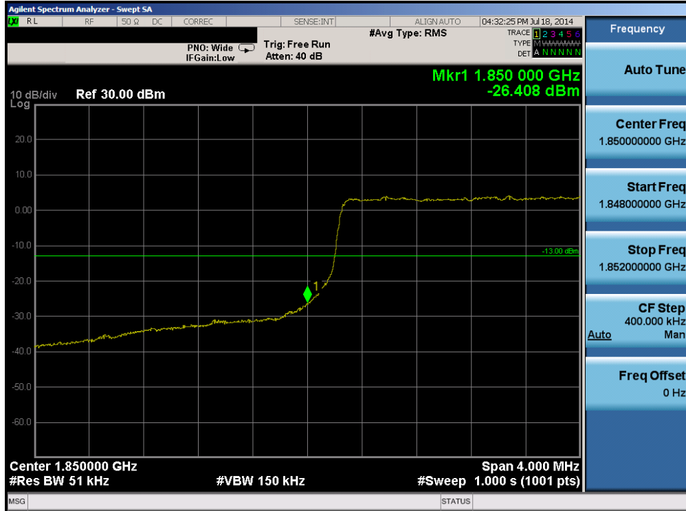
Plot 6-57. Lower Band Edge Plot (Band 2 – 5.0MHz QPSK – RB Size 25)
