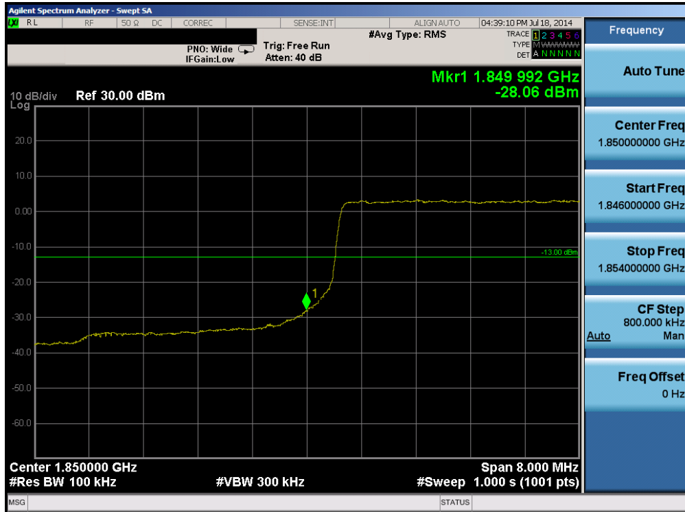
Plot 6-61. Lower Band Edge Plot (Band 2 – 10.0MHz QPSK – RB Size 50)
