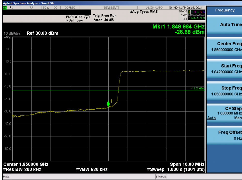
Plot 6-69. Lower Band Edge Plot (Band 2 – 20.0MHz QPSK – RB Size 100)
