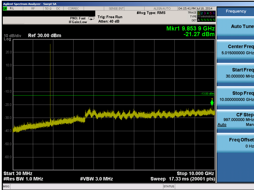
Plot 6-29. Conducted Spurious Plot (Band 2 – 1.4MHz QPSK – RB Size 1, RB Offset 0 – Mid Channel)
