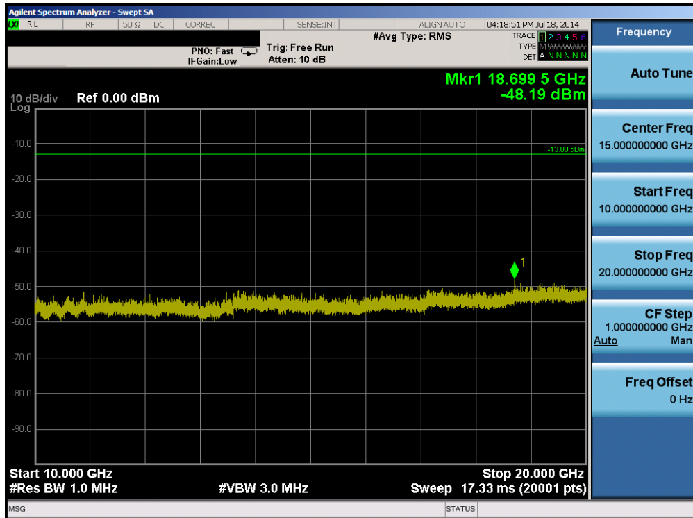
Plot 6-28. Conducted Spurious Plot (Band 2 – 1.4MHz QPSK – RB Size 1, RB Offset 0 – Low Channel)
