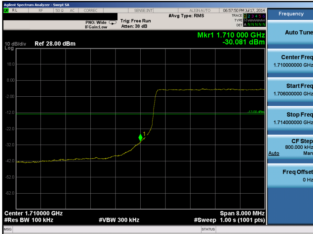
Plot 6-91. Lower Band Edge Plot (Band 4 – 10.0MHz QPSK – RB Size 50)
