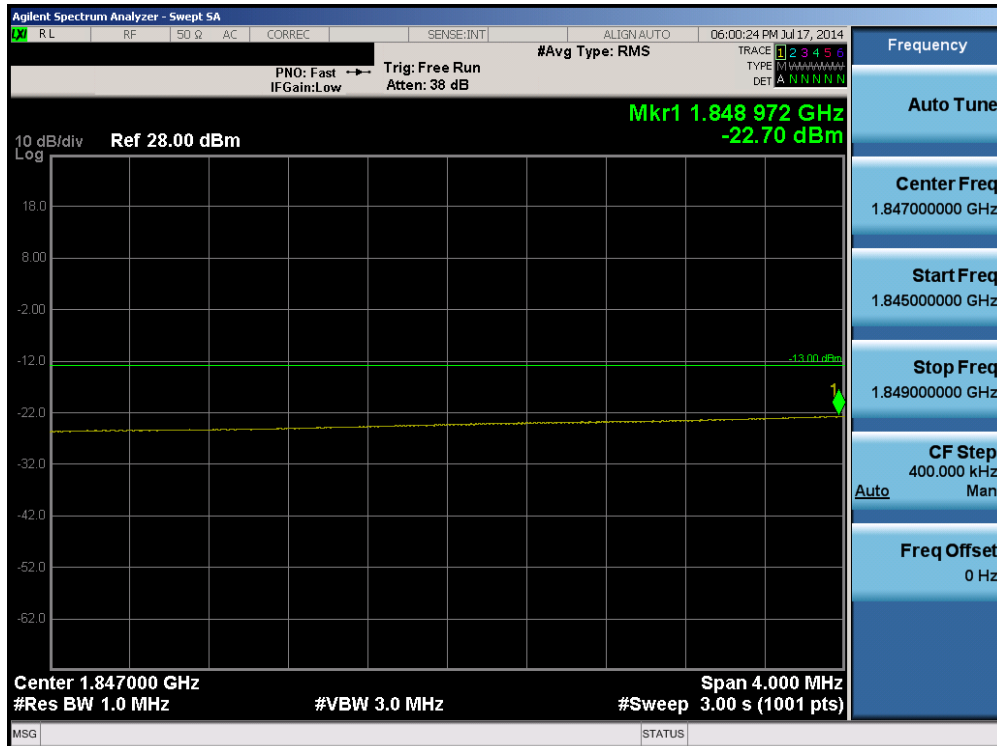
Plot 6-124. Lower Extended Band Edge Plot (Band 2 – 20.0MHz QPSK – RB Size 100)
