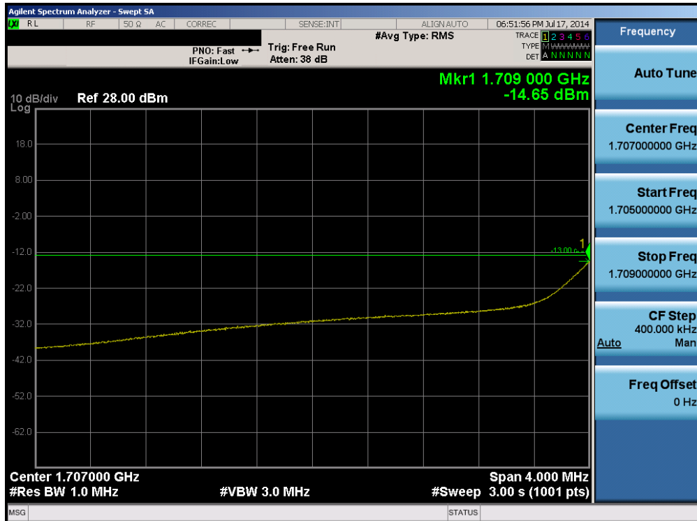
Plot 6-88. Lower Extended Band Edge Plot (Band 4 – 5.0MHz QPSK – RB Size 25)
