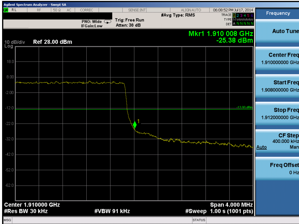
Plot 6-109. Upper Band Edge Plot (Band 2 – 3.0MHz QPSK – RB Size 15)
