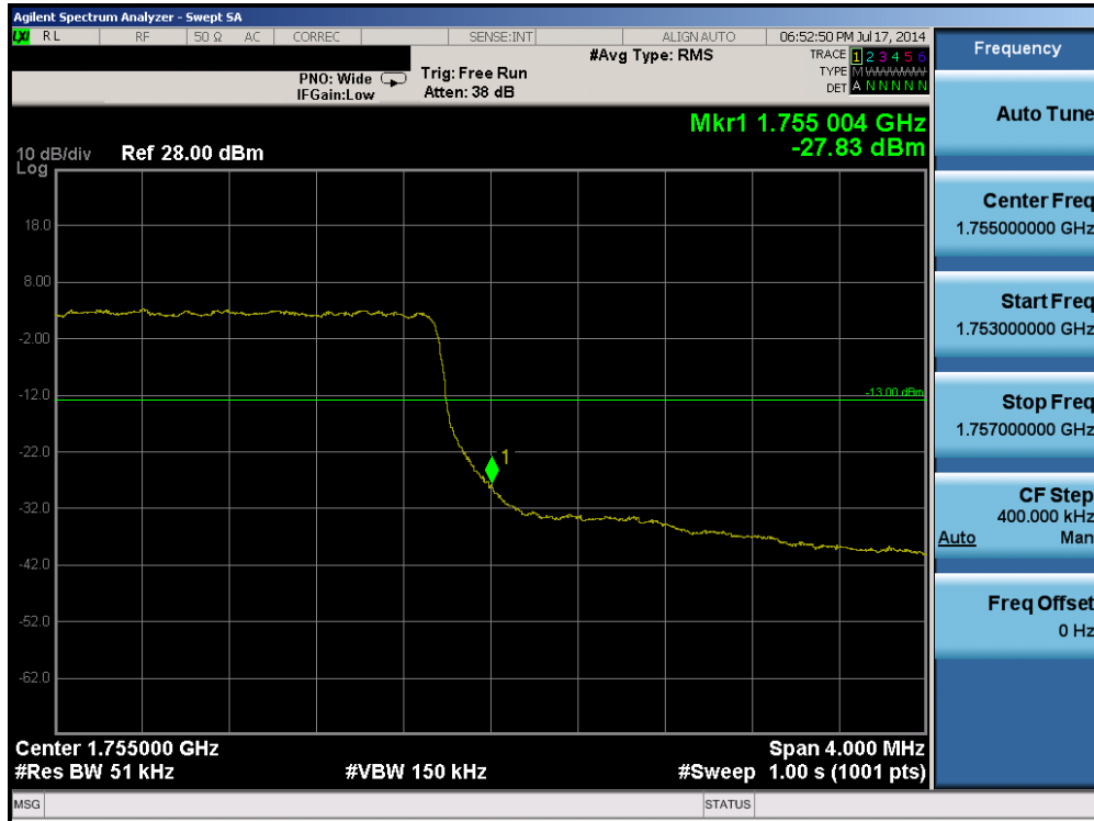
Plot 6-89. Upper Band Edge Plot (Band 4 – 5.0MHz QPSK – RB Size 25)
