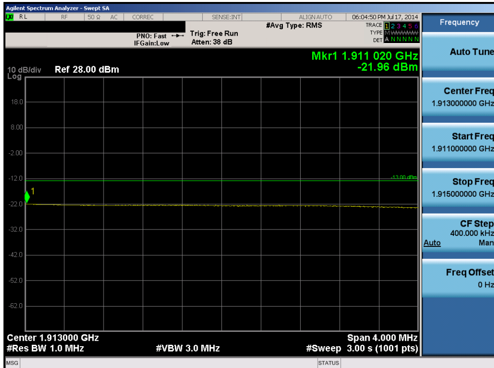
Plot 6-126. Upper Extended Band Edge Plot (Band 2 – 20.0MHz QPSK – RB Size 100)
