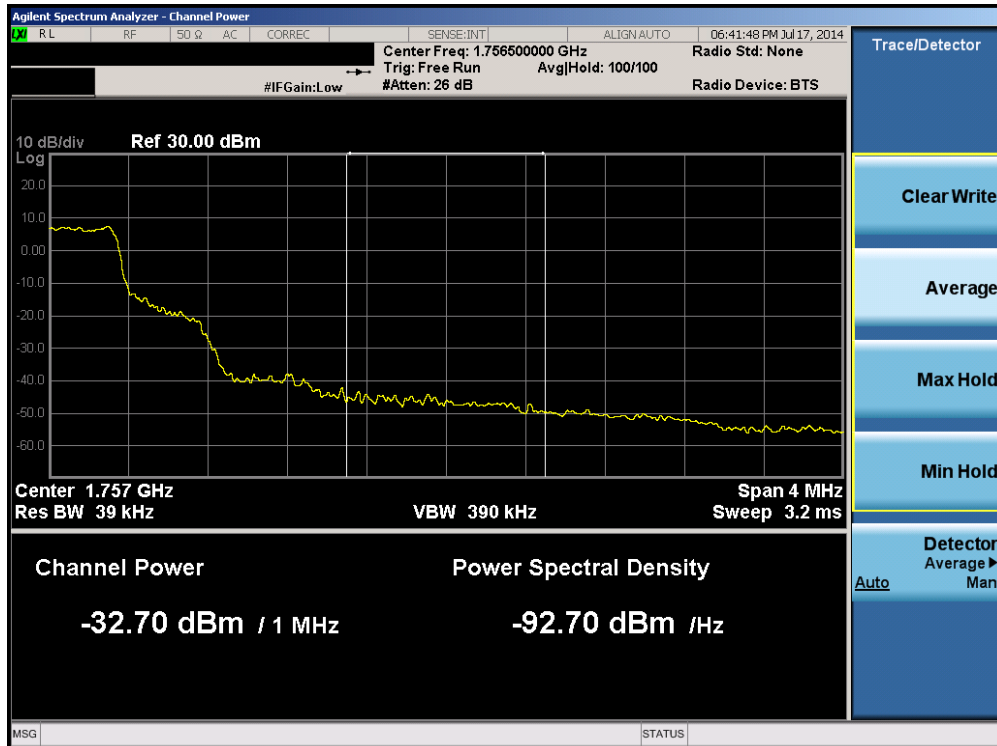
Plot 6-82. Upper Extended Band Edge Plot (Band 4 – 1.4MHz QPSK – RB Size 6)
