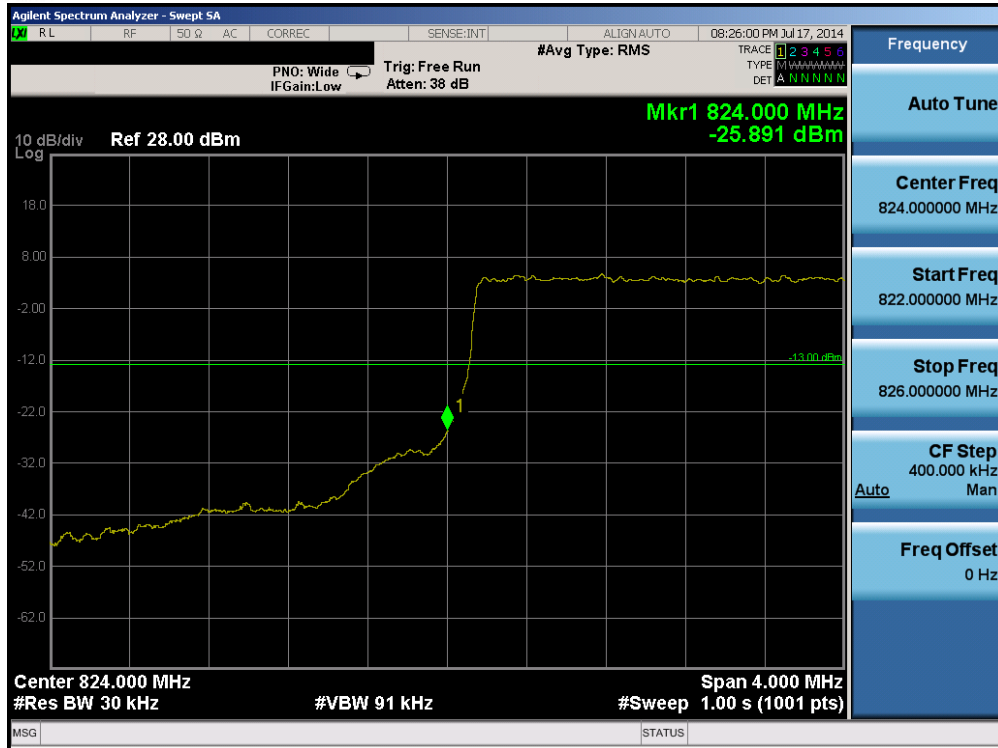
Plot 6-69. Lower Band Edge Plot (Band 5 – 3.0MHz QPSK – RB Size 15)
