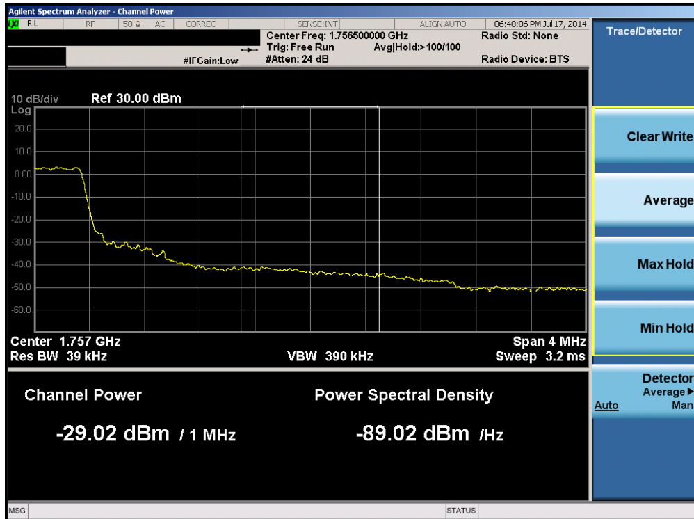
Plot 6-86. Upper Extended Band Edge Plot (Band 4 – 3.0MHz QPSK – RB Size 15)
