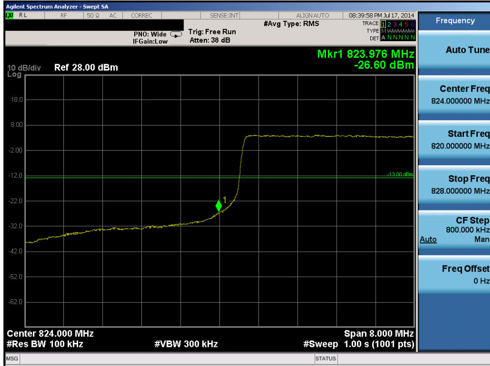
Plot 6-77. Lower Band Edge Plot (Band 5 – 10.0MHz QPSK – RB Size 50)
