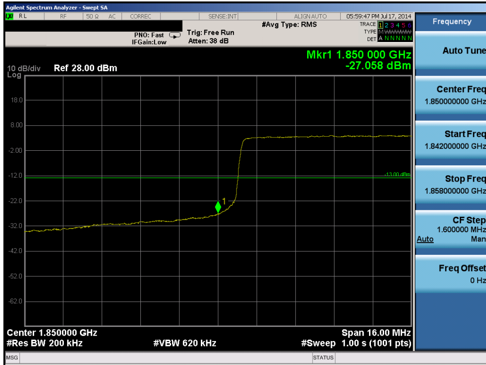
Plot 6-123. Lower Band Edge Plot (Band 2 – 20.0MHz QPSK – RB Size 100)
