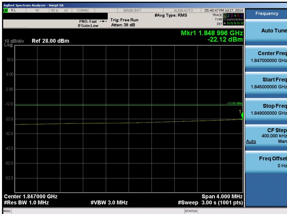
Plot 6-120. Lower Extended Band Edge Plot (Band 2 – 15.0MHz QPSK – RB Size 75)
