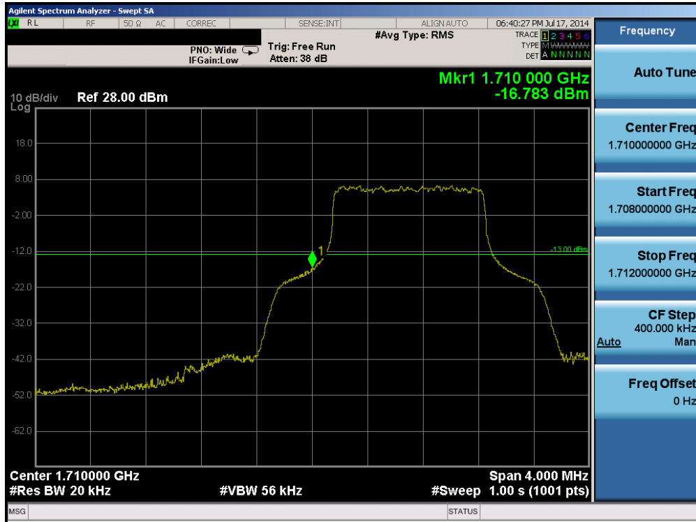
Plot 6-79. Lower Band Edge Plot (Band 4 – 1.4MHz QPSK – RB Size 6)
