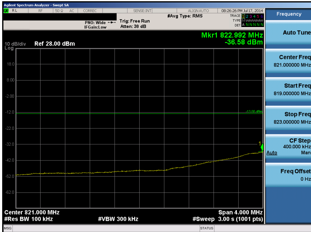
Plot 6-70. Lower Extended Band Edge Plot (Band 5 – 3.0MHz QPSK – RB Size 15)
