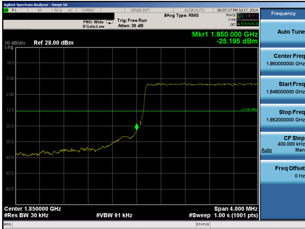
Plot 6-107. Lower Band Edge Plot (Band 2 – 3.0MHz QPSK – RB Size 15)
