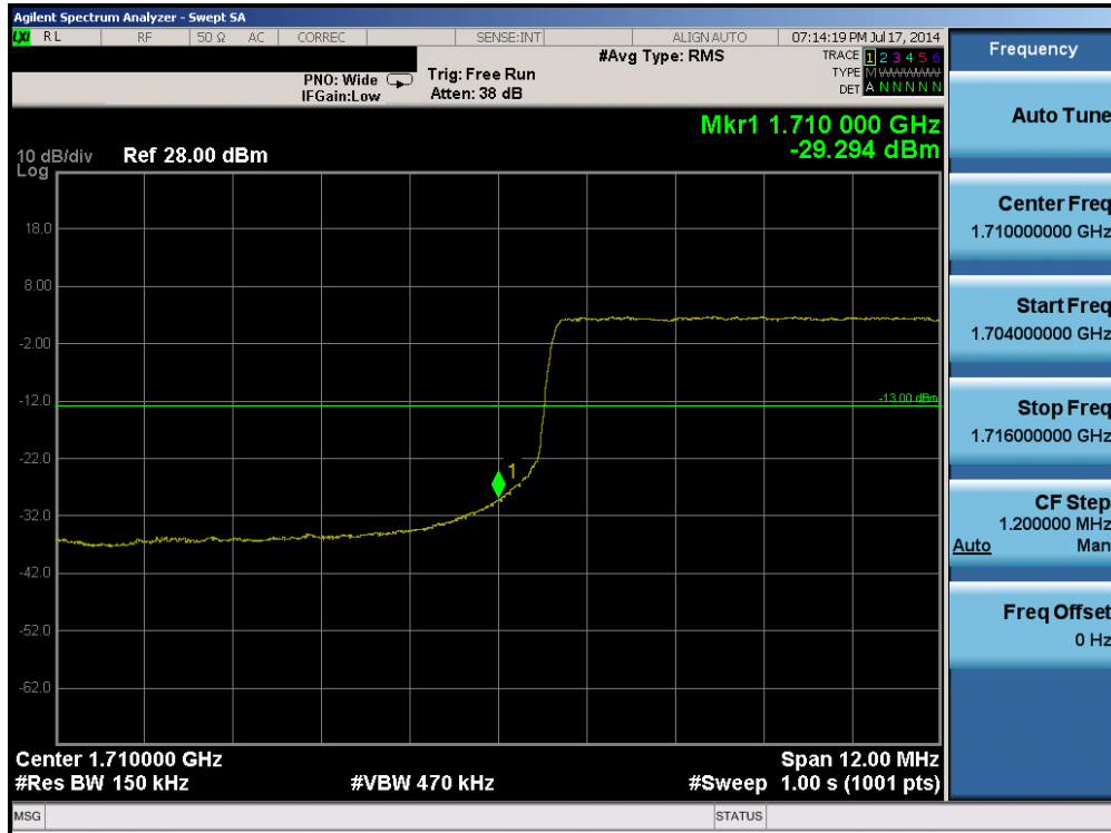
Plot 6-95. Lower Band Edge Plot (Band 4 – 15.0MHz QPSK – RB Size 75)
