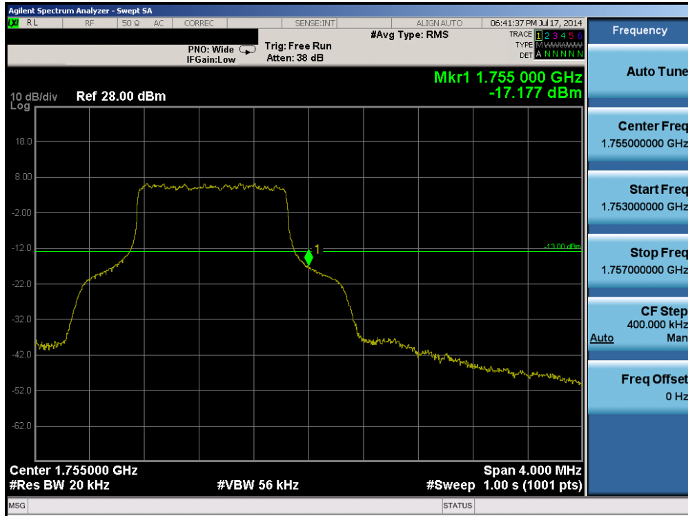
Plot 6-81. Upper Band Edge Plot (Band 4 – 1.4MHz QPSK – RB Size 6)
