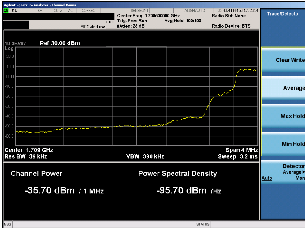
Plot 6-80. Lower Extended Band Edge Plot (Band 4 – 1.4MHz QPSK – RB Size 6)
