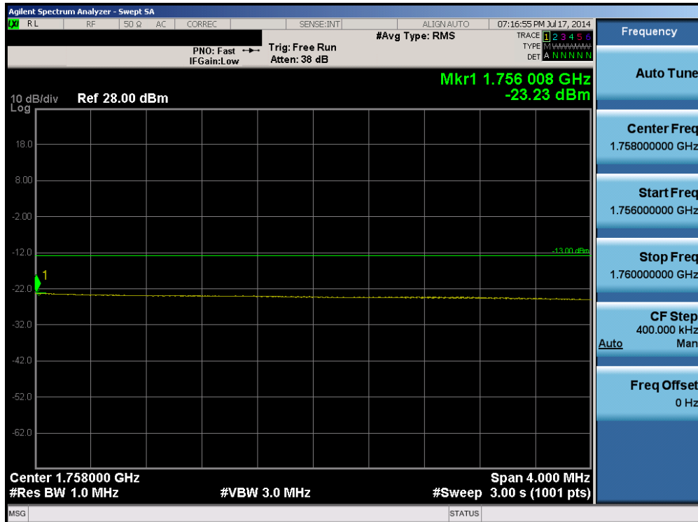
Plot 6-98. Upper Extended Band Edge Plot (Band 4 – 15.0MHz QPSK – RB Size 75)
