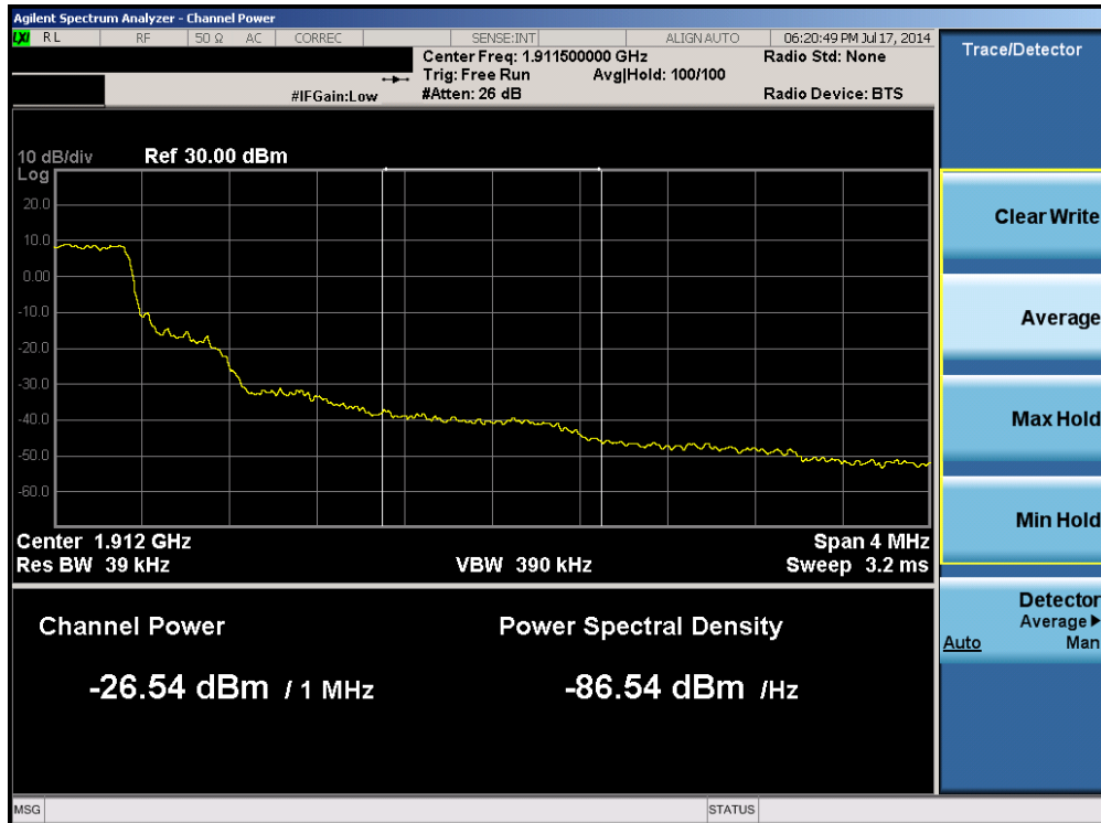
Plot 6-106. Upper Extended Band Edge Plot (Band 2 – 1.4MHz QPSK – RB Size 6)
