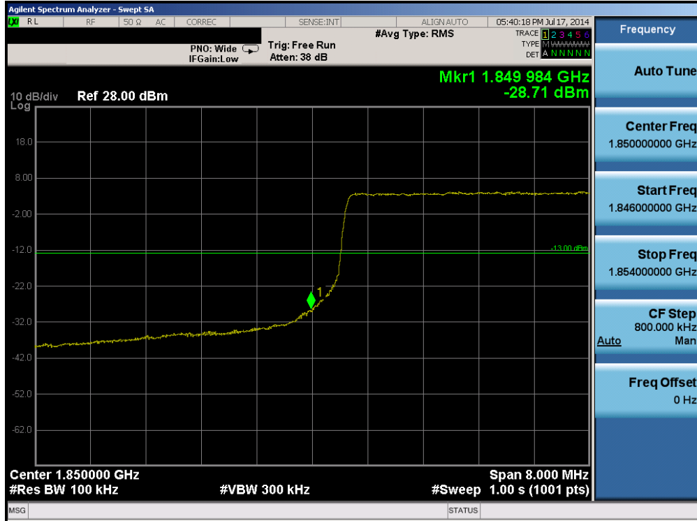
Plot 6-115. Lower Band Edge Plot (Band 2 – 10.0MHz QPSK – RB Size 50)
