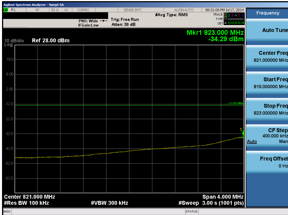
Plot 6-74. Lower Extended Band Edge Plot (Band 5 – 5.0MHz QPSK – RB Size 25)
