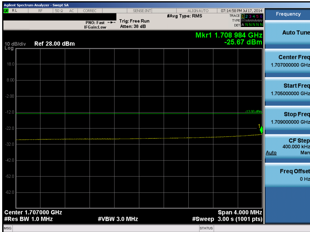
Plot 6-96. Lower Extended Band Edge Plot (Band 4 – 15.0MHz QPSK – RB Size 75)
