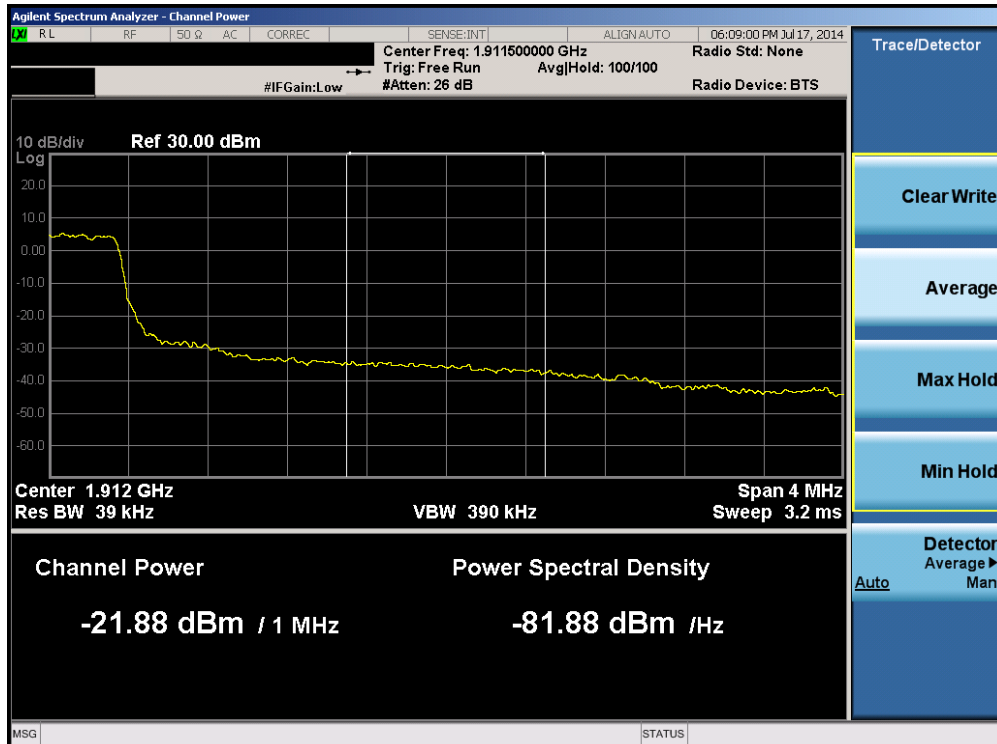
Plot 6-110. Upper Extended Band Edge Plot (Band 2 – 3.0MHz QPSK – RB Size 15)
