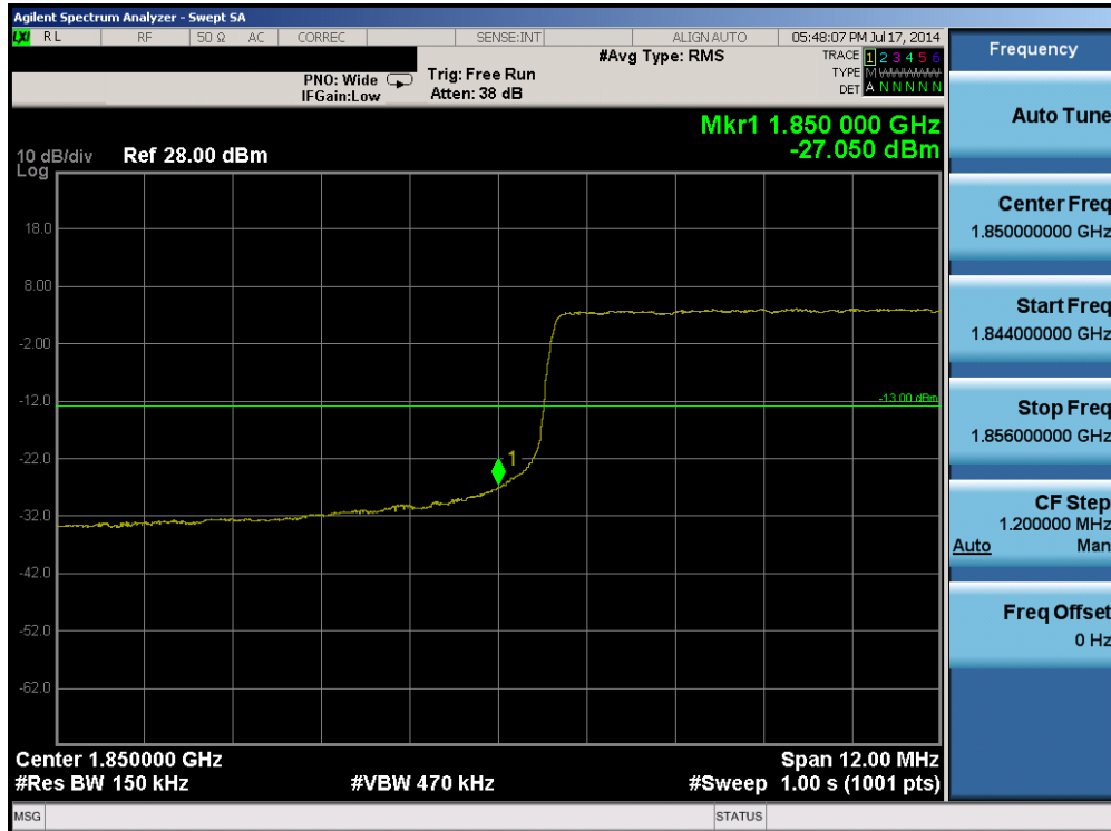
Plot 6-119. Lower Band Edge Plot (Band 2 – 15.0MHz QPSK – RB Size 75)
