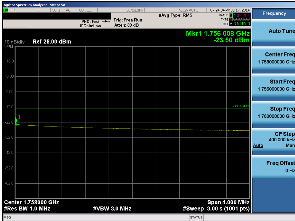
Plot 6-102. Upper Extended Band Edge Plot (Band 4 – 20.0MHz QPSK – RB Size 100)
