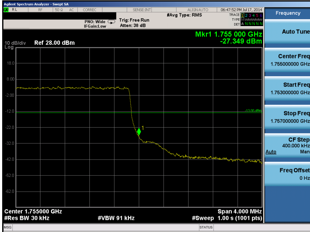
Plot 6-85. Upper Band Edge Plot (Band 4 – 3.0MHz QPSK – RB Size 15)
