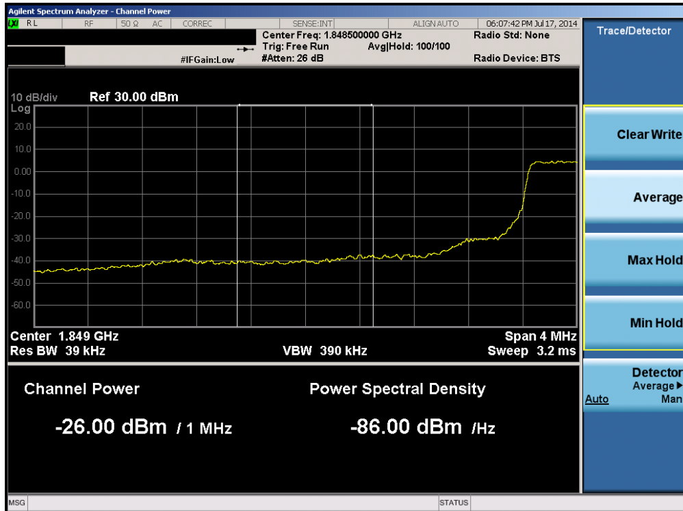
Plot 6-108. Lower Extended Band Edge Plot (Band 2 – 3.0MHz QPSK – RB Size 15)
