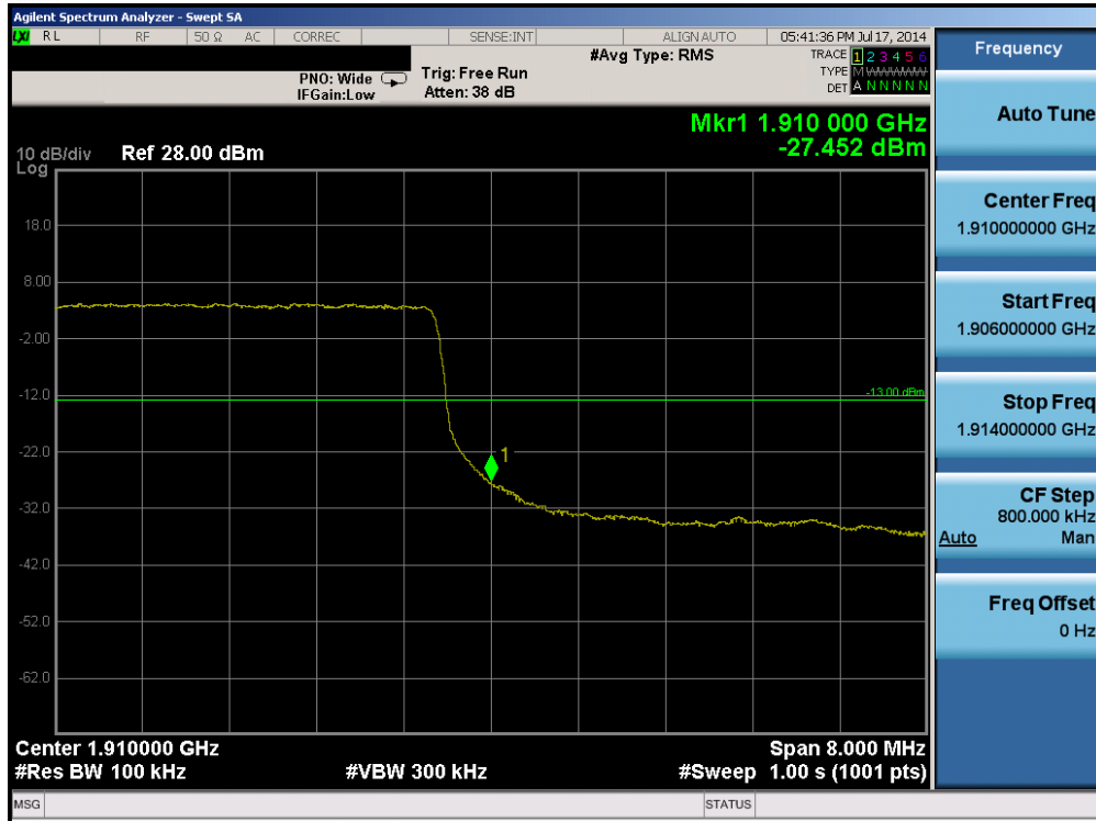
Plot 6-117. Upper Band Edge Plot (Band 2 – 10.0MHz QPSK – RB Size 50)
