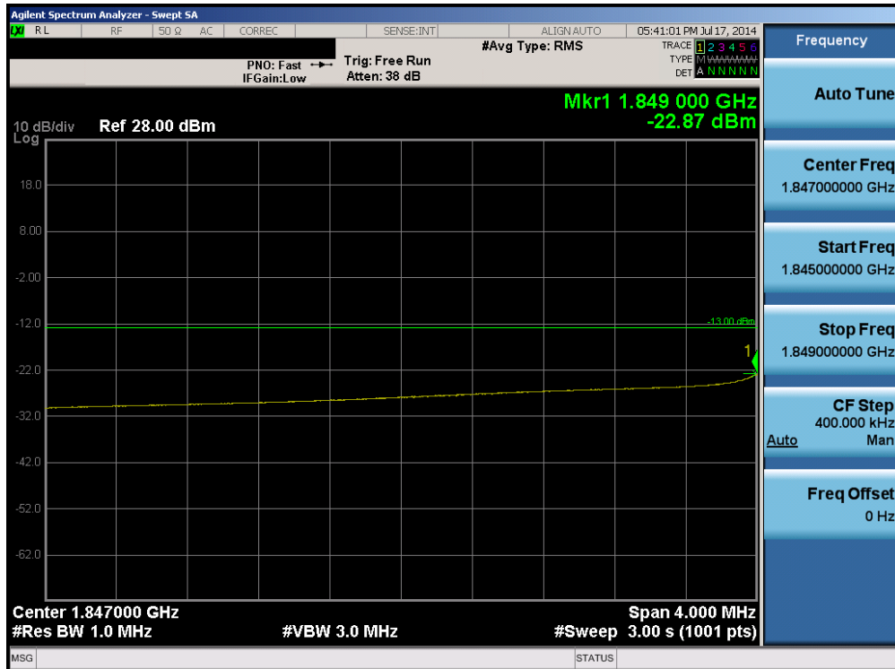
Plot 6-116. Lower Extended Band Edge Plot (Band 2 – 10.0MHz QPSK – RB Size 50)
