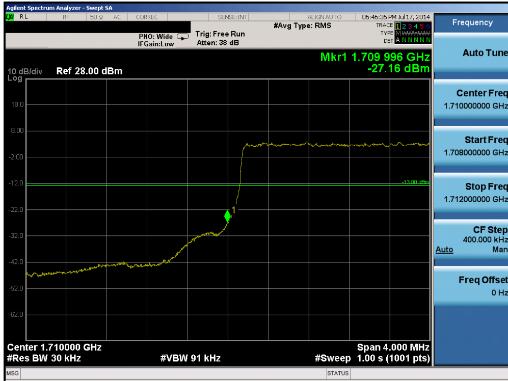
Plot 6-83. Lower Band Edge Plot (Band 4 – 3.0MHz QPSK – RB Size 15)
