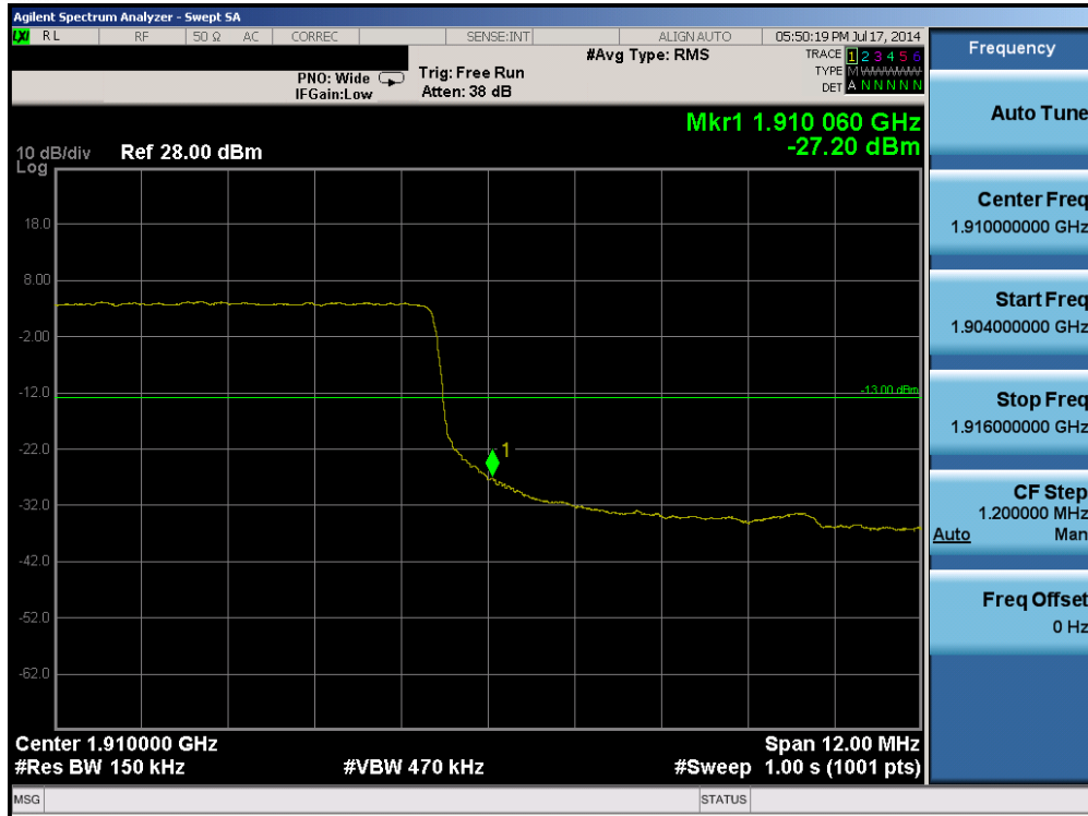
Plot 6-121. Upper Band Edge Plot (Band 2 – 15.0MHz QPSK – RB Size 75)
