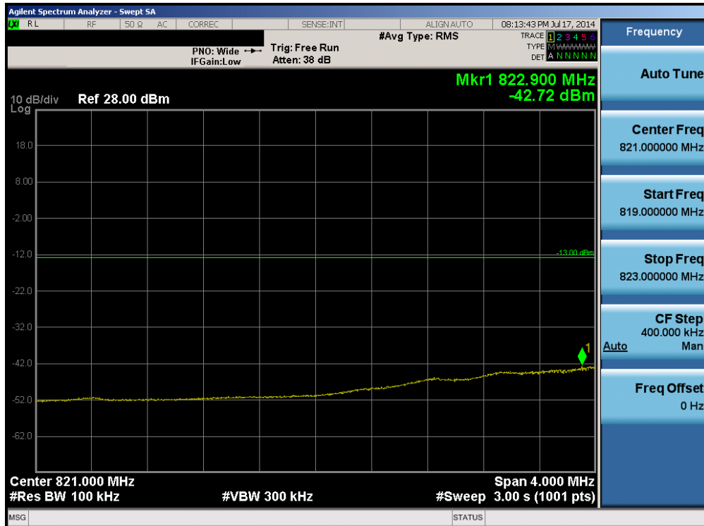
Plot 6-66. Lower Extended Band Edge Plot (Band 5 – 1.4MHz QPSK – RB Size 6)
