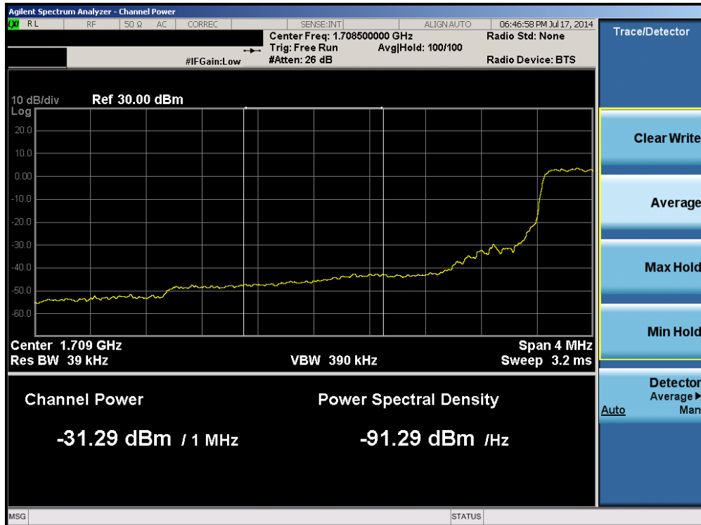
Plot 6-84. Lower Extended Band Edge Plot (Band 4 – 3.0MHz QPSK – RB Size 15)
