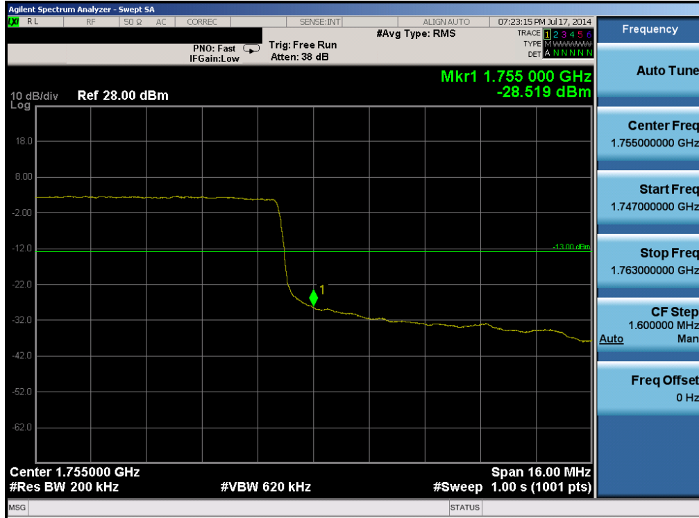
Plot 6-101. Upper Band Edge Plot (Band 4 – 20.0MHz QPSK – RB Size 100)
