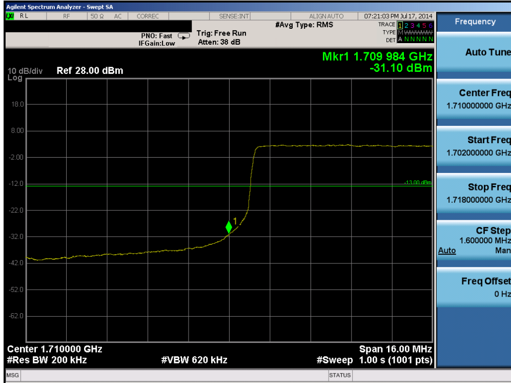
Plot 6-99. Lower Band Edge Plot (Band 4 – 20.0MHz QPSK – RB Size 100)
