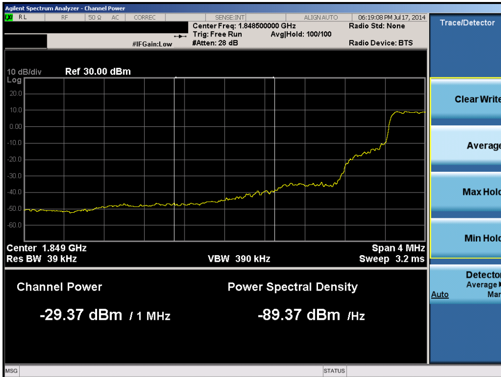
Plot 6-104. Lower Extended Band Edge Plot (Band 2 – 1.4MHz QPSK – RB Size 6)
