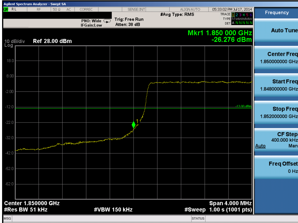
Plot 6-111. Lower Band Edge Plot (Band 2 – 5.0MHz QPSK – RB Size 25)
