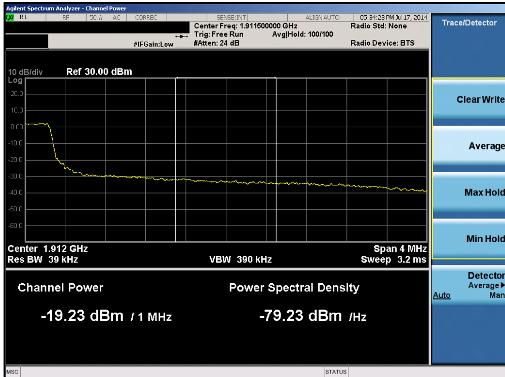
Plot 6-114. Upper Extended Band Edge Plot (Band 2 – 5.0MHz QPSK – RB Size 25)
