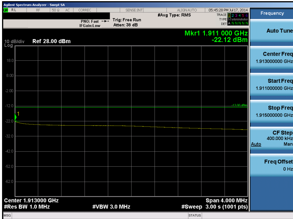
Plot 6-118. Upper Extended Band Edge Plot (Band 2 – 10.0MHz QPSK – RB Size 50)
