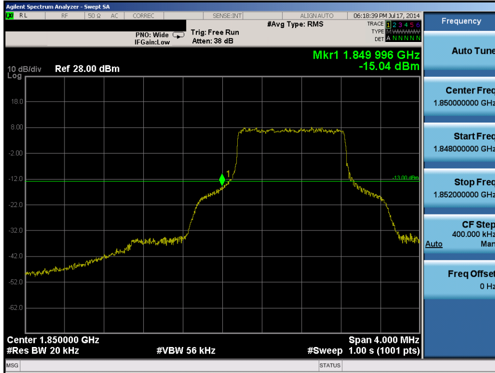
Plot 6-103. Lower Band Edge Plot (Band 2 – 1.4MHz QPSK – RB Size 6)
