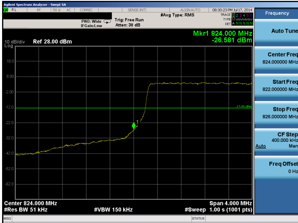
Plot 6-73. Lower Band Edge Plot (Band 5 – 5.0MHz QPSK – RB Size 25)
