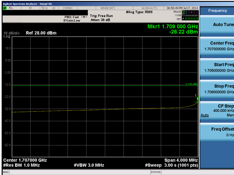
Plot 6-92. Lower Extended Band Edge Plot (Band 4 – 10.0MHz QPSK – RB Size 50)
