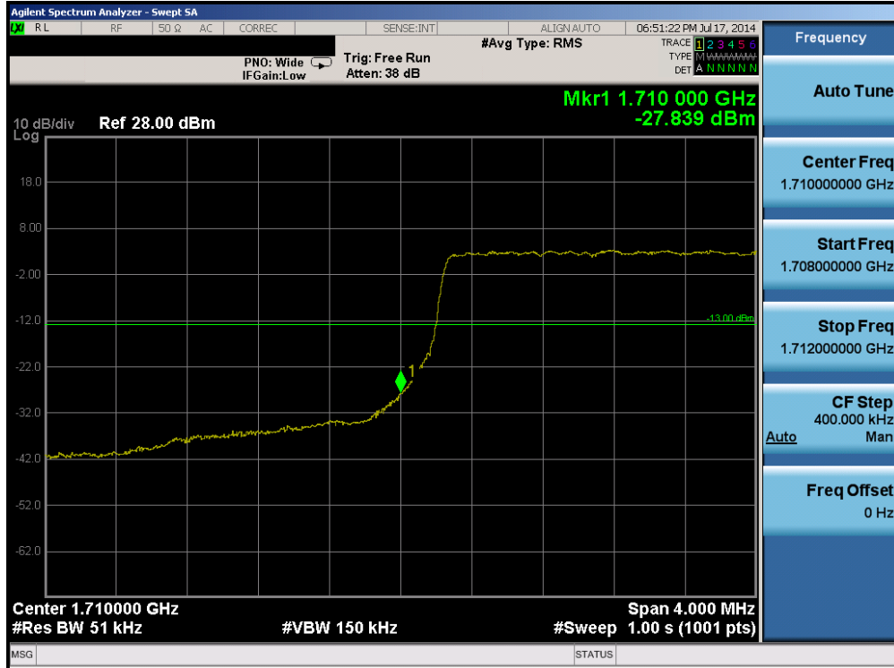
Plot 6-87. Lower Band Edge Plot (Band 4 – 5.0MHz QPSK – RB Size 25)
