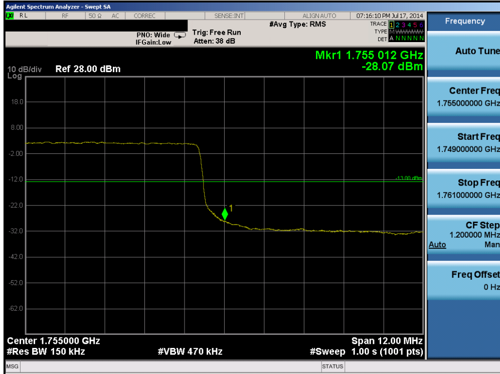
Plot 6-97. Upper Band Edge Plot (Band 4 – 15.0MHz QPSK – RB Size 75)
