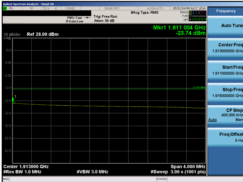
Plot 6-122. Upper Extended Band Edge Plot (Band 2 – 15.0MHz QPSK – RB Size 75)
