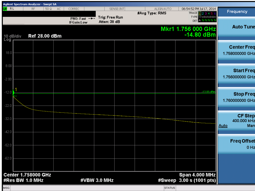
Plot 6-90. Upper Extended Band Edge Plot (Band 4 – 5.0MHz QPSK – RB Size 25)
