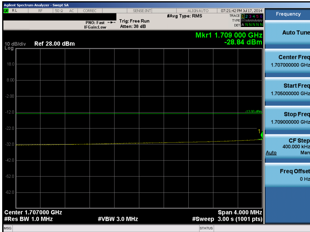
Plot 6-100. Lower Extended Band Edge Plot (Band 4 – 20.0MHz QPSK – RB Size 100)
