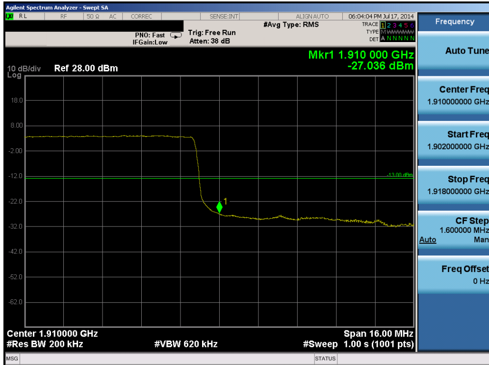
Plot 6-125. Upper Band Edge Plot (Band 2 – 20.0MHz QPSK – RB Size 100)
