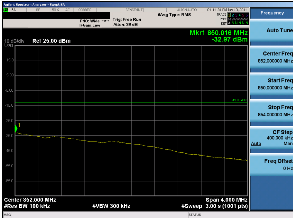
Plot 6-44. Upper Extended Band Edge Plot (Band 5 – 5.0MHz QPSK – RB Size 25)
